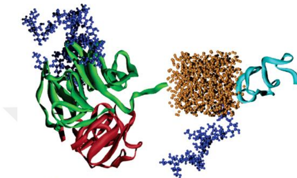
Figure 2.9. Molecular structure of vitronectin [113]. The green: central domain, the red: heparin-binding domain, and the blue: carbohydrates.
