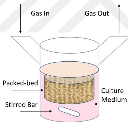
Figure 2.4. Schematic diagram of packed-bed bioreactor.
