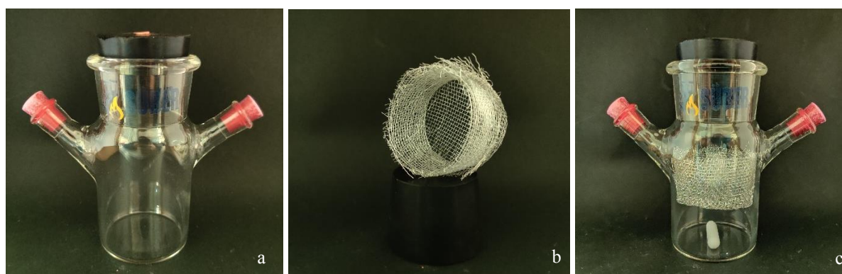
Figure 3. 2. Photographs showing the main parts of packed-bed bioreactor, a) Glass body, b) the basket, c) packed-bed bioreactor with all units.
