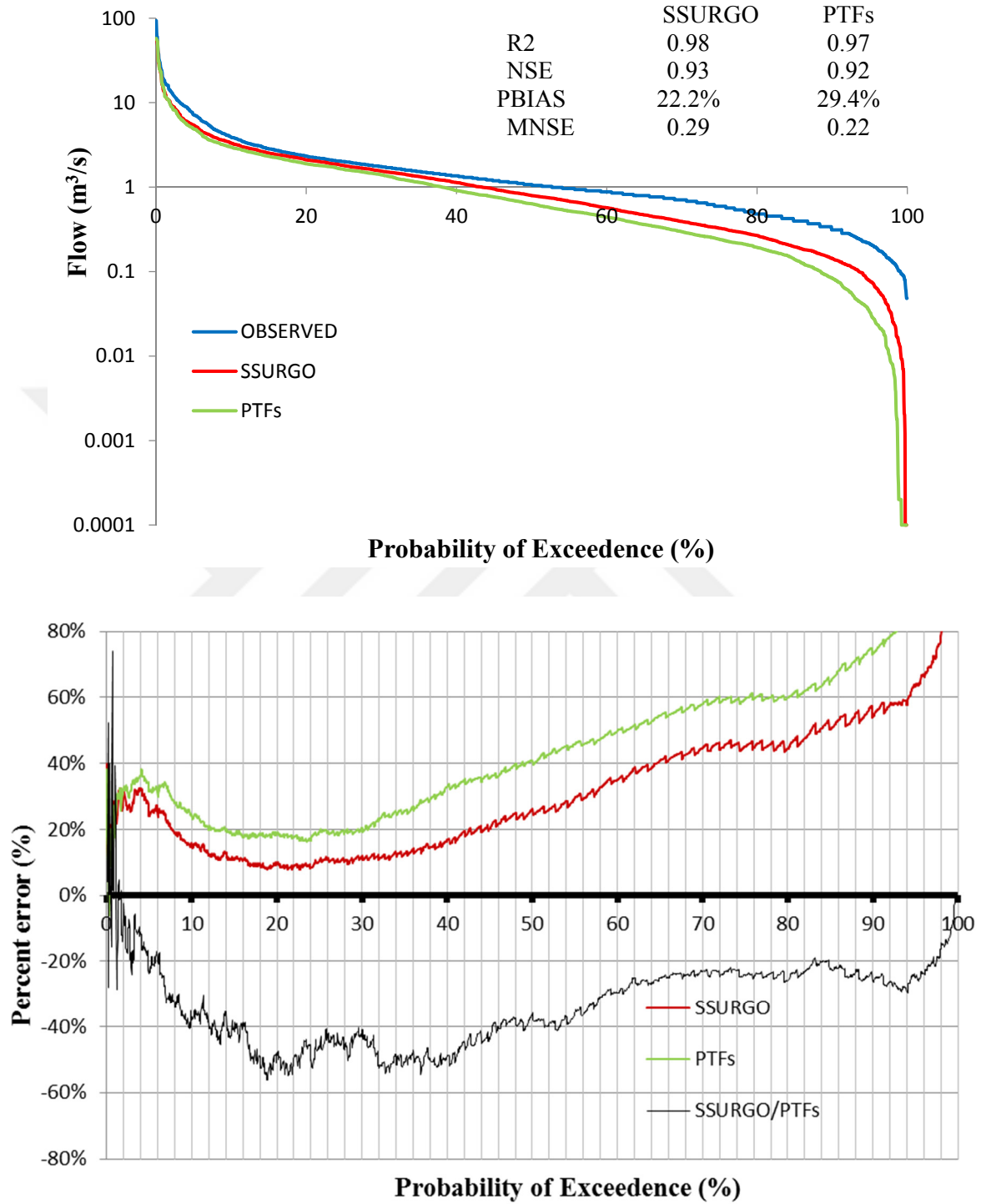
Figure 3.8: Flow duration curves (FDCs) (above) and percent error graph (below) in Suwanee Creek Watershed with MNSE objective function ( p=0.25 ) for the SSURGO and UPDATED soil. The black line in the error graph was calculated as \left[Ratio = \frac{(\epsilon_{SSURGO})}{(\epsilon_{PTF})} - 1\right] , where \epsilon_{SSURGO} and \epsilon_{PTF} are percent errors of PTF and SSURGO based simulations.
