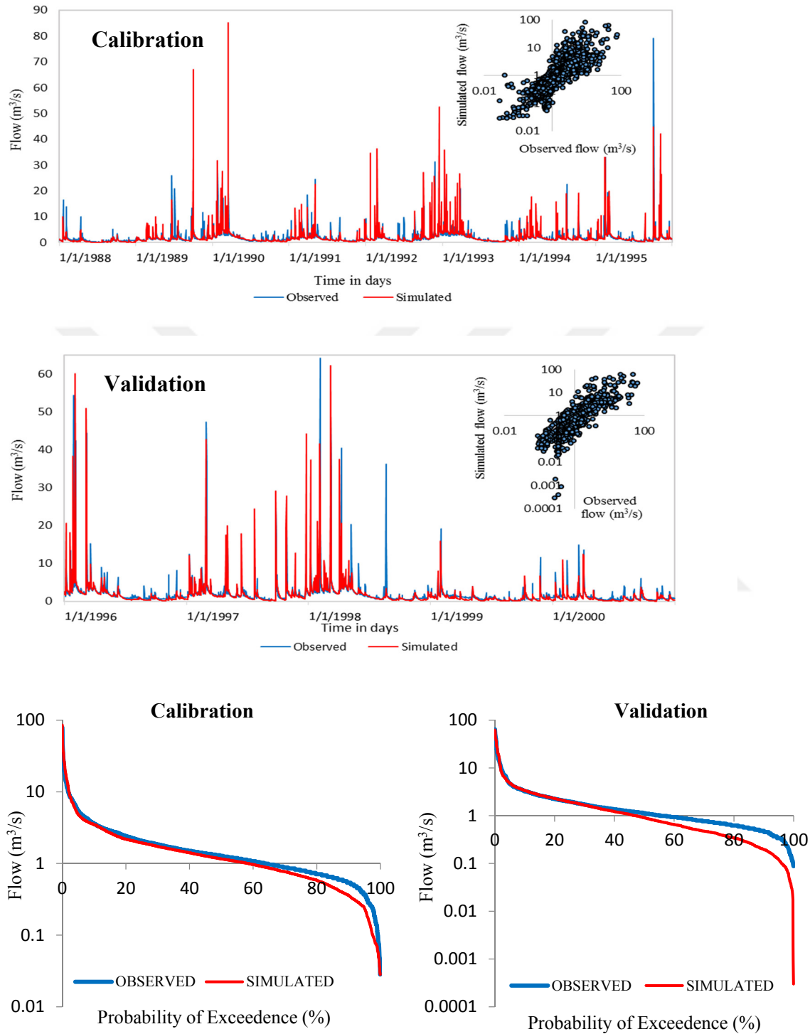
Figure 3.4: Observed and simulated daily streamflow during calibration and validation periods for the best performance scatter plots of simulated and observed streamflow in Suwanee Creek Watershed with MNSE objective function ( p=0.25 ). Flow duration curves (FDCs) for the calibration (1988-1995) and validation (1996-2000) periods.
