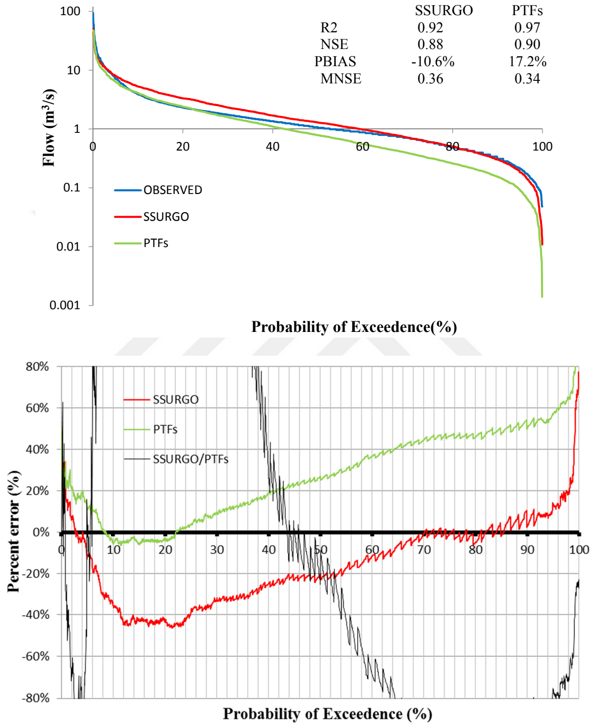
Figure 3.7: Flow duration curves (FDCs) (above) and percent error graph (below) in Suwanee Creek Watershed with NSE objective function for the SSURGO and UPDATED soil. The black line in the error graph was calculated as \left[Ratio = \frac{(\epsilon_{SSURGO})}{(\epsilon_{PTF})} - 1\right] , where \epsilon_{SSURGO} and \epsilon_{PTF} are percent errors of PTF and SSURGO based simulations.
