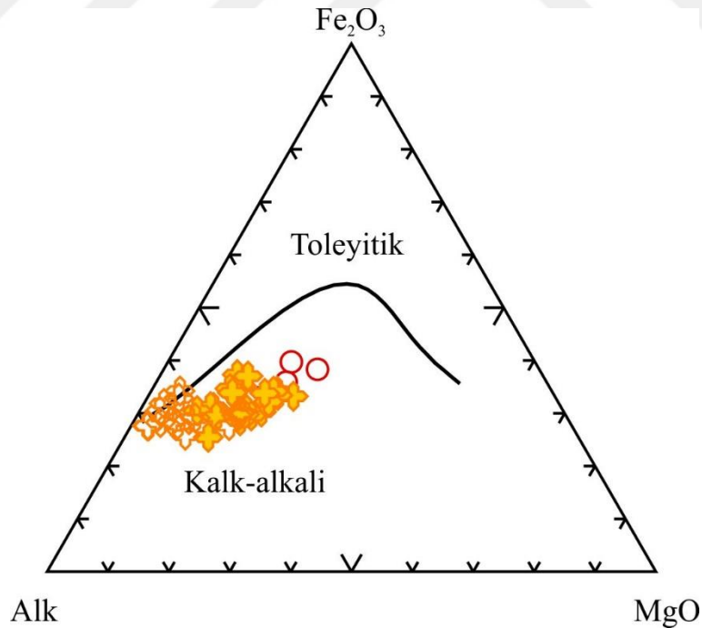
Şekil 6.2. AFM (Alk: \text{Na}_2\text{O}+\text{K}_2\text{O} - \text{Fe}_2\text{O}_3 - \text{MgO} ) diyagramı (Irvine ve Baragar, 1971).
