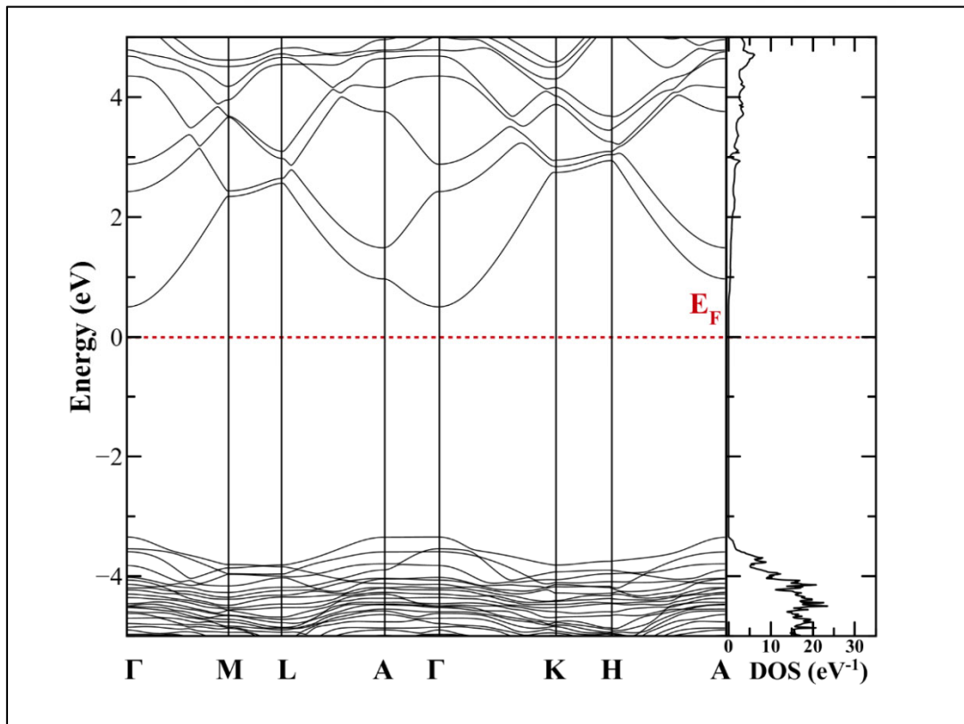
Figure 5.14. The band structure and density of states wz\text{-Mg}_{0.3125}\text{Zn}_{0.6875}\text{O}
