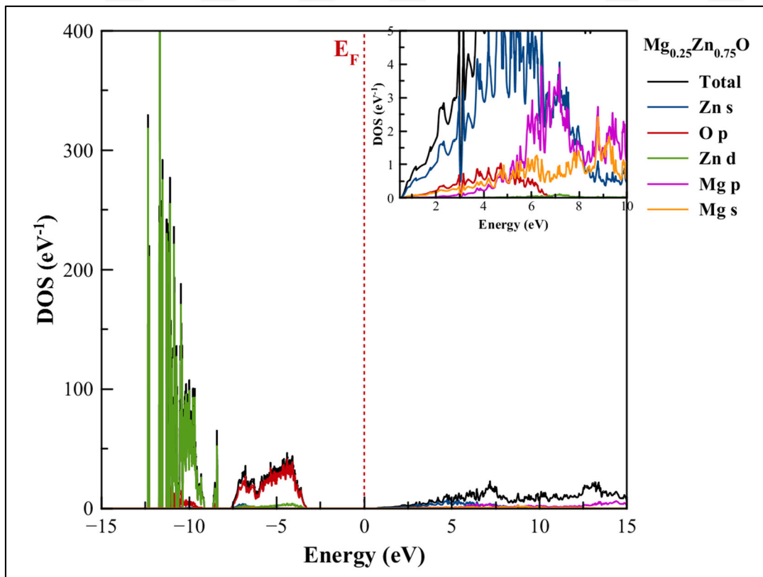
Figure 5.18. The partial density of states W-Mg 0.25 Zn 0.75 O
