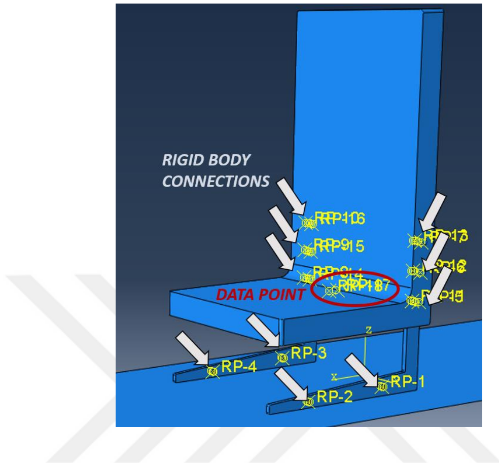
Figure 25: Reference points created on the seat model
