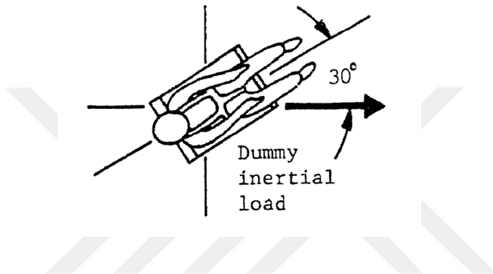
Figure 15: Seat/restraint system dynamic test 2 [17]
