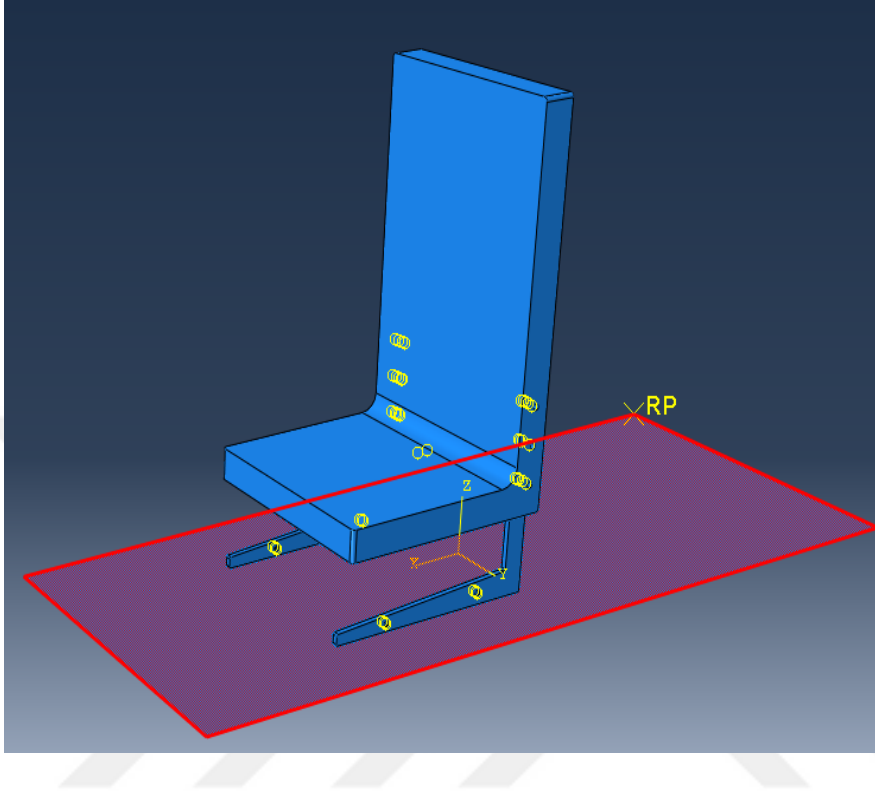
Figure 36: Reference point of rigid wall
