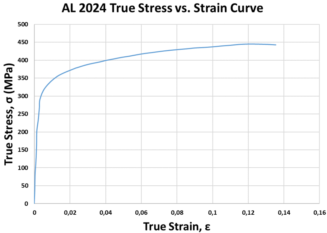
Figure 34: True stress-strain diagram of AL 2024 [23]
