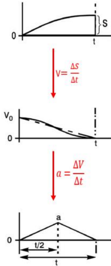
Figure 8: Displacement, velocity & acceleration relations during a crash event
