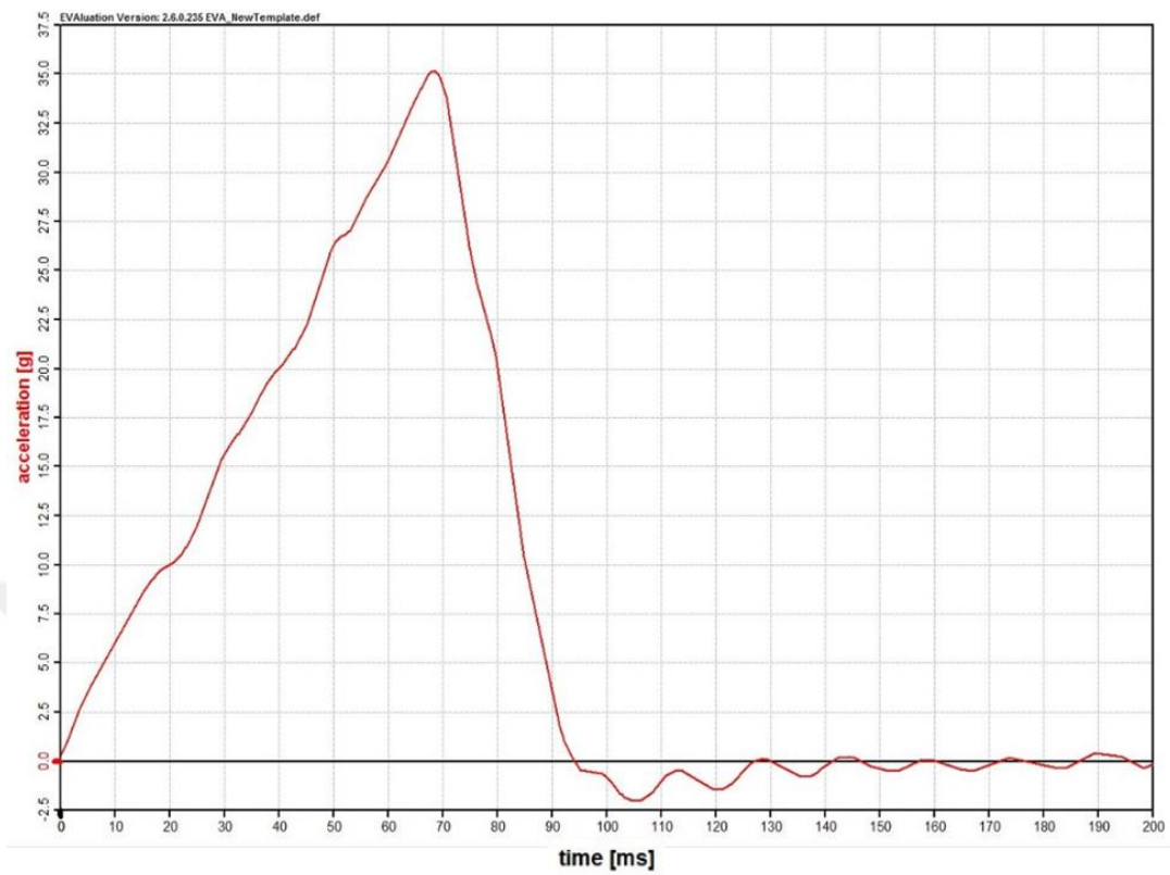
Figure 50: Acceleration time history of test fixture
