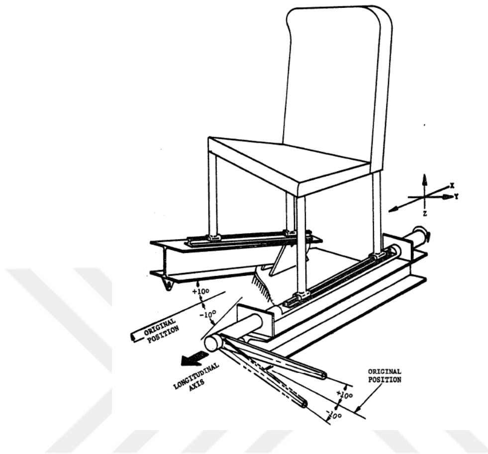
Figure 16: Floor warpage requirement [17]
