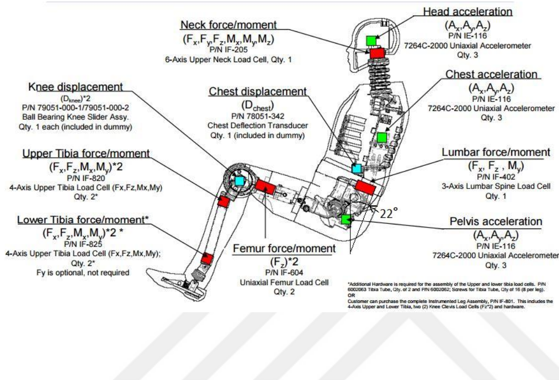
Figure 49: Accelerometer and load cell positions on Hybrid III test dummy
