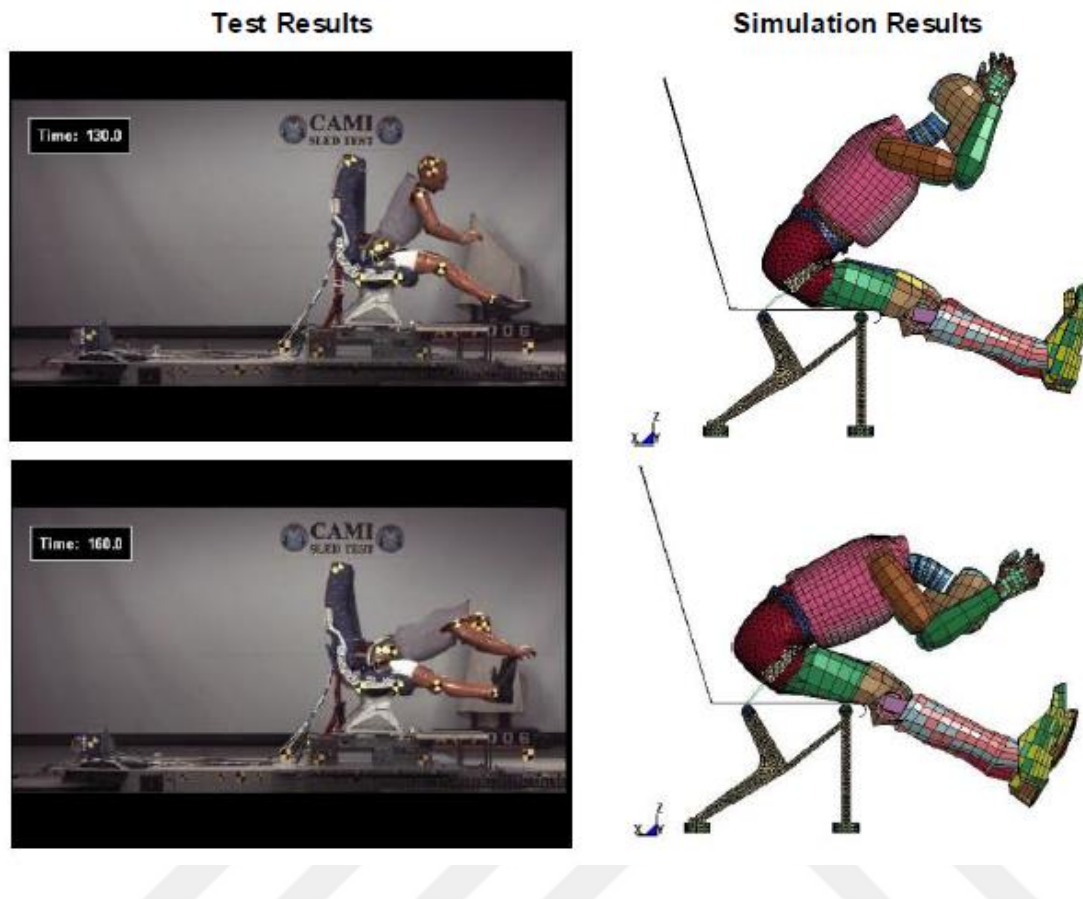
Figure 2: Comparison of test and simulation results [10]
