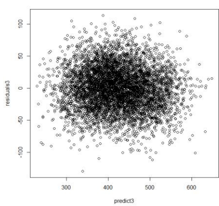
Figure 5. Residual plots emerged from data set 1, data set 2 and data set 3.
