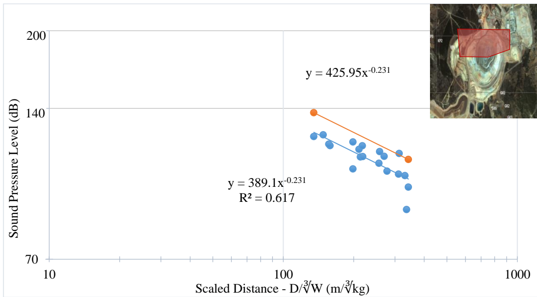
Figure 5.31 Katrancilar presplit blasting air blast overpressure levels in dB (Pit location- NE, N, NW, W- in front of the pit)
