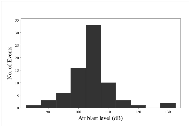
Figure 4.39 Gümüşkol Path 2 production blasting air blast histogram
