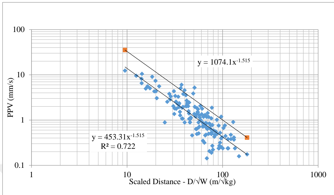
Figure 5.4 Katrancilar unclassified production blasting PPV values
