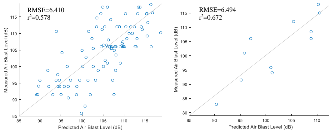
Figure 6.10 Predicted vs measured air blast levels for modeling set and testing set, respectively
