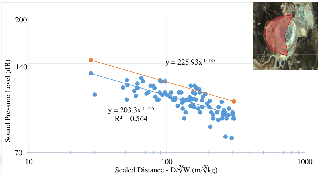
Figure 5.57 Karapınar production blasting air blast overpressure levels in dB (Pit location- NE, N, W, S, SSE - in front of the pit)
