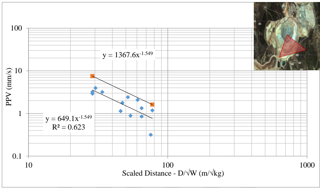
Figure 5.23 Gümüşkol Path 2 production blasting PPV values (Pit location- S, SSE, SE - in front of the pit)
