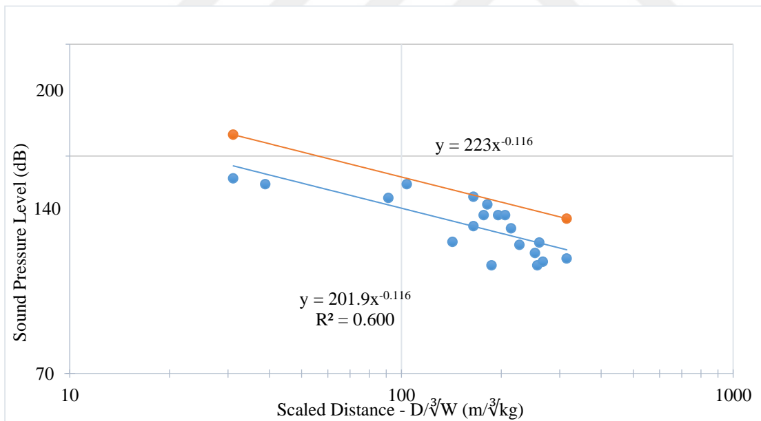
Figure 5.35 Karapınar presplit blasting air blast overpressure levels in dB (Eastern winds-N, NE, E, SSE, SE)
