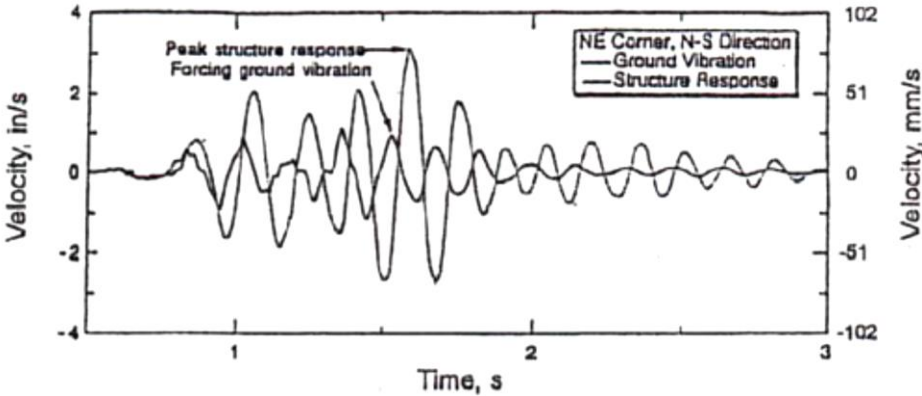
Figure 2.16 Ground and structure vibrations with frequency of 5.8 Hz near structure resonance from Siskind (2000) (Svinkin, 2008)
