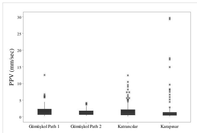
Figure 4.18 Boxplots of PPV from production blasts with respect to villages
