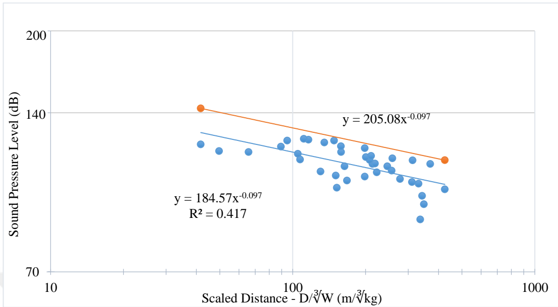
Figure 5.29 Katrancilar presplit blasting air blast overpressure levels in dB (Northern winds-N, NE, NW)
