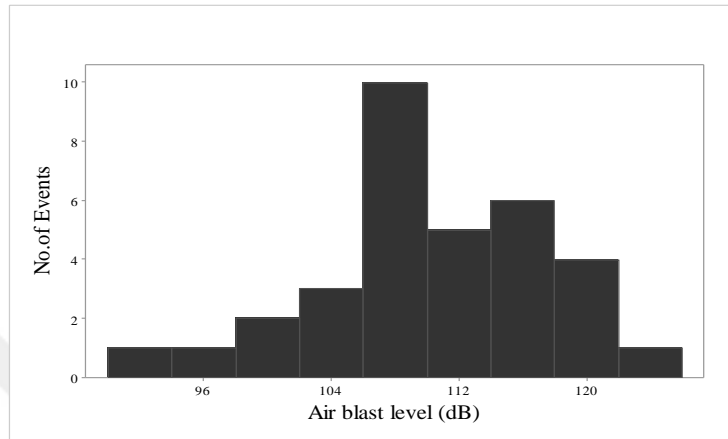
Figure 4.37 Gümüşkol Path 2 presplit blasting air blast histogram
