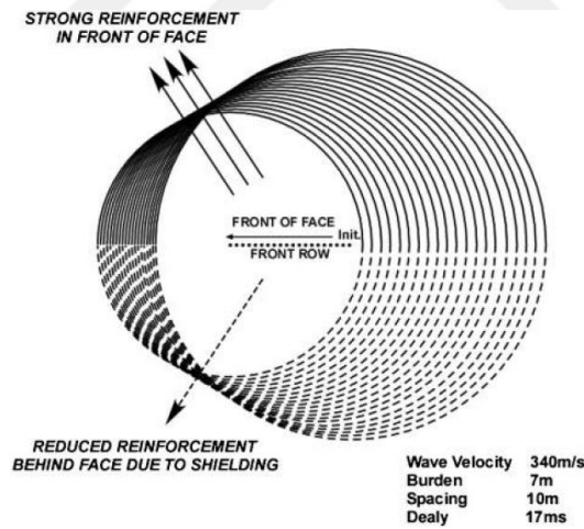
Figure 2.12 Wavefront diagram showing reinforcement (Richards, 2013)
