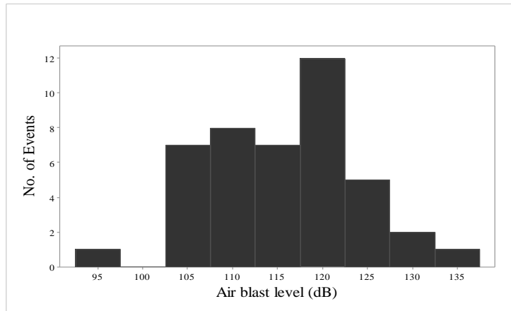
Figure 4.32 Gümüşkol Path 1 presplit blasting air blast histogram
