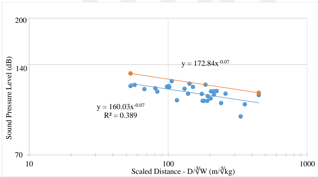
Figure 5.38 Gümüşkol Path 1 unclassified presplit blasting air blast overpressure levels
