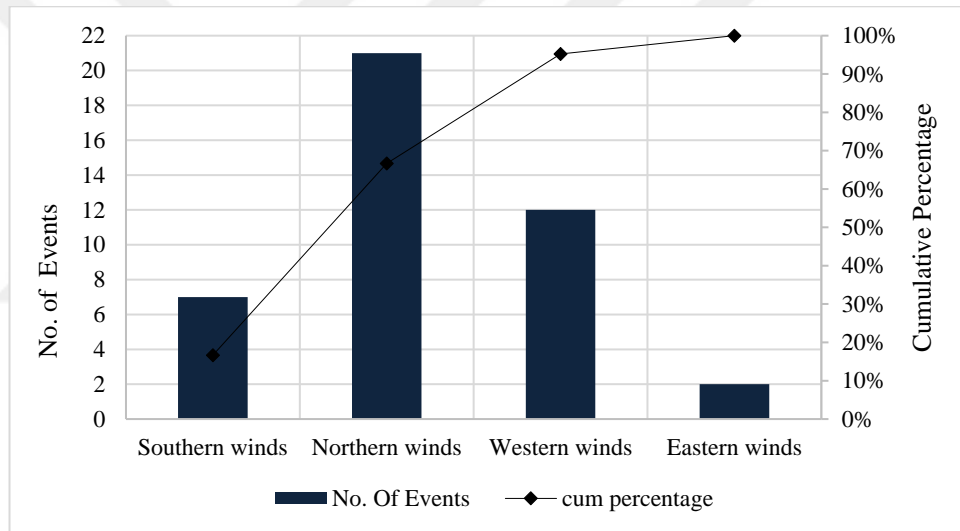
Figure 4.25 Frequency distribution of wind directions at the moment of blasting for Karapınar
