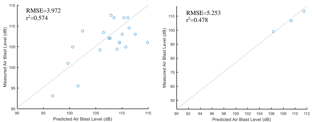
Figure 6.8 Predicted vs measured air blast levels for modeling set and testing set, respectively
