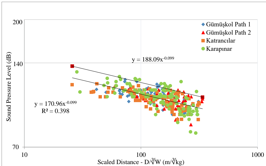
Figure 5.48 Air shock prediction from whole production blast data
