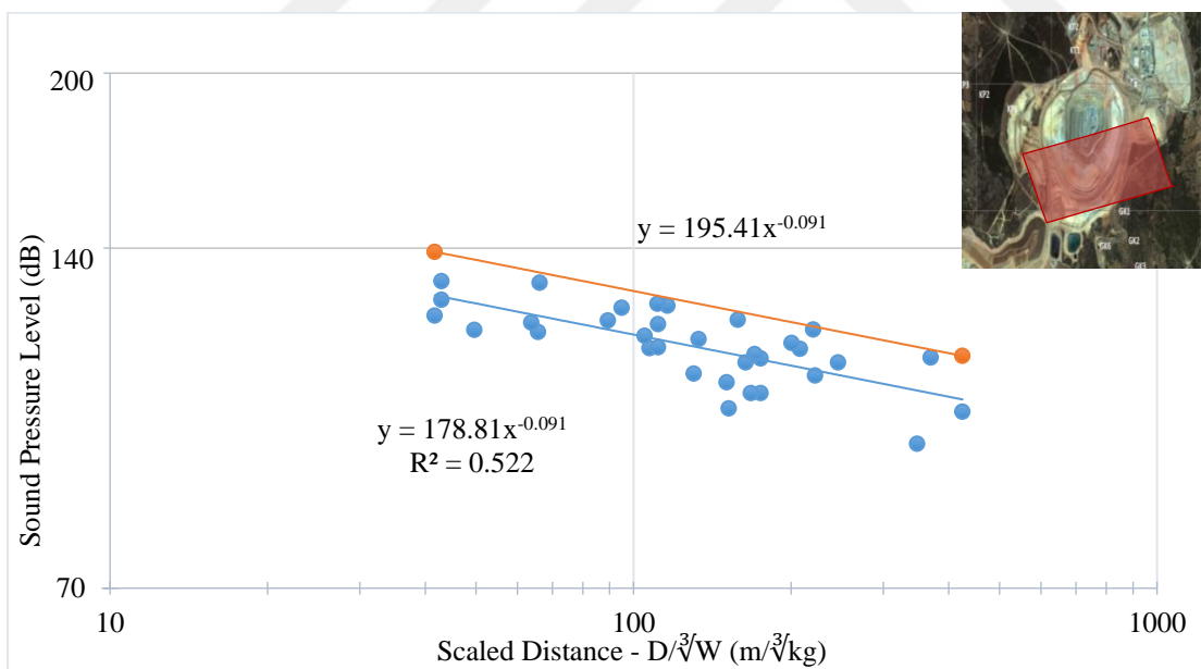
Figure 5.32 Katrancilar presplit blasting air blast overpressure levels in dB (Pit location- S, E, ENE, SSW - behind the pit)
