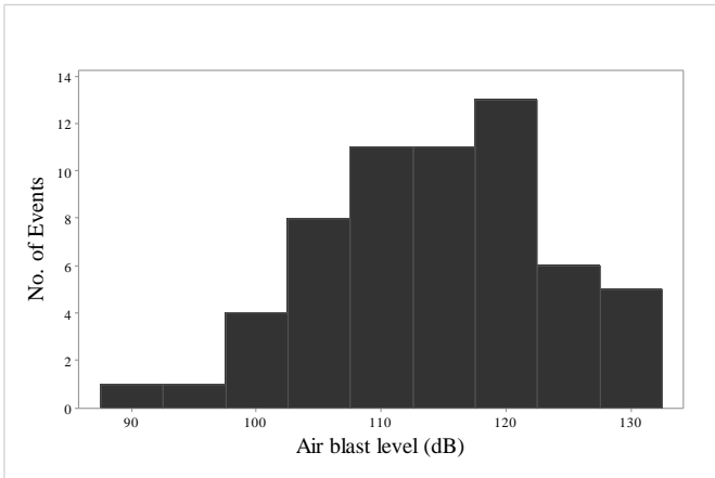
Figure 4.22 Katrancilar presplit blasting air blast histogram
