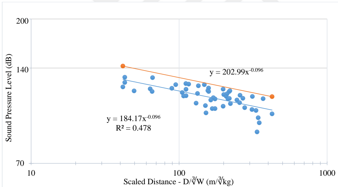
Figure 5.28 Katrancilar unclassified presplit blasting air blast overpressure levels in dB
