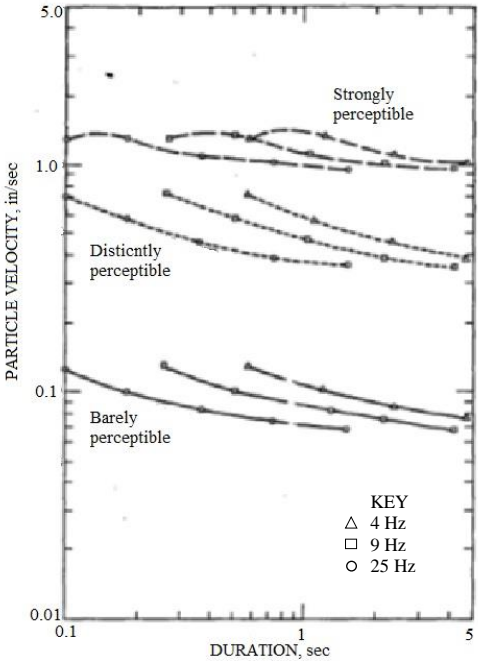
Figure 2.20 Human response to transient vibration velocities of various durations (Siskind et al., 1980b)
