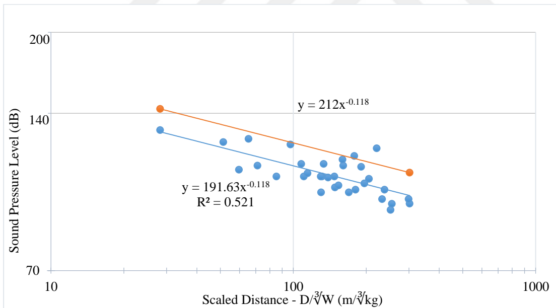
Figure 5.56 Karapınar production blasting air blast overpressure levels in dB (Eastern winds-SSE, SE, E, NE, NNE)
