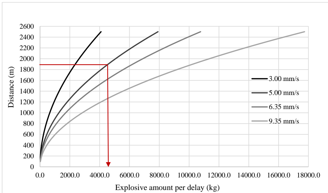
Figure 5.8 Safe explosive amounts for Katrancilar village for ‘behind the pit’ blasts
