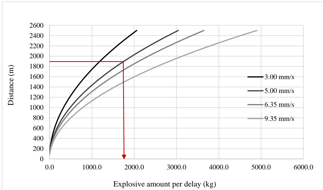
Figure 5.20 Safe explosive amounts for Gümüşkol village Path 1 for ‘behind the pit’ blasts
