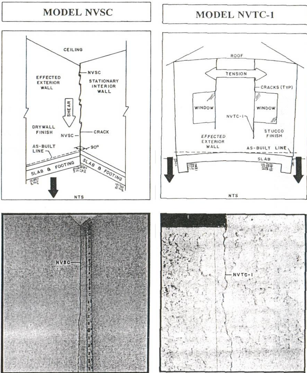
Figure 4.11 Crack forming mechanisms (normal vertical shear crack on the left and normal vertical tension crack on the right) (Audell, 1996)
