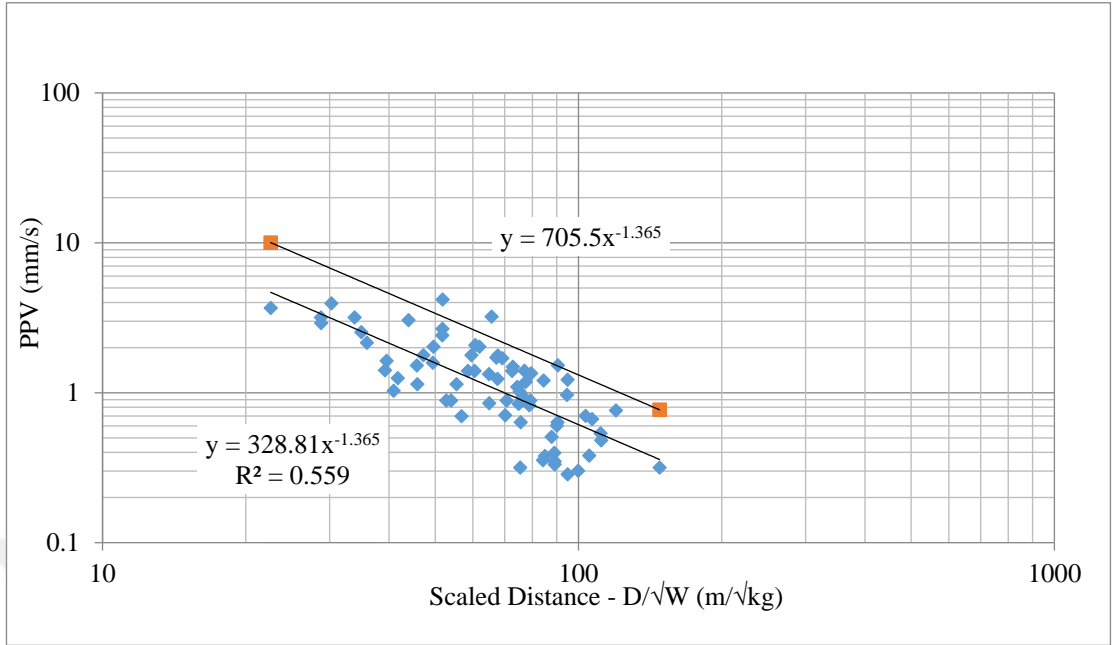
Figure 5.22 Gümüşkol Path 2 unclassified production blasting PPV values
