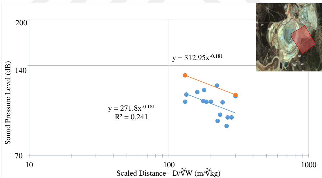
Figure 5.58 Karapınar production blasting air blast overpressure levels in dB (Pit location- ENE, E, SE - behind the pit)
