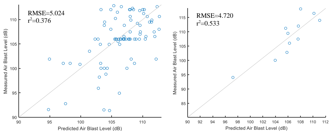
Figure 6.11 Predicted vs measured air blast levels for modeling set and testing set, respectively
