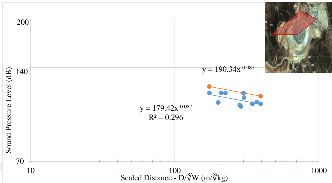
Figure 5.47 Gümüşkol Path 2 presplit blasting air blast overpressure levels in dB (Pit location- W, NW, N, NE- behind the pit)
