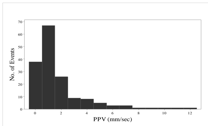
Figure 4.23 Katrancilar production blasting PPV histogram
