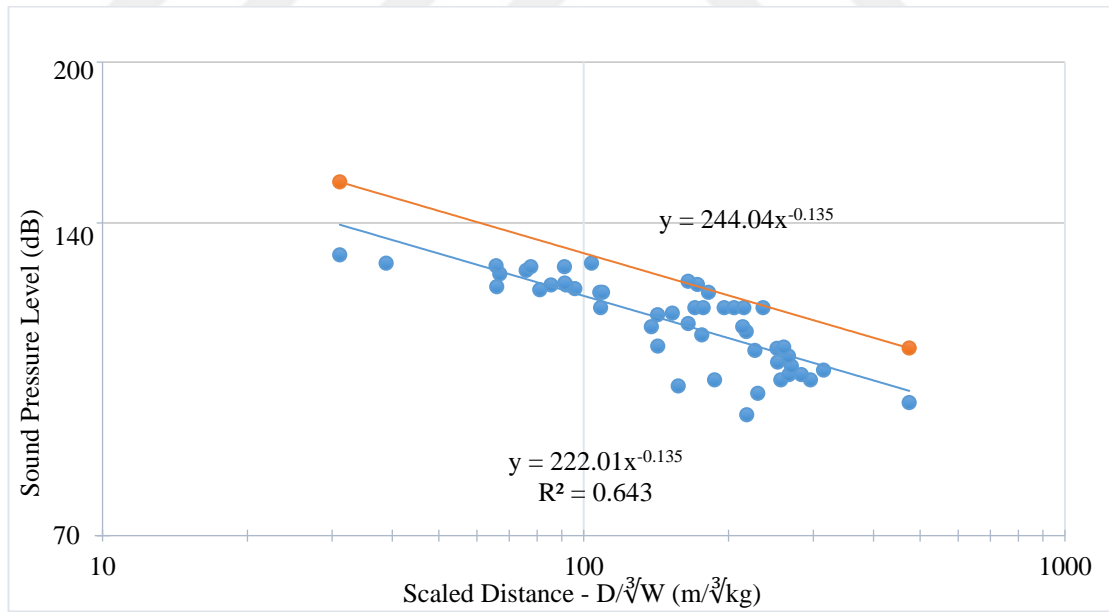
Figure 5.33 Karapınar unclassified presplit blasting air blast overpressure levels in dB
