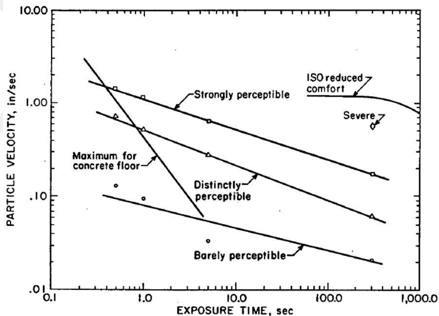
Figure 2.19 Human response to vibrations of various durations, summary. ISO values are from Standard 2631 (Siskind et al., 1980b)
