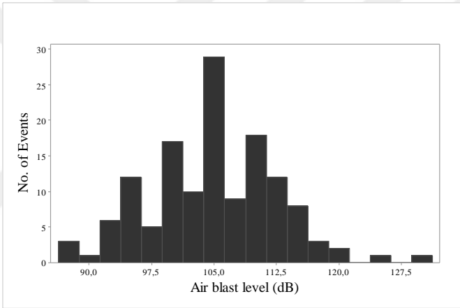
Figure 4.24 Katrancilar production blasting air blast histogram
