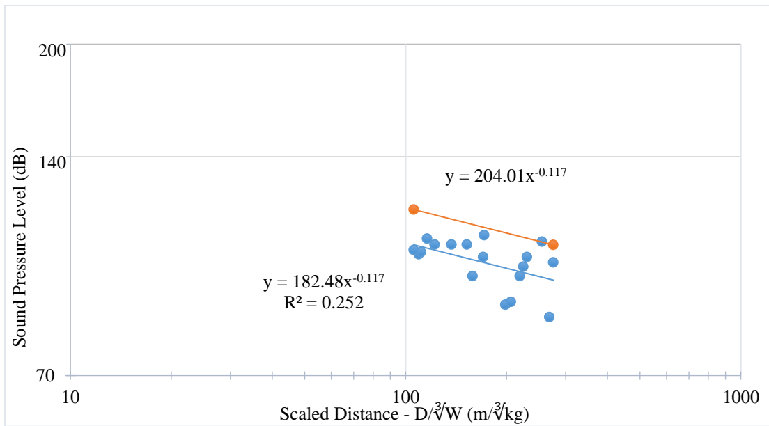
Figure 5.66 Gümüşkol Path 2 production blasting air blast overpressure levels in dB (Southern winds- SE, ESE)
