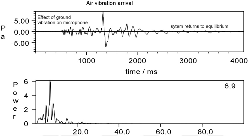
Figure 2.5 Air vibration (Pascal) wave trace for a single hole firing (Richards & Moore, 2009b)
