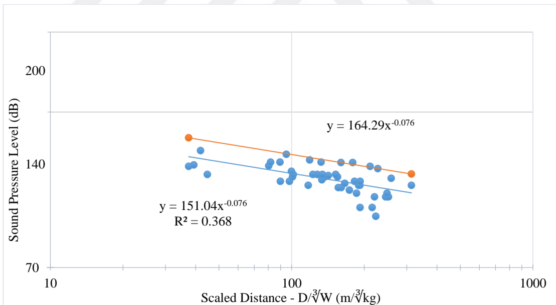
Figure 5.51 Katrancilar production blasting air blast overpressure levels in dB (Southern winds-S, SSE, SSW)
