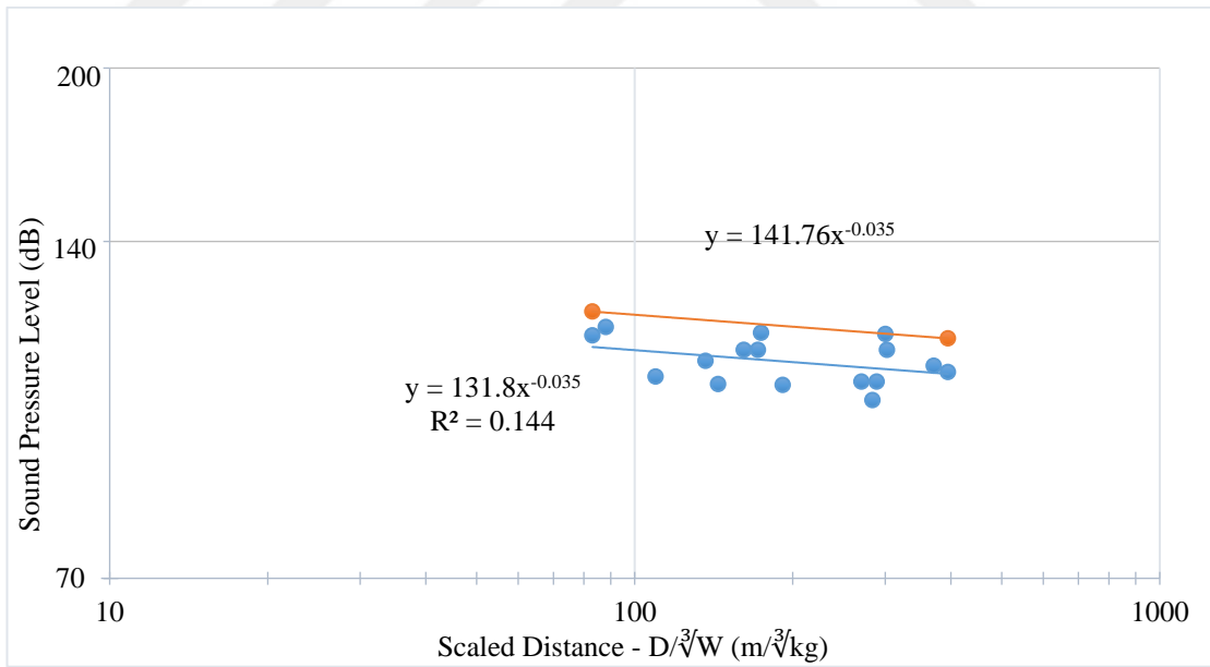
Figure 5.44 Gümüřkol Path 2 presplit blasting air blast overpressure levels in dB (Northern winds- NNE, NNW, WNW)
