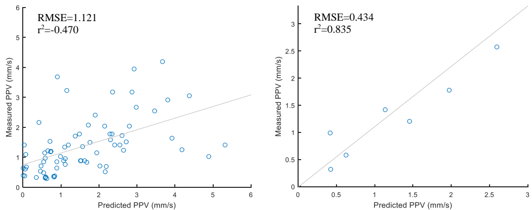
Figure 6.4 Predicted vs measured ground vibration levels for modeling set and testing set, respectively
