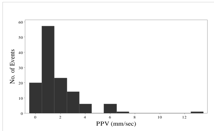
Figure 4.33 Gümüşkol Path 1 production blasting PPV histogram
