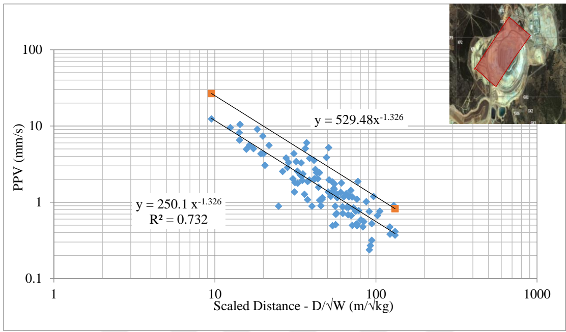
Figure 5.5 Katrancilar production blasting PPV values (Pit location- NE, N, W, SW- in front of the pit)
