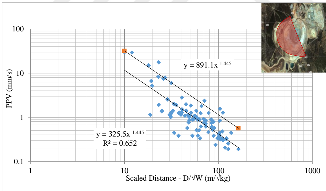
Figure 5.11 Karapınar production blasting PPV values (Pit location- NNW, W, S, SSE- in front of the pit)
