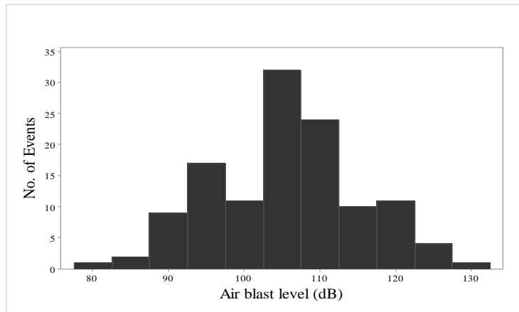
Figure 4.29 Karapınar production blasting air blast histogram
