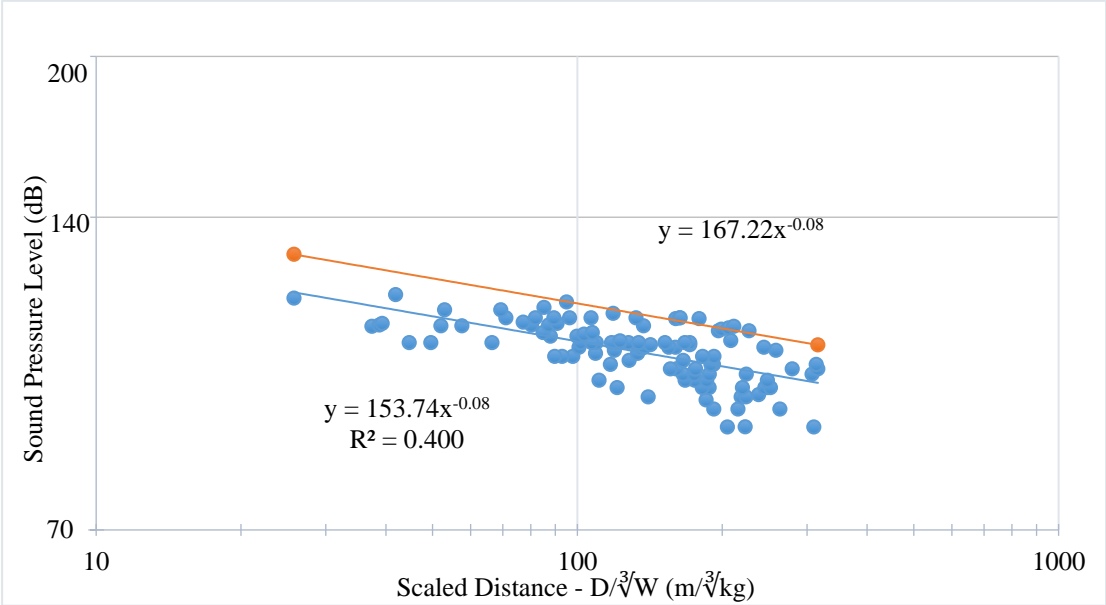
Figure 5.49 Katrancilar unclassified production blasting air blast overpressure levels in dB
