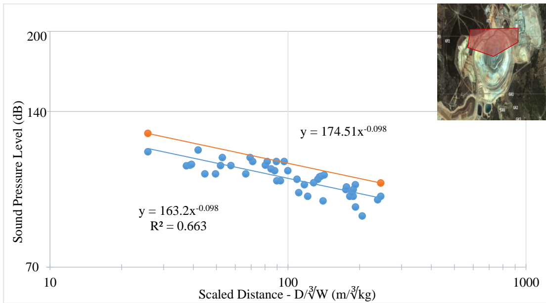
Figure 5.52 Katrancilar production blasting air blast overpressure levels in dB (Pit location- N, NE, WNW, NW, NNW - in front of the pit)
