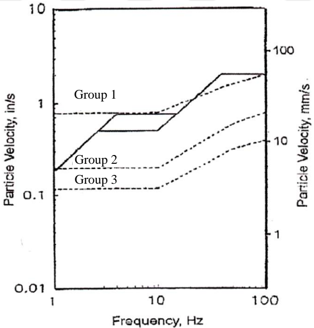
Figure 2.18 Vibration guidelines - USBM RI 8507 (solid line) compared to DIN 4150 (dashed line). Group 1, Group 2, Group 3. From AASHTO Designation: R 8-96 (Svinkin, 2008)
