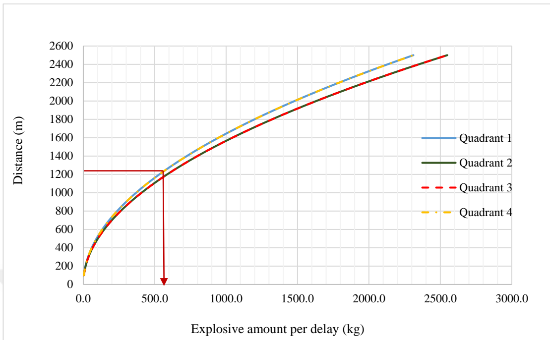
Figure 5.71 Safe explosive amounts for each quadrant not to exceed 3.00 mm/s in villages
