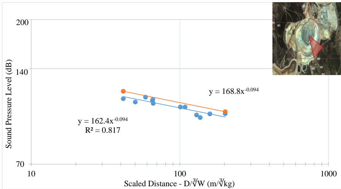
Figure 5.62 Gümüřkol Path 1 production blasting air blast overpressure levels in dB (Pit location- SE, SSE - in front of the pit)
