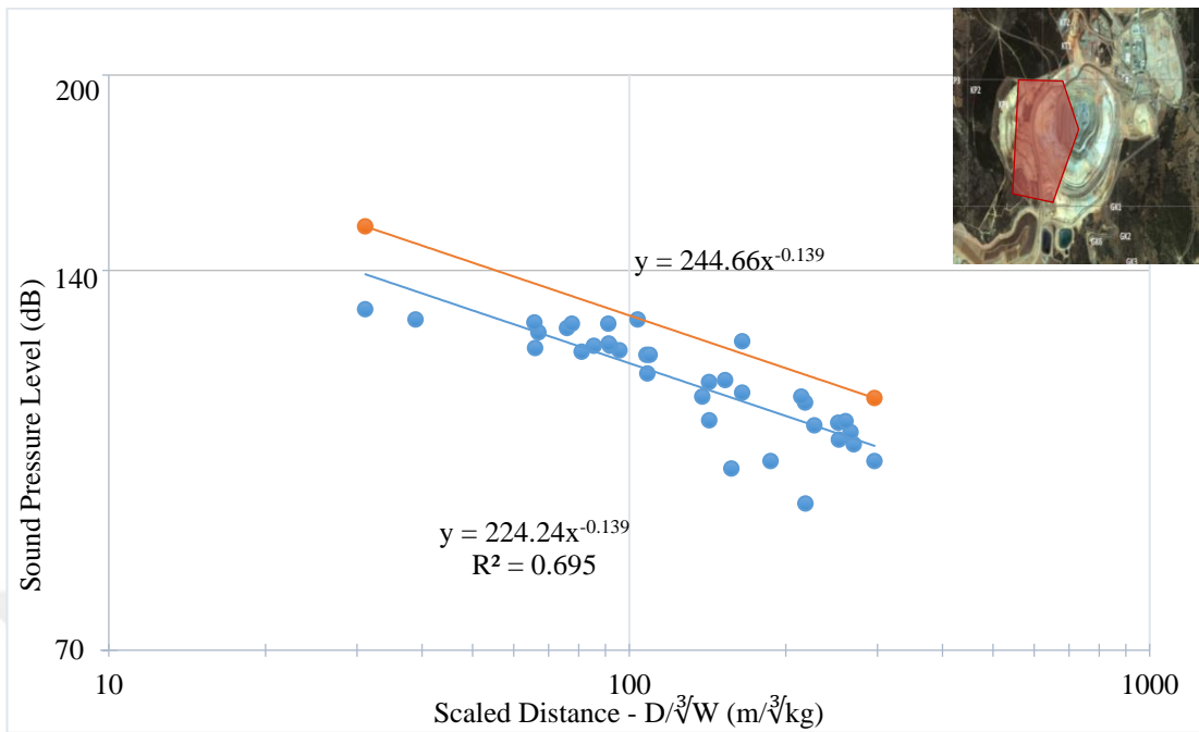
Figure 5.36 Karapinar presplit blasting air blast overpressure levels in dB (Pit location- SW, W, NNW - in front of the pit)
