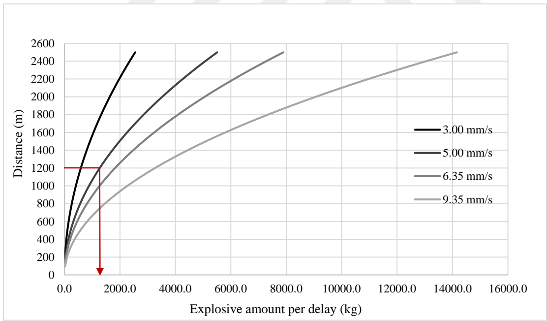
Figure 5.6 Safe explosive amounts for Katrancilar village for 'in front of the pit' blasts
