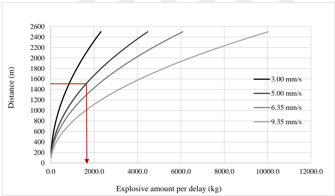
Figure 5.24 Safe explosive amounts for Gümüşkol village Path 2 for 'in front of the pit' blasts
