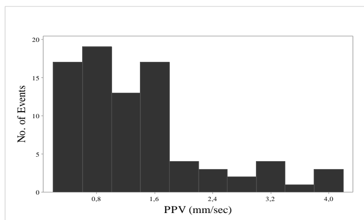
Figure 4.38 Gümüşkol Path 2 production blasting PPV histogram
