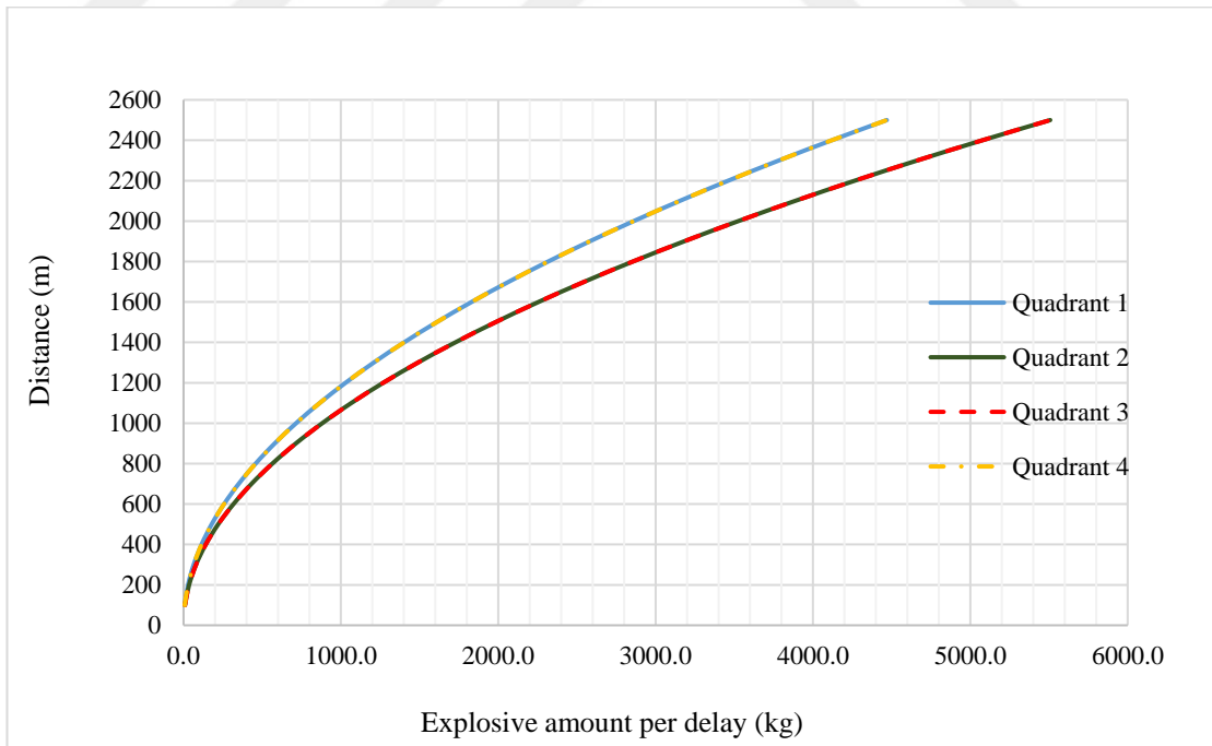
Figure 5.72 Safe explosive amounts for each quadrant not to exceed 5.00 mm/s in villages
