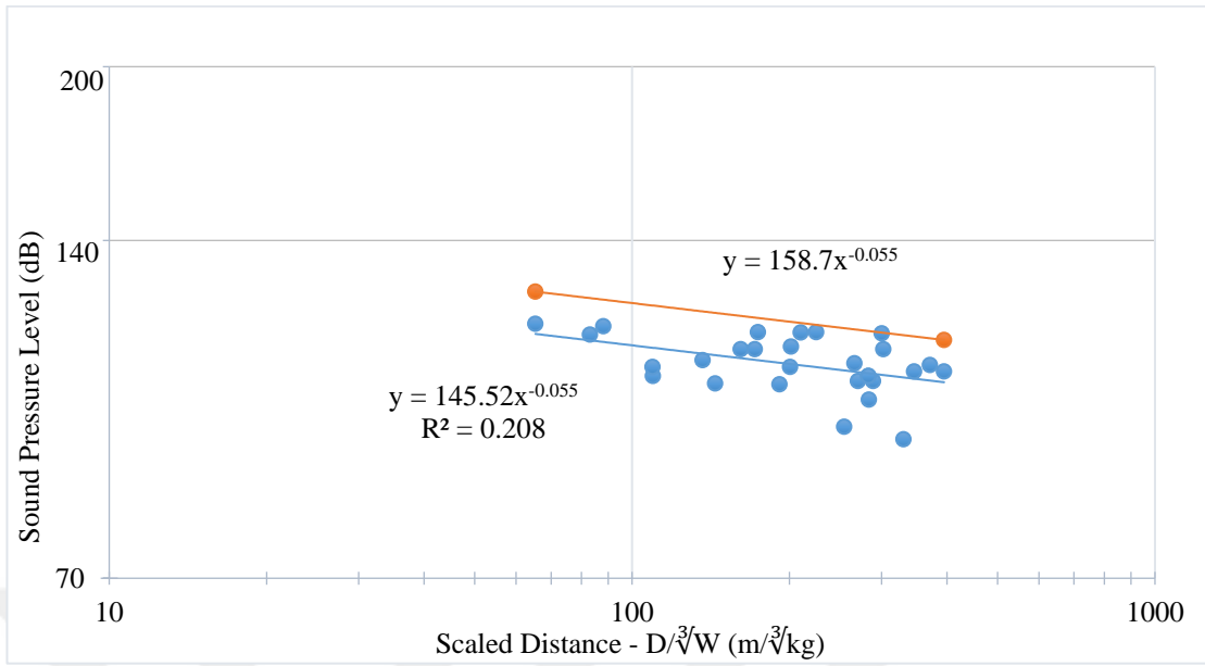
Figure 5.43 Gümüřkol Path 2 unclassified presplit blasting air blast overpressure levels in dB
