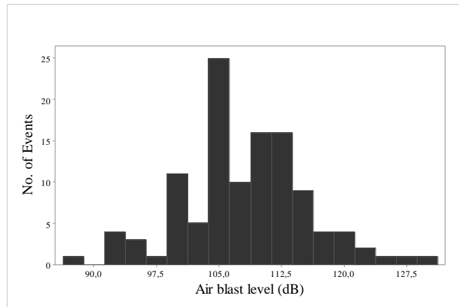
Figure 4.34 Gümüşkol Path 1 production blasting air blast histogram
