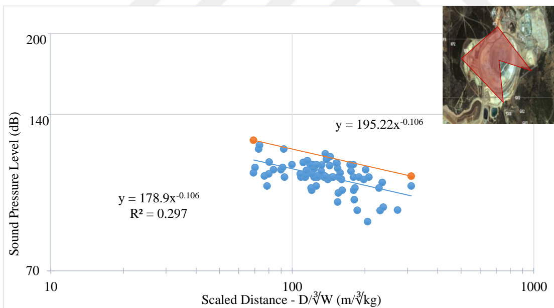
Figure 5.63 Gümüřkol Path 1 production blasting air blast overpressure levels in dB (Pit location- N, NE, E, ESE, S, SSW, W, NNW- behind the pit)
