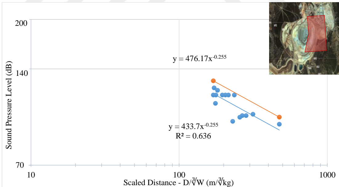
Figure 5.37 Karapinar presplit blasting air blast overpressure levels in dB (Pit location- N, E, SSW - behind the pit)
