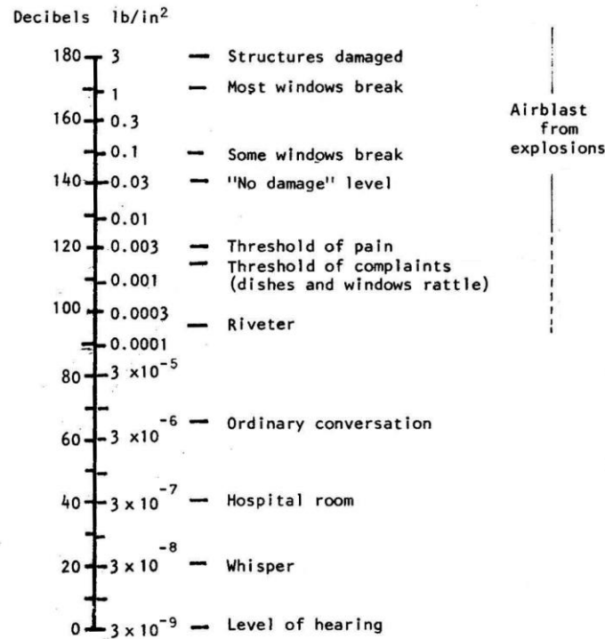
Figure 2.22 Human and structural response to sound pressure levels (Ladegaard-Pedersen & Dally, 1975)
