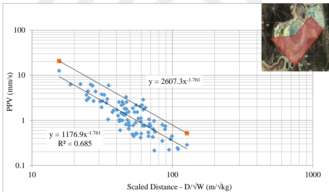
Figure 5.17 Gümüşkol Path 1 production blasting PPV values (Pit location-W, WSW, SW, S, E, NE- in front of the pit)
