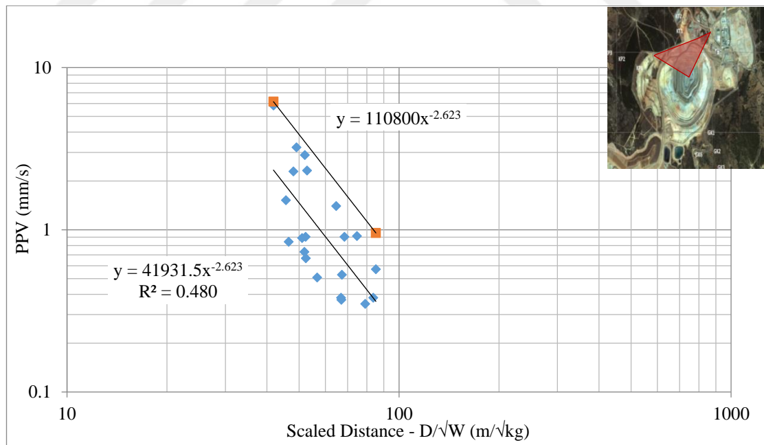
Figure 5.19 Gümüşkol Path 1 production blasting PPV values (Pit location- WNW, N, NNE- behind the pit)
