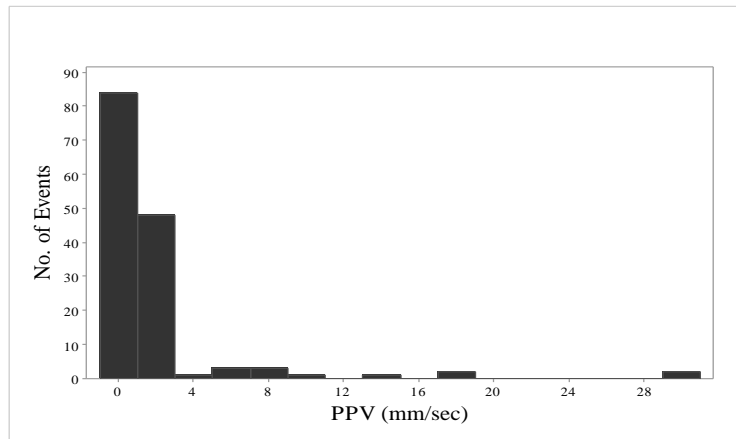
Figure 4.28 Karapınar production blasting PPV histogram
