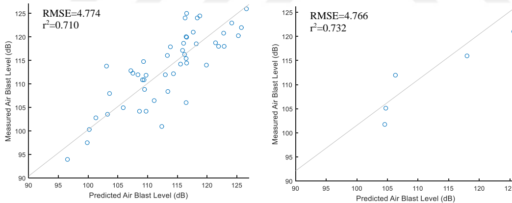
Figure 6.5 Predicted vs measured air blast levels for modeling set and testing set, respectively
