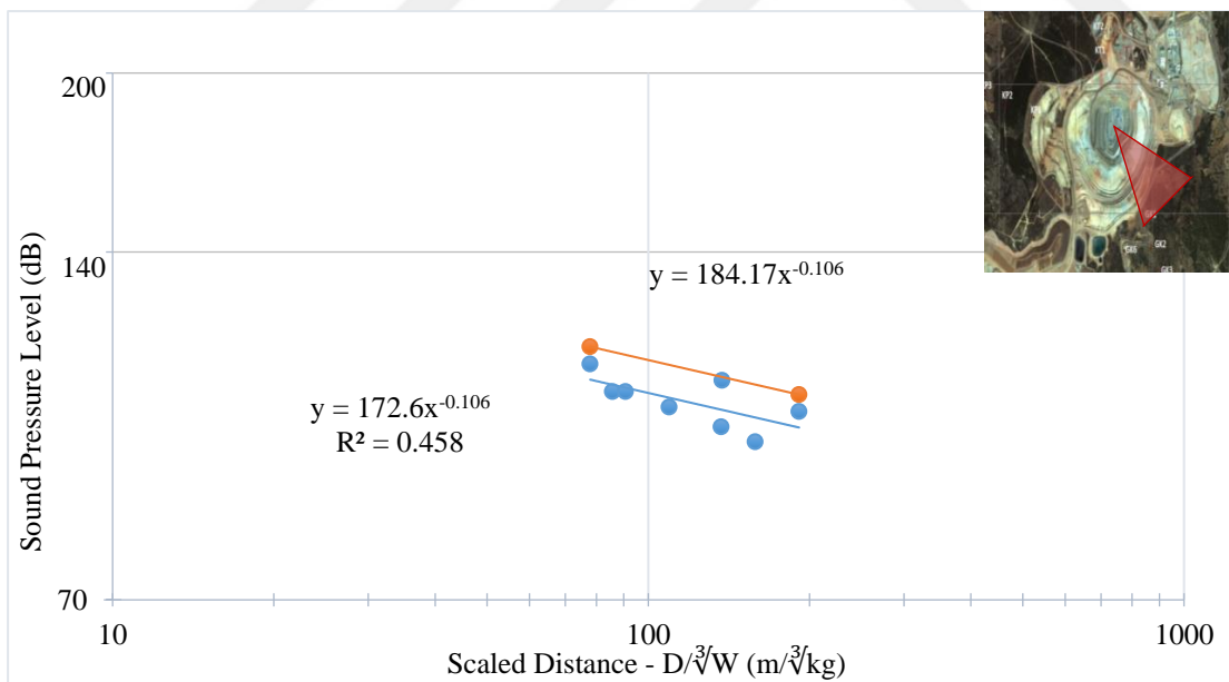
Figure 5.67 Gümüşkol Path 2 production blasting air blast overpressure levels in dB (Pit location- SE, SSE - in front of the pit)
