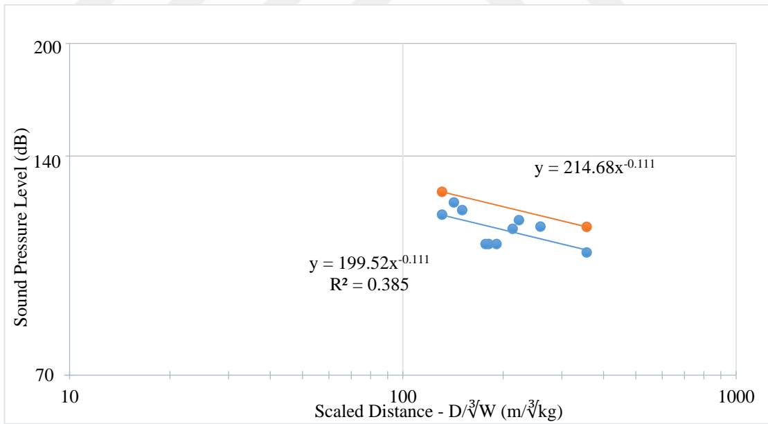
Figure 5.40 Gümüşkol Path 1 presplit blasting air blast overpressure levels (Southern winds-SE, S)
