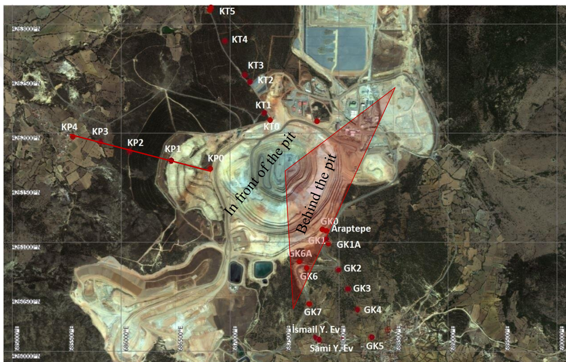
Figure 5.9 ‘behind the pit’ and ‘in front of the pit’ concepts for Karapınar
