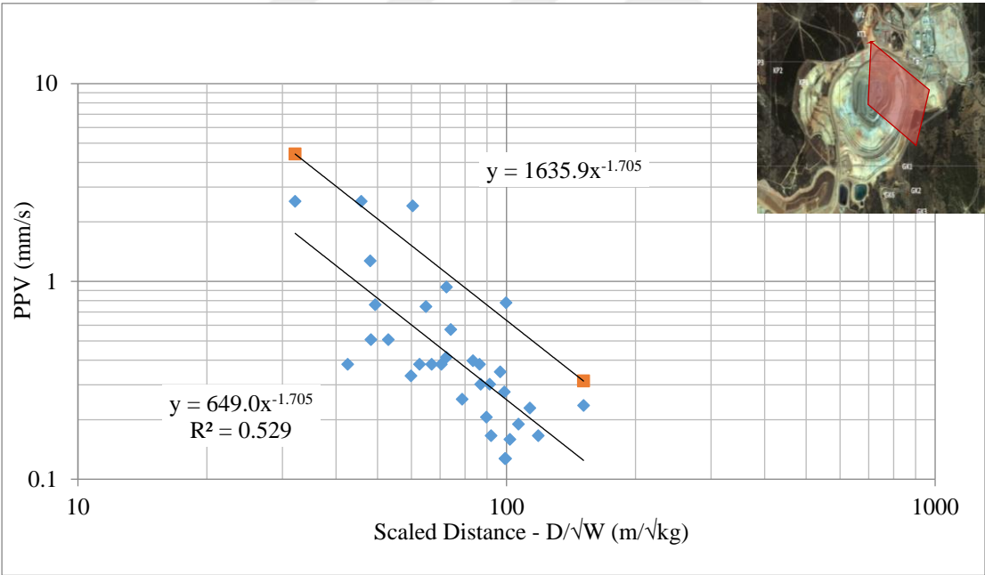
Figure 5.13 Karapınar production blasting PPV values (Pit location- N, NE, E, SE - behind the pit)
