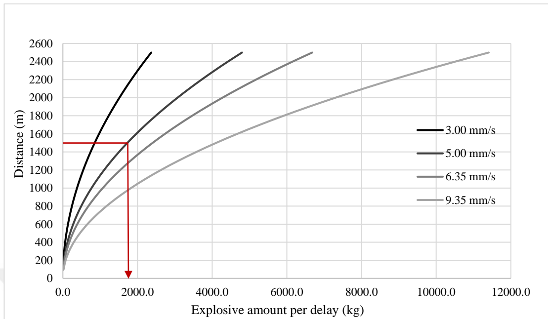
Figure 5.12 Safe explosive amounts for Karapınar village for ‘in front of the pit’ blasts
