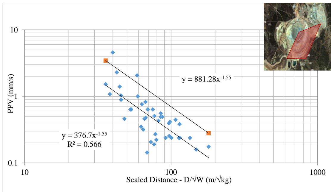
Figure 5.7 Katrancilar production blasting PPV values (Pit location- SSW, S, E, ENE- behind the pit)
