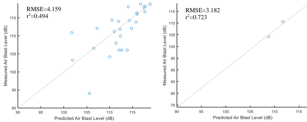
Figure 6.7 Predicted vs measured air blast levels for modeling set and testing set, respectively
