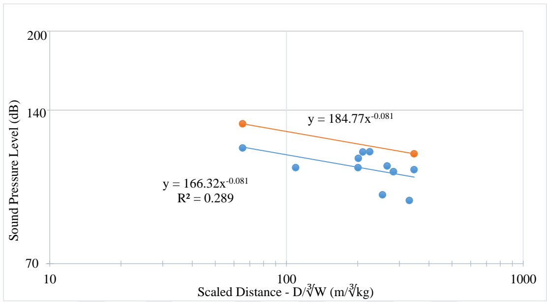
Figure 5.45 Gümüşkol Path 2 presplit blasting air blast overpressure levels in dB (Southern winds- WSW, S, ESE)
