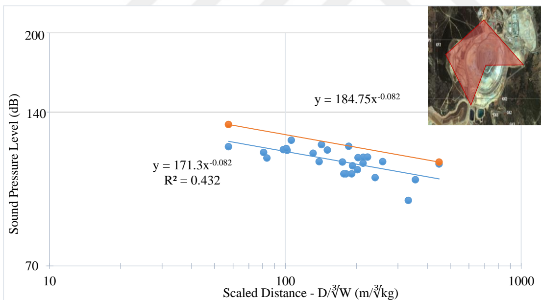
Figure 5.42 Gümüşkol Path 1 presplit blasting air blast overpressure levels (Pit location- N, NE, E, SSW, W - behind the pit)
