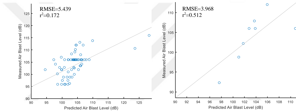
Figure 6.12 Predicted vs measured air blast levels for modeling set and testing set, respectively
