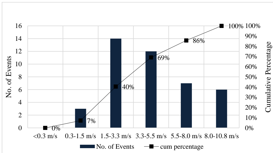
Figure 4.26 Frequency distribution of wind speeds at the moment of monitoring for Karapınar
