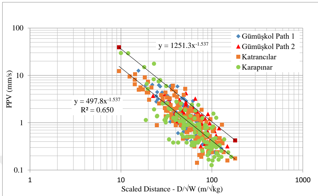
Figure 5.1 PPV prediction from whole production blast data
