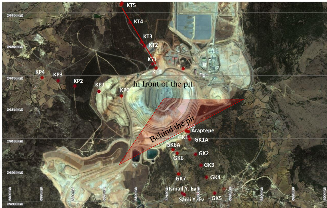
Figure 5.3 'behind the pit' and 'in front of the pit' concepts for Katrancilar
