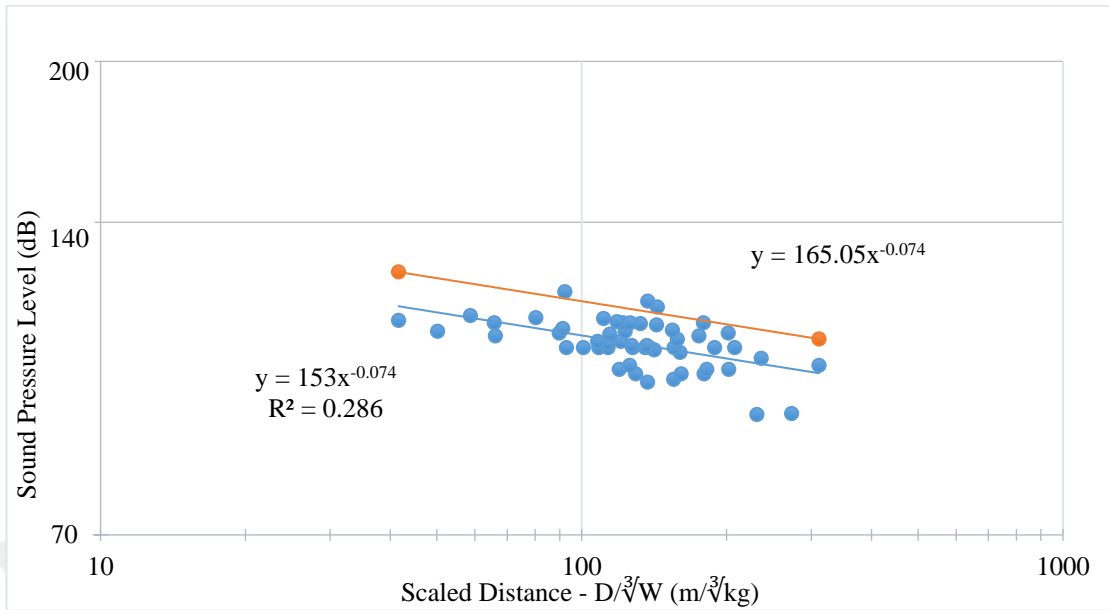
Figure 5.60 GümüŖkol Path 1 production blasting air blast overpressure levels in dB (Northern winds- N, NW, NE, NNE, ENE)
