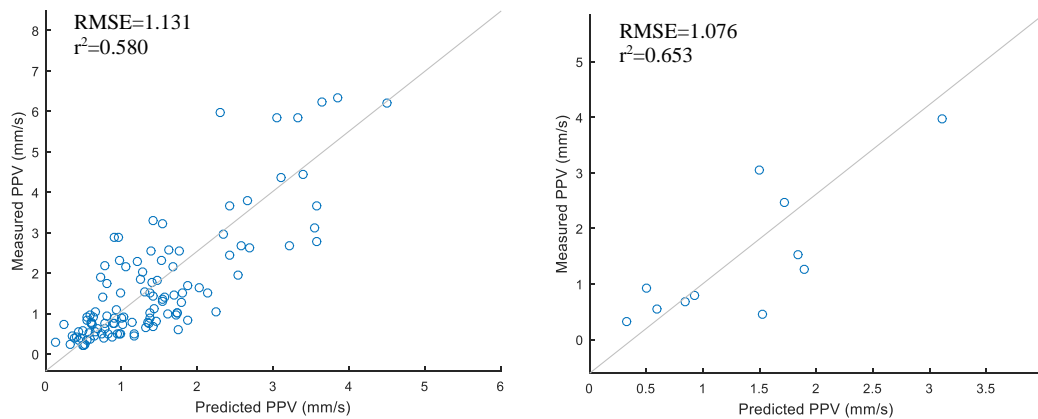
Figure 6.3 Predicted vs measured ground vibration levels for modeling set and testing set, respectively
