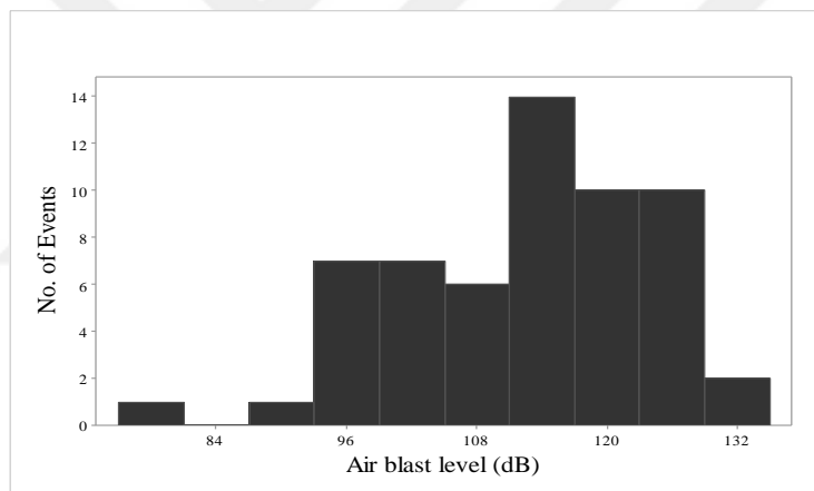
Figure 4.27 Karapınar presplit blasting air blast histogram
