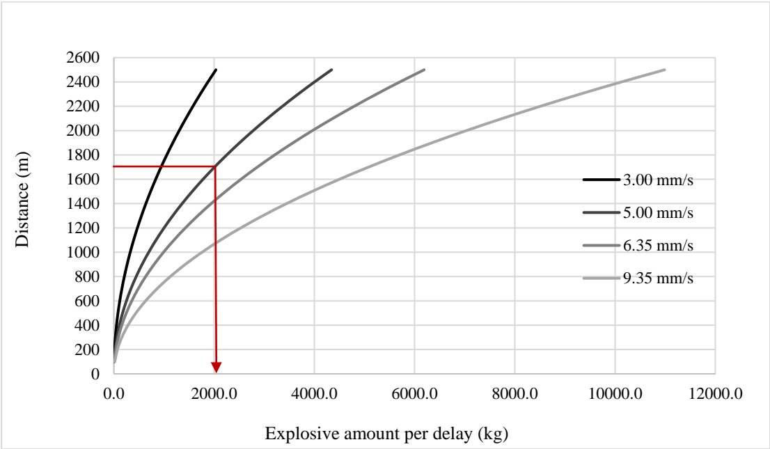
Figure 5.26 Safe explosive amounts for Gümüüşkol village Path 2 for ‘behind the pit’ blasts
