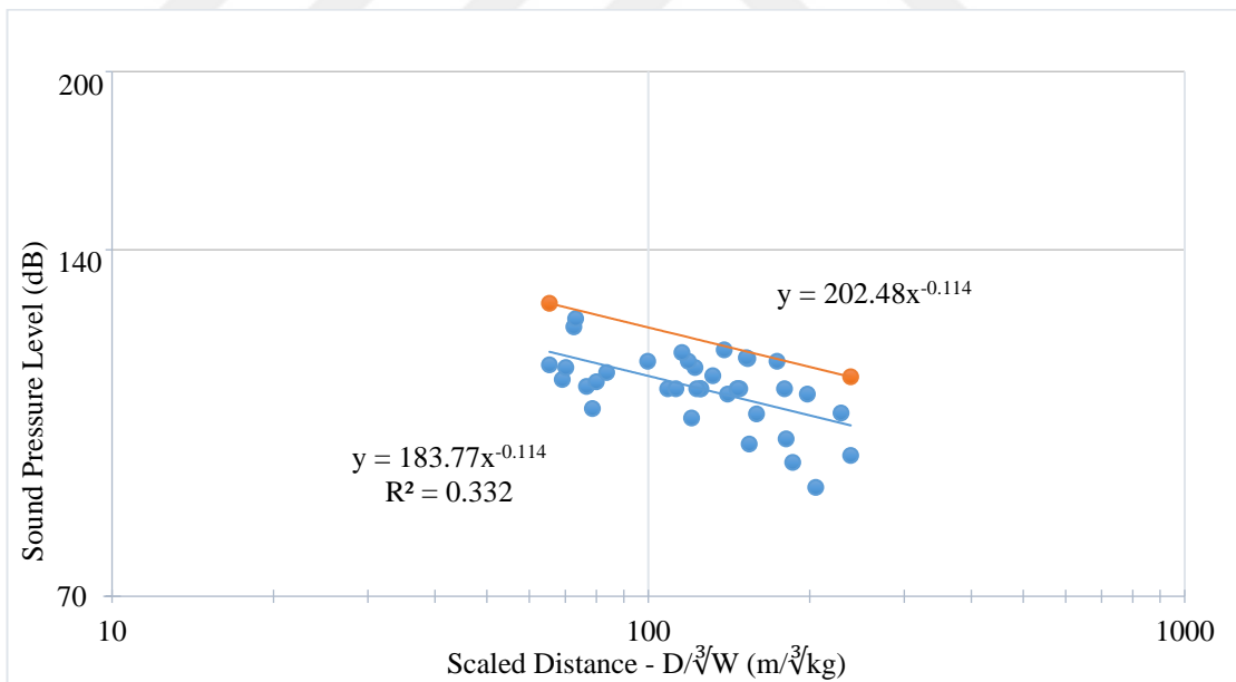
Figure 5.61 GümüŖkol Path 1 production blasting air blast overpressure levels in dB (Southern winds- SE, SSW, S)
