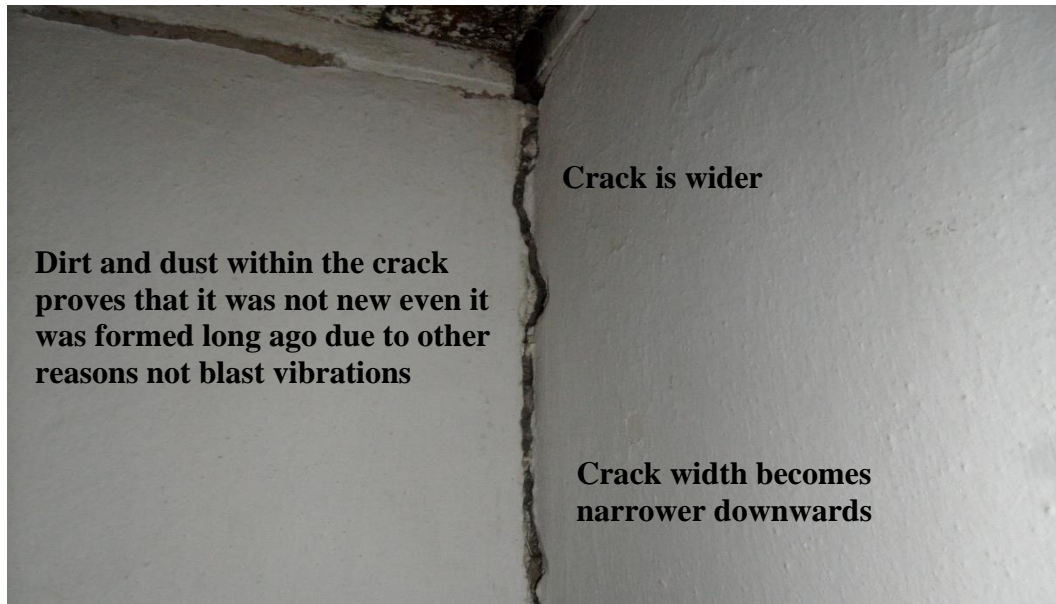
Figure 4.13 Normal vertical shear crack at the joint of inner and outer walls at the first floor of Sami Yildirim's house (Bilgin et al., 2015)
