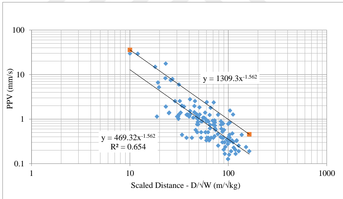
Figure 5.10 Karapınar unclassified production blasting PPV
