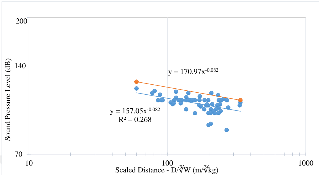
Figure 5.64 Gümüřkol Path 2 unclassified production blasting air blast overpressure levels in dB
