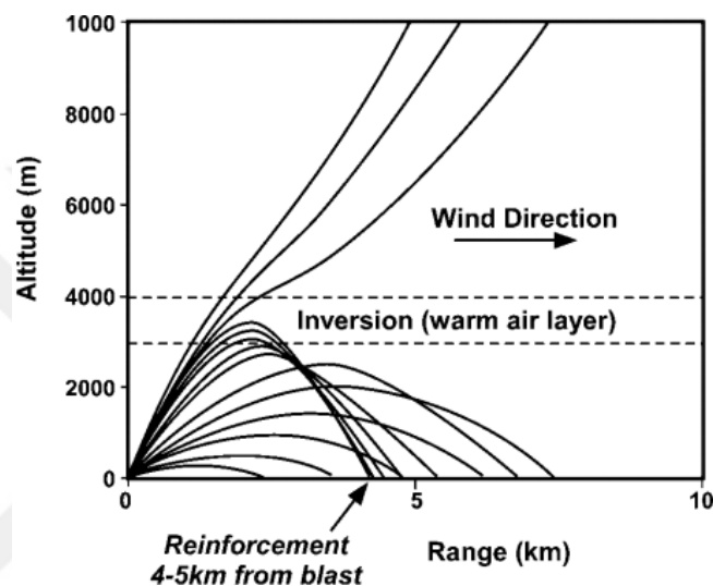
Figure 2.13 Meteorological reinforcement caused by warm air inversion layer (Richards, 2013)
