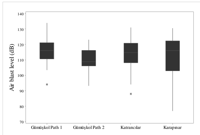
Figure 4.16 Boxplots of air blast levels from presplit blasts with respect to villages
