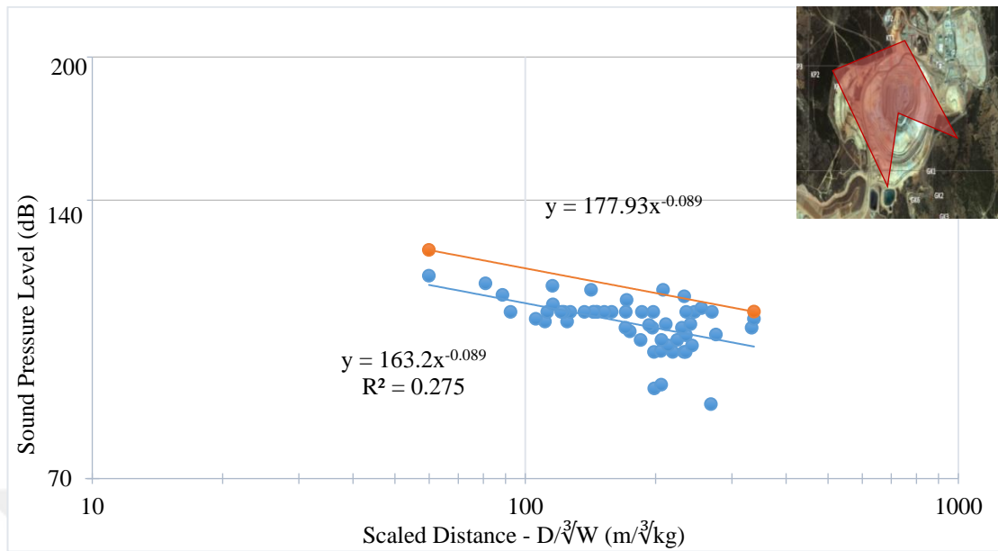
Figure 5.68 Gümüşkol Path 2 production blasting air blast overpressure levels in dB (Pit location- N, NE, E, S, SW, W, NNW - behind the pit)
