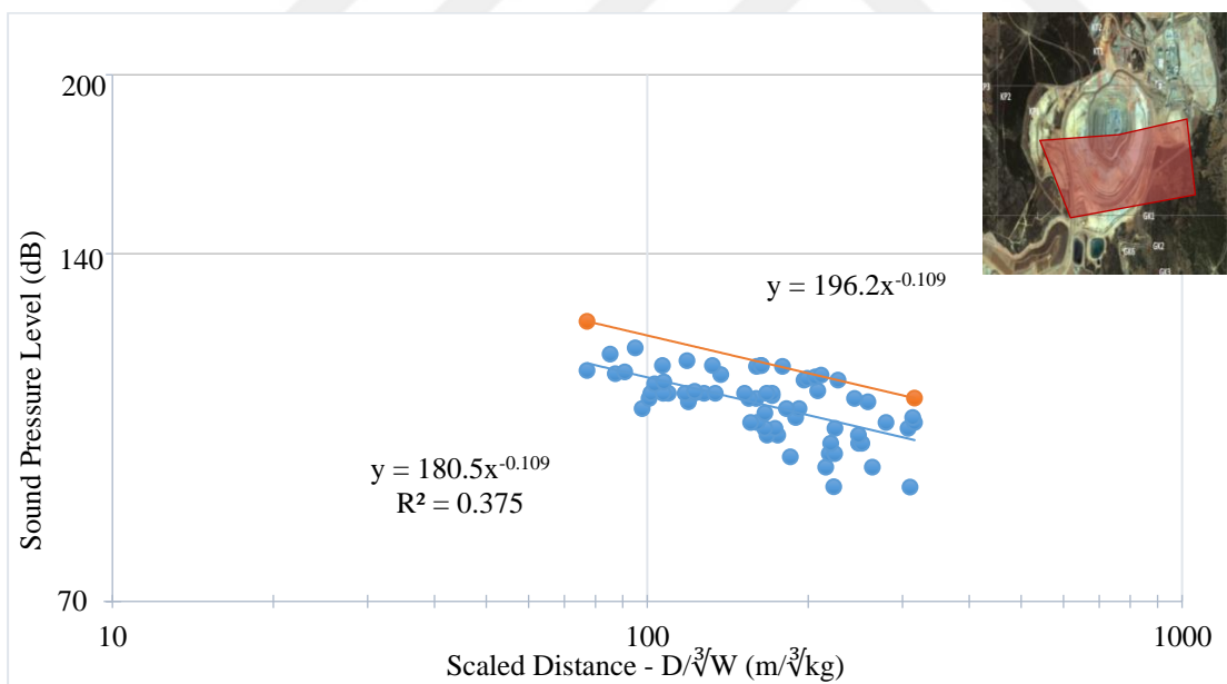
Figure 5.53 Katrancilar production blasting air blast overpressure levels in dB (Pit location- ENE, E, SE, S, SW, W- behind the pit)
