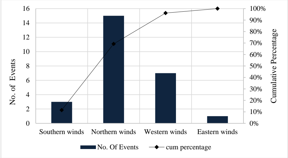
Figure 4.35 Frequency distribution of wind directions at the moment of blasting for Gümüşkol path 2
