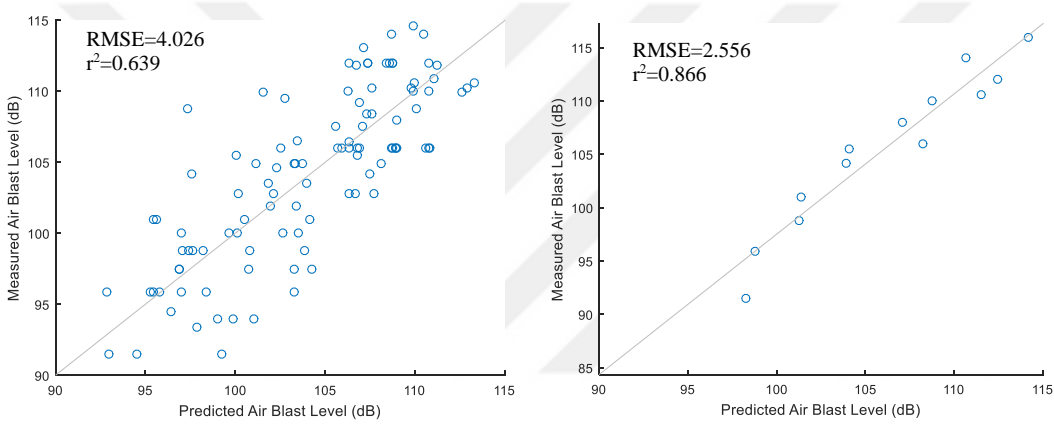
Figure 6.9 Predicted vs measured air blast levels for modeling set and testing set, respectively
