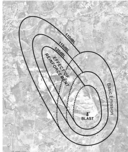
Figure 2.15 Basic air blast emission with wavefront reinforcement (Richards, 2013)
