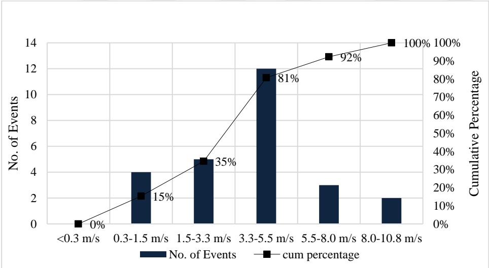
Figure 4.36 Frequency distribution of wind directions at the moment of blasting for Gümüşkol path 2
