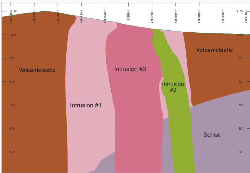
Figure 3.4 A-A' Cross-Section at 687300E, Looking West (Juras et al., 2010)
