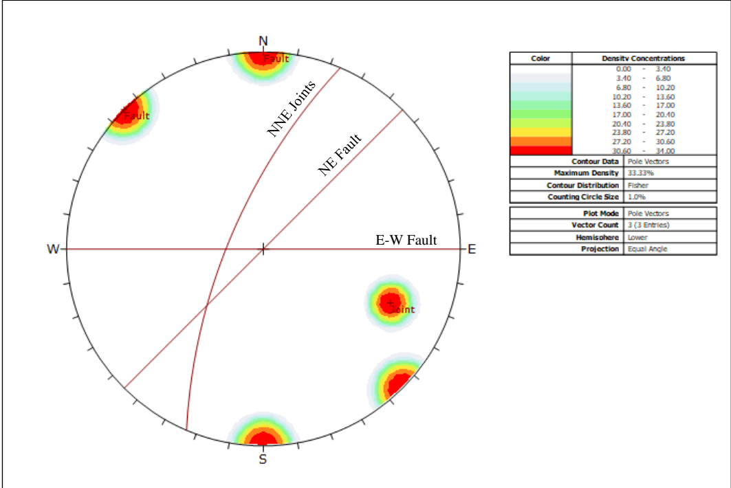
Figure 3.5 Discontinuity mapping of the pit cone (Rocscience Dips version 7)
