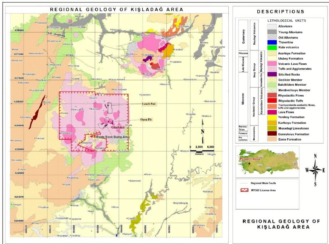
Figure 3.1 Kışladağ regional geology (Yazıcıgil et al., 2000)
