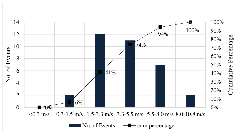
Figure 4.31 Frequency distribution of wind speeds at the moment of monitoring for Gümüşkol path 1
