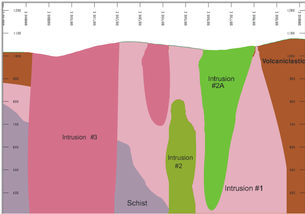
Figure 3.3 B-B' Cross-Section at 4261500N with Lithologies (looking north) (Juras et al., 2010)
