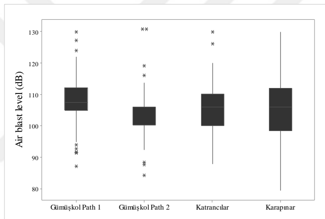
Figure 4.17 Boxplots of air blast levels from production blasts with respect to villages
