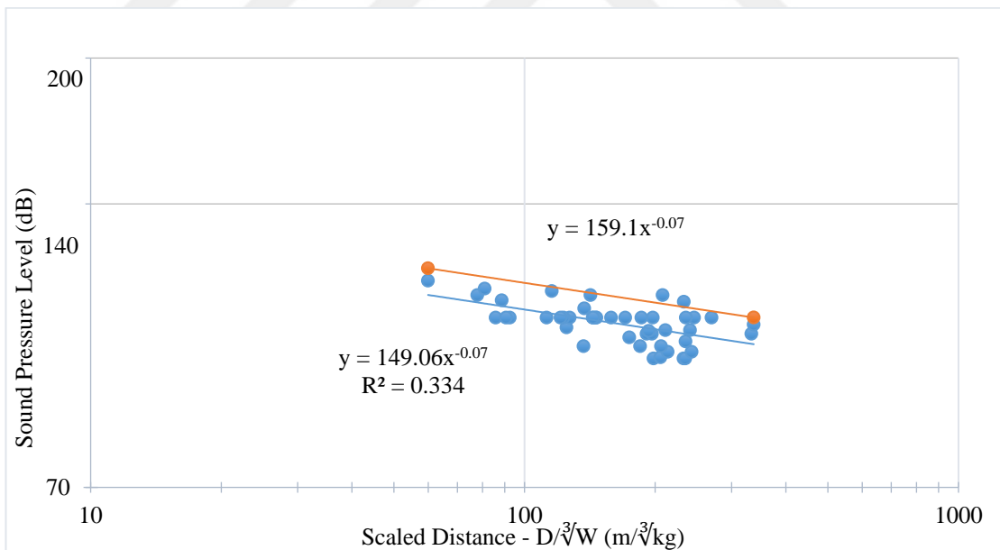
Figure 5.65 Gümüřkol Path 2 production blasting air blast overpressure levels in dB (Northern winds - N, NE, NW)
