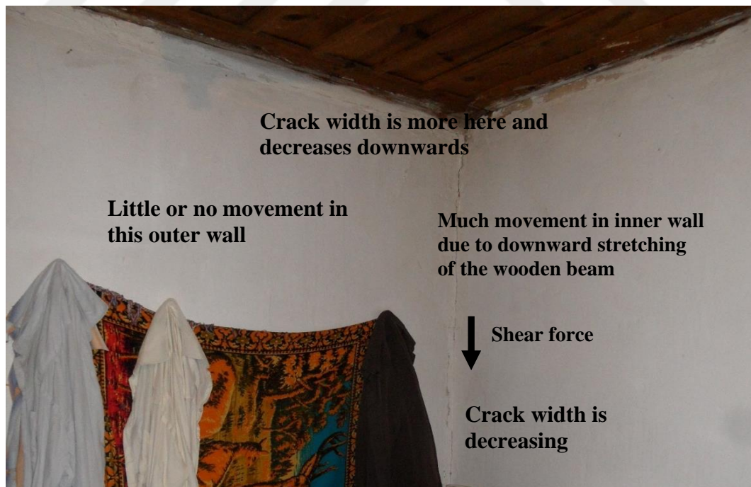
Figure 4.12 Normal vertical shear crack at the joint of inner wall and outer wall of first floor of Sami Yıldırım's house (Bilgin et al., 2015)
