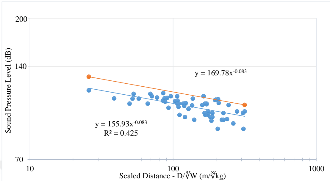
Figure 5.50 Katrancilar production blasting air blast overpressure levels in dB (Northern winds-N, NE, NW)
