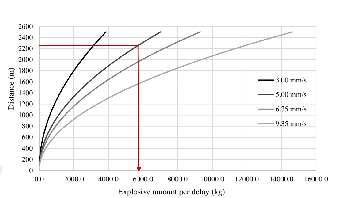
Figure 5.14 Safe explosive amounts for Karapınar village for ‘behind the pit’ blasts
