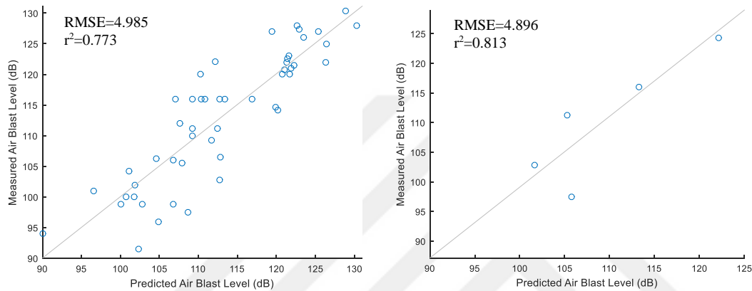
Figure 6.6 Predicted vs measured air blast levels for modeling set and testing set from, respectively
