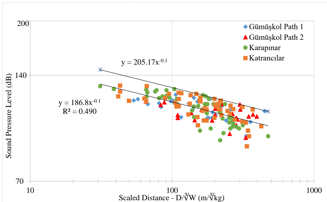
Figure 5.27 Air shock prediction from whole presplit blast data
