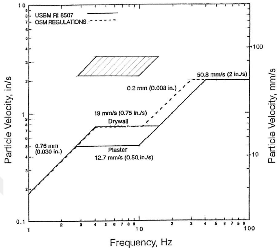
Figure 2.17 Safe ground vibration level criteria from USBM RI 8507 and OSM surface coal mine regulations; shaded area shows structural vibration velocity with amplification of 4.5 at resonance (Siskind, 2000 and Svinkin, 2008)
