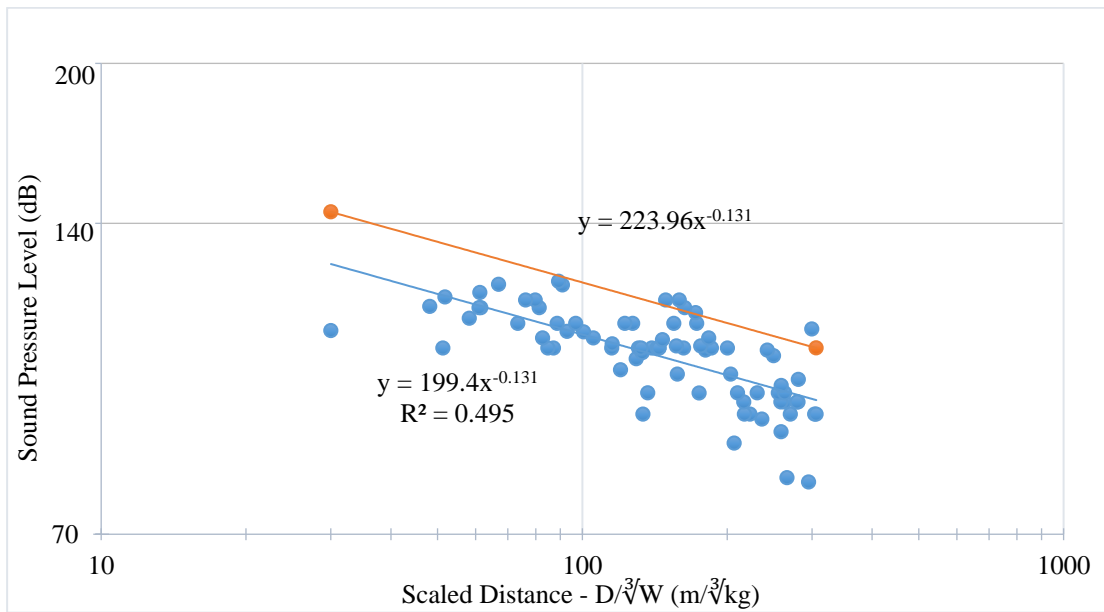
Figure 5.55 Karapınar production blasting air blast overpressure levels in dB (Western winds- SSW, SW, W, NW, NNW)
