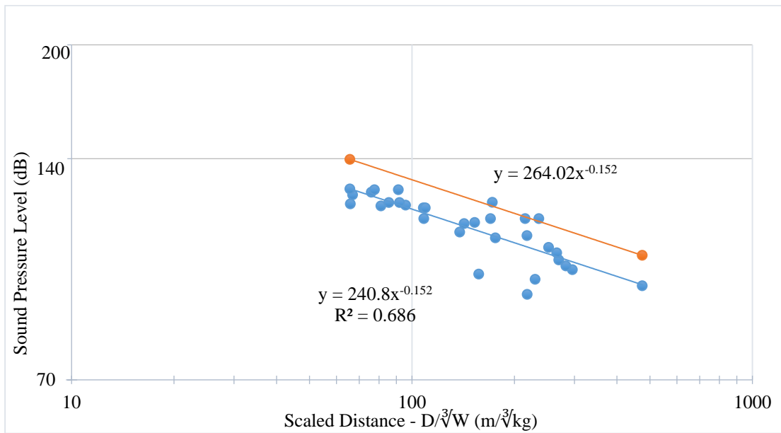
Figure 5.34 Karapınar presplit blasting air blast overpressure levels in dB (Western winds-W, SSW, NW, SW, NNW)
