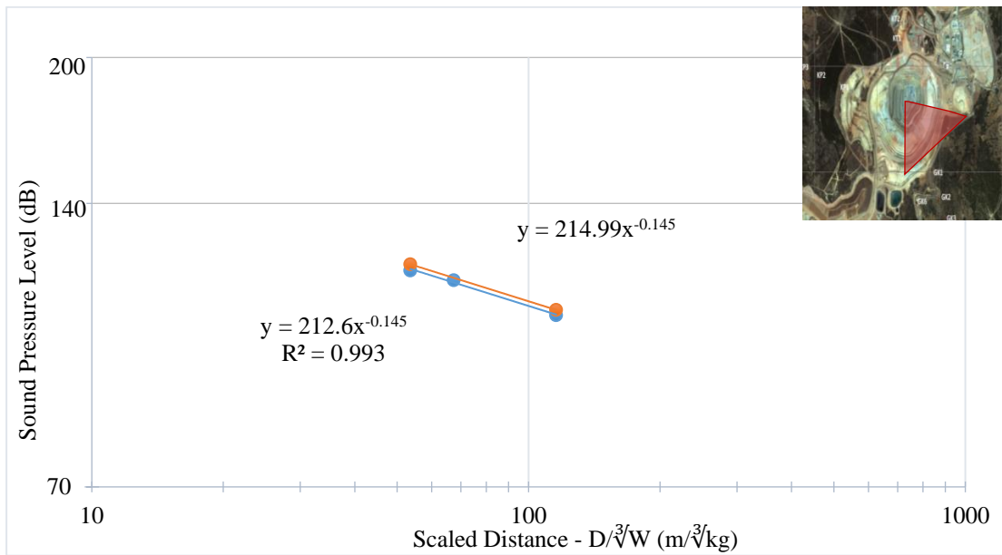
Figure 5.41 Gümüşkol Path 1 presplit blasting air blast overpressure levels (Pit location- ESE, SE, SSE, S - in front of the pit)
