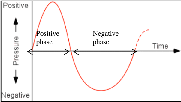
Figure 2.6 Synthesized air blast 'N' wave from single hole blasting (Richards & Moore, 2006)
