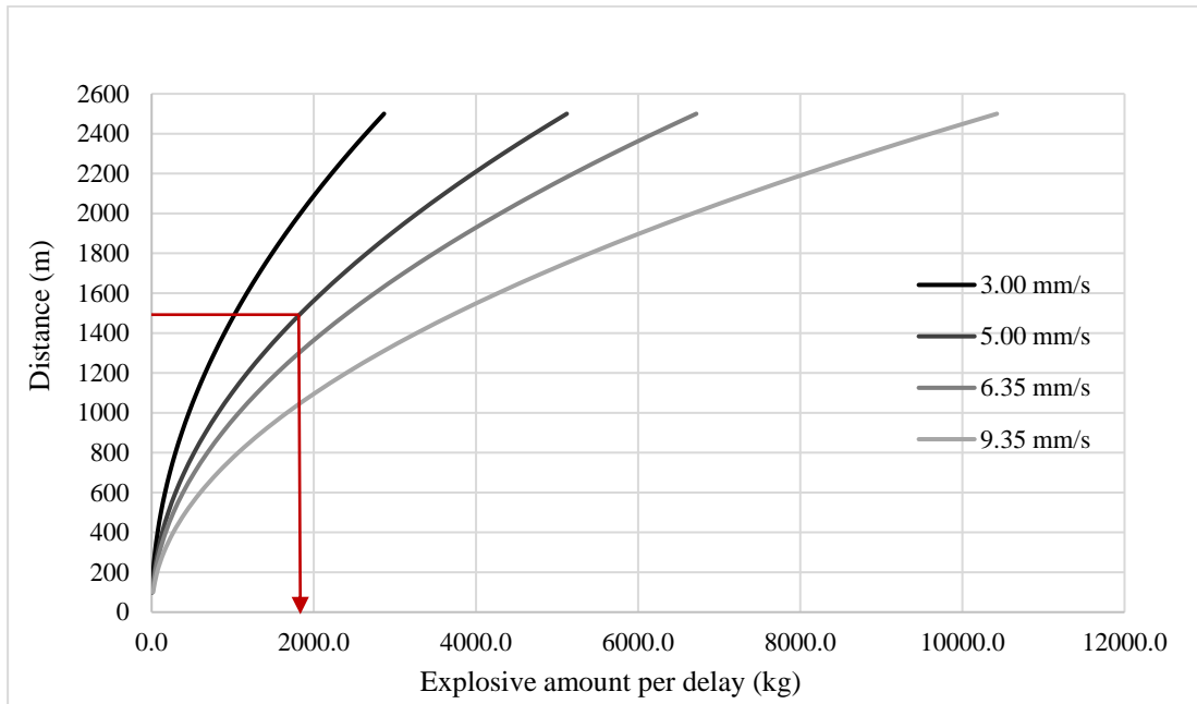
Figure 5.18 Safe explosive amounts for Gümüřkol village Path 1 for ‘in front of the pit’ blasts
