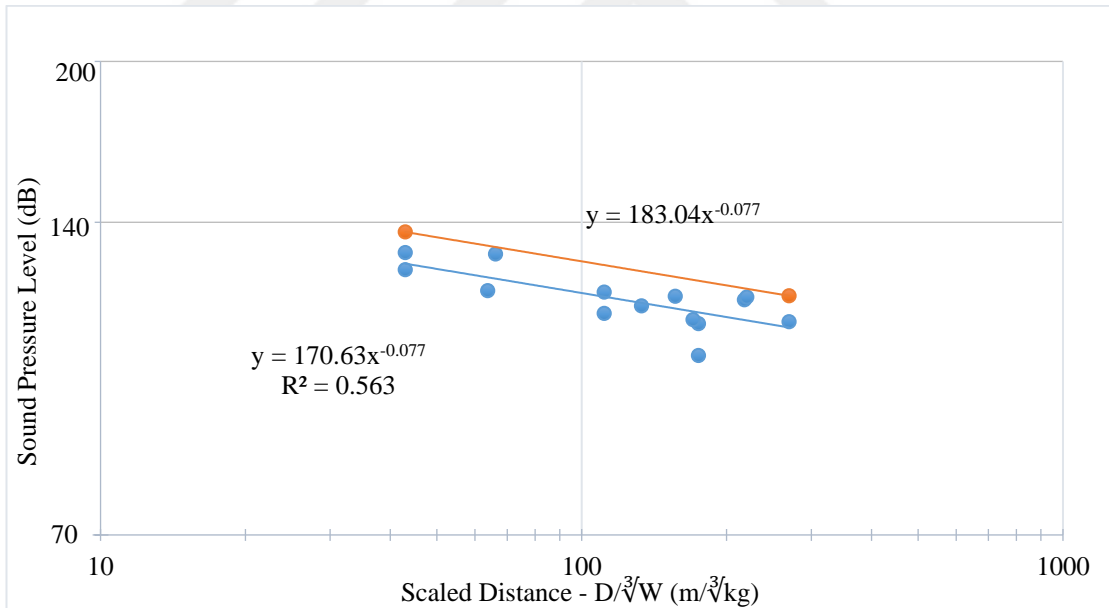
Figure 5.30 Katrancilar presplit blasting air blast overpressure levels in dB (Southern winds-WSW, W, SSE, S)
