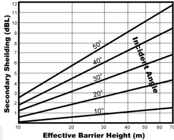
Figure 2.11 Estimation graph for secondary shielding (Richards & Moore, 2009b)
