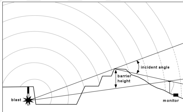
Figure 2.10 Shielding terminology (Richards & Moore, 2009b)
