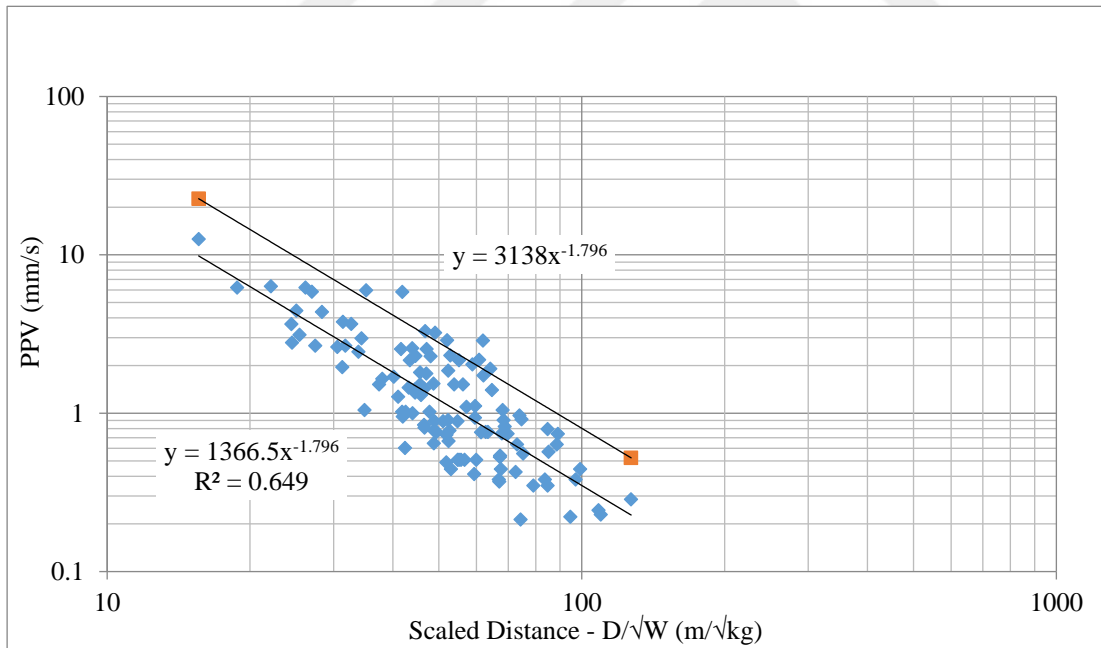
Figure 5.16 Gümüşkol Path 1 unclassified production blasting PPV values
