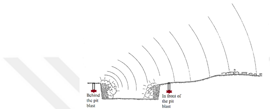
Figure 2.8 Effect of face orientation (Jimeno et al., 1995)
