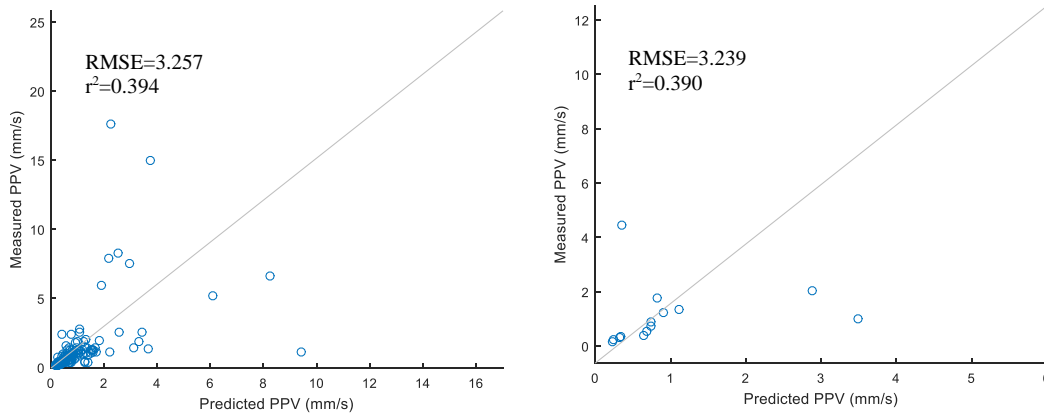
Figure 6.2 Predicted vs measured ground vibration levels for modeling set and testing set, respectively
