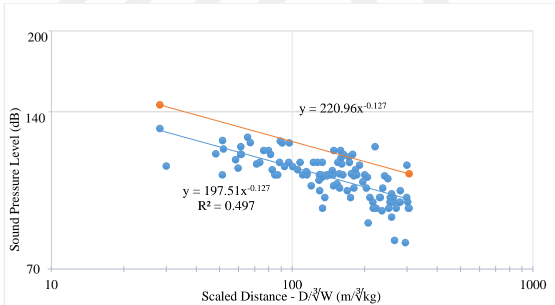
Figure 5.54 Karapinar unclassified production blasting air blast overpressure levels in dB
