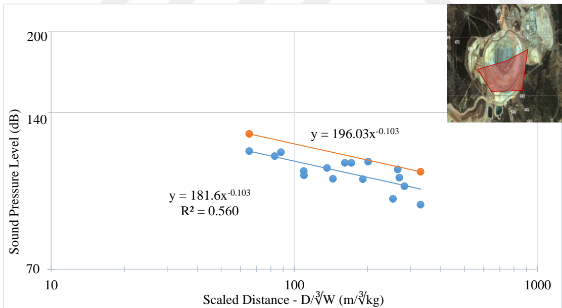
Figure 5.46 Gümüşkol Path 2 presplit blasting air blast overpressure levels in dB (Pit location- WSW, S, E, ENE - in front of the pit)
