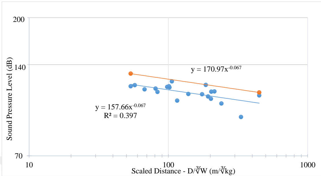
Figure 5.39 Gümüşkol Path 1 presplit blasting air blast overpressure levels (Northern winds-N, NE, NW)
