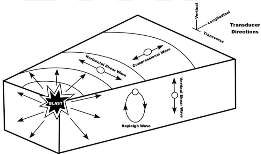
Figure 2.4 Particle motion associated with the different wave types (Richards & Moore, 2009a)
