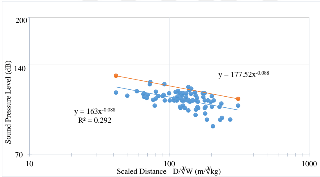
Figure 5.59 Gümüşkol Path 1 unclassified production blasting air blast overpressure levels in dB
