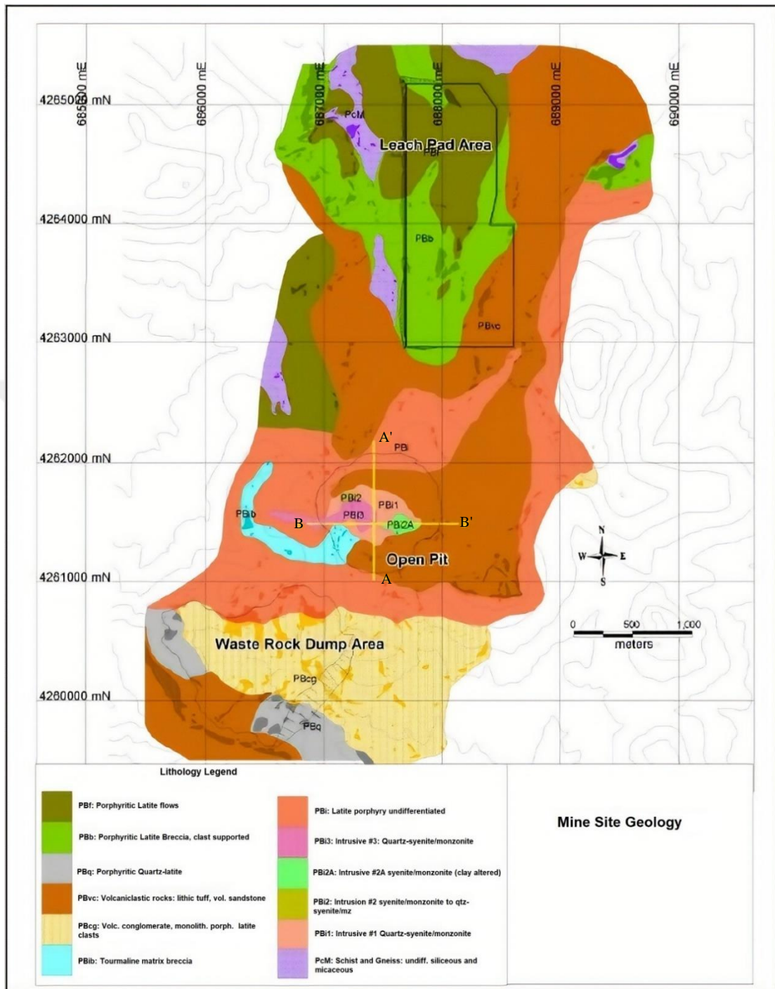
Figure 3.2 Mine site geology (Juras et al., 2010)
