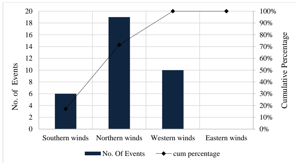
Figure 4.20 Frequency distribution of wind directions at the moment of blasting for Katrancılar
