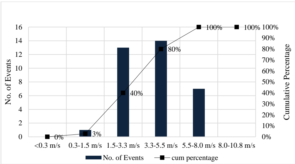
Figure 4.21 Frequency distribution of wind speeds at the moment of monitoring for Katrancilar
