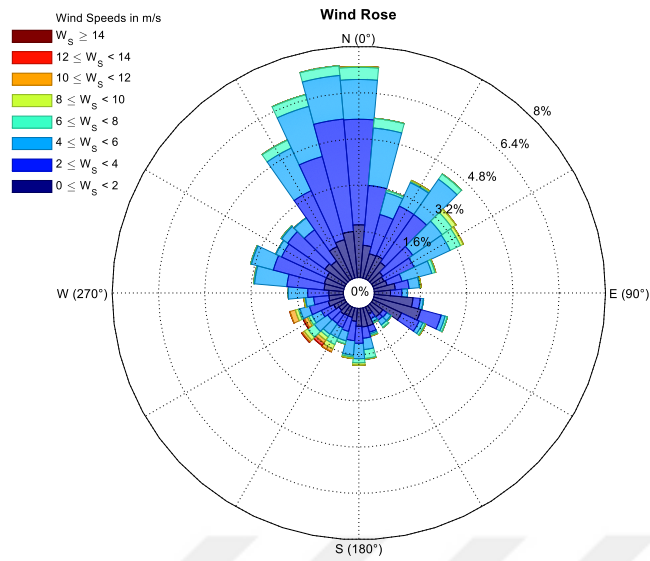
Figure 4.19 Wind rose for Kışladağ between April-July
