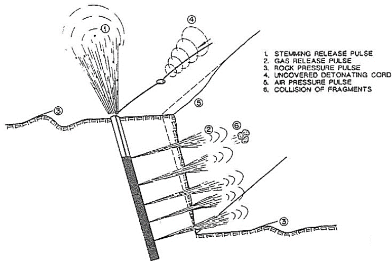
Figure 2.7 Sources of air blast (Jimeno et al., 1995)
