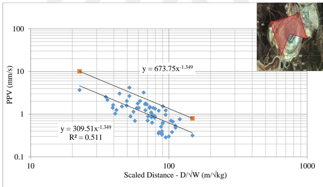
Figure 5.25 Gümüşkol Path 2 production blasting PPV values (Pit location- N, E, ESE, SSW, W, NNW- behind the pit)
