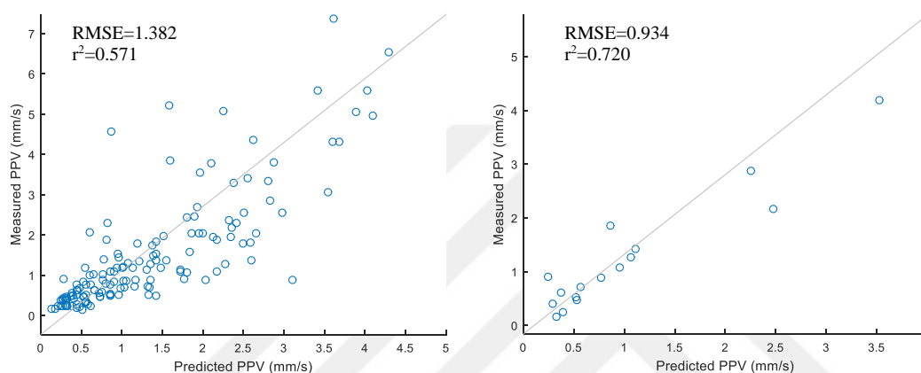
Figure 6.1 Predicted vs measured ground vibration levels for modeling set and testing set, respectively
