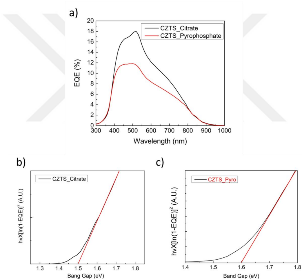
Figure 7.14 a) External quantum efficiency of CZTS films and band gaps of b) ITO/ZnO/CdS/CZTS_Citrate and c) ITO/ZnO/CdS/CZTS-Pyro cells
