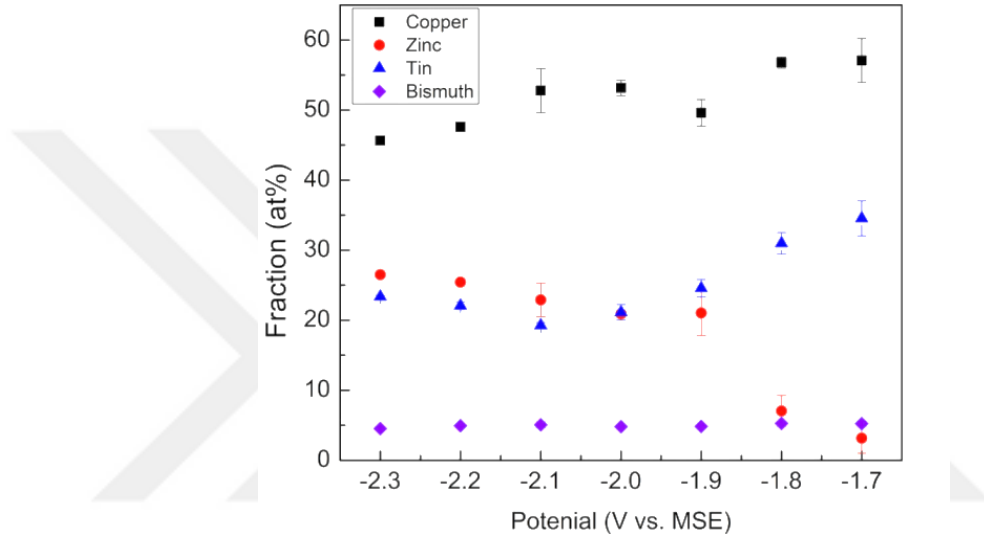
Figure 6.2 Compositional trends of Cu-Zn-Sn-Bi metallic precursors
