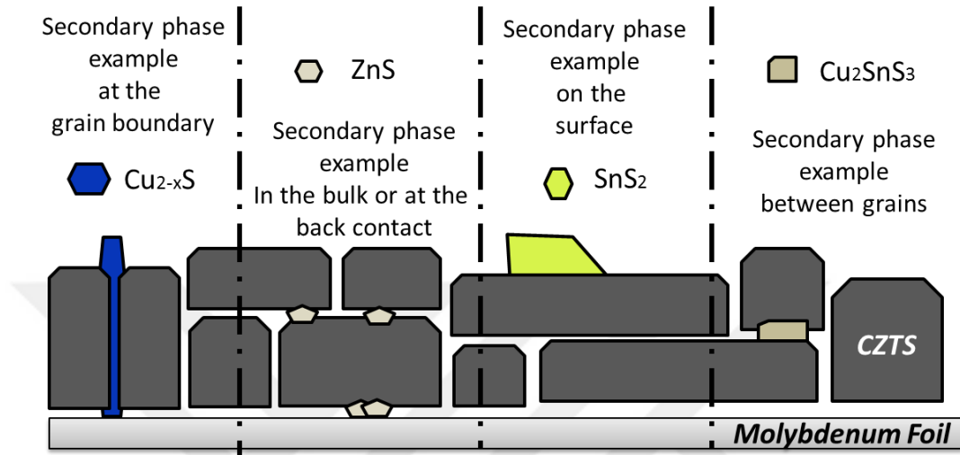
Figure 7.5 The most common secondary phases in CZTS absorber layers
