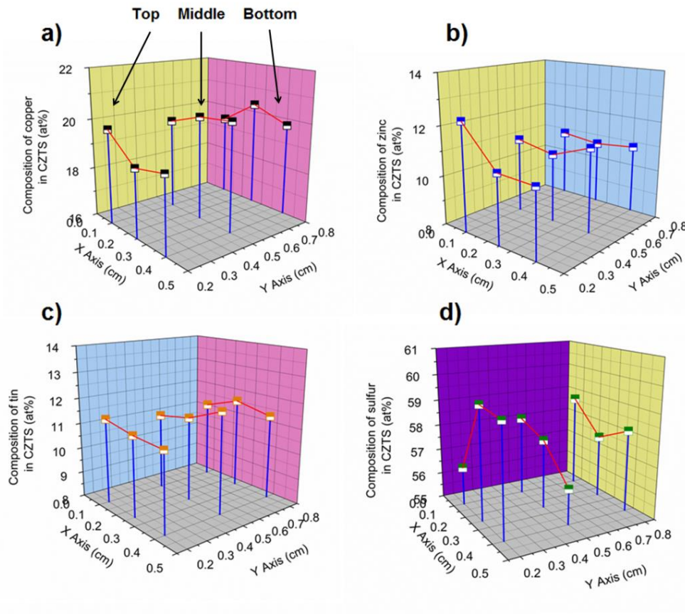
Figure 4.3 Composition of CZTS layers after sulfurization for a) copper, b) zinc, c) tin and d) sulfur (CZT precursor deposited at -2.05 V)
