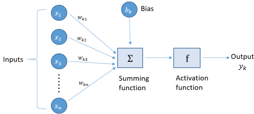
Figure 3.3: The General Concept of Artificial Neural Network
