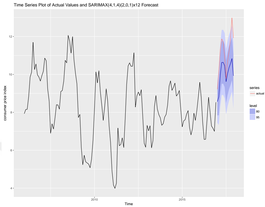
Figure A.8: Forecast Plot of SARIMAX(4, 1, 4)(2, 0, 1)_{12} with all exogenous variables
