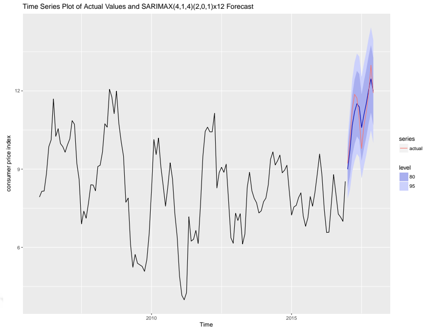
Figure 4.6: The SARIMAX forecasts of the CPI giving the best forecasts
