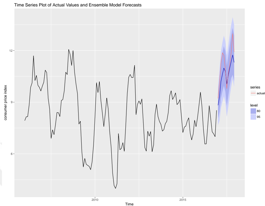
Figure 4.17: Ensemble Model of auto.arima and NNAR Methods
