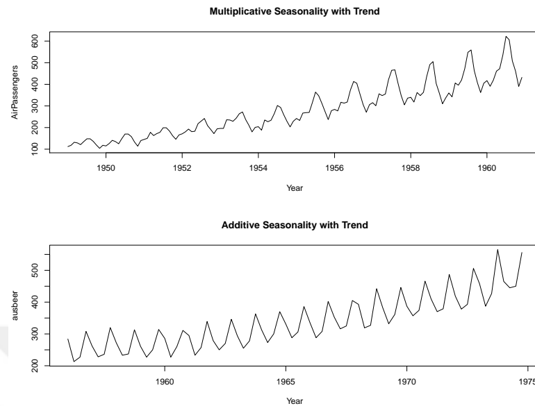
Figure 3.1: The time series plot of Additive and Multiplicative Seasonality
