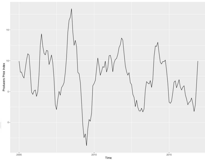
Figure A.2: Time Series plot of Producer Price Index
