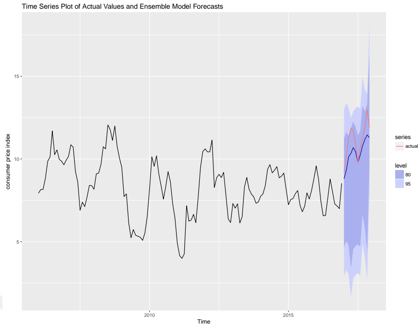
Figure 4.16: Ensemble Model of auto.arima, Theta and NNAR Methods
