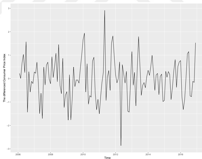
Figure 4.3: The overview of differenced consumer price index data
