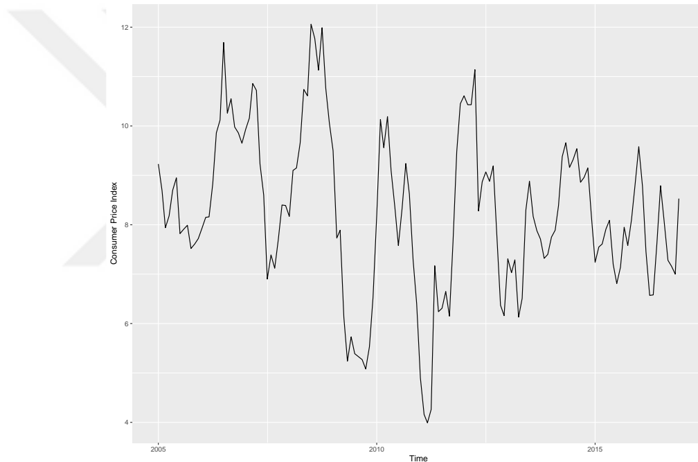
Figure 4.1: The overview of consumer price index
