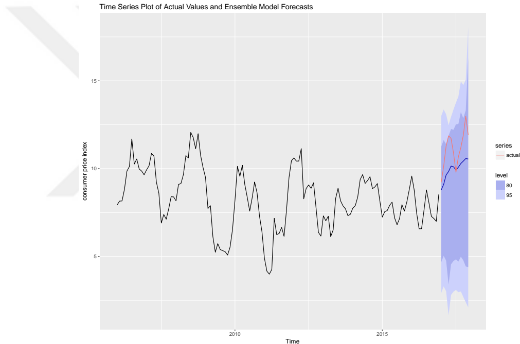
Figure 4.14: Ensemble Model of auto.arima, TBATS, NNAR, Theta and STL Models
