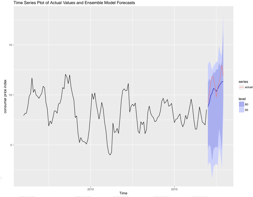
Figure 4.15: Ensemble Model of auto.arima, NNAR, Theta and STL Methods
