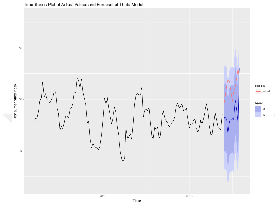
Figure 4.11: The Theta model's forecasts of the CPI
