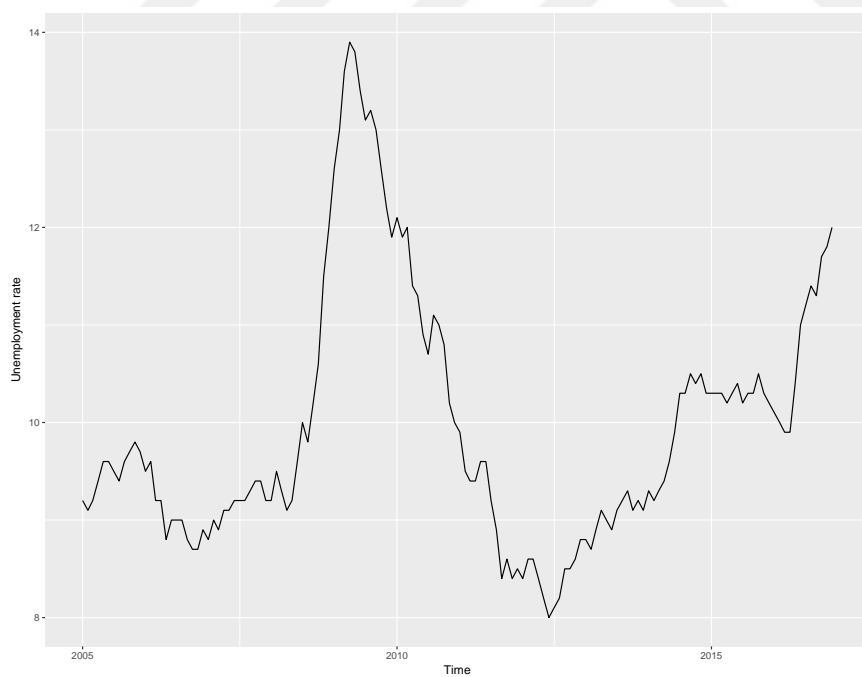
Figure A.3: Time Series Plot of Unemployment rate
