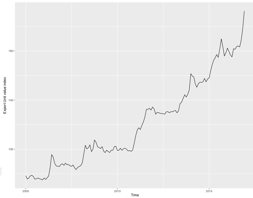
Figure A.6: Time Series Plot of Export Unit Value Index
