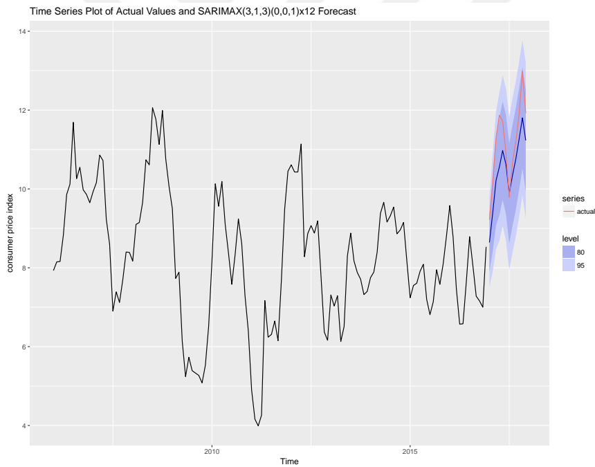
Figure 4.7: The SARIMAX forecasts of the CPI given the best train set performance
