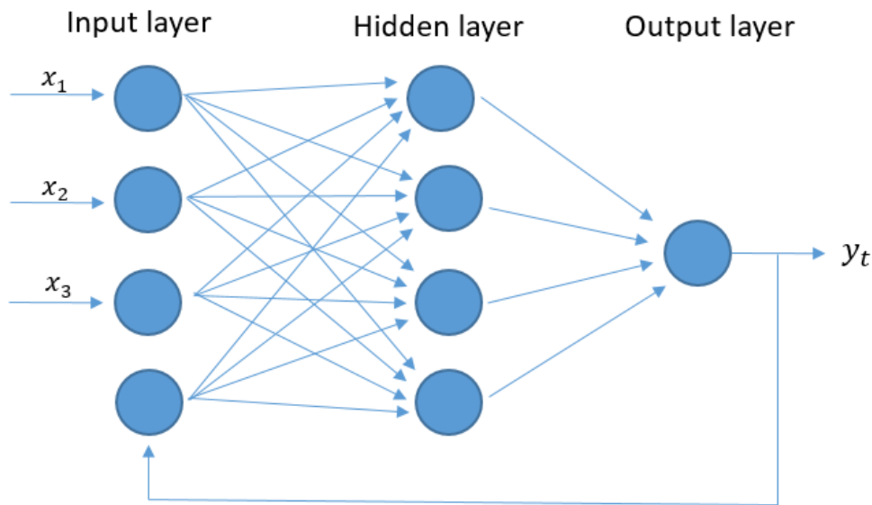
Figure 3.5: Recurrent Neural Network with Single Hidden Layer
