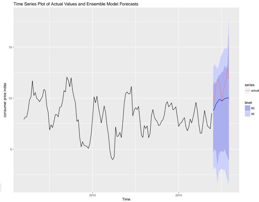
Figure 4.13: Ensemble Model of auto.arima, HW, TBATS, NNAR, Theta and STL Models with CV error
