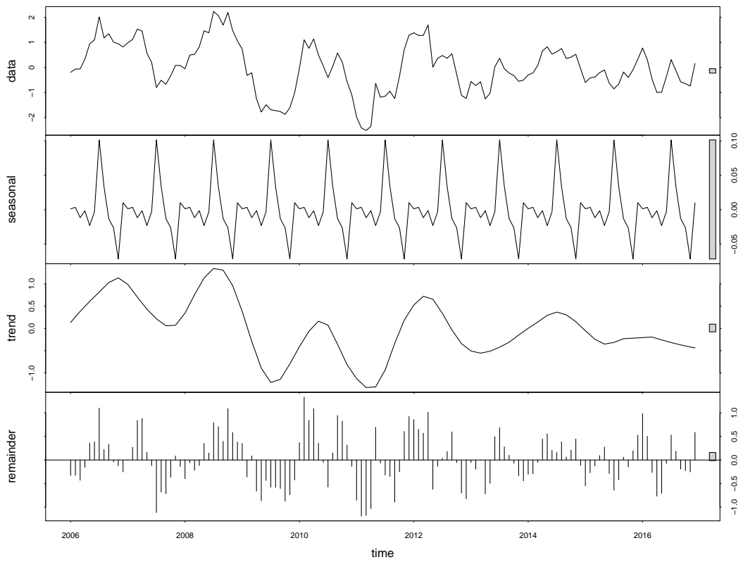
Figure A.1: STL Decomposition of the Turkish CPI
