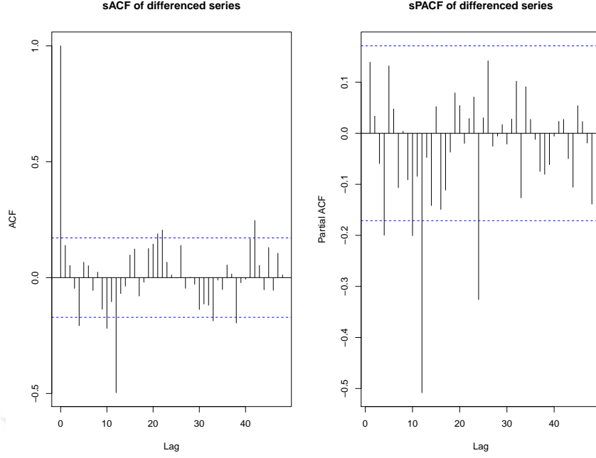
Figure 4.5: The sACF and sPACF of the differenced series
