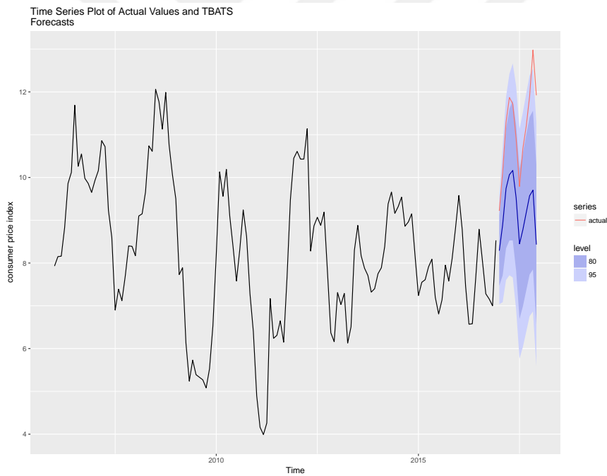
Figure 4.9: The TBATS forecasts of the CPI
