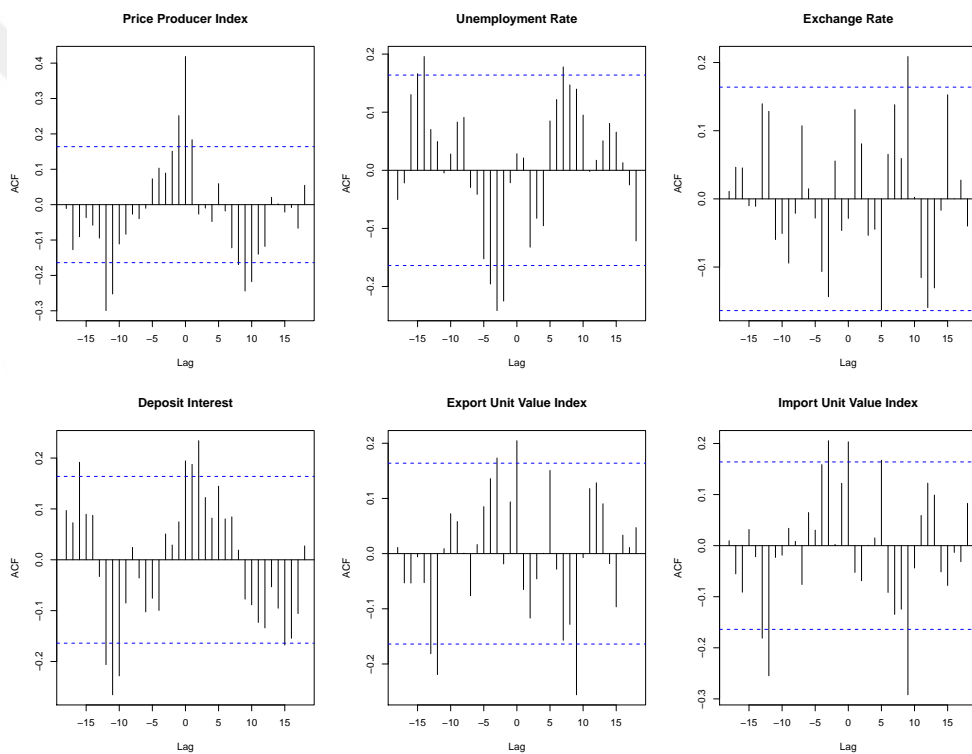
Figure 4.4: The CCF between Turkish CPI and each exogeneous variables
