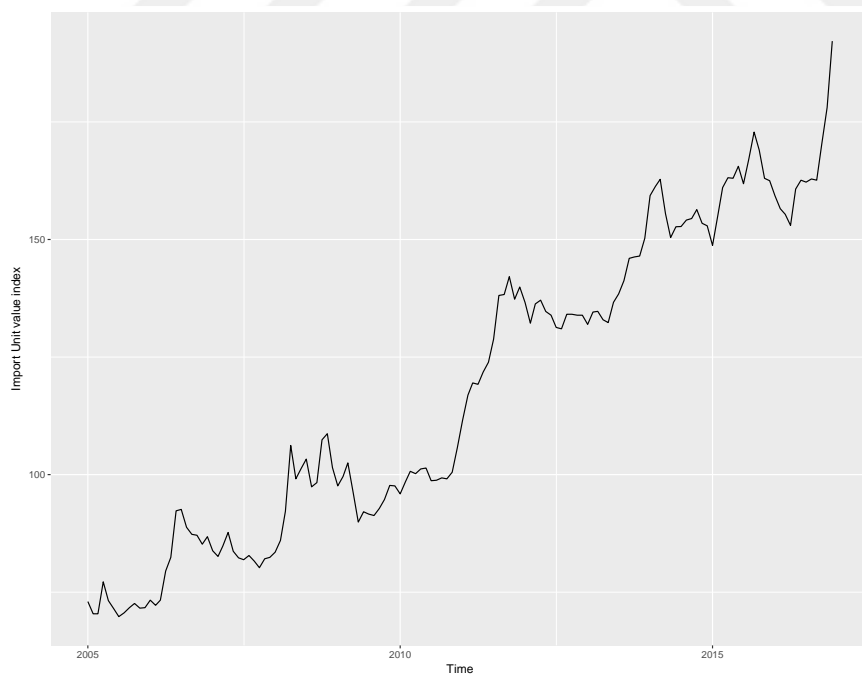
Figure A.7: Time Series Plot of Import Unit Value Index
