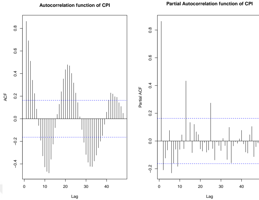
Figure 4.2: The sACF and sPACF of The Turkish CPI
