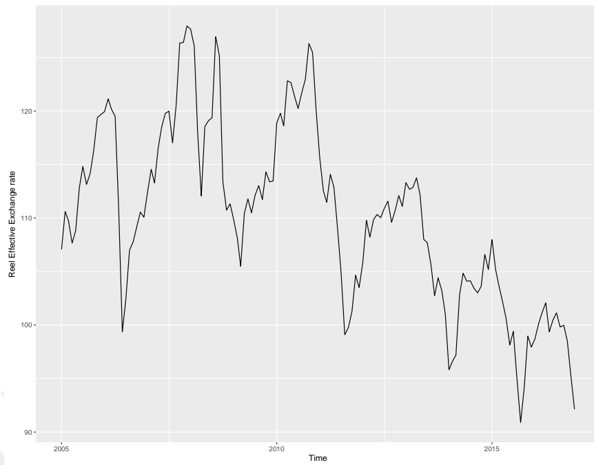
Figure A.4: Time Series Plot of Real Effective Exchange Rate
