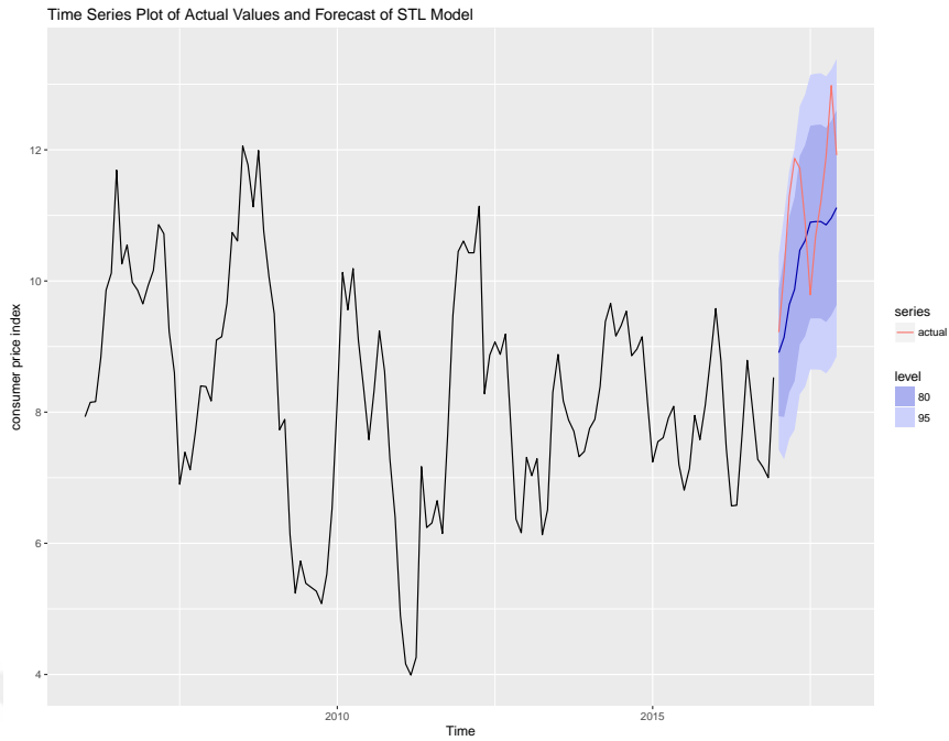
Figure 4.12: The STL forecast of the CPI
