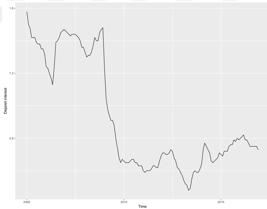
Figure A.5: Time Series Plot of Deposit Interest
