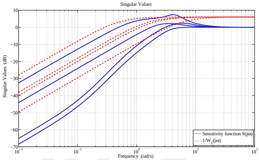
Figure 5.6: Singular value plots of the sensitivity function and inverse of the performance weight with the hinfstruct .
