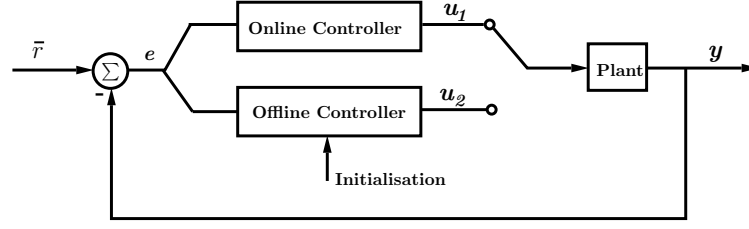
Figure 6.12: Switched controller diagram.
