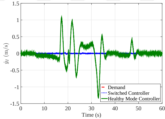
Figure 6.16: Velocity in y -direction while performing vertical velocity tracking of LOC in motor 3.
