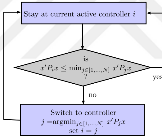
Figure 7.2: Min-switching strategy.
