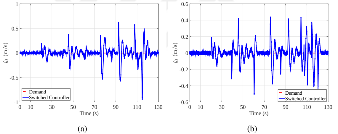
Figure 6.21: Velocity in y -direction during the vertical velocity tracking demand with the intermittent fault (a) with no controller state initialisation, (b) when controller state initialisation is employed.
