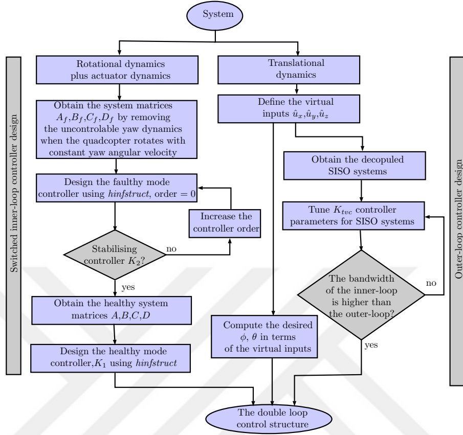
Figure 6.3: Flow diagram of the developed control structure of Fig. 6.1(b).
