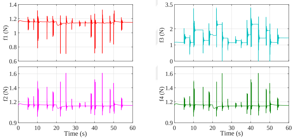
Figure 7.16: Switched H_2 state feedback control output when using the relaxed minimum switching strategy.
