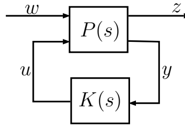
Figure 5.1: Standard feedback system.
