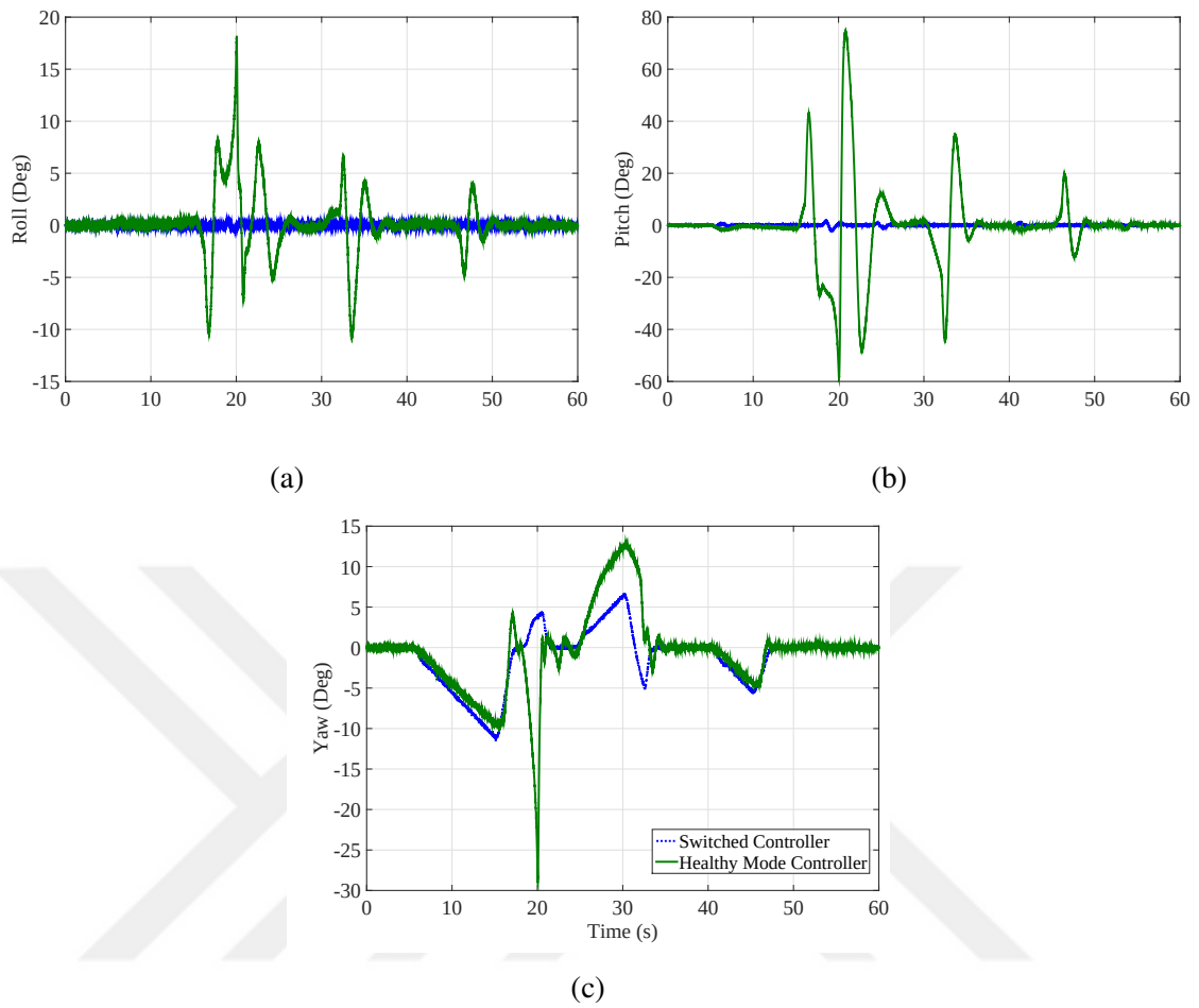
Figure 6.17: Euler angles corresponding to Fig. 6.14.
