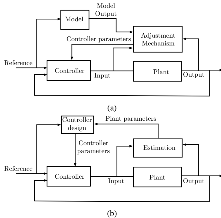
Figure 2.5: Adaptive control systems (a) MRAC, (b) STC (adopted from [9]).
