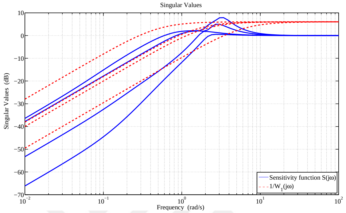
Figure 5.4: Singular value plots of the sensitivity function and inverse of the performance weight with the controller designed using the hifoo .
