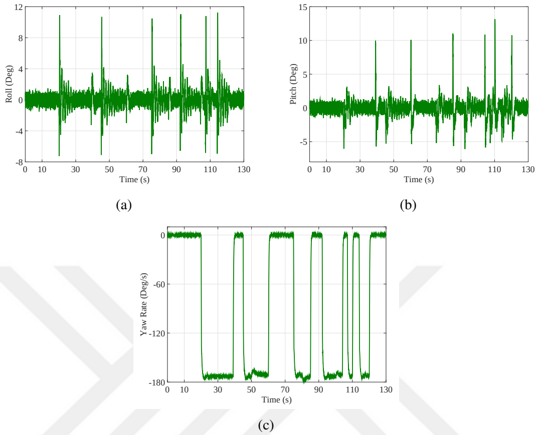
Figure 6.23: Roll and pitch angles, and yaw angular velocity, corresponding to Figs. 6.19-6.21 when the switched recovery controller with state initialisation is used.
