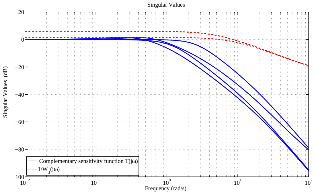
Figure 5.9: Singular value plots of the complementary sensitivity function and inverse of the stability weight with the LMI.
