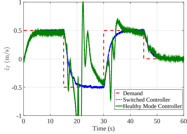
Figure 6.14: Heave velocity tracking response when the quadcopter vehicle experiences an intermittent LOC for motor 3.
