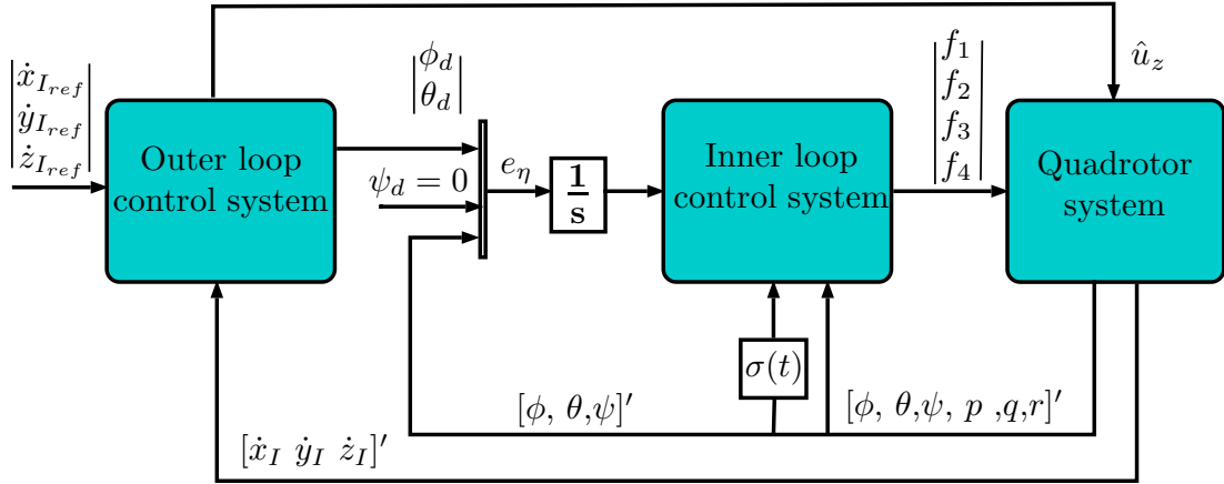
Figure 7.6: An overview of the control structure.
