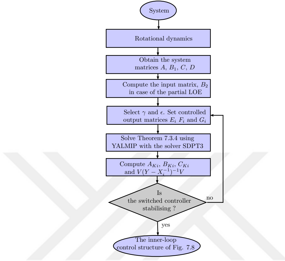
Figure 7.9: Flow diagram of the switched H_\infty dynamic output feedback control design.
