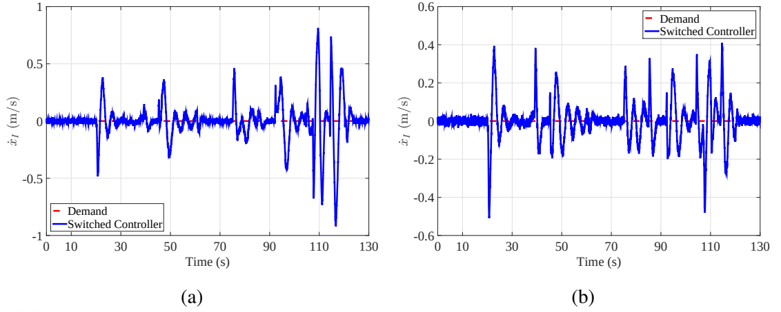
Figure 6.20: Velocity in x -direction while the quadcopter tracks the vertical velocity demand of Fig. 6.21 with the intermittent fault (a) when there is no controller state initialisation, (b) when the controller state initialisation is employed.
