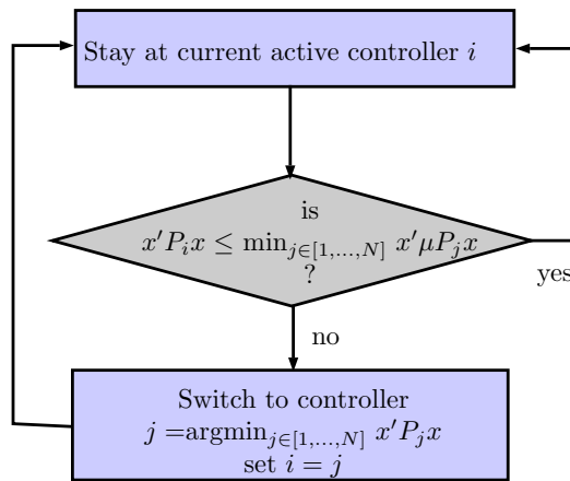
Figure 7.4: Relaxed min-switching strategy.
