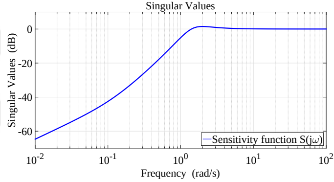
Figure 6.8: Singular value plot of the S(j\omega) for the closed-loop outer subsystem
