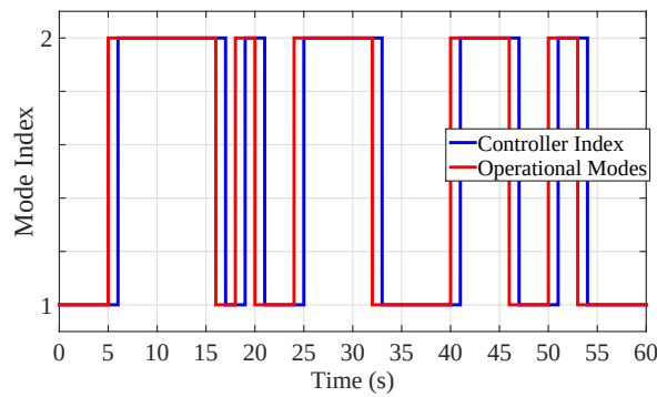
Figure 6.13: A random LOC profile and the corresponding controller with T_D delay: 2 indicates the loss of control mode and 1 indicates the fault-free mode.
