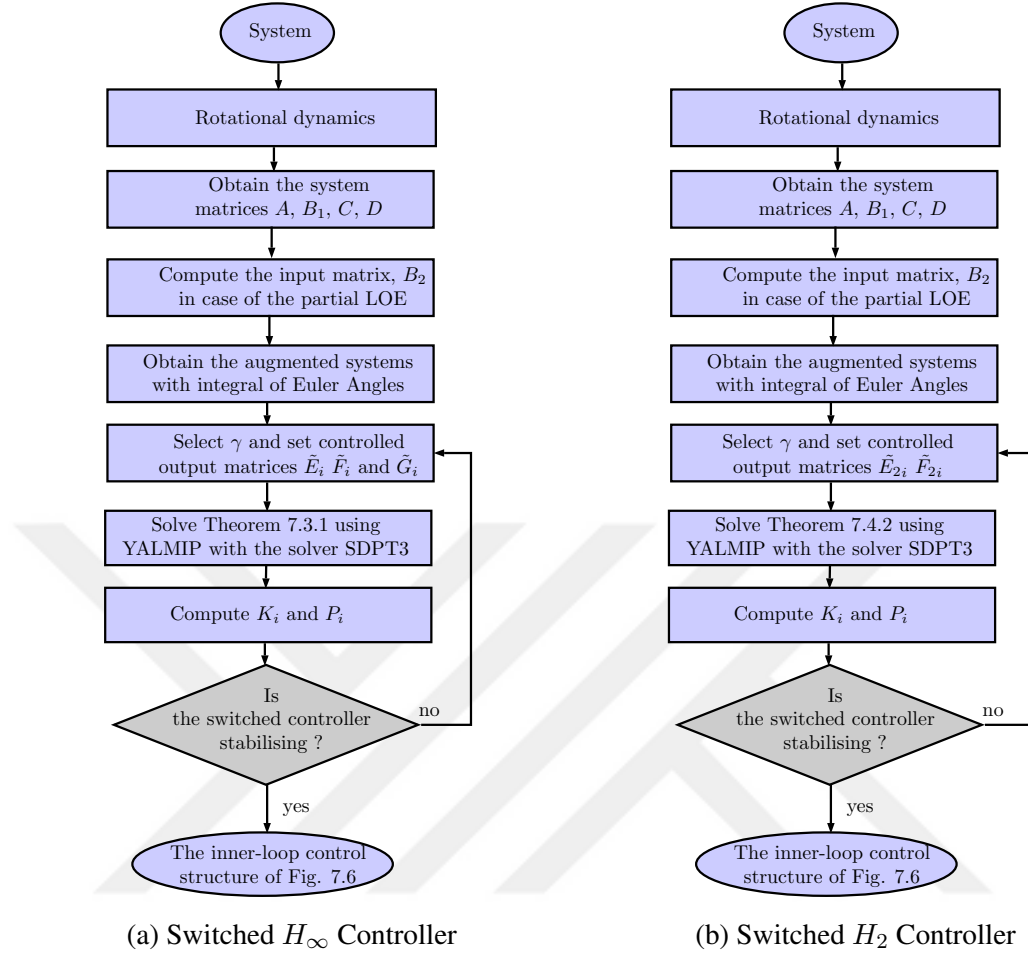
Figure 7.7: Flow diagrams of the switched state feedback controller designs.
