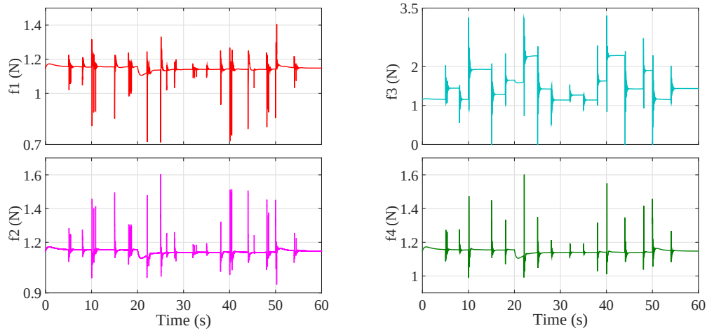
Figure 7.15: Switched H_\infty state feedback control output when using the relaxed minimum switching strategy.
