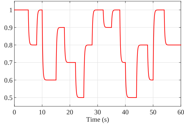
Figure 7.10: Profile for the loss of effectiveness in motor 3.
