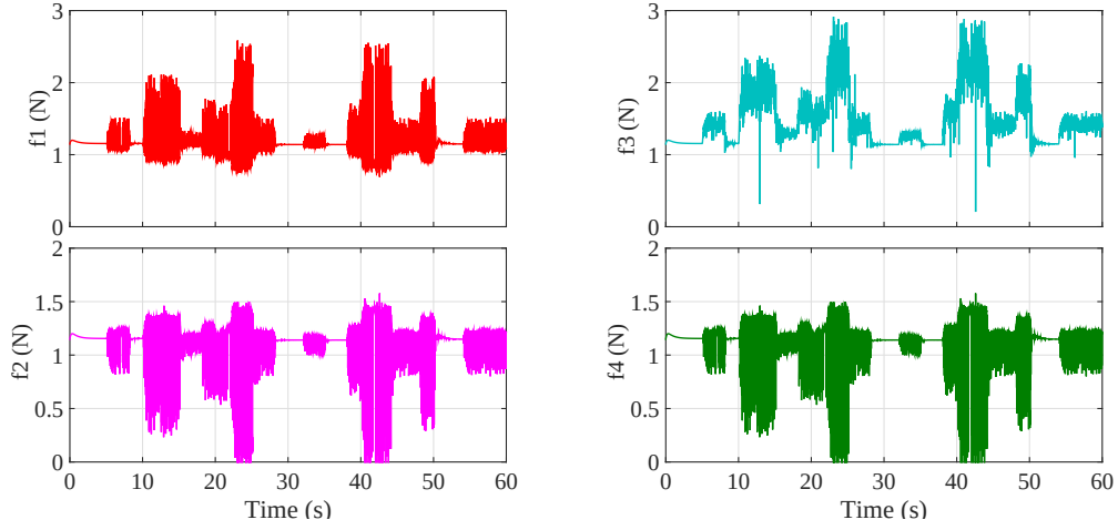
Figure 7.18: Switched dynamic output feedback H_\infty control outputs.
