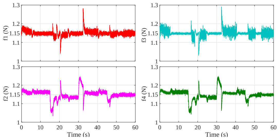
Figure 6.18: Control inputs when the switched controller is used under LOC conditions.
