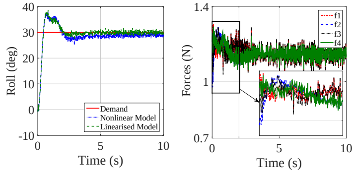
(a) Roll angle and corresponding motor forces.
