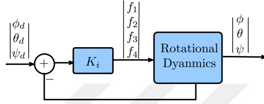
Figure 6.4: Inner-loop control structure in the case of ILOC, where K_i \in \{K_1, K_2\} .
