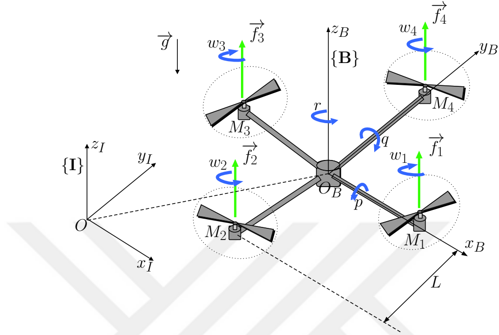
Figure 4.1: Body-fixed and inertial-fixed frames for a quadcopter UAV model.
