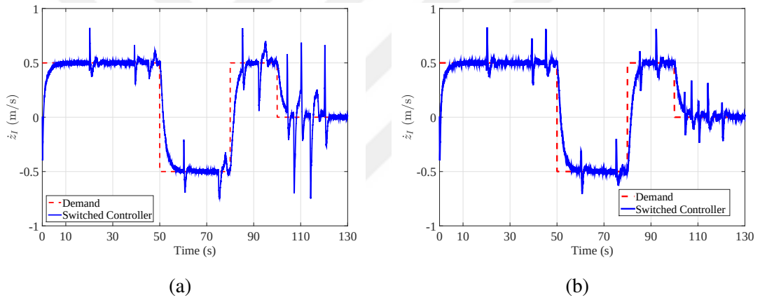
Figure 6.19: Heave velocity tracking responses (a) when there is no controller state initialisation, (b) when controller state initialisation is employed.
