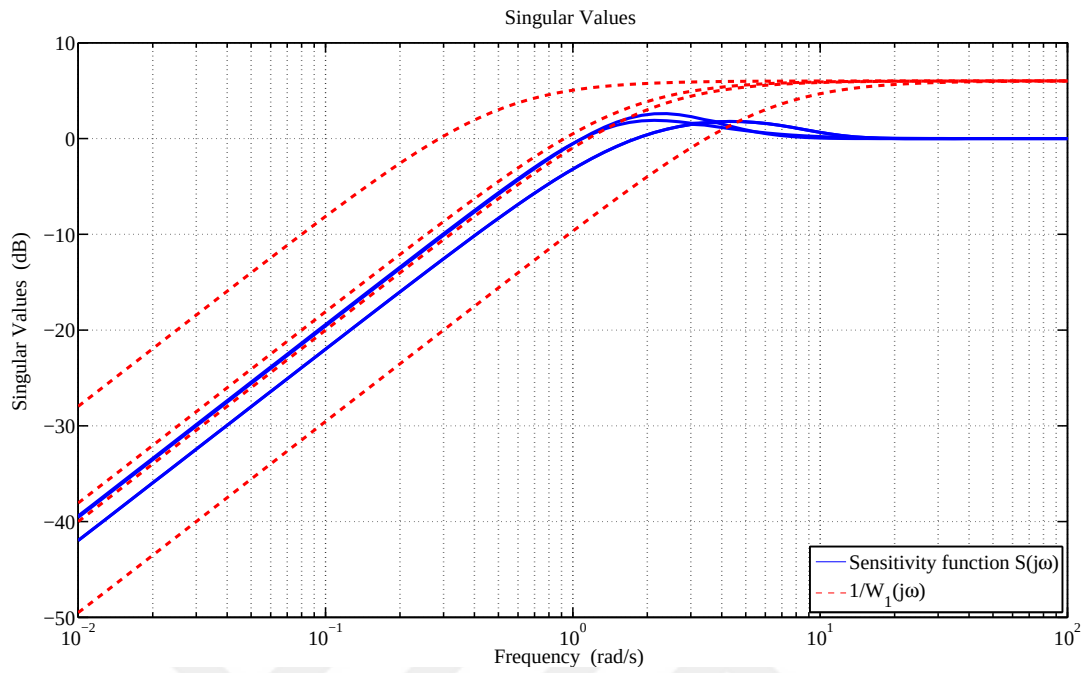
Figure 5.10: Singular value plots of the sensitivity function and inverse of the performance weight with the Glover-Doyle.
