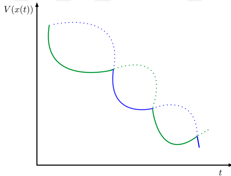
Figure 3.3: Lyapunov function values versus time ( N = 2 ) with the min-switching strategy.
