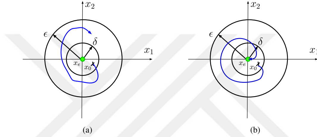
Figure 3.1: Illustrations of (a) a stable equilibrium in the sense of Lyapunov, and (b) an asymptotically stable equilibrium.
