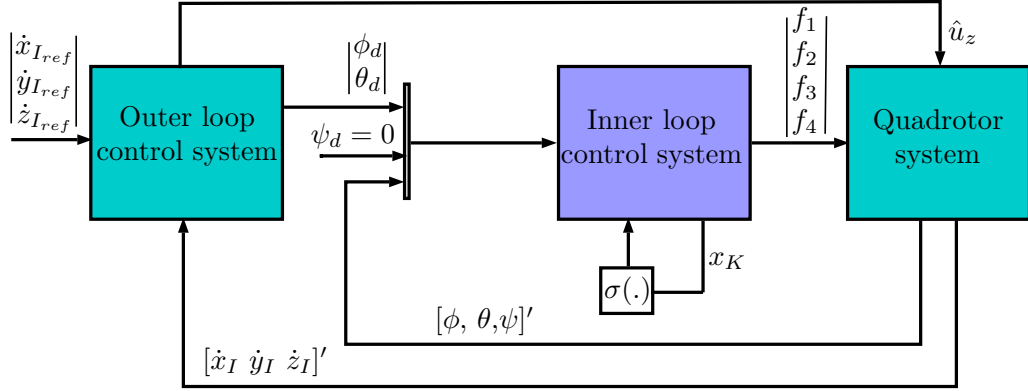
Figure 7.8: Modified structure for switched dynamic output feedback control.
