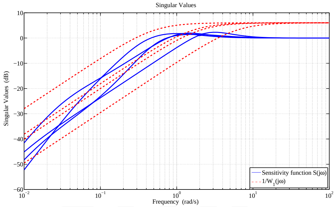
Figure 5.8: Singular value plots of the sensitivity function and inverse of the performance weight with the LMI.
