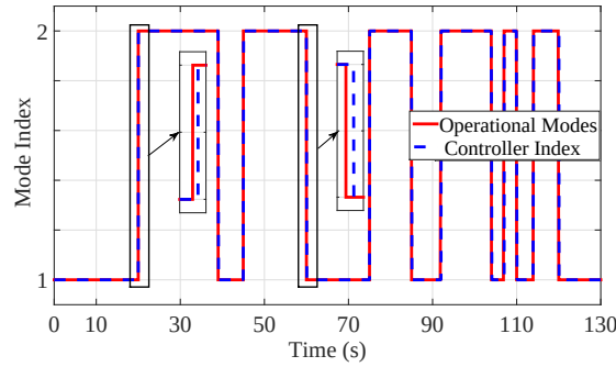
Figure 6.22: A random intermittent rotor fault profile: 2 is the rotor fault mode and 1 is the fault-free mode; the solid red line shows the operational modes and the blue dotted line shows the controller index.
