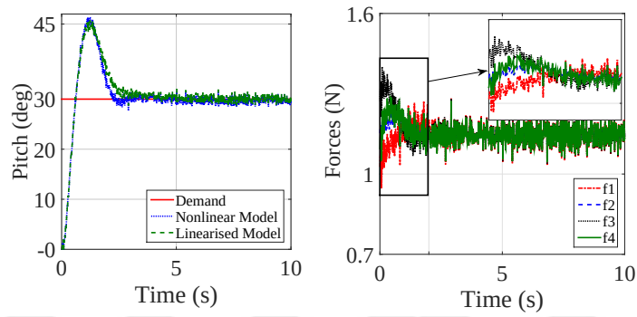
(b) Pitch angle and corresponding motor forces.
