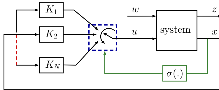
Figure 7.1: A state-dependent switched control scheme.
