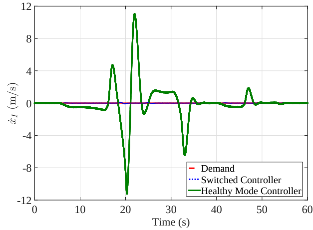
Figure 6.15: Velocity in the x -direction while performing vertical velocity tracking of LOC in motor 3.
