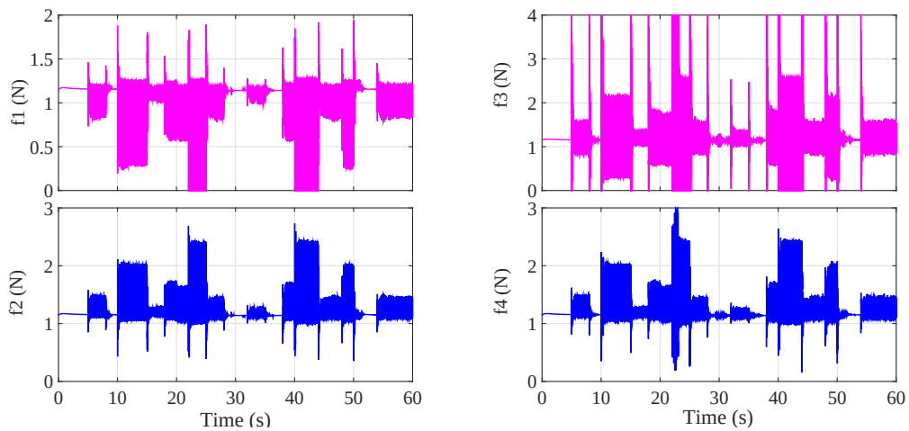
Figure 7.13: Switched H_2 state feedback control output.
