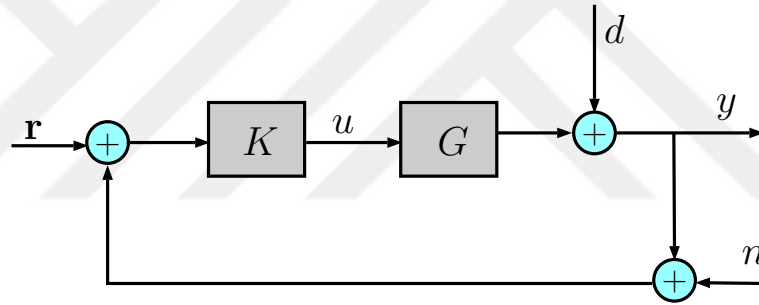
Figure 2.4: Closed-loop system.
