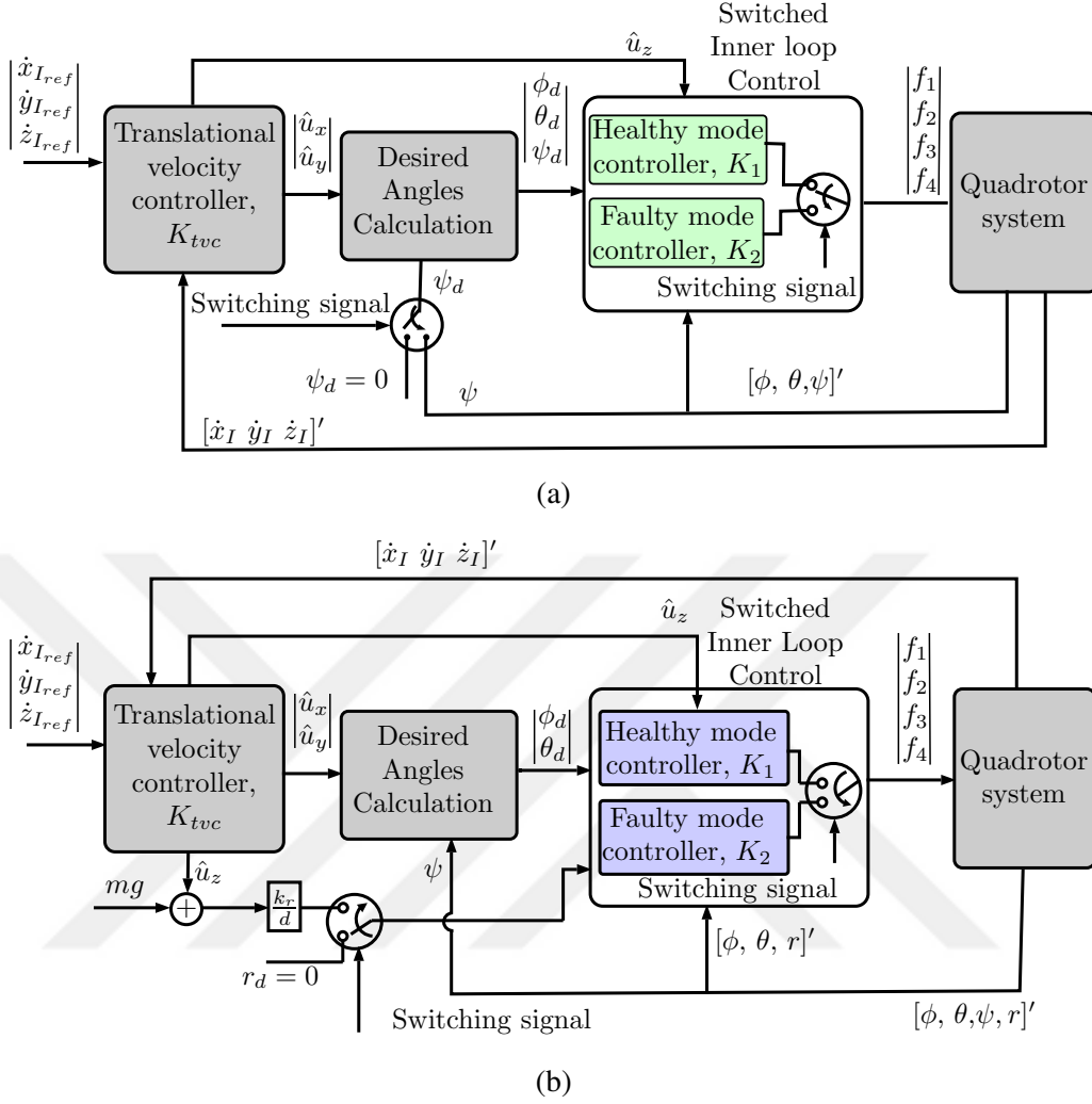
Figure 6.1: The double-loop control structure for translational tracking (a) in the case of ILOC, (b) in the case of ILOM.
