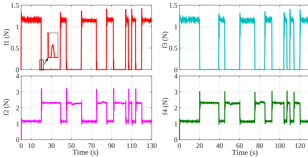
Figure 6.24: Control inputs when the switched controller with state initialisation is used.
