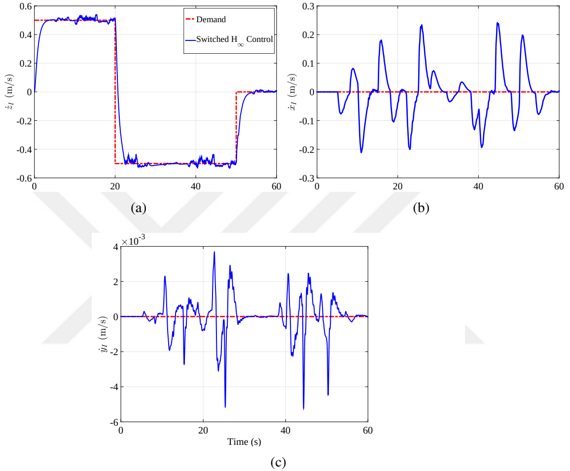
Figure 7.17: Translational velocities in the presence of a time-varying LOE in motor 3 when the switched H_\infty dynamic output controller is used.
