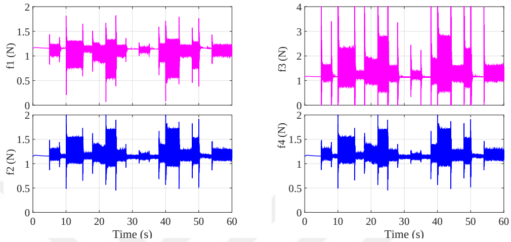
Figure 7.12: Switched H_\infty state feedback control output.
