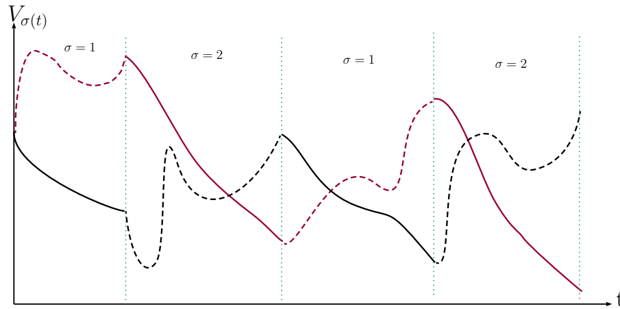
Figure 3.2: Multiple Lyapunov function values versus time ( N = 2 ). Solid/dotted denotes corresponding system activity/inactivity (adopted from [21]).
