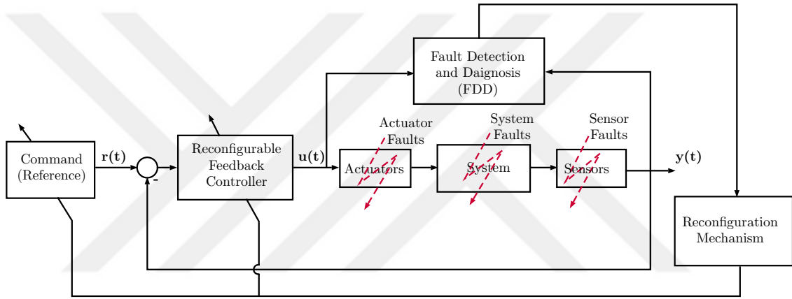
Figure 2.2: A structure of an active fault tolerant control system (adopted from [160]).
