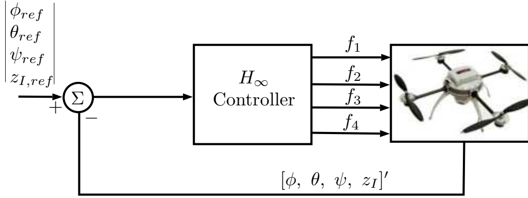
Figure 5.3: Closed-loop control structure.
