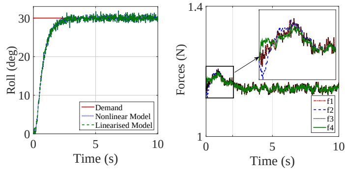
(a) Roll angle and corresponding motor forces.
