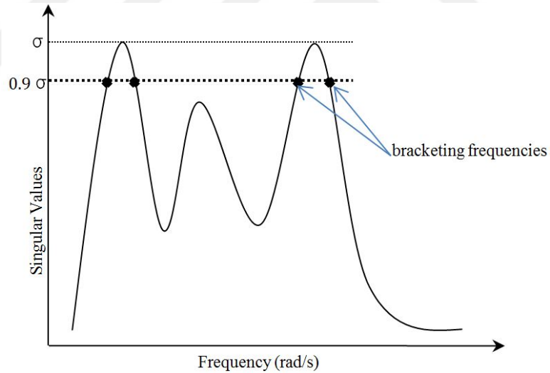
Figure 5.2: Frequencies at current iteration to build a tangent model [44].
