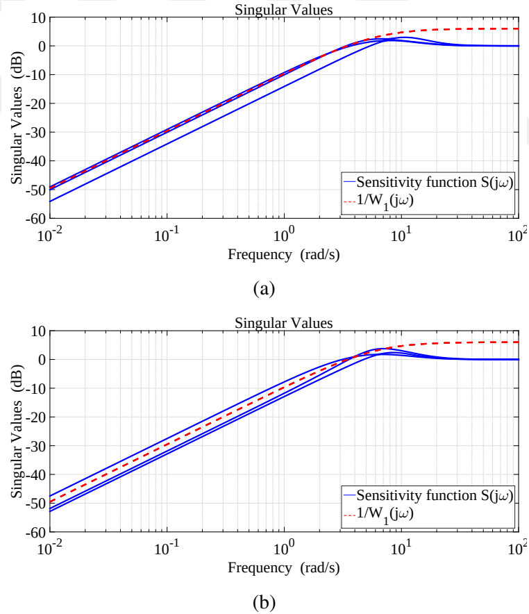
Figure 6.5: Singular value plots of the S(j\omega) and inverse of the performance weight in the case of ILOC (a) for the healthy mode, and (b) for the faulty mode of operation.
