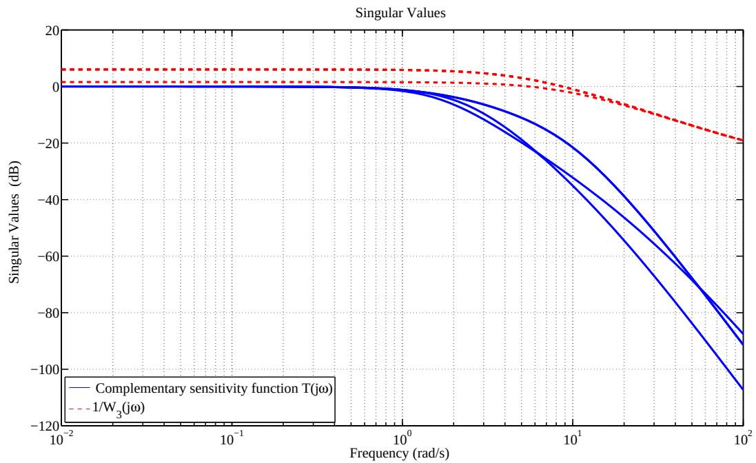
Figure 5.11: Singular value plots of the complementary sensitivity function and inverse of the stability weight with the Glover-Doyle.
