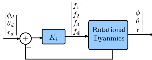
Figure 6.6: Inner-loop control structures (a) in the case of ILOC and (b) in the case of ILOM, where K_i \in \{K_1, K_2\} .
