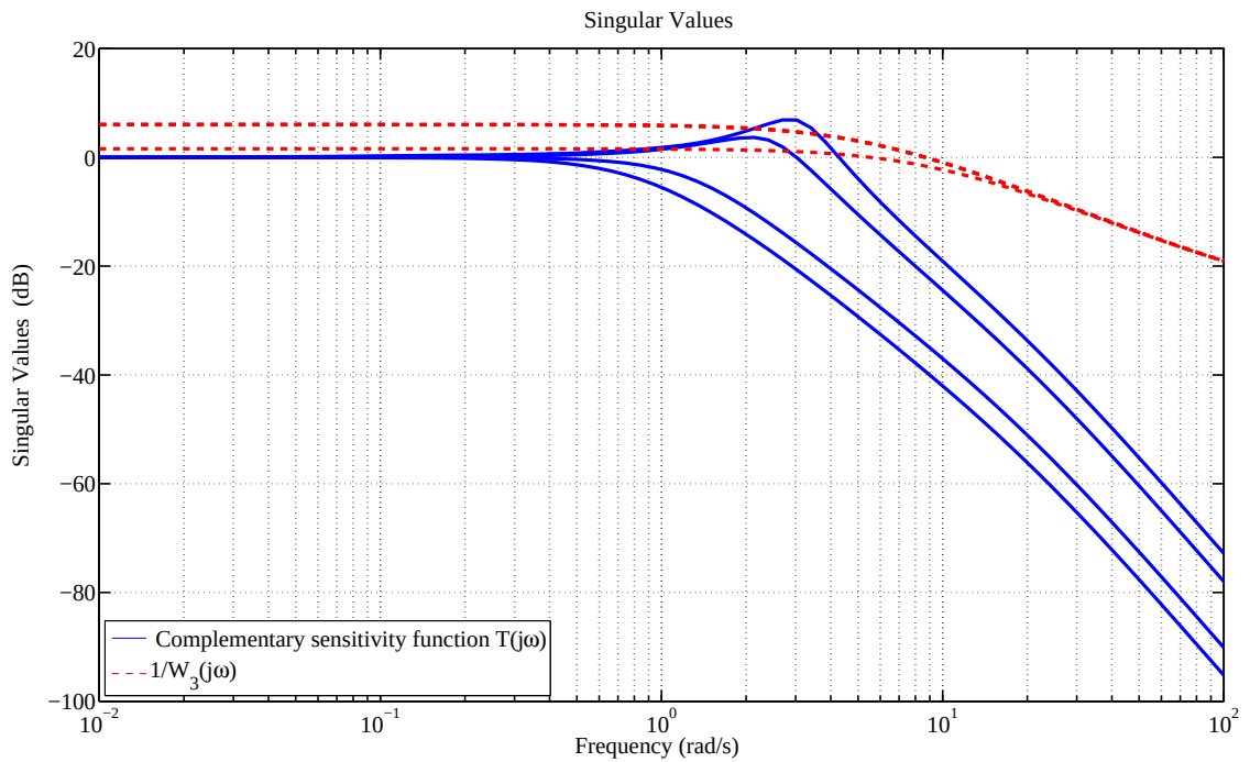
Figure 5.5: Singular value plots of the complementary sensitivity function and inverse of the stability weight with the hifoo .
