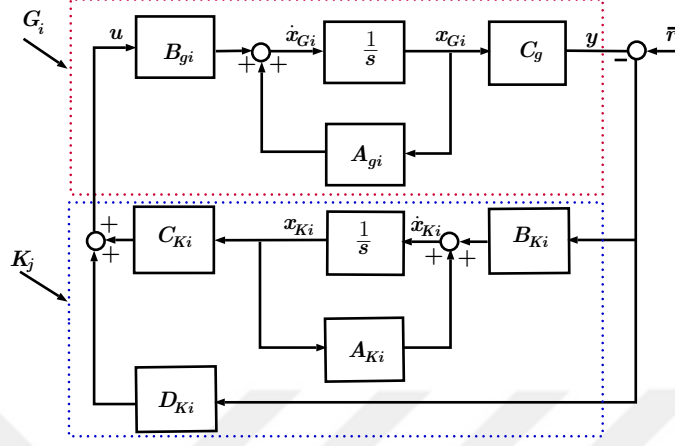
Figure 6.9: A state-space realisation of the closed-loop system.
