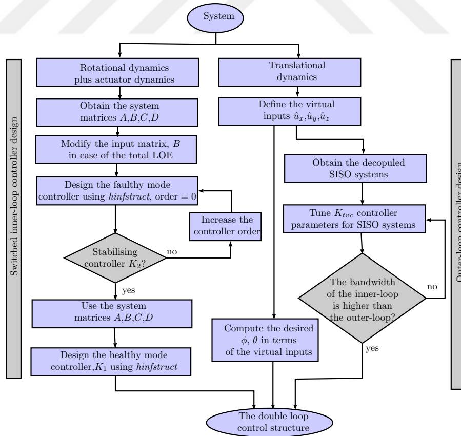
Figure 6.2: Flow diagram of the developed control structure of Fig. 6.1(a).
