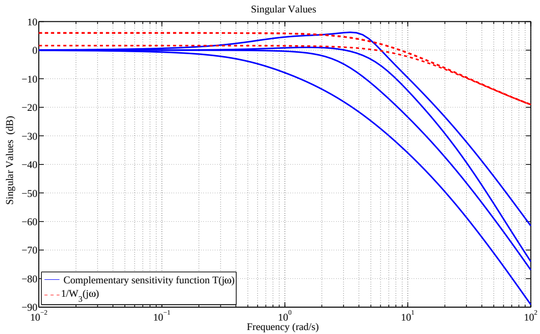
Figure 5.7: Singular value plots of the complementary sensitivity function and inverse of the stability weight with the hinfstruct .
