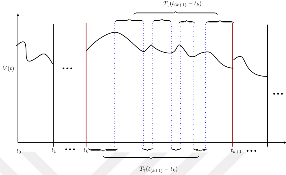
Figure 6.11: Extended Lyapunov-like function.
