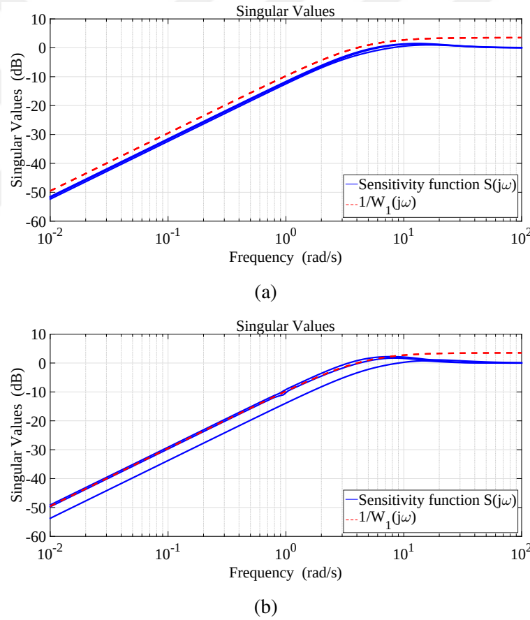
Figure 6.7: Singular value plots of the S(j\omega) and inverse of the performance weight in the case of ILOM (a) for the healthy mode, (b) for the faulty mode of operation.
