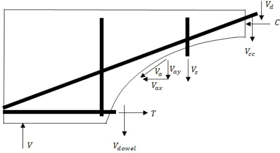
Figure 4.4. Shear resisting forces in a beam after the formation of a shear crack
