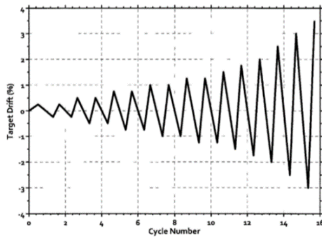
Figure 5.54. Lateral displacement history for coupled wall systems
