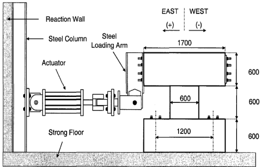
a) Specimen model when there are no arms holding the ends of the top wall segment (Canbolat, 2004)
