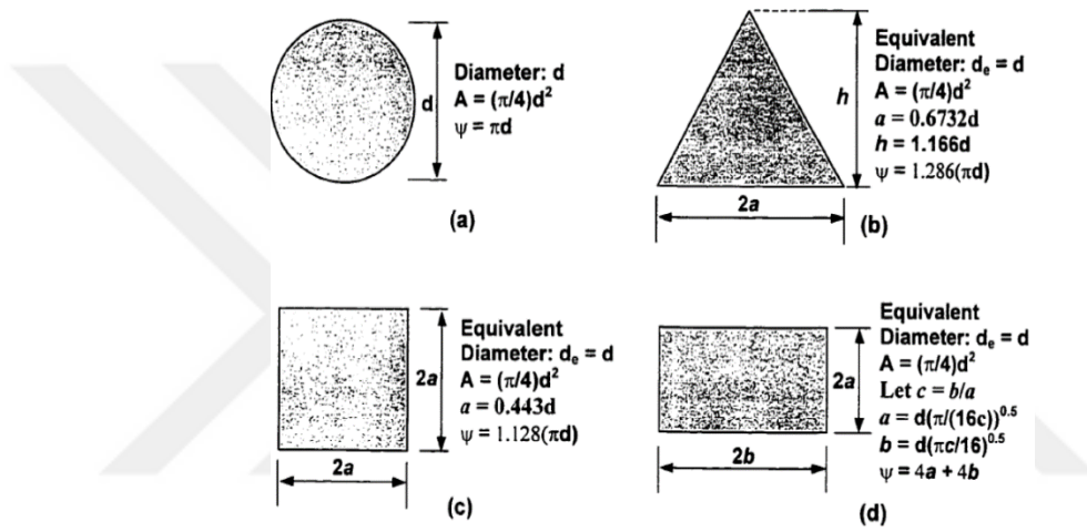
Figure 3.1. Equivalent cross-sections: a) circular, b) triangular, c) square, d) rectangular
