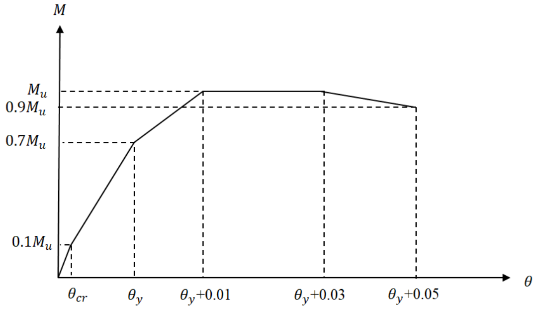
b) Moment-rotation relationship for DCBs
