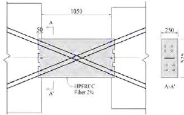
Figure 5.42. Reinforcement detailing of Specimen FC-0.0
