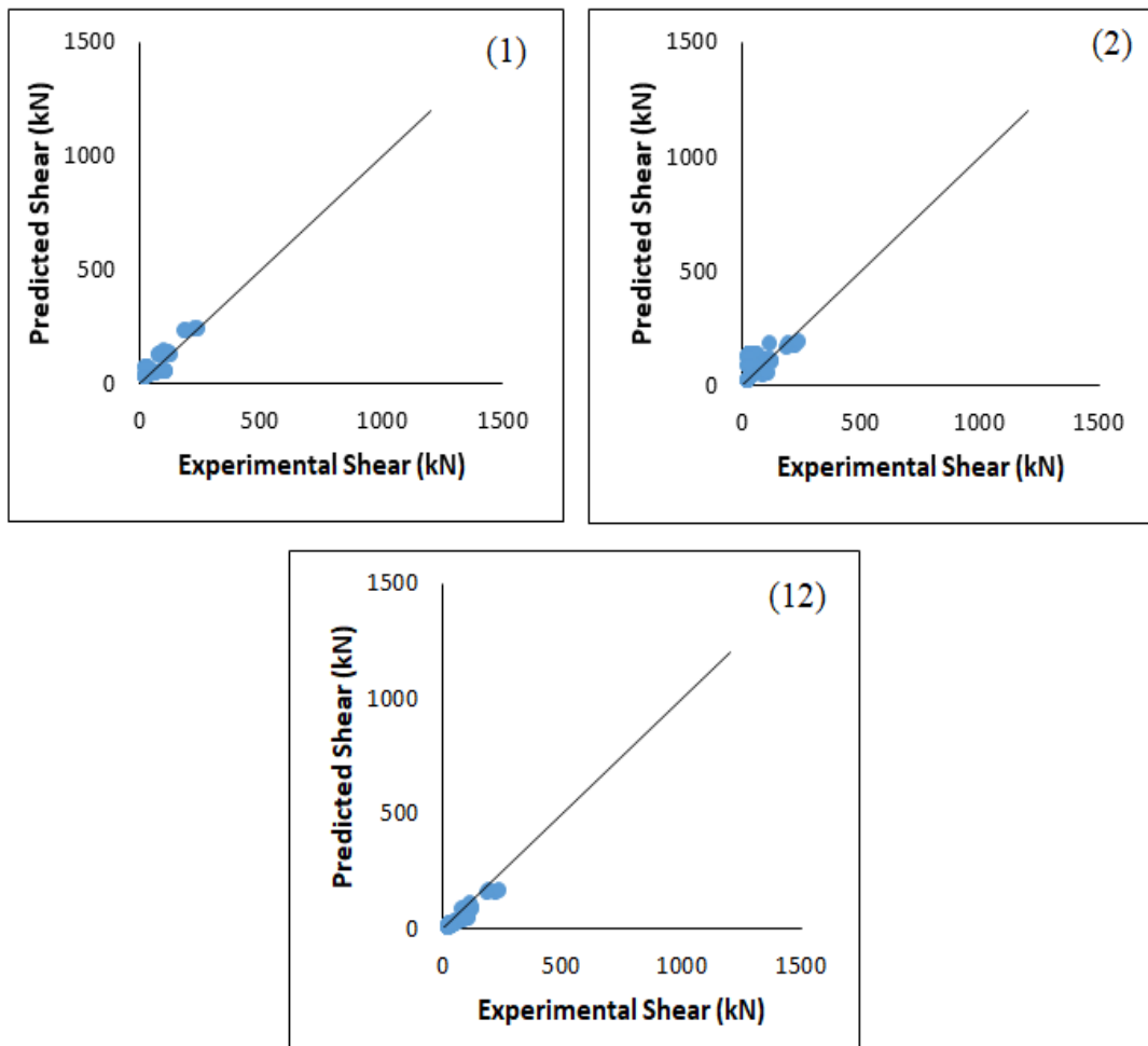
Figure 4.11. Shear strength predictions for Deep Beams ( a/d > 2.5 ) with transverse reinforcement: (1) ACI 318-14 (2014); (2) Sharma (1986); (12) Proposed method
