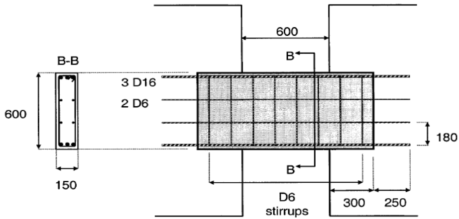
Figure 5.24. Reinforcement detailing of Specimen 2
