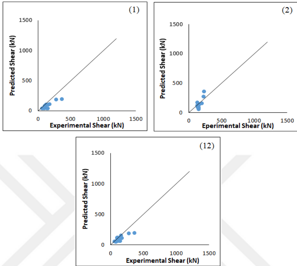
Figure 4.9. Shear strength predictions for Deep Beams ( a/d \leq 2.5 ) with transverse reinforcement: (1) ACI 318-14 (2014); (2) Sharma (1986); (12) Proposed method
