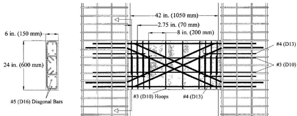
Figure 5.22. Reinforcement detailing of Specimen CB-3
