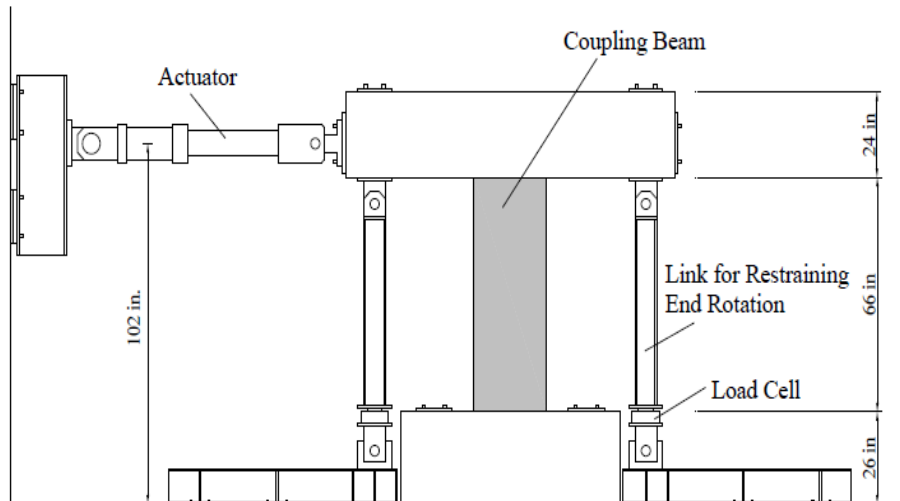
b) Test setup when there are arms holding the ends of the top wall segment
