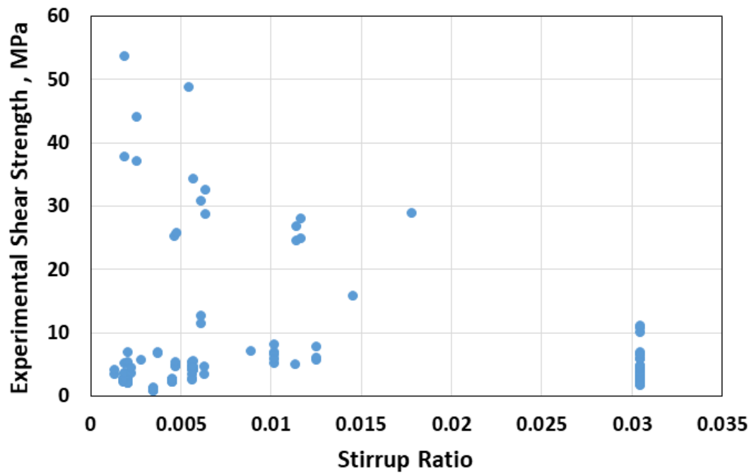
Figure 4.7. Influence of the stirrup ratio on shear strength of FRC beams
