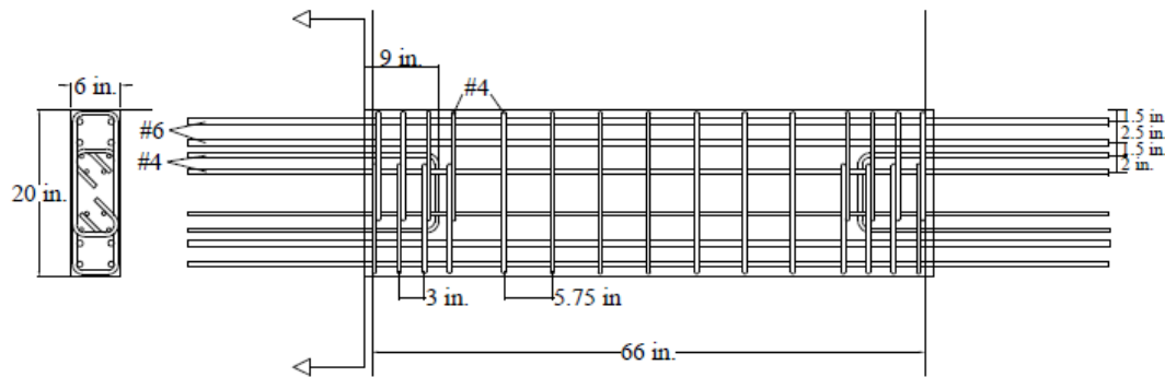
Figure 5.14. Reinforcement detailing of Specimen CB-5
