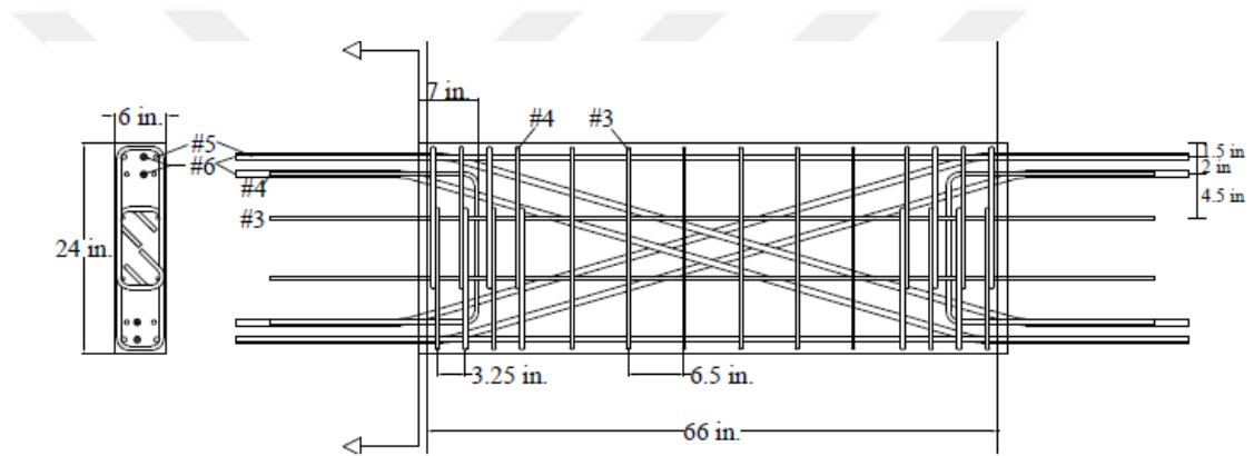
Figure 5.10. Reinforcement detailing of Specimen CB-2
