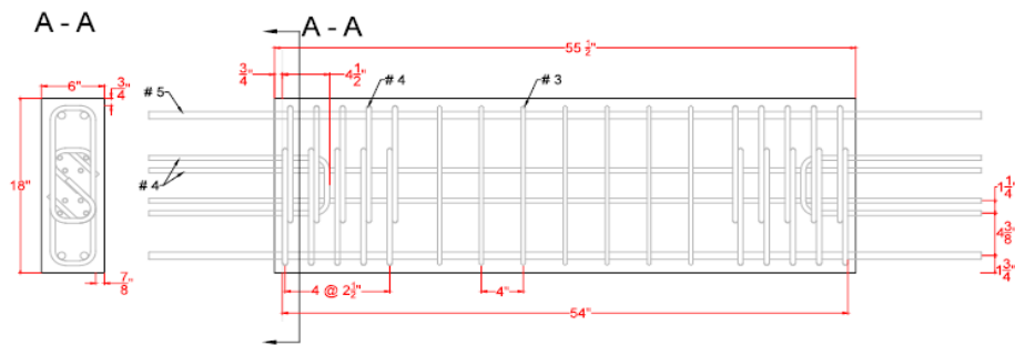
Figure 5.49. Reinforcement detailing of Specimen CB4
