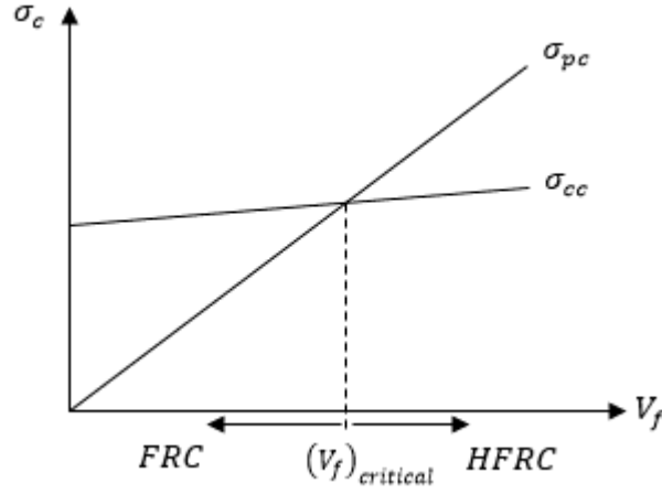
Figure 2.2. Critical fiber volume fraction (Hull and Clyne, 1996)
