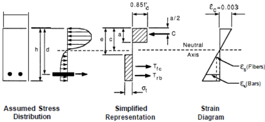
Figure 2.10. Stress and Strain Distributions for Single Reinforced SFRC Beams (Hanegar and Doherty, 1976)
