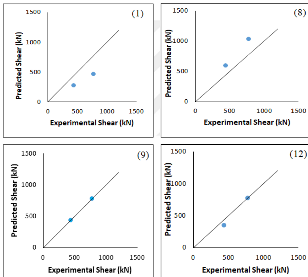
Figure 4.16. Shear strength predictions for HPFRC Coupling Beams without transverse reinforcement:
