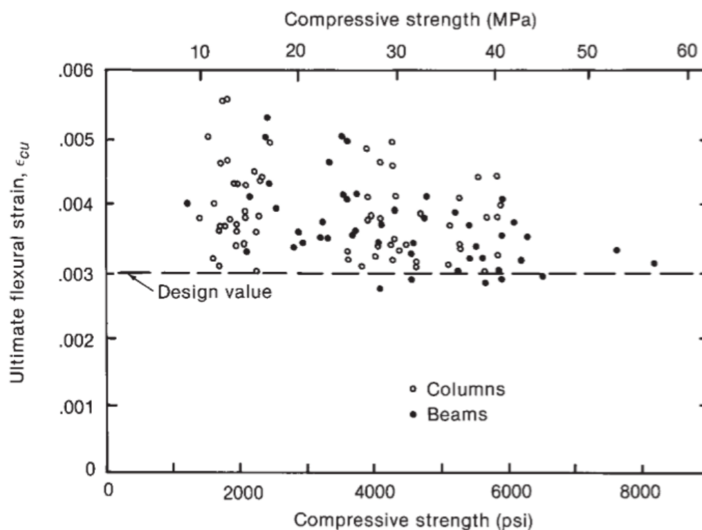
Figure 4.1. Concrete compressive strain limit for reinforced concrete members (Mattock et al., 1961)
