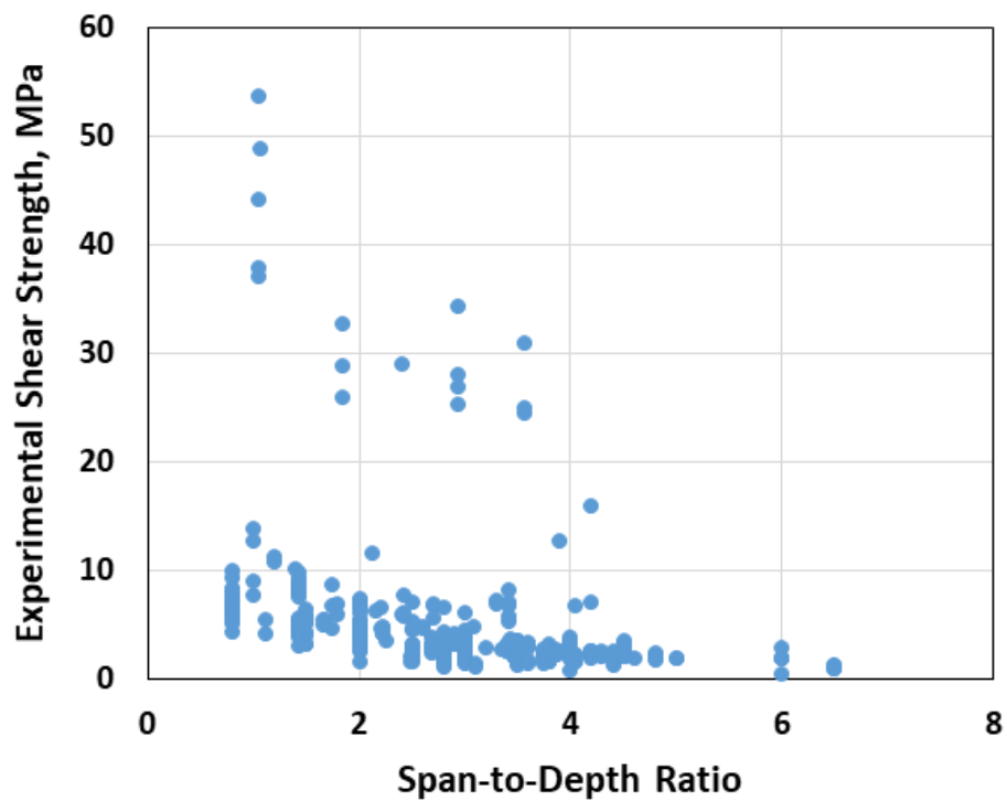
Figure 4.8. Influence of the shear span-to-depth ratio on shear strength of FRC beams
