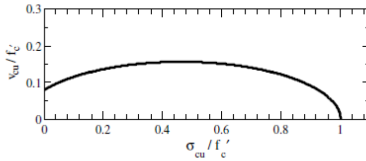
Figure 2.12. Bresler and Pister's failure criterion for concrete subjected to combined compression and shear stresses.
