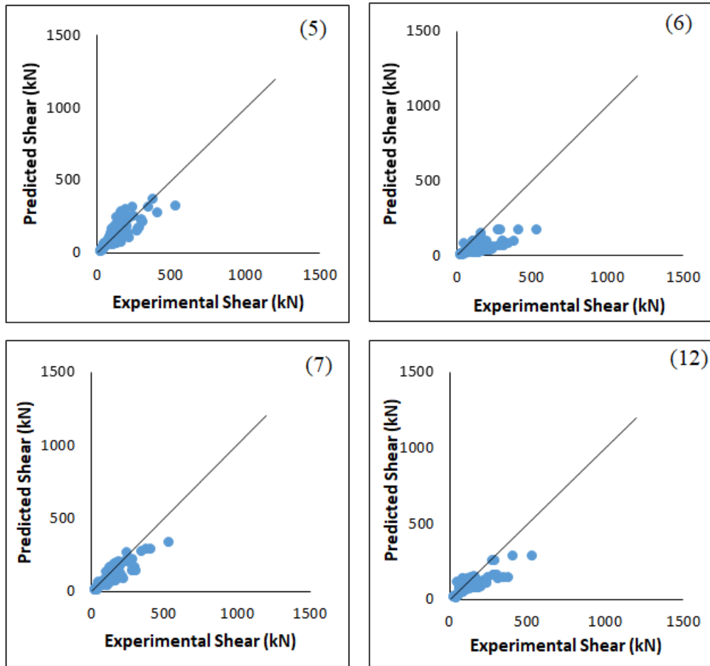
Figure 4.10. Shear strength predictions for Deep Beams ( a/d \leq 2.5 ) without transverse reinforcement (continued):
