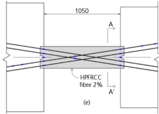
Figure 5.34. Reinforcement detailing of Specimen FC-0.0-3.5
