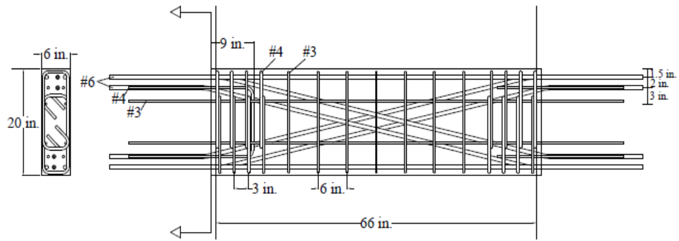
Figure 5.12. Reinforcement detailing of Specimen CB-3
