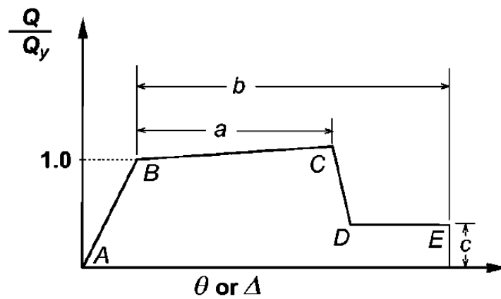
Figure 5.3. Generalized force versus deformation curve (ASCE 41, 2013)
