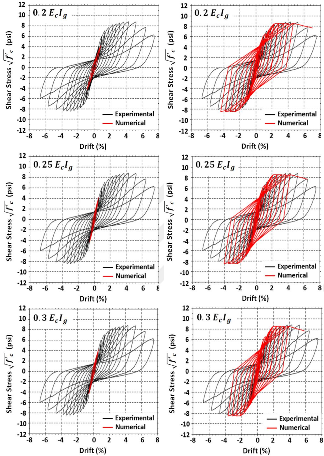
Figure 5.7. Shear stress vs. drift response for Specimen CB-6 (Setkit, 2012)
