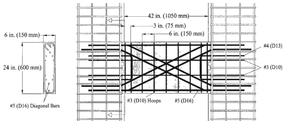
Figure 5.18. Reinforcement detailing of Specimen CB-1
