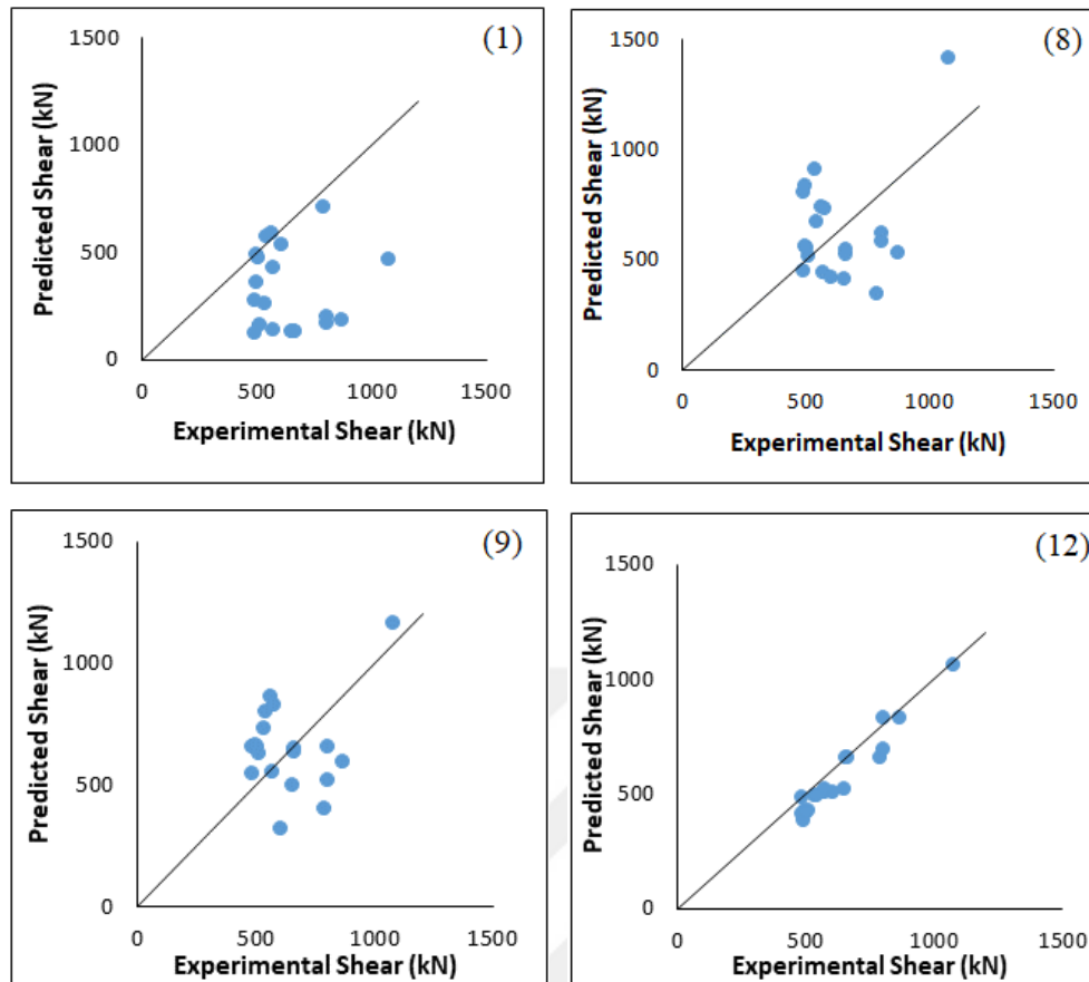
Figure 4.15. Shear strength predictions for HPFRC Coupling Beams with transverse reinforcement: (1) ACI 318-14 (2014); (8) Canbolat (2004); (9) Lequesne (2011); (12) Proposed method
