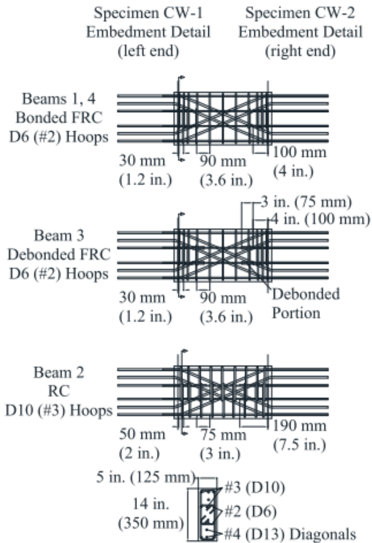
Figure 5.55. Coupling beam reinforcement detailing for CW-1 and CW-2
