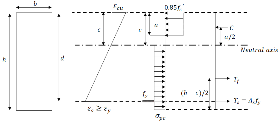
Figure 4.2. Considered stress distribution and equivalent forces for rectangular single reinforced section
