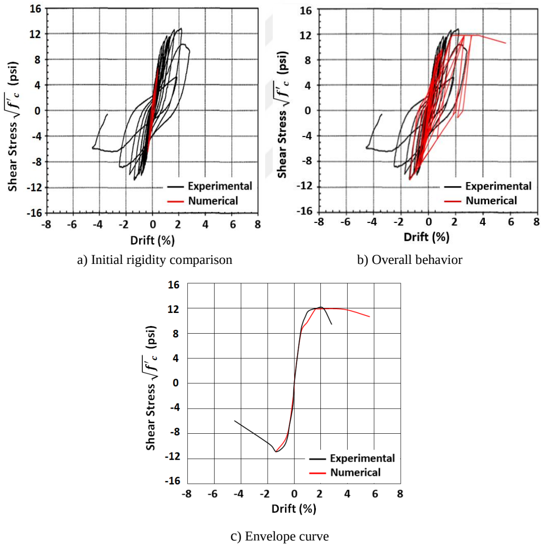
Figure 5.19. Shear stress vs. drift response of Specimen CB-1
