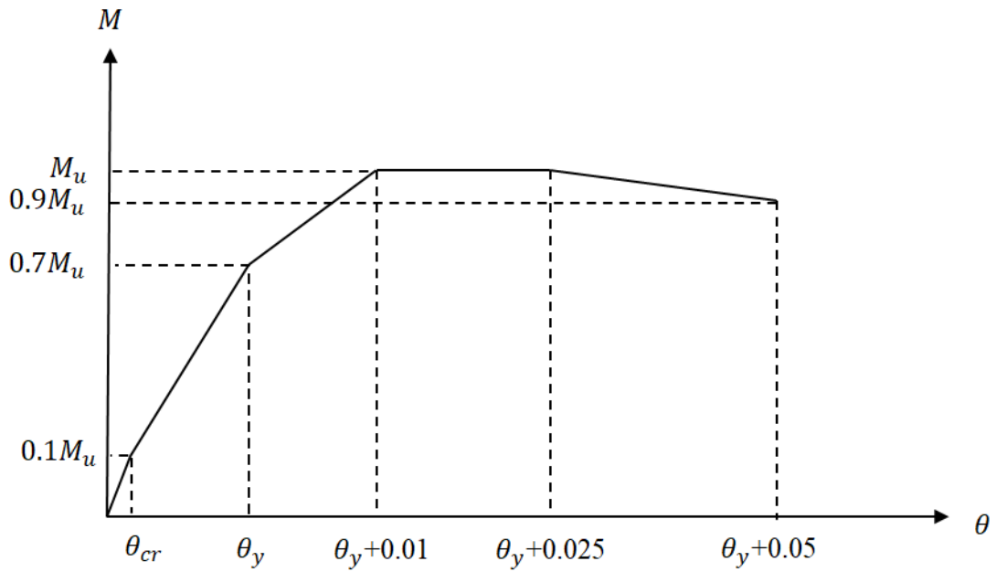
a) Moment-rotation relationship for CCBs.
