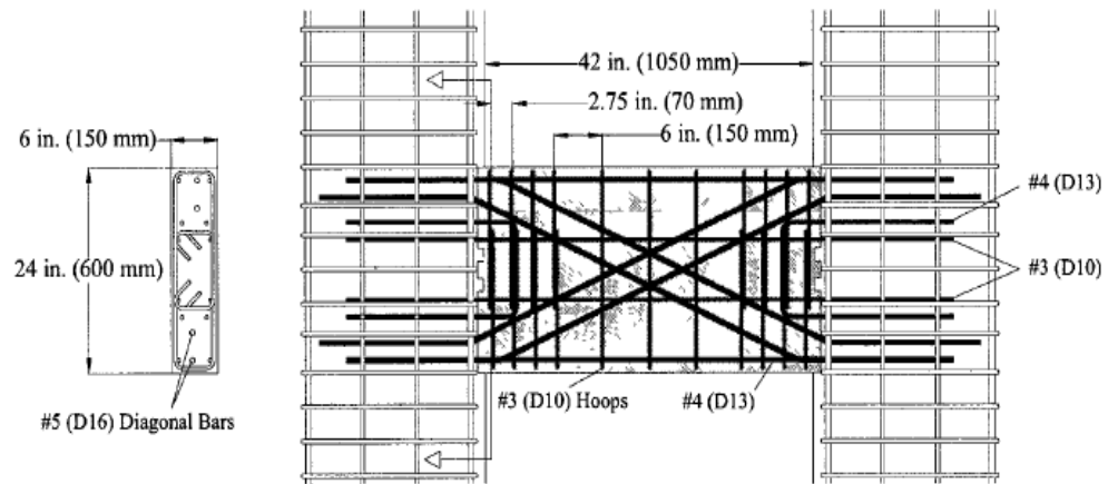
Figure 5.20. Reinforcement detailing of Specimen CB-2
