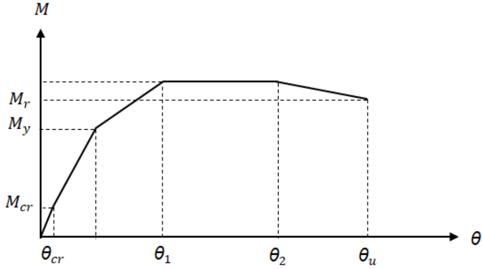
Figure 5.4. Moment-rotation backbone curve for beams
