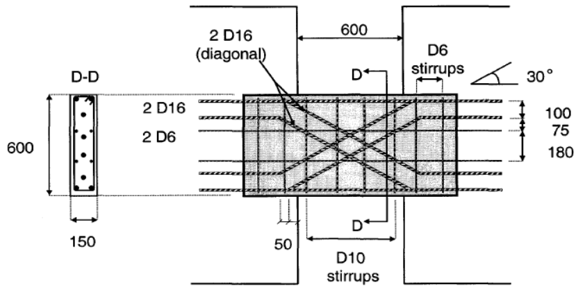
Figure 5.28. Reinforcement detailing of Specimen 4
