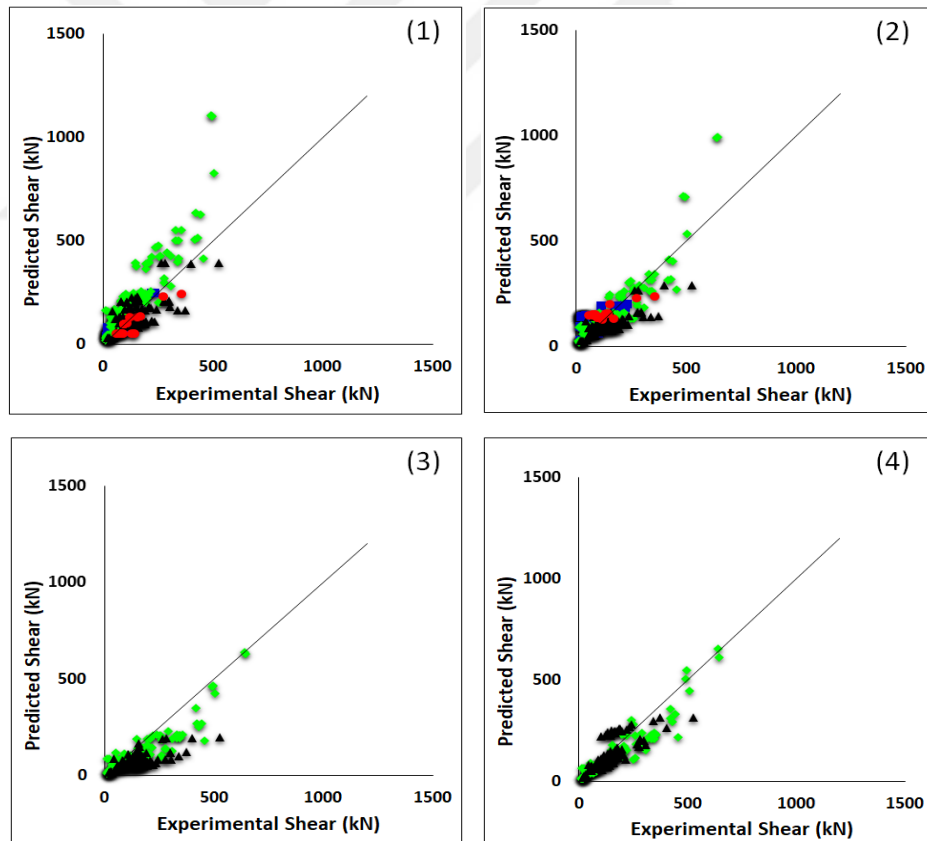
Figure 4.17. Shear strength predictions for Deep Beams:
