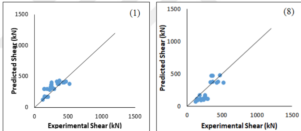
Figure 4.13. Shear strength predictions for FRC Coupling Beams with transverse reinforcement: (1) ACI 318-14 (2014); (8) Canbolat (2004)
