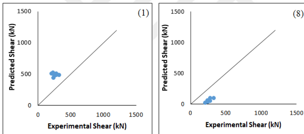
Figure 4.14. Shear strength predictions for FRC Coupling Beams without transverse reinforcement:
