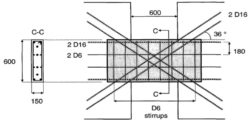
Figure 5.26. Reinforcement detailing of Specimen 3
