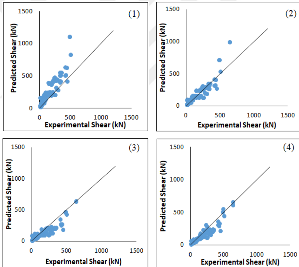
Figure 4.12. Shear strength predictions for Deep Beams ( a/d > 2.5 ) without transverse reinforcement: (1) ACI 318-14 (2014); (2) Sharma (1986); (3) Mansur et al. (1986); (4) Narayanan and Darwish (1987)
