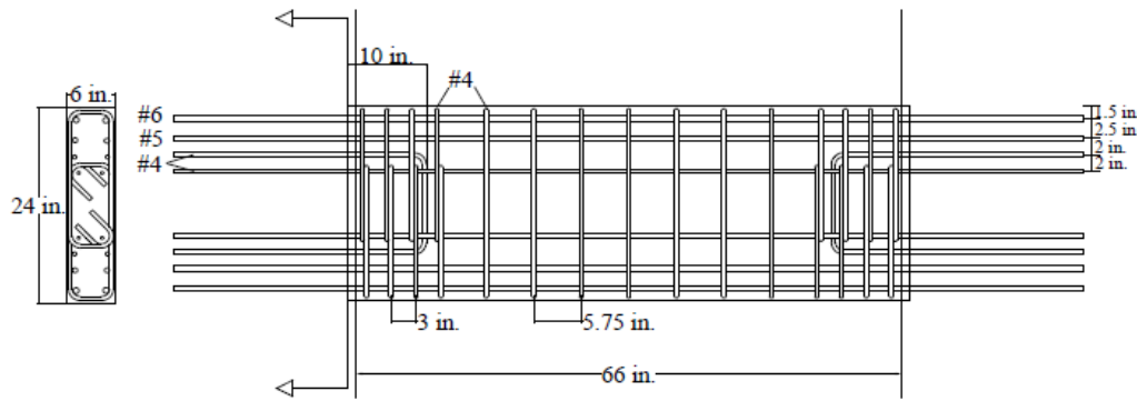
Figure 5.16. Reinforcement detailing of Specimen CB-6
