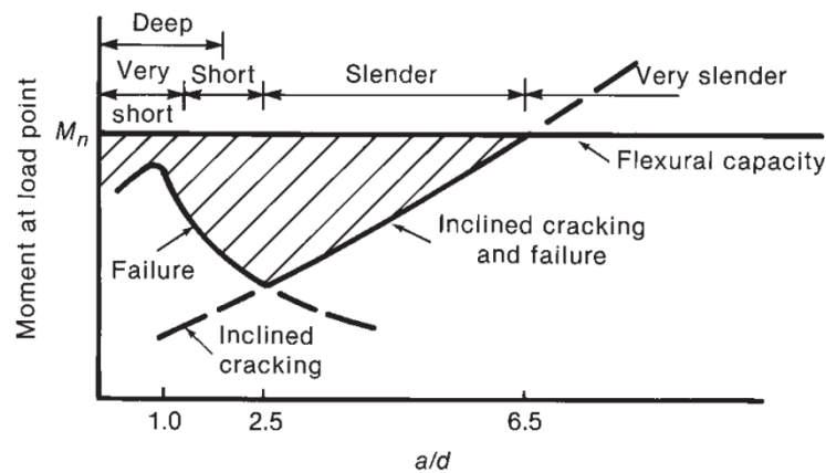
Figure 2.3. Moment capacity based on a/d ratio (Wight and MacGregor, 2016)
