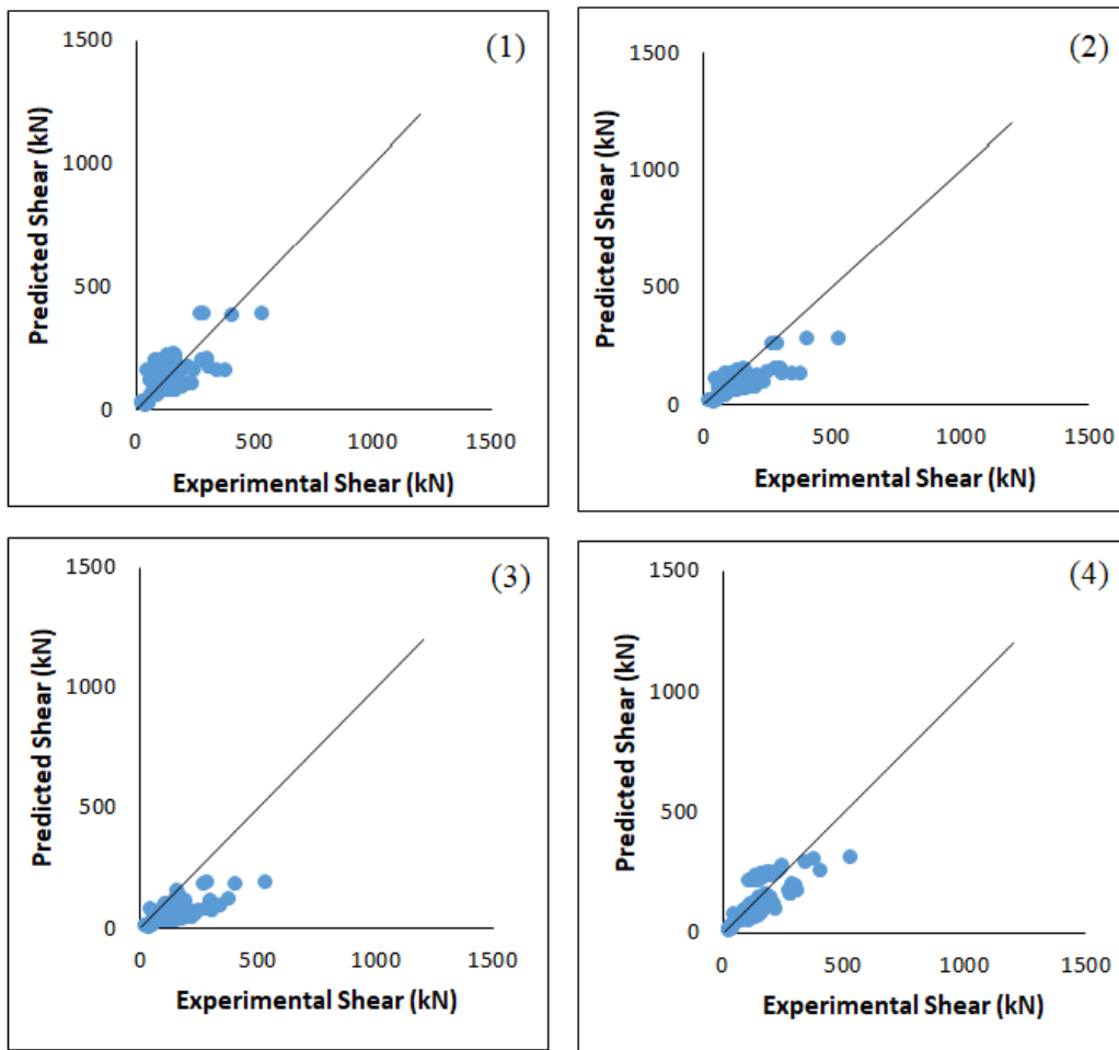
Figure 4.10. Shear strength predictions for Deep Beams ( a/d \leq 2.5 ) without transverse reinforcement:
