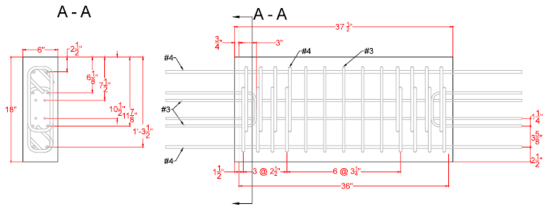
Figure 5.51. Reinforcement detailing of Specimen CB8
