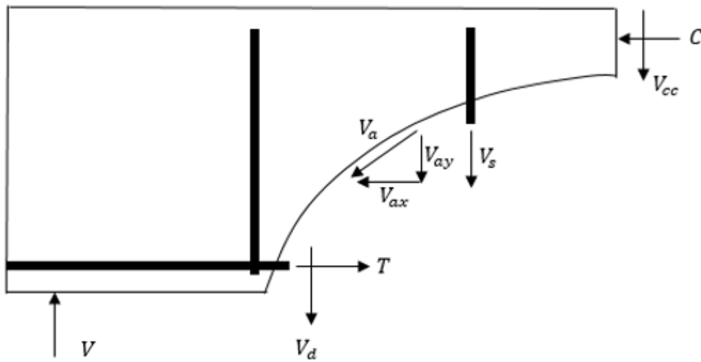
Figure 2.8. Shear resisting forces in a beam with transverse reinforcement
