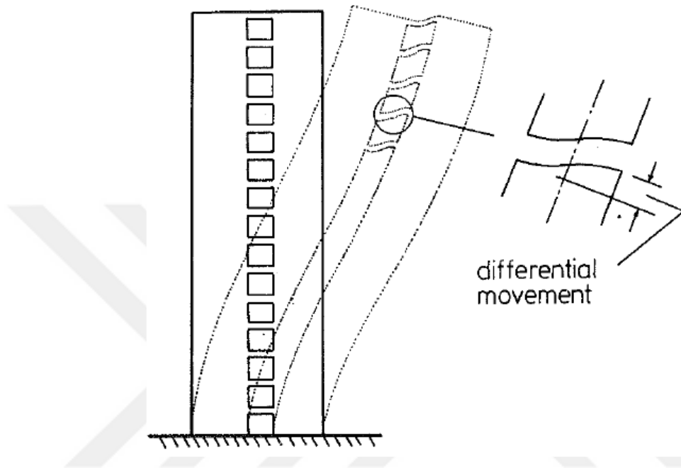
Figure 2.4. Differential movement of coupling beam (Subedi, 1991)
