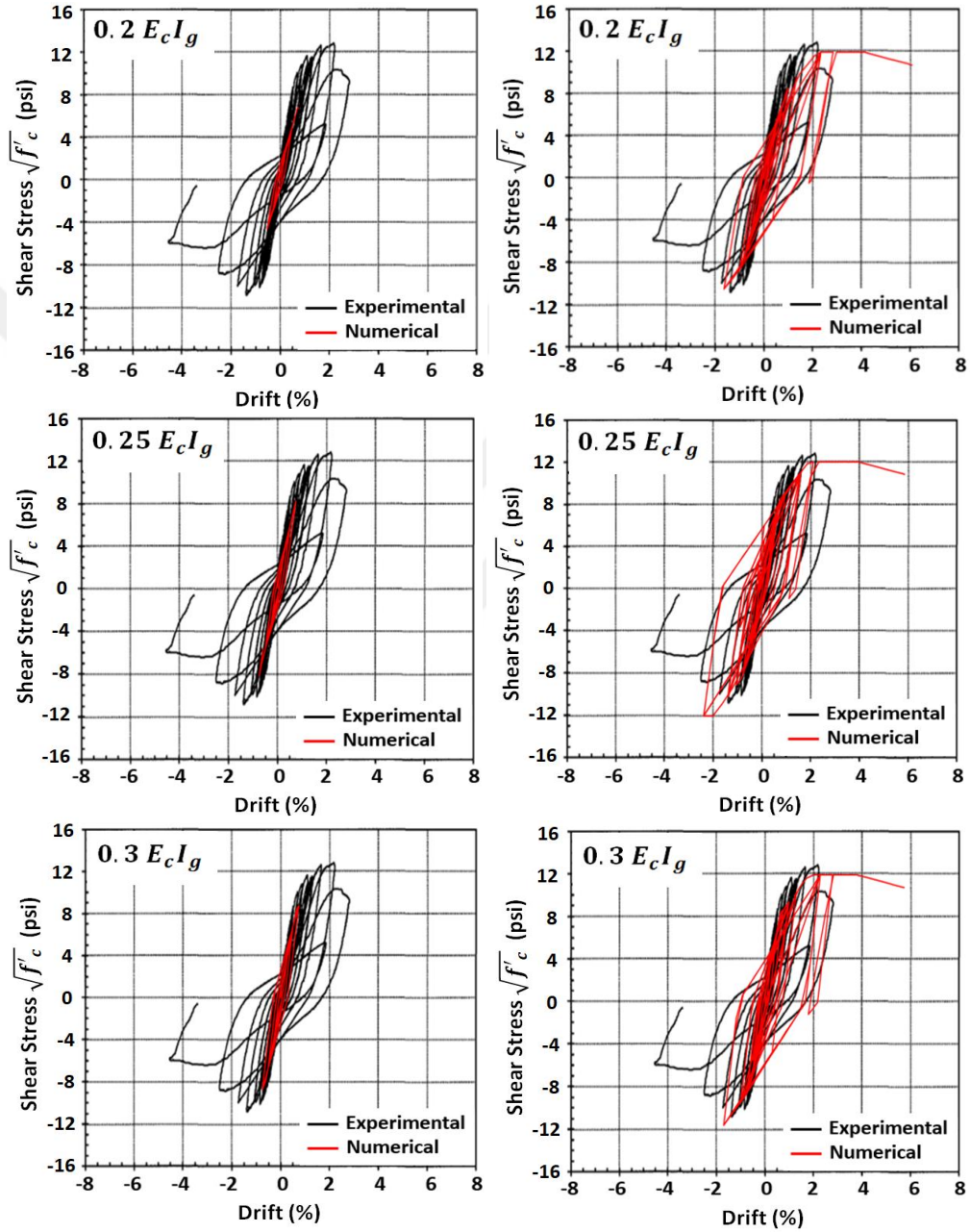
Figure 5.6. Shear stress vs. drift response for Specimen CB-1 (Lequesne, 2011)
