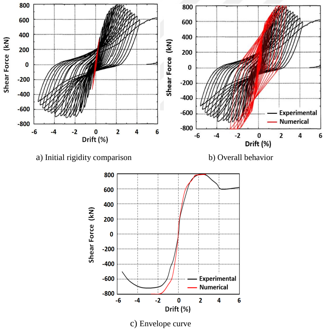
Figure 5.29. Shear stress vs. drift response of Specimen 4
