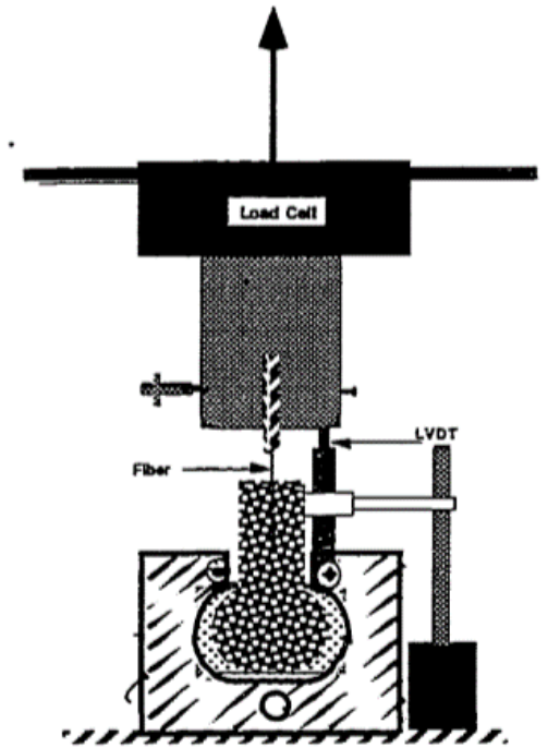
Figure 4.3. Single fiber pull-out test setup (Guerrero, 1999)
