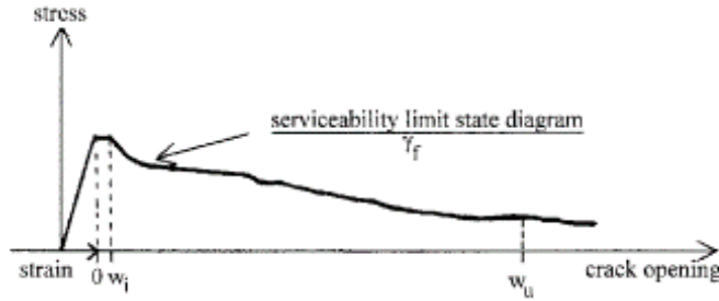
Figure 2.11. Characteristic stress-strain relationship (Casanova and Rossi, 1997)
