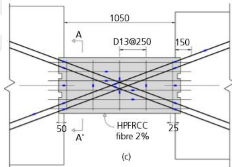
Figure 5.30. Reinforcement detailing of Specimen FC-0.5-2.0
