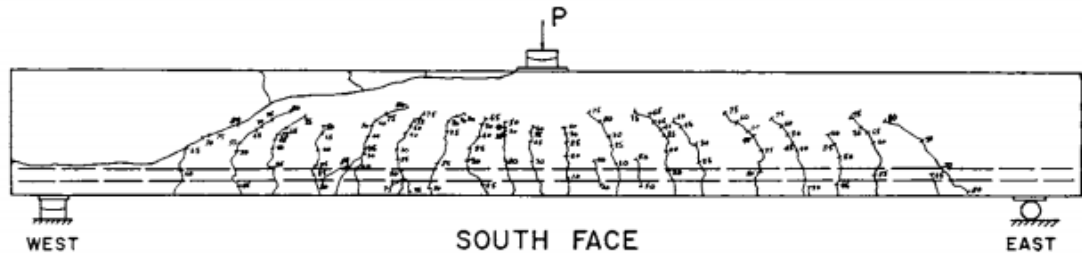
Figure 2.7. Typical crack pattern for a simply-supported reinforced concrete beam (Bresler and Scordelis, 1963)
