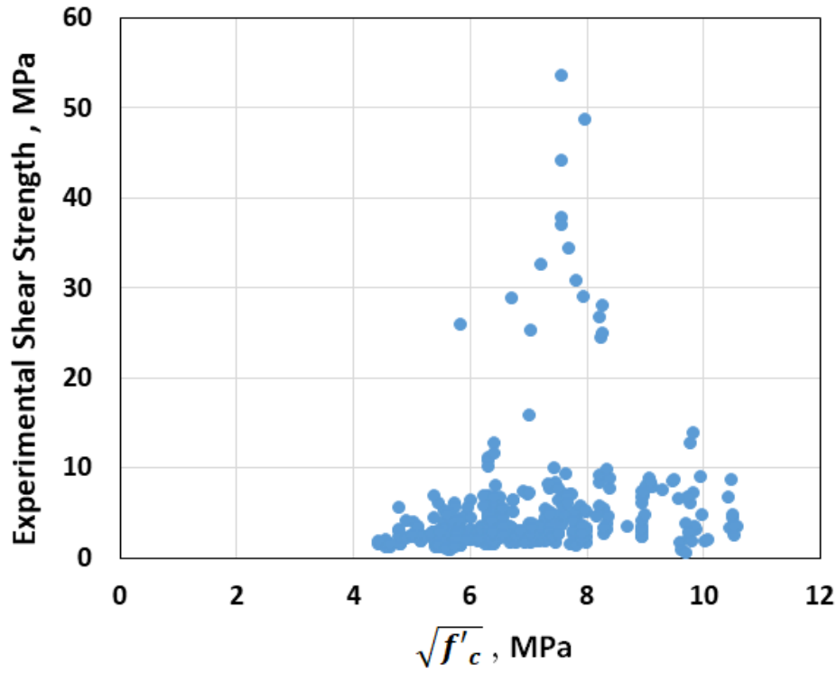
Figure 4.5. Influence of \sqrt{f'_c} on shear strength of FRC beams
