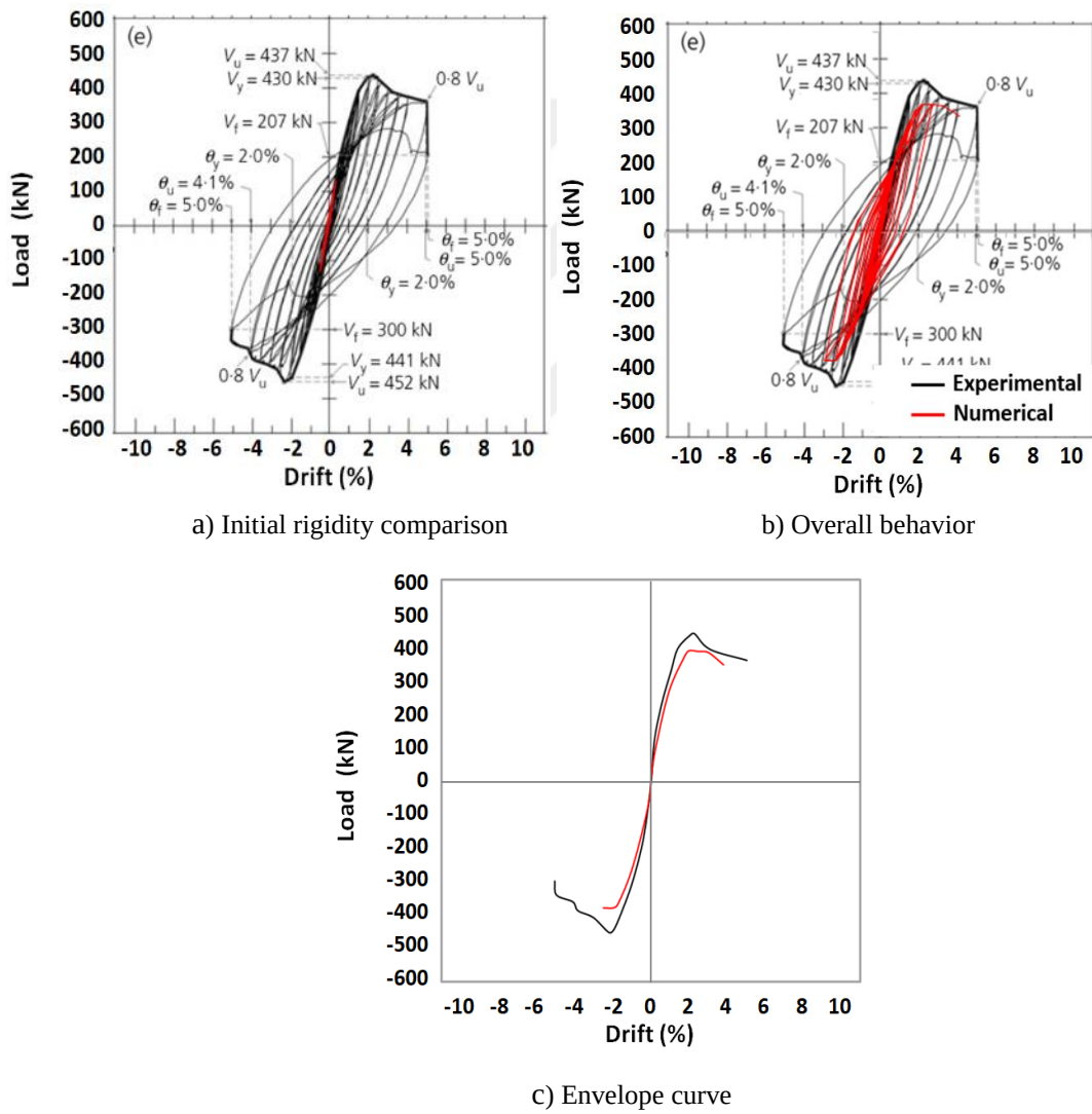
Figure 5.35. Shear stress vs. drift response of Specimen FC-0.0-3.5
