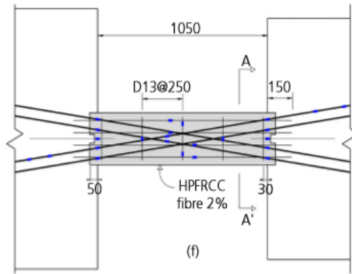
Figure 5.32. Reinforcement detailing of Specimen FC-0.5-3.5
