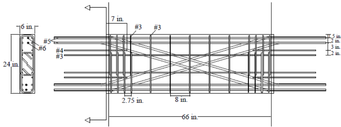
Figure 5.8. Reinforcement detailing of Specimen CB-1
