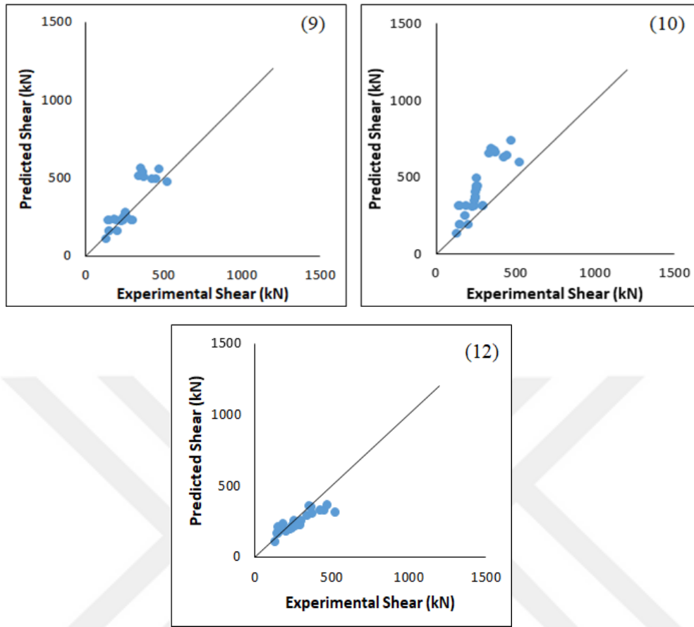
Figure 4.13. Shear strength predictions for FRC Coupling Beams with transverse reinforcement (continued):
