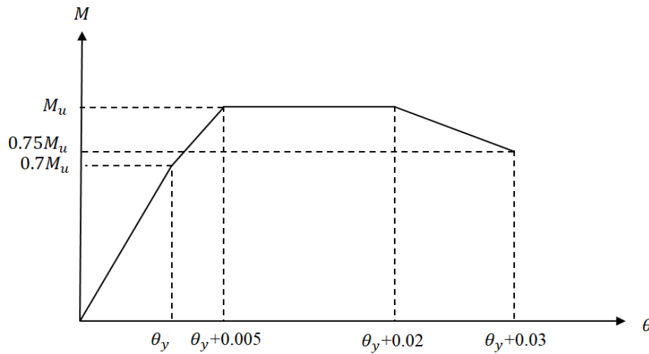
(a) Moment-rotation relationship
