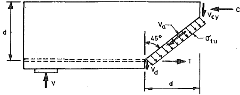
Figure 2.9. Forces through a diagonal crack of a FRC beam without transverse reinforcement (Mansur et al., 1986)
