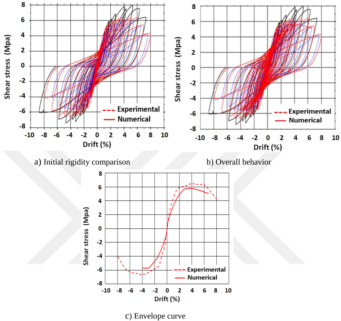
Figure 5.48. Shear stress vs. drift response of Specimen 3 (Aspect ratio = 3.3)
