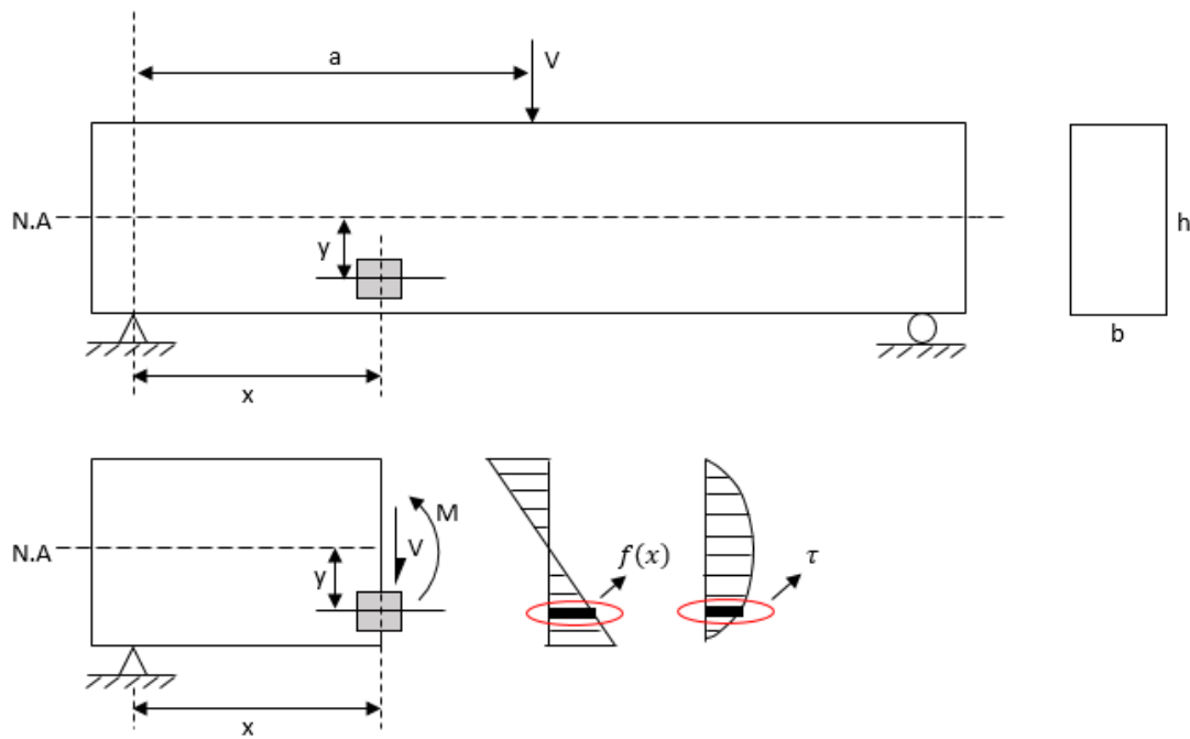
Figure 2.6. Shear and flexural stresses for plain concrete beam subjected to a concentrated load.
