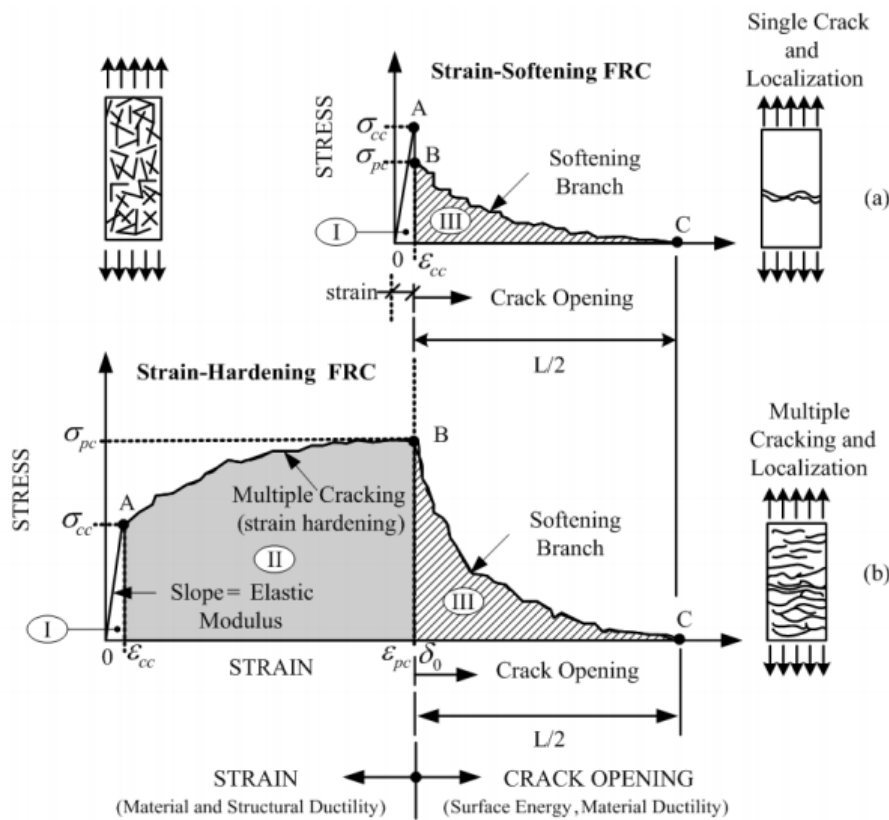
Figure 2.1. Tensile stress-strain relationship for FRC and HPFRC members (Naaman and Reinhardt, 1996).
