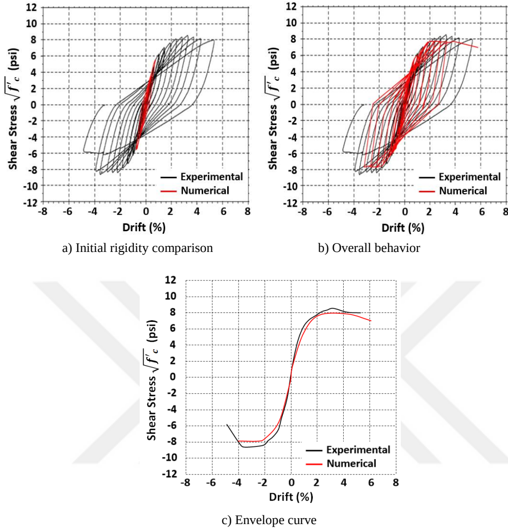
Figure 5.11. Shear stress vs. drift response of Specimen CB-2
