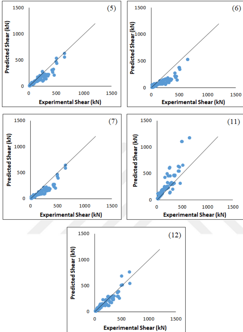
Figure 4.12. Shear strength predictions for Deep Beams ( a/d > 2.5 ) without transverse reinforcement (continued):
