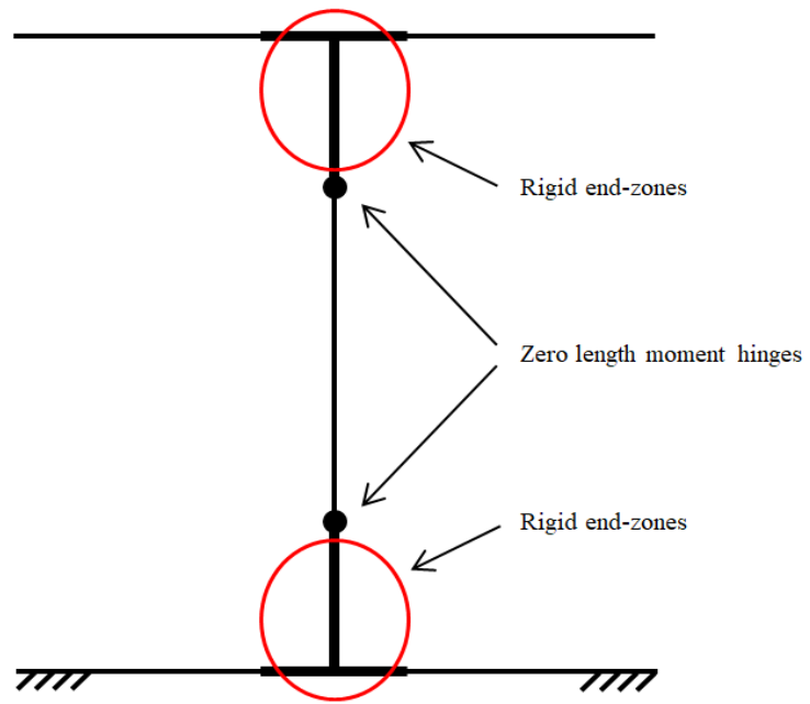
a) Specimen model when there are no arms holding the ends of the top wall segment
