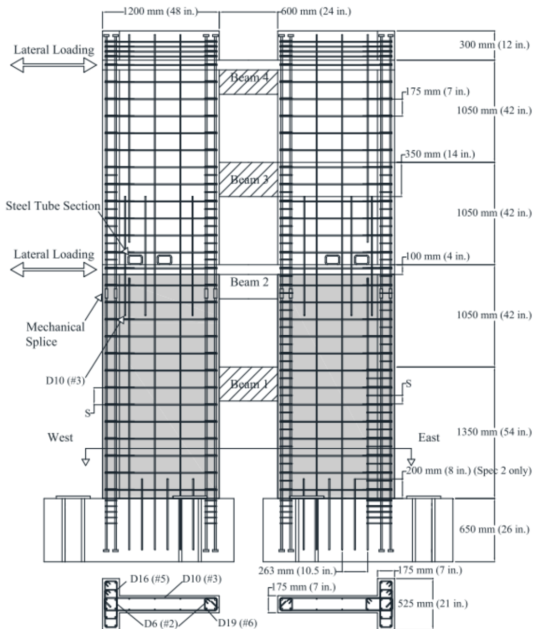
Figure 5.53. Coupled wall system
