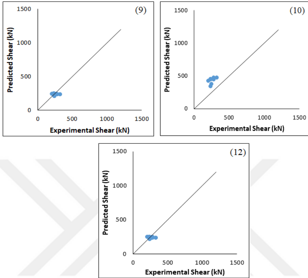
Figure 4.14. Shear strength predictions for FRC Coupling Beams without transverse reinforcement (continued):
