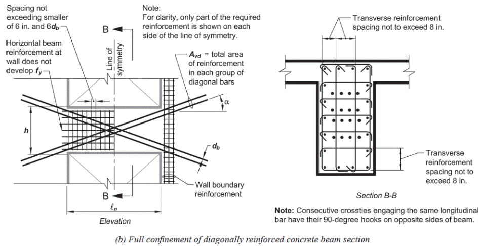
Figure 2.5. Reinforcement detailing of diagonally reinforced coupling beams (ACI 318-14)
