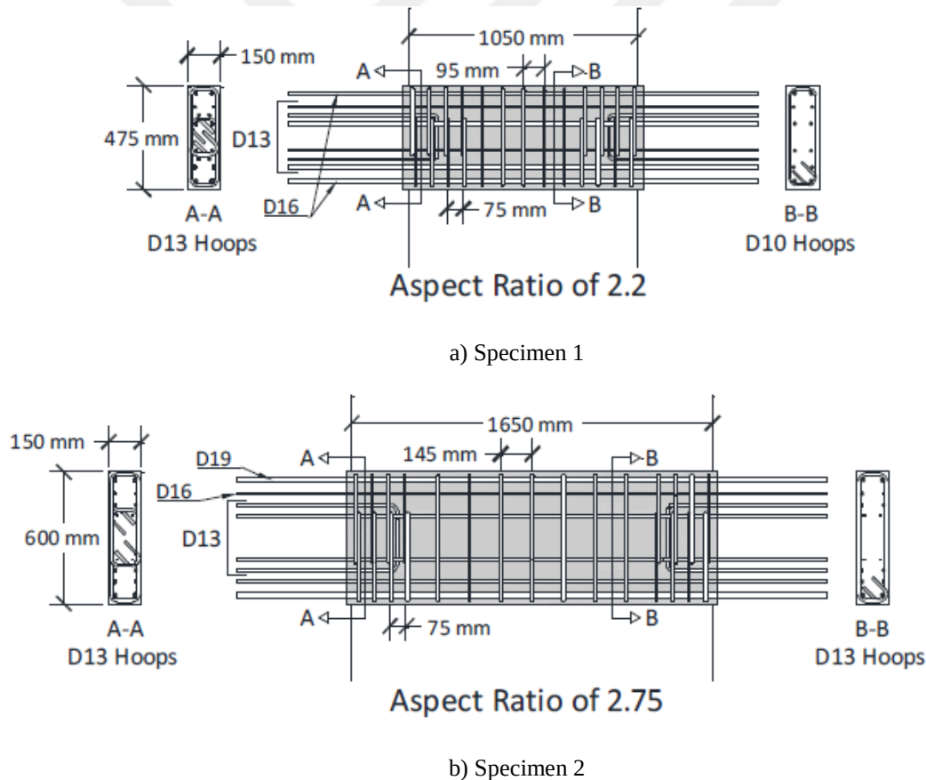
Figure 5.44. Reinforcement detailing of Specimens
