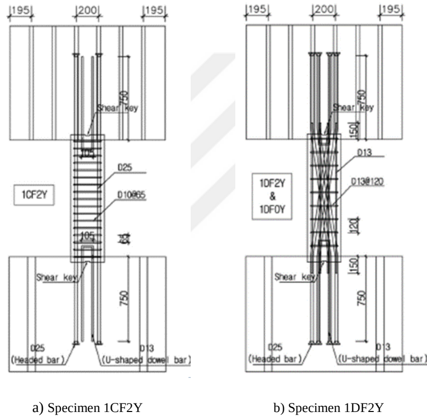
Figure 5.36. Reinforcement detailing of Specimens
