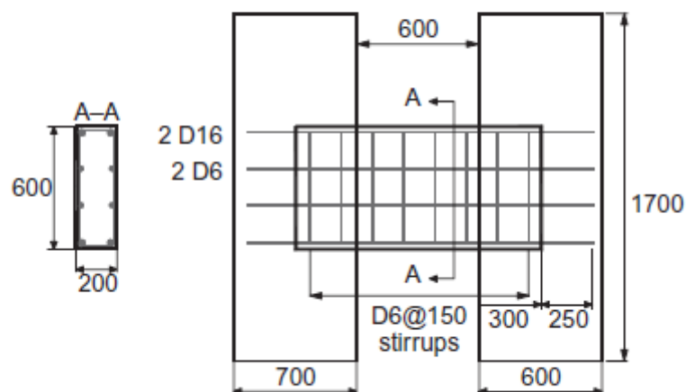
Figure 5.39. Reinforcement detailing of (a) Specimen CB2 and (b) Specimen CB3
