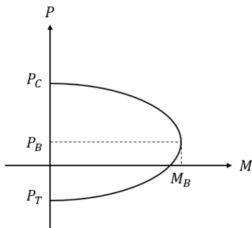
(b) Axial load-moment relationship
