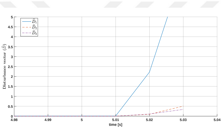
Figure 4.8: Elements of the disturbance vector during the occurrence of the fault
