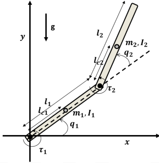
Figure 3.5: Vertical two-link robot manipulator system
