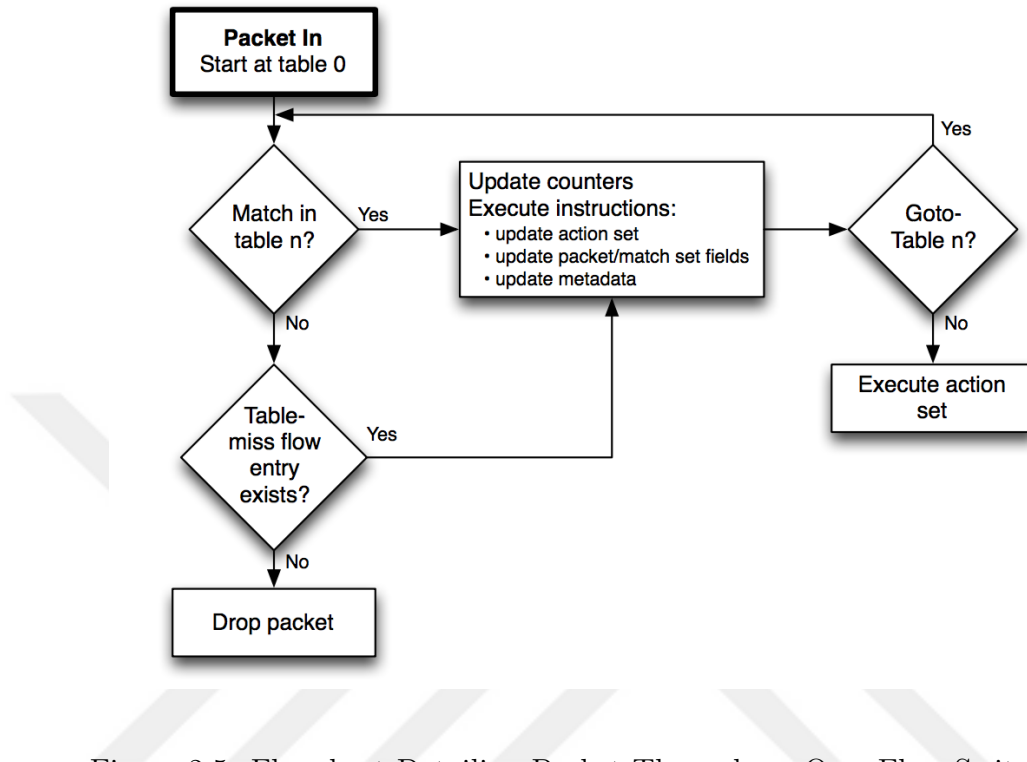
Figure 2.5. Flowchart Detailing Packet Through an OpenFlow Switch [1]
