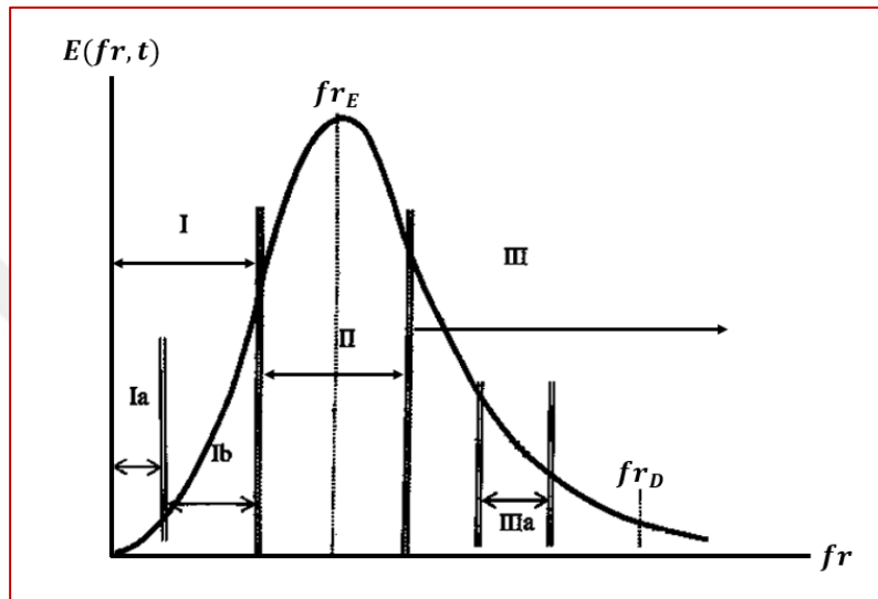
Figure 2.2 Three-dimensional energy spectrum with critical regions [7]
