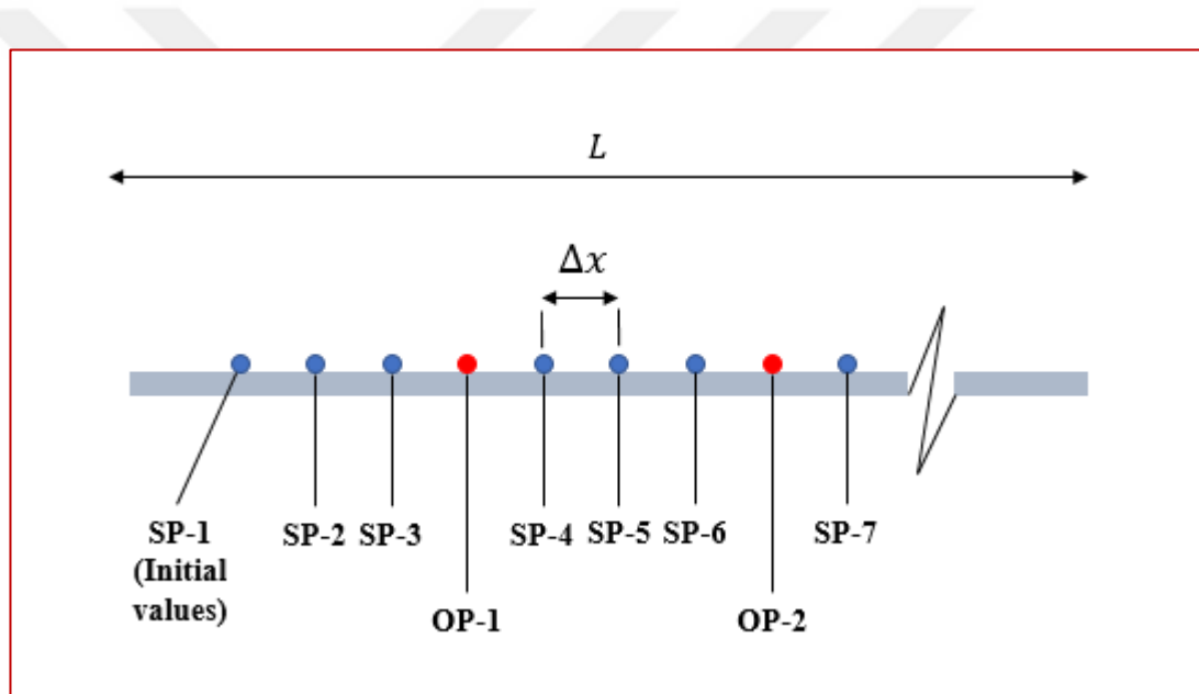
Figure 2.8 Grid length ( \Delta x ), solution-points (SPs), output-points (OPs), length of the plate's portion interested in fully-turbulent flow ( L )
