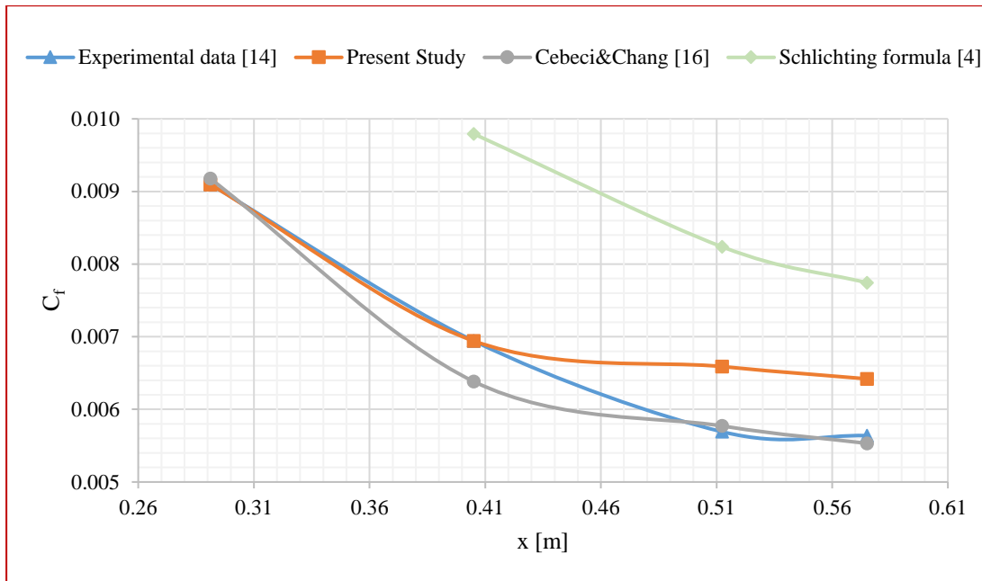
Figure 3.2 Results of Arndt and Ippen's experiment: U_E=12.27 m/s, k_s=0.7010 mm, \nu=8.83 \times 10^{-7} m 2 /s, Re=8.47 \times 10^6
