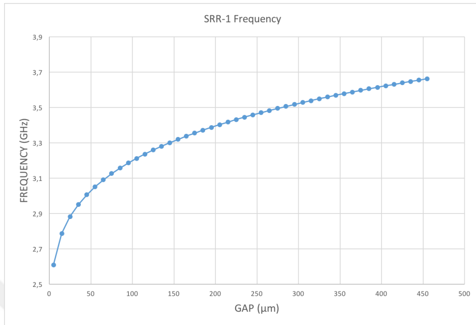
Figure 2.18. Resonance frequency - single gap.
