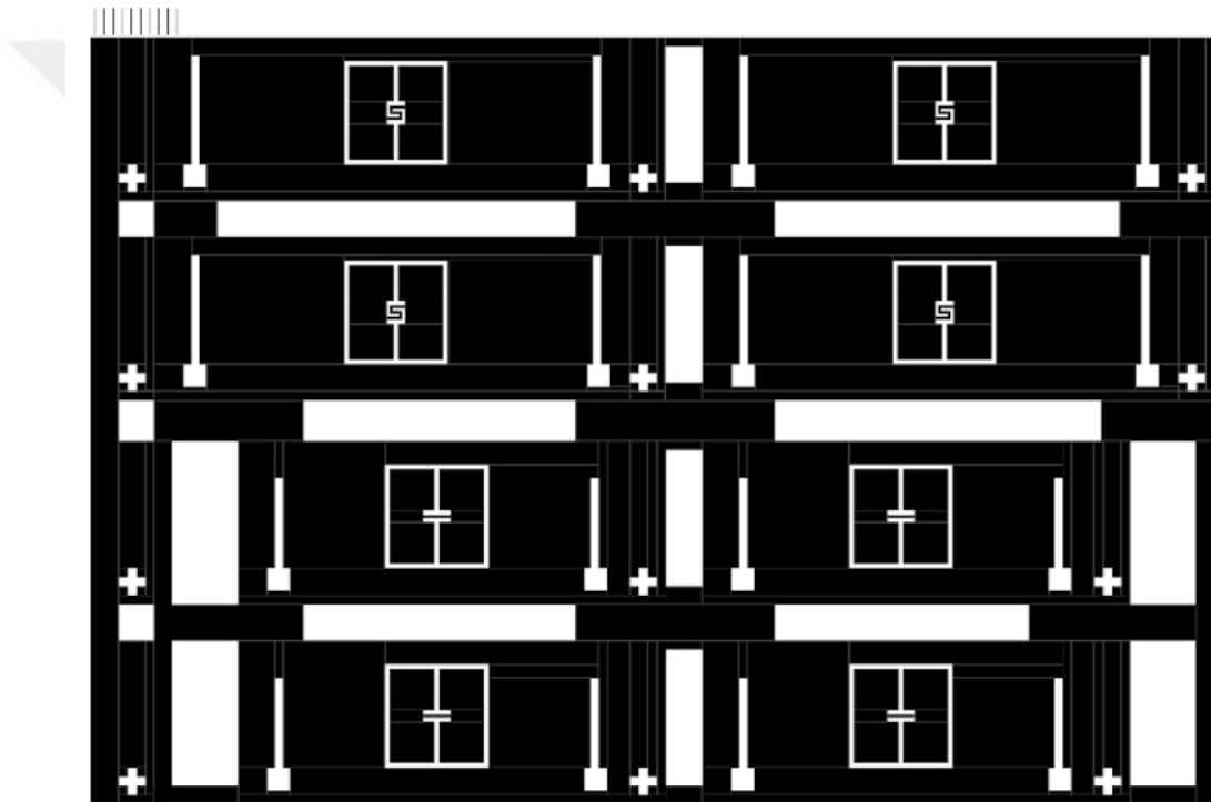
Figure 3.4. 2^{nd} bunch - mask for the first photolithography step.
