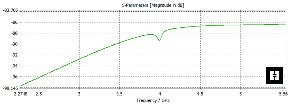
Figure 2.26. S21 of single gap steel resonator-1.
