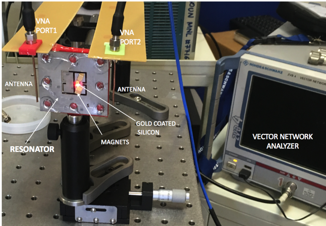
Figure 4.4. Measurement setup-2.
