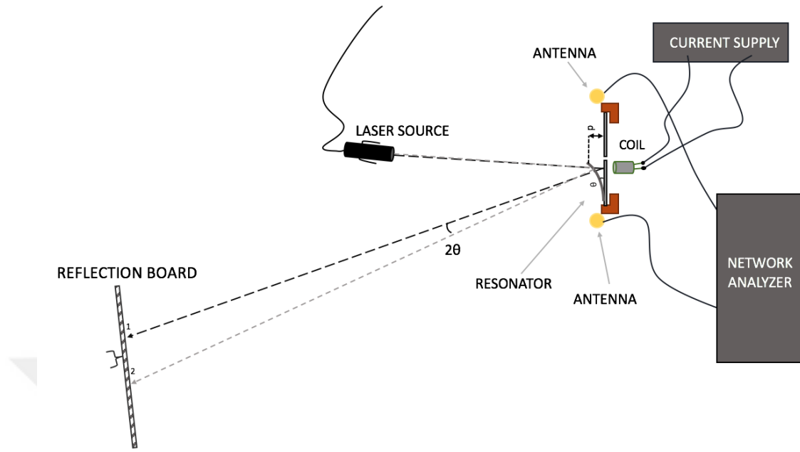
Figure 4.1. Representative measurement setup.
