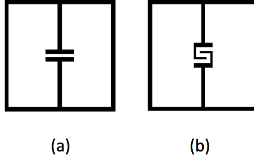
Figure 2.3. The two designed resonator structures. (a) single gap split ring resonator. (b) nested gap split ring resonator.
