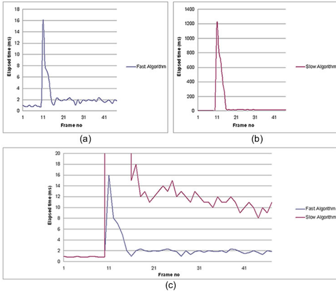
Figure 6.7: Calculation times for the breaking cube animation (a) Fast Algorithm (b) Slow Algorithm (c) A close-up of the chart for both algorithms
