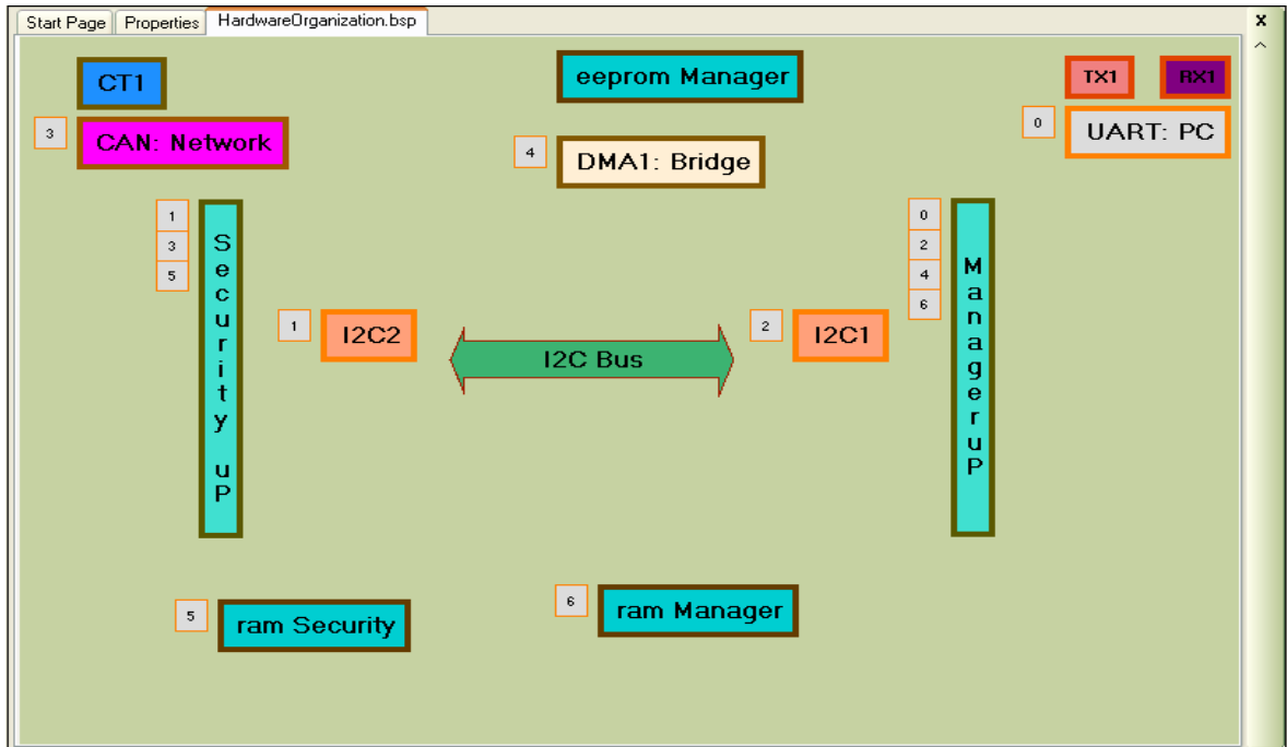
Figure 5.2. Hardware organization
