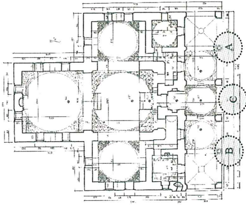
Plan 4.6 Muradiye Cami Plan (Aslanapa, 1987)
