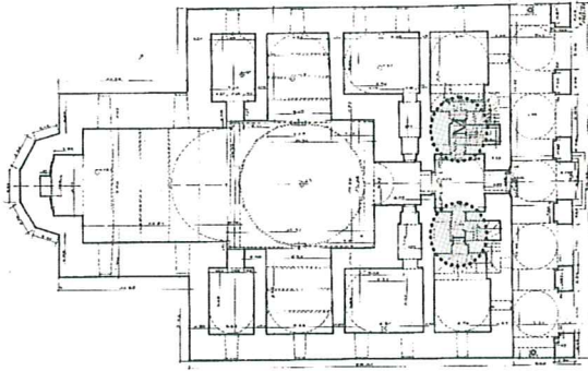
Plan 4.9 Hüdavendigâr Cami Alt Kat Plan (Ayverdi, 1989)
