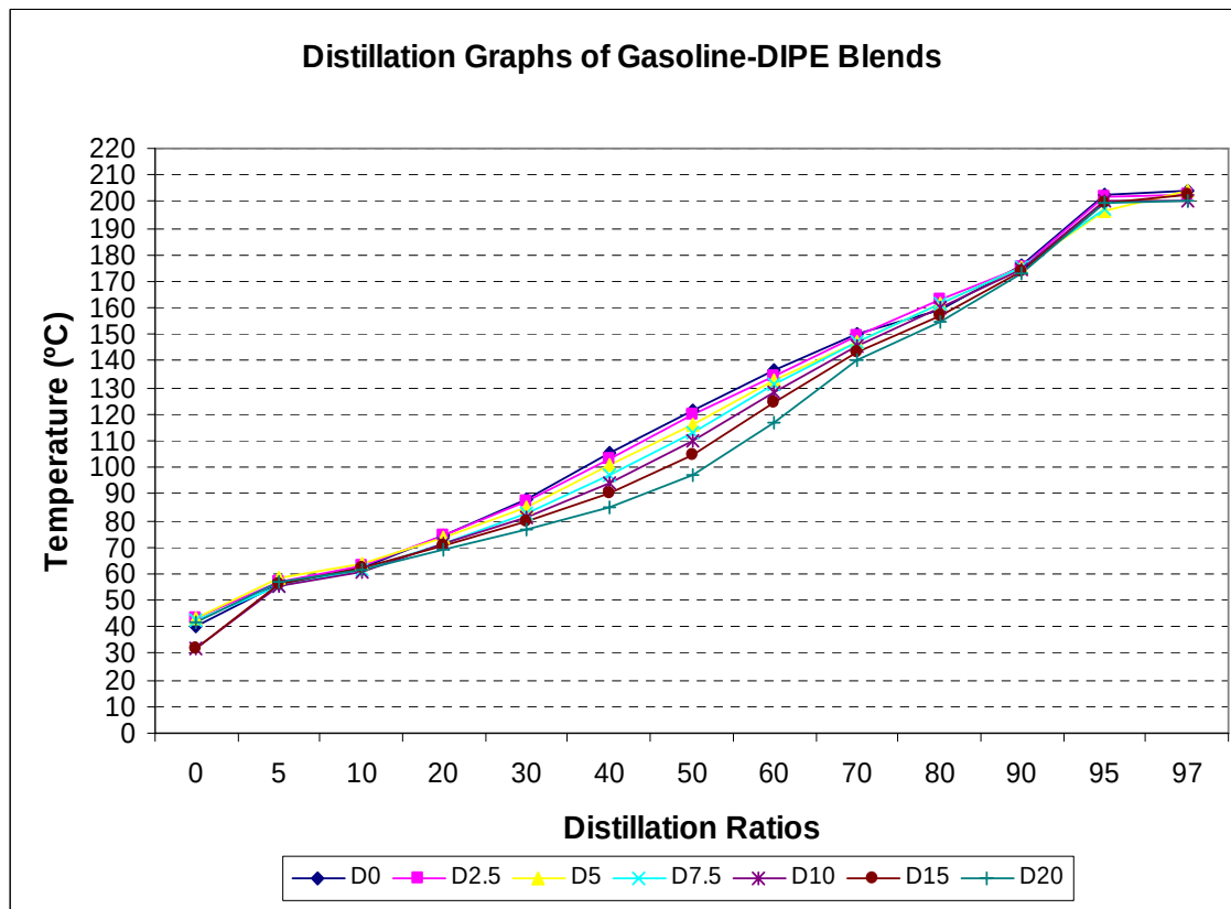
Figure 5.42. Distillation Graphs of Gasoline-DIPE Blends.
