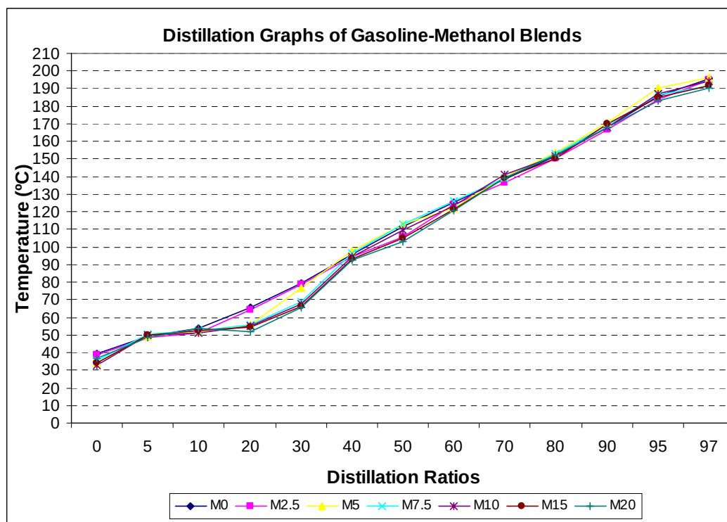
Figure 5.14. Distillation Graphs of Gasoline Methanol Blends.
