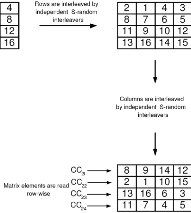
Figure 3.7: Firstly the rows are interleaved, then the columns [10].
