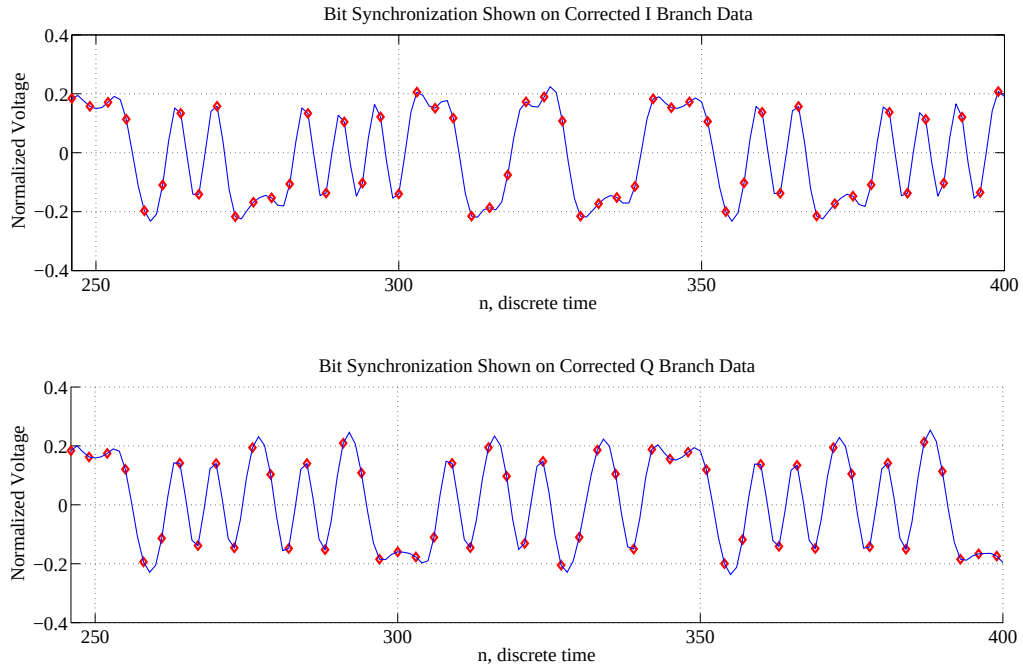
Figure 2.20: Diamonds represent the optimal sampling points obtained by the testbed.
