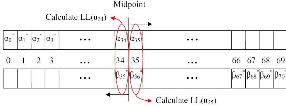
Figure 3.13: At time 35, first LL values are ready to be calculated.
