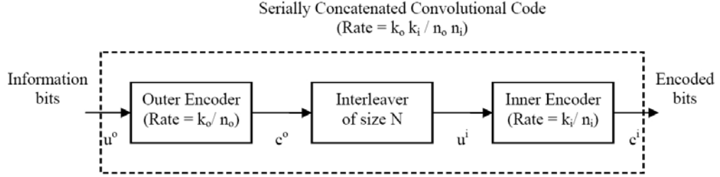
Figure 3.4: Structure of a serially concatenated convolutional code.
