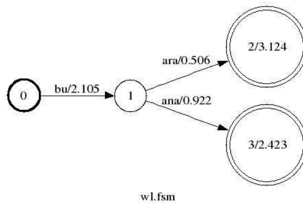
Figure 3.1. Word-based Lattice
