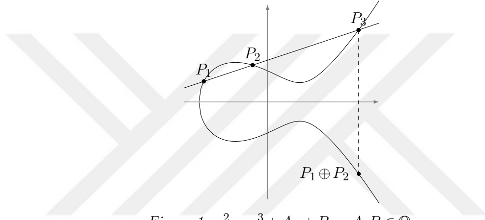
Figure 1: y^2 = x^3 + Ax + B , A, B \in \mathbb{Q} .
