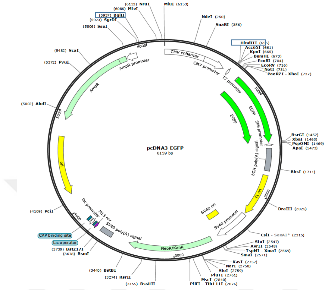
Figure 16. Structure of pcDNA3-EGFP plasmid. To investigate the effect of VSTM5 gene expression on the cell growth rate, we planned to clone the VSTM5 gene into the HCT116 cell line. To achieve this, we prepared the pcDNA3-EGFP.VSTM5 construct using BglIII and HindIII double digestion.
