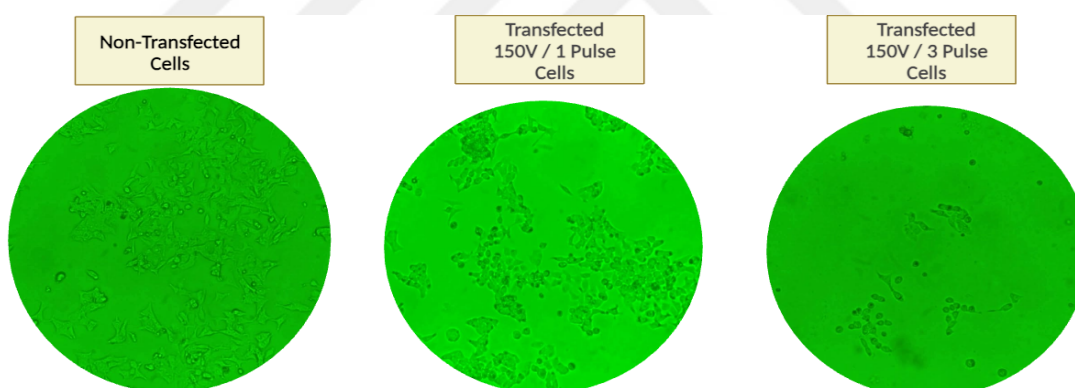
Figure 21. Fluorescence Microscopy Images. Fluorescence microscopy images were captured at 40X magnification, showcasing non-transfected cells, 150 Volt 1 pulse transfected cells, and 150 Volt 3 pulse transfected cells.
