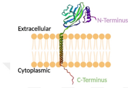
Figure 8. The membrane topology of VSTM5. The N-terminus is represented by purple, while the transmembrane region is indicated by the helix structure. The C-terminus is depicted in red.
