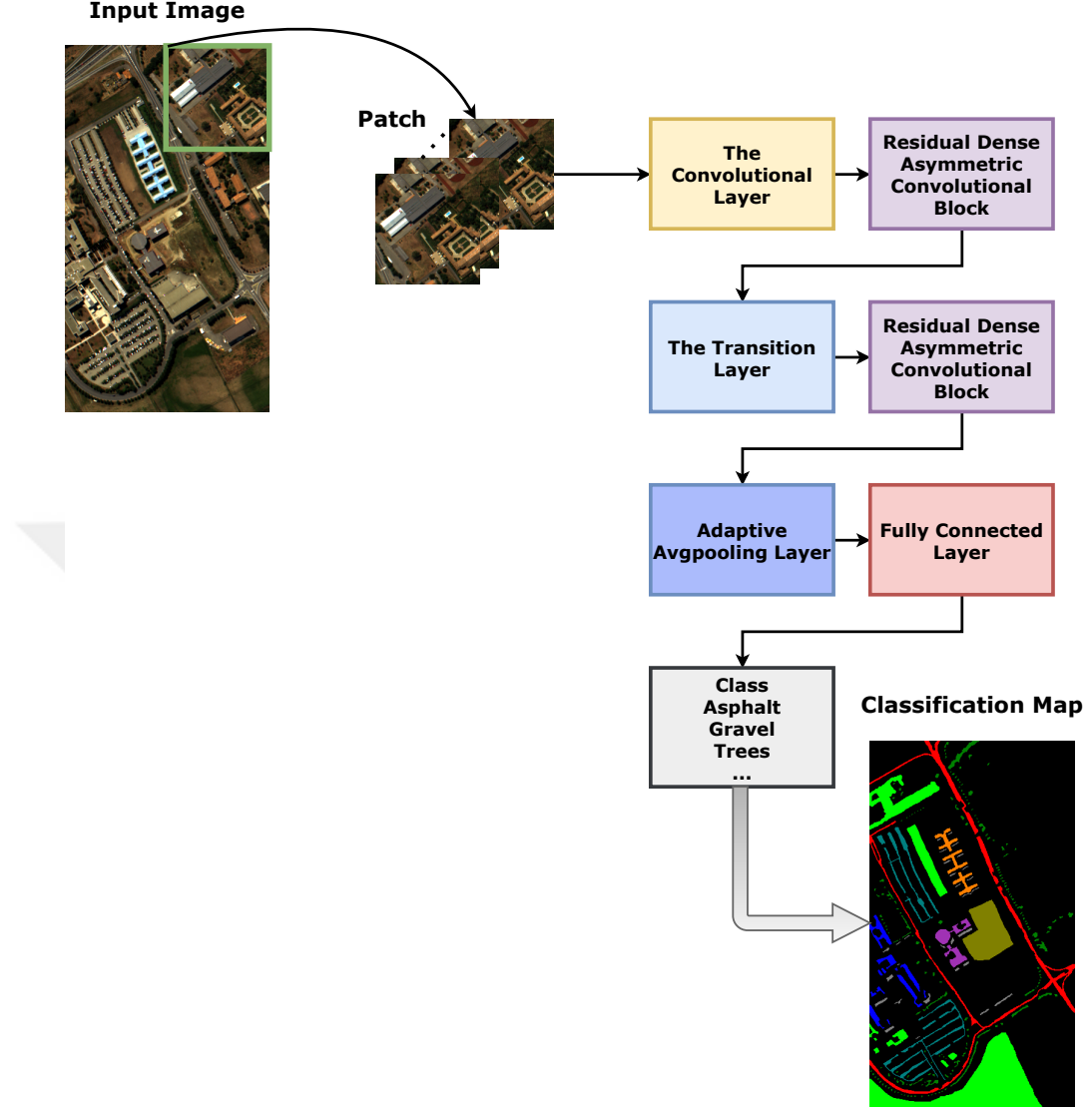
Figure 3.1 Residual Dense Asymmetric Convolutional Network Framework
