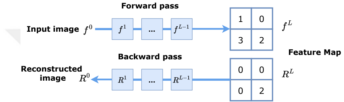
Figure 3.4 The visualization of higher layer neuron activations. Forward pass is performed to a layer when an input image is given. Then all of the activations are zeroed out except one, and this signal is propagated back to to obtain a reconstructed image R^0
