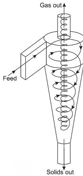
Figure 1.2 Preheater cyclone
