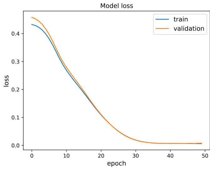
(a) Single-shot learning curve
