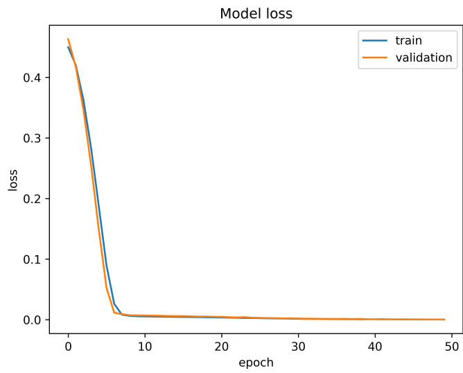
(b) Encoder-Decoder RNN learning curve
