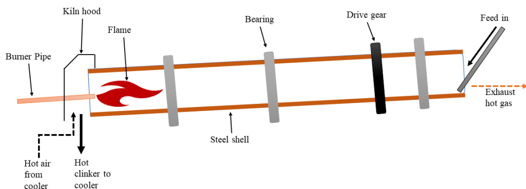
Figure 1.3 Rotary kiln
