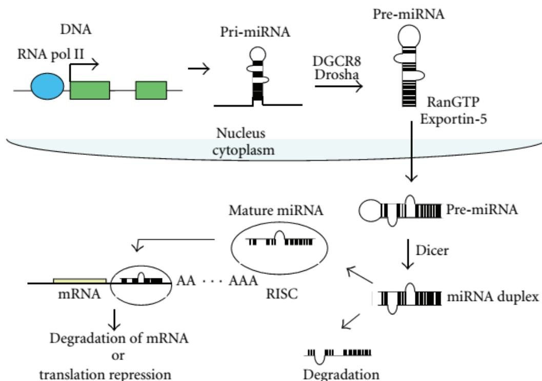
Figure 1.13 : MicroRNA biogenesis [40].
