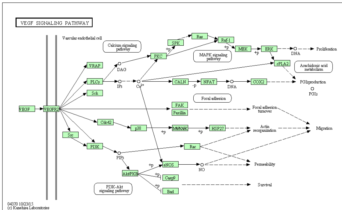
Figure 1.12 : VEGFR2 signalling [110].
