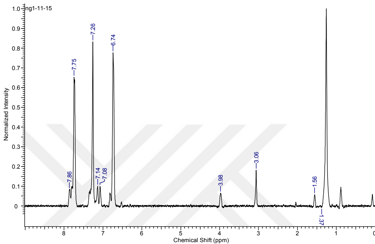
EK 2- 4-(4H-ditiyol [3,2-b:2',3'-d]pirol-4-il)anilin (N-Ph-NH 2 monomerinin) anilin 400 MHz 1 H-NMR spektrumu (CDCl 3 )
