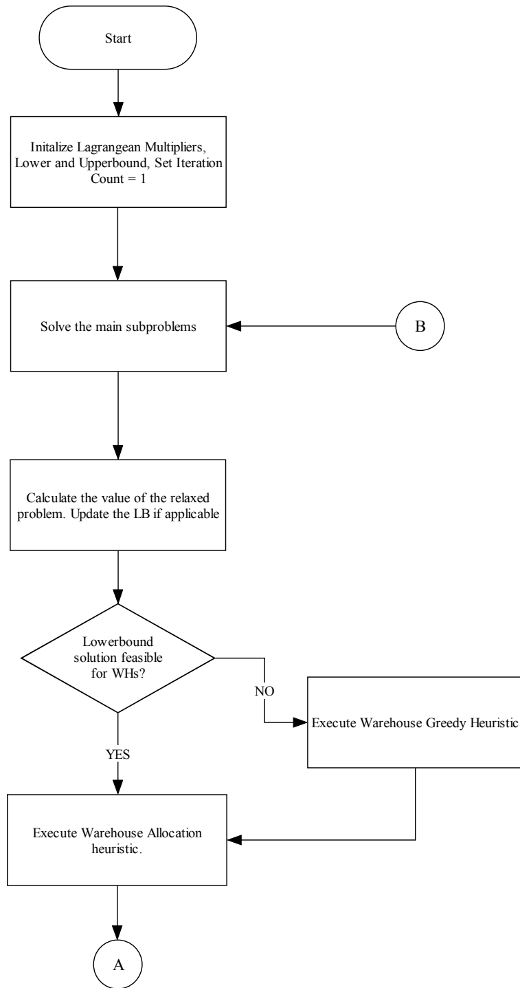
Figure 4.1: The Proposed Lagrangean Heuristic Approach
