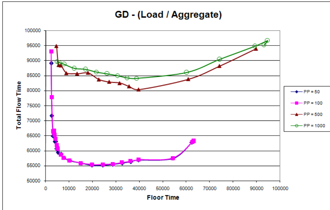
Figure B.7. GD flow pattern with aggregate and load-based listing methods for four levels of ORR period length
