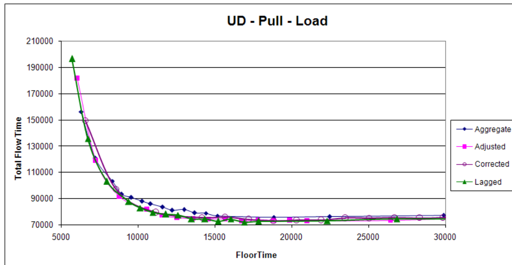
Figure 5.19. UD model pull-type simulated with effect of workload determination methods for load-based listing
