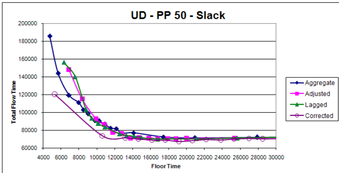
Figure 5.15. The effect of workload determination methods with slack-based listing for UD model
