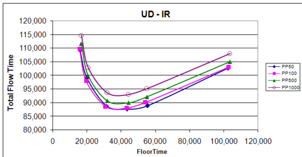
Figure 5.21. IR on UD with period effects
