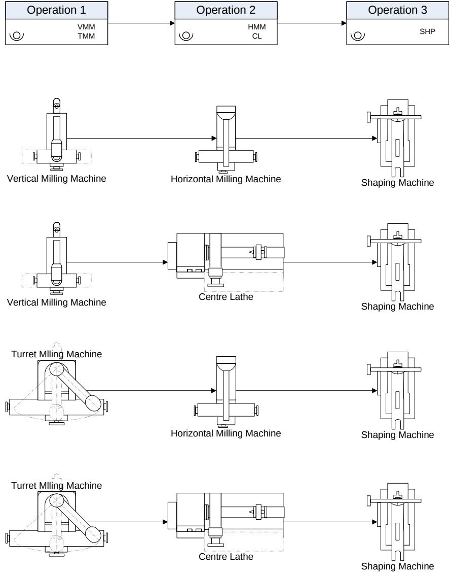
Figure 4.1. Derivation of job sequences from an alternative process route
