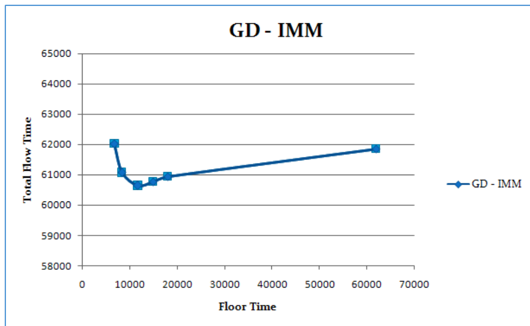
Figure 5.14. GD immediate release with variable I/O. Buffer Sizes
