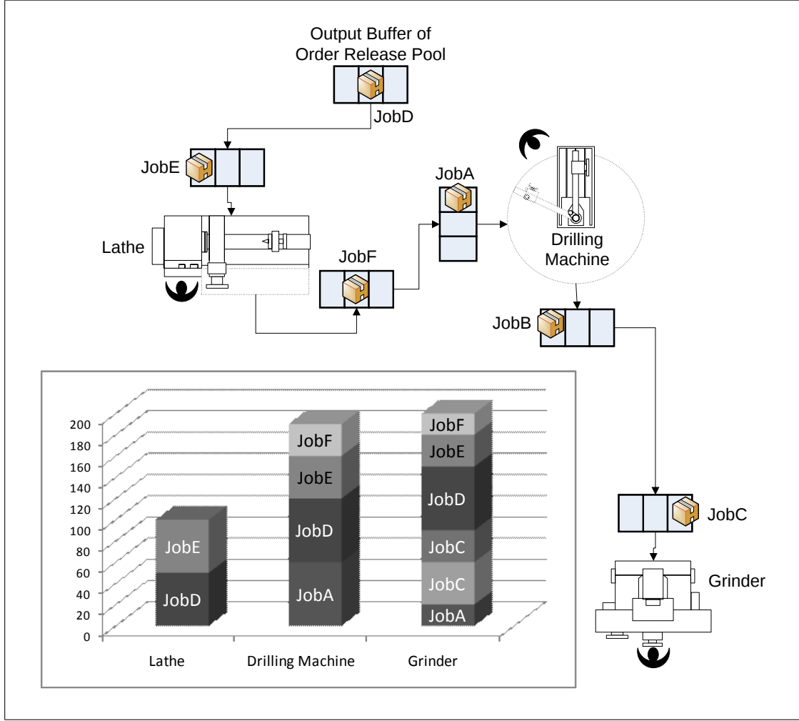
Figure 4.6. Representation of direct and indirect loads
