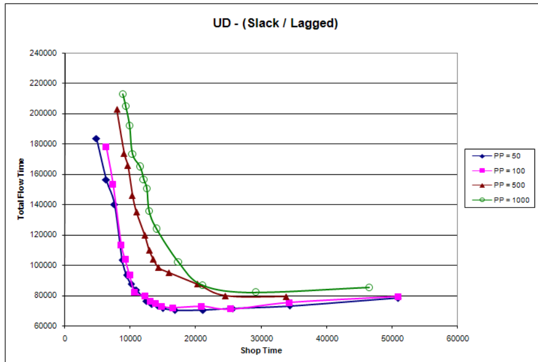
Figure B.13. UD flow pattern with lagged and slack-based listing methods for four levels of ORR period length
