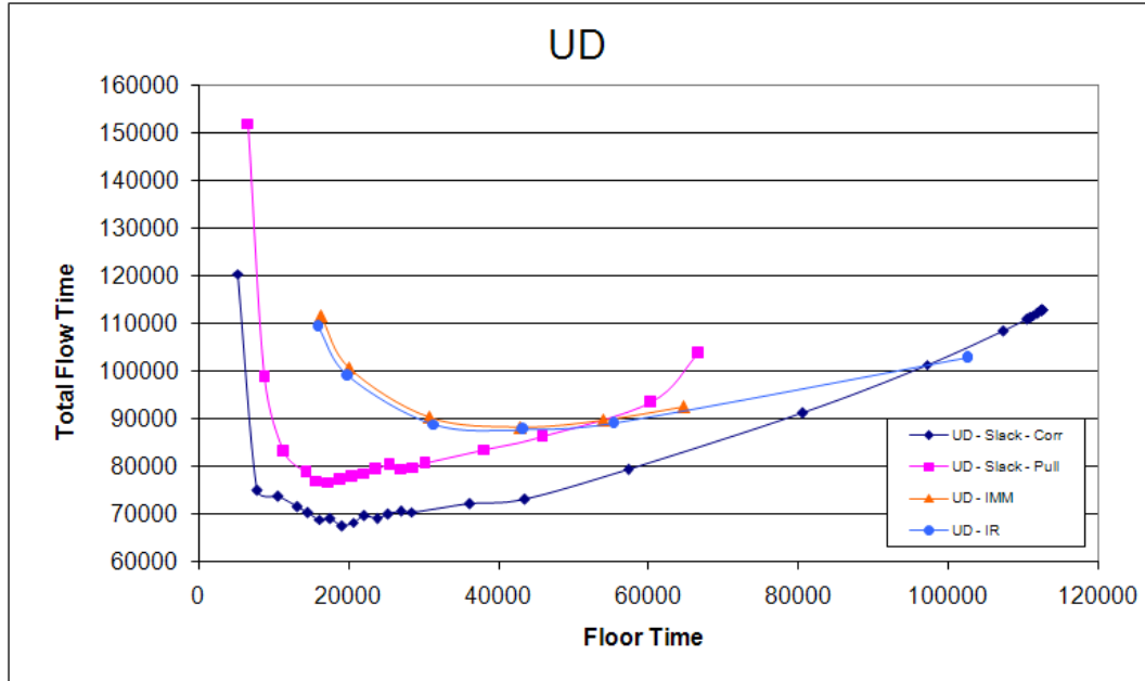
Figure 5.24. Best performing ORR mechanisms for UD part flow pattern
