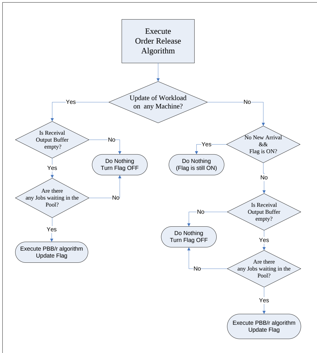
Figure 4.5. Path-based bottleneck execution
