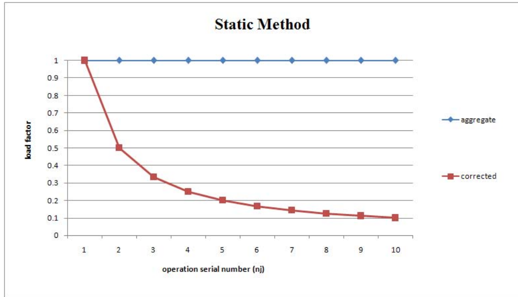
Figure 4.2. Static machine workload determination
