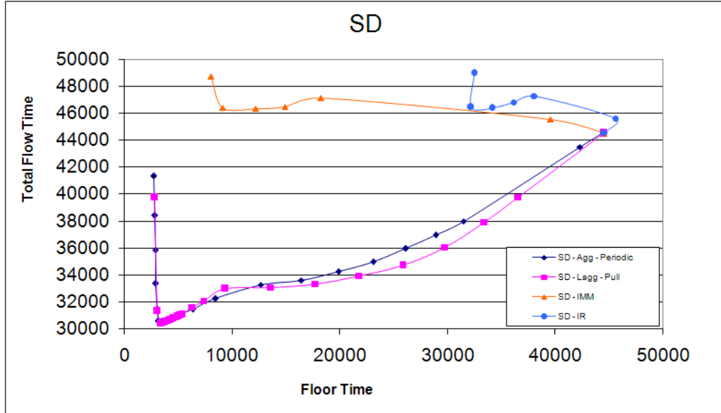
Figure 5.22. Best performing ORR mechanisms for SD part flow pattern
