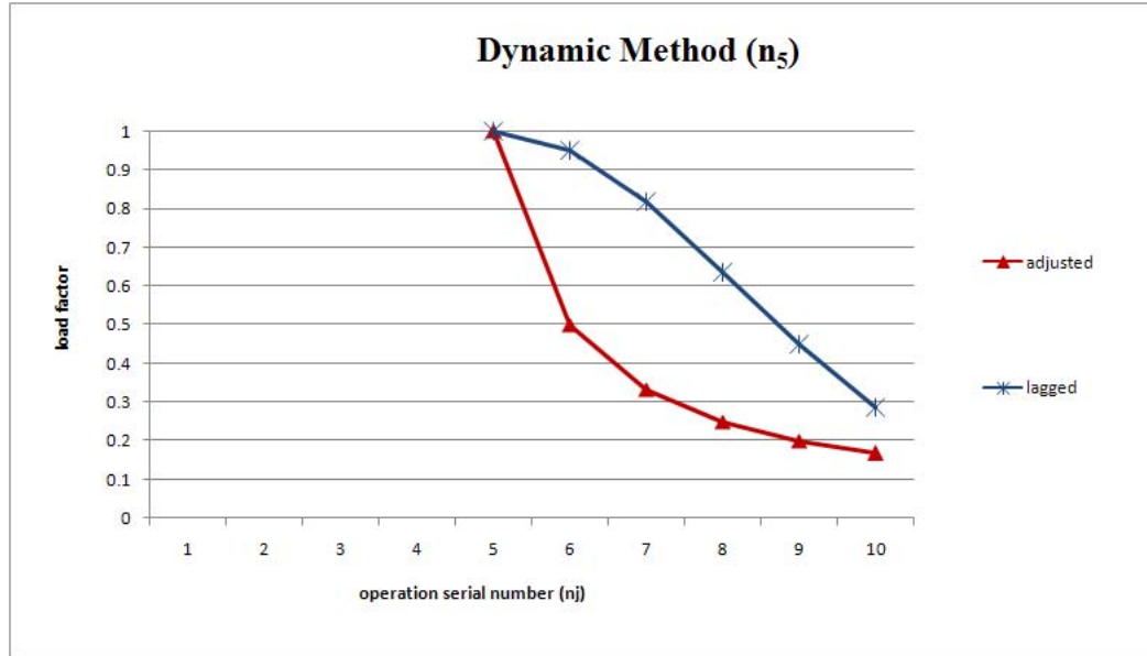
Figure 4.4. Dynamic machine workload determination
