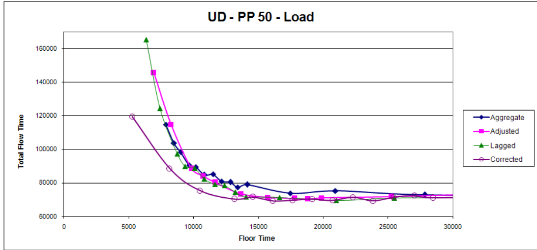
Figure 5.16. UD model with effect of workload determination methods for load-based listing
