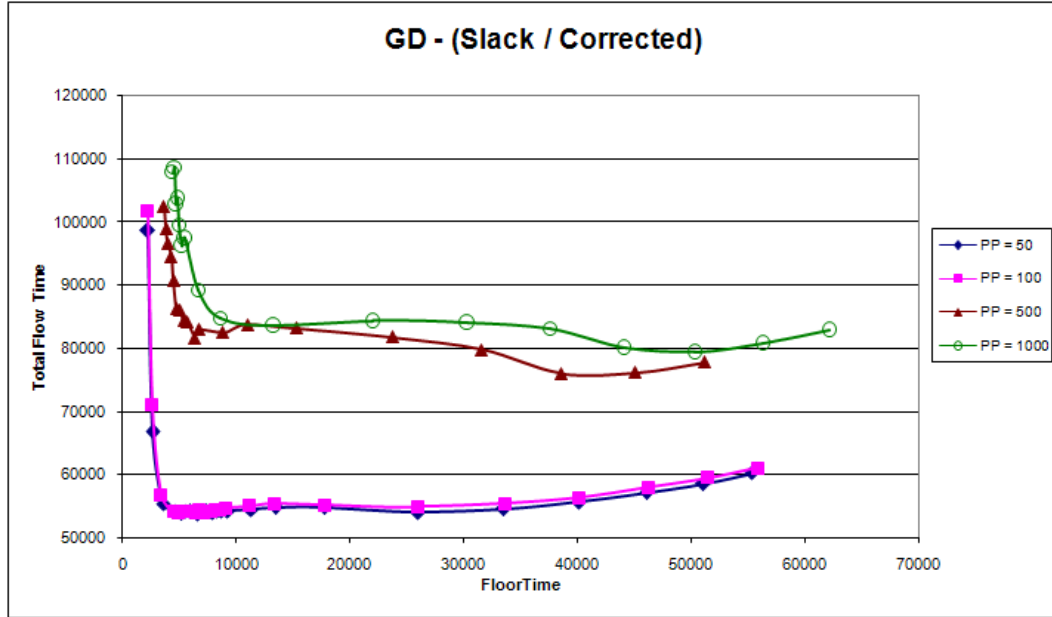
Figure 5.10. GD model with corrected and slack-based listing method for four levels of ORR period length
