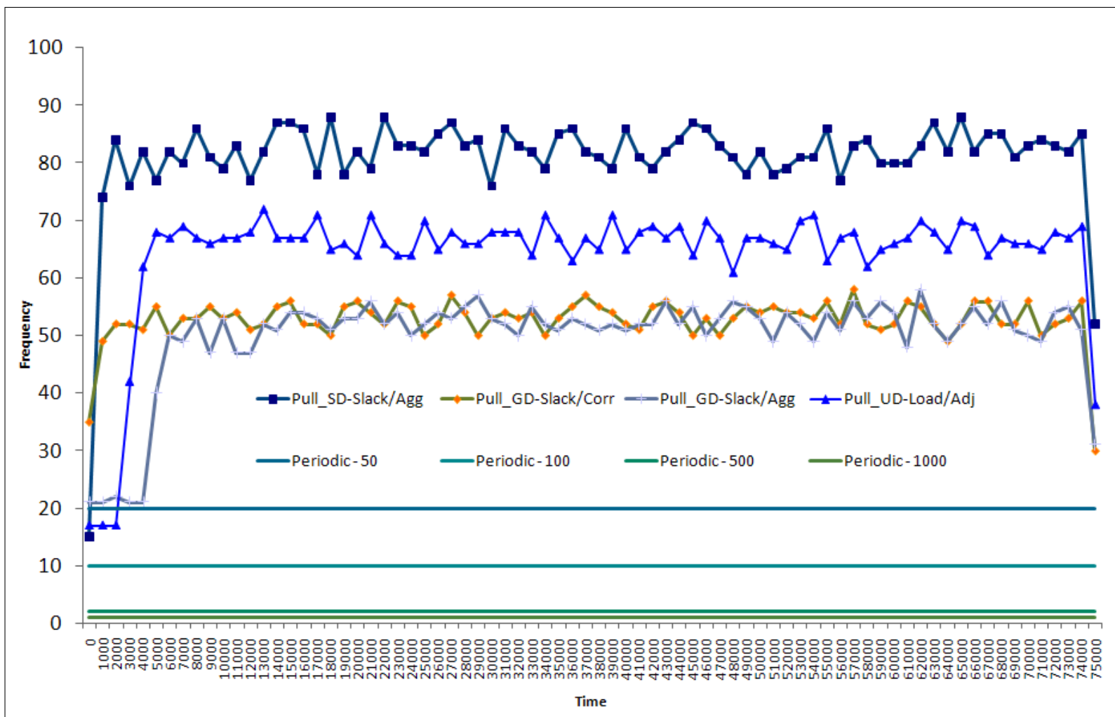
Figure 5.25. Number of ORR mechanism calls per 1000 time units for one of the seeds
