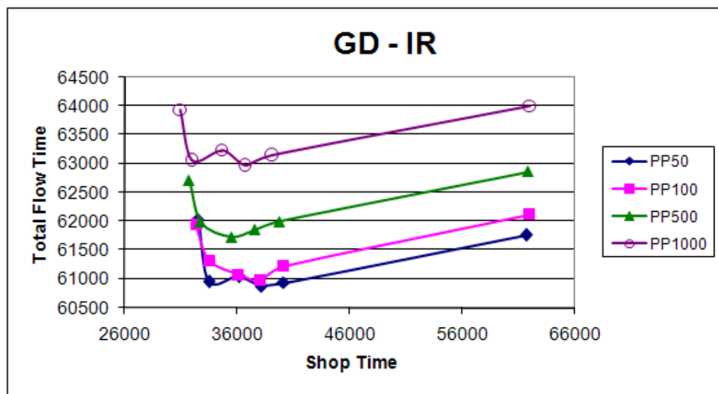
Figure 5.13. IR on GD with period effects
