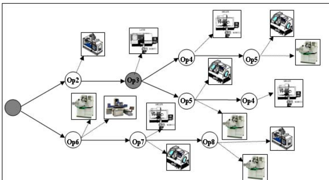
Figure 2.4. Flexible process plan for a part with all Types flexibility
