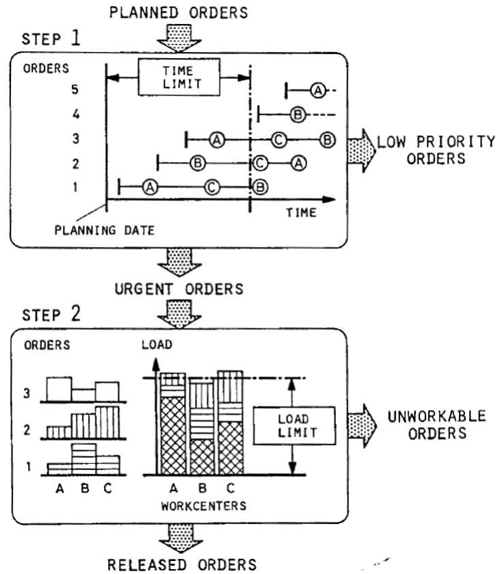
Figure 2.2. First two steps of LOOR after Bechte (1988)
