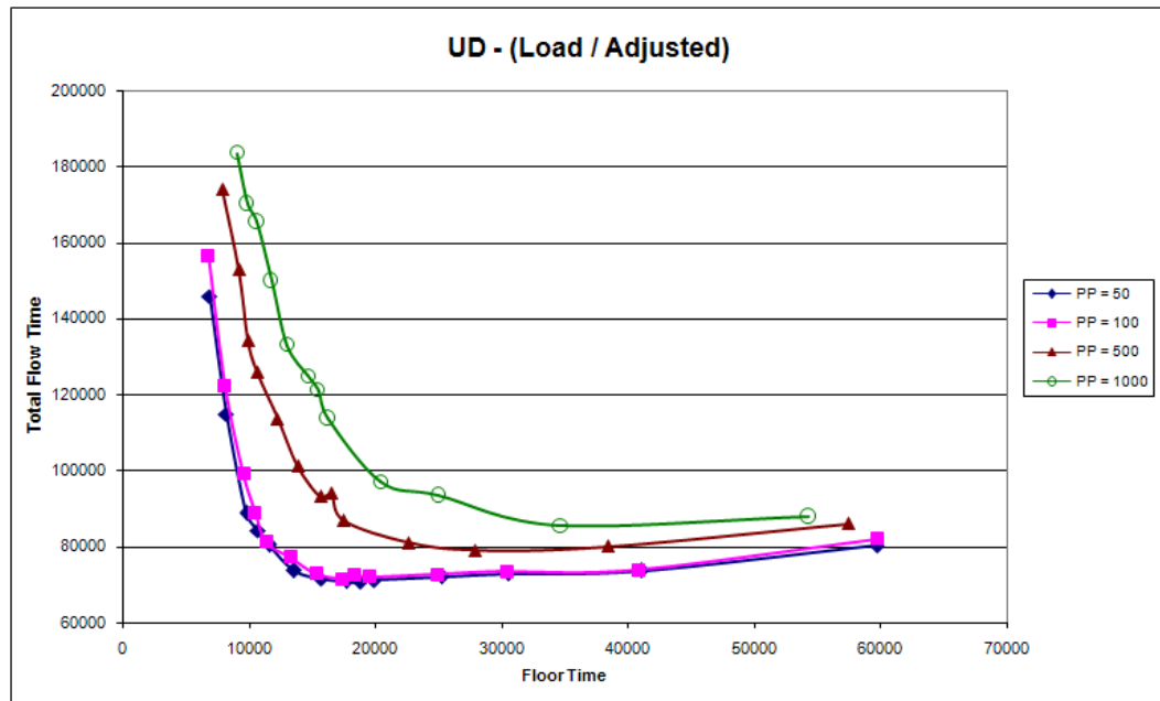
Figure B.15. UD flow pattern with adjusted and load-based listing methods for four levels of ORR period length
