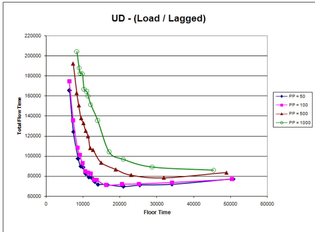
Figure B.17. UD flow pattern with lagged and load-based listing methods for four levels of ORR period length
