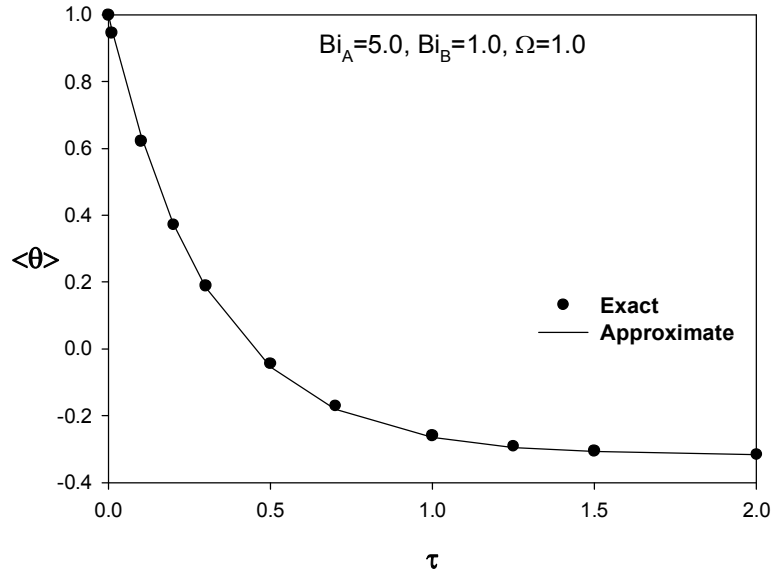
Figure 3.6. Comparison of the analytical and approximate solutions when \Omega = 1.0 , \text{Bi}_A = 5.0 , \text{Bi}_B = 1.0 .
