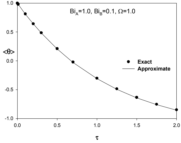
Figure 3.5. Comparison of the analytical and approximate solutions when \Omega = 1.0 , \text{Bi}_A = 1.0 , \text{Bi}_B = 0.1 .
