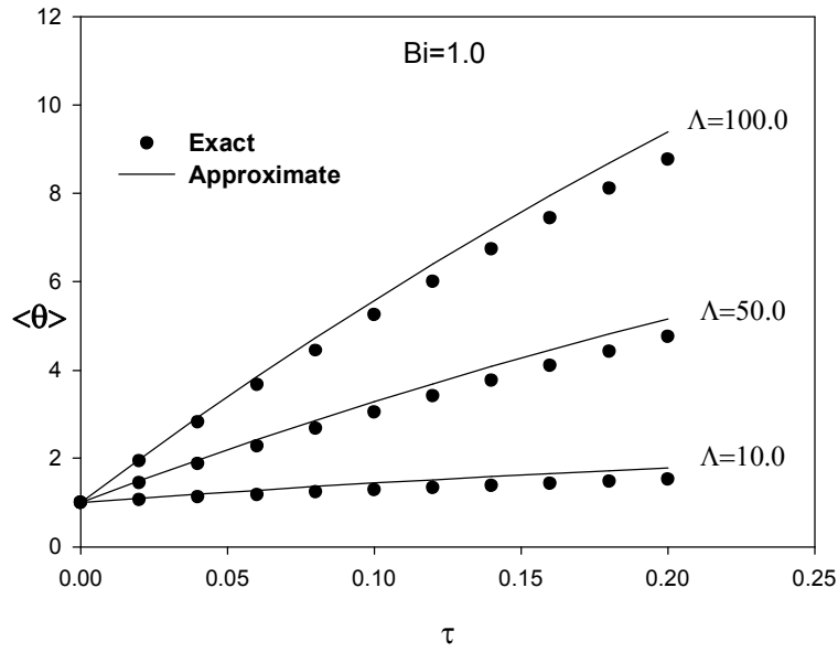
Figure 3.12. Comparison of the analytical and approximate solutions when \text{Bi} = 1.0 with \Lambda as a parameter.
