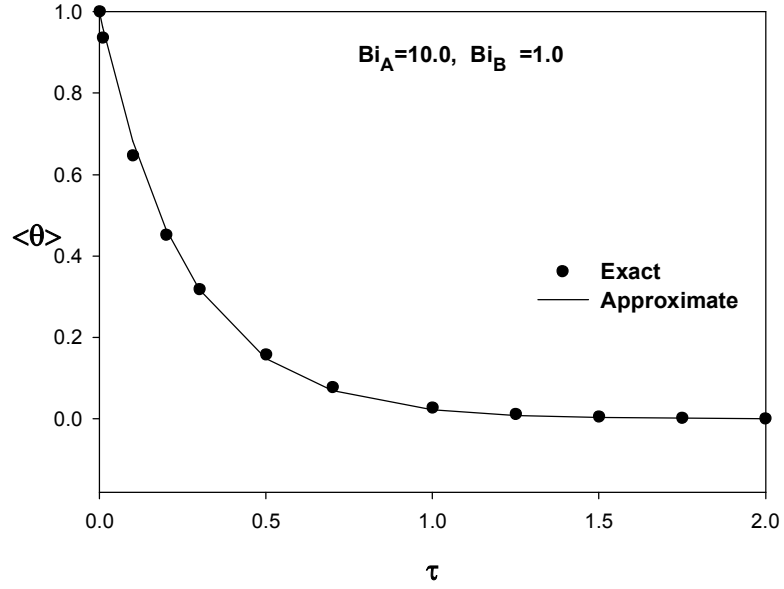
Figure 3.9. Comparison of the analytical and approximate solutions when \Omega = 0 , \text{Bi}_A = 10.0 , \text{Bi}_B = 1.0 .
