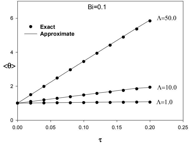
Figure 3.11. Comparison of the analytical and approximate solutions when \text{Bi} = 0.1 with \Lambda as a parameter.
