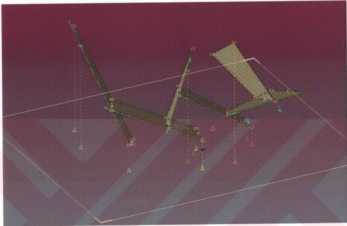
Figure 10: Associative geometric model defined for the Philibert De L'Orme pavilion designed by Objectile.
