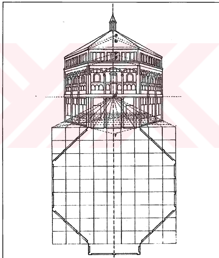
Figure 1: Schematic representation of perspective panel by Brunelleschi
