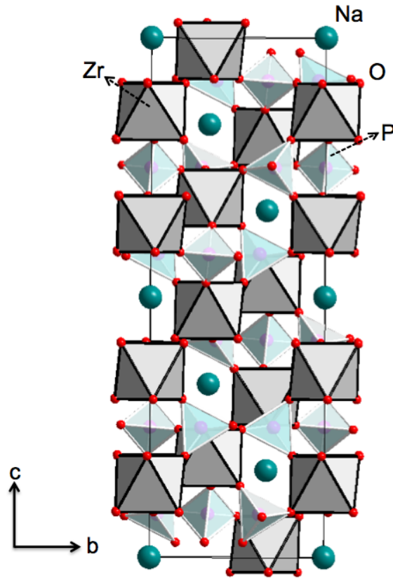
Figure 1.3. Crystal structure of NASICON type solid electrolytes [13]
