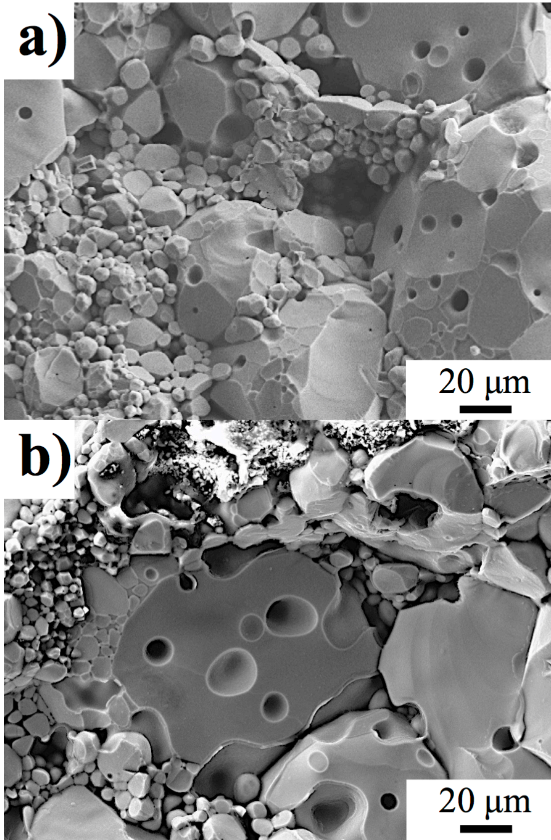
Figure 2.8. Secondary electron images obtained from the fractured surfaces of the pellets of 30 mole % Al containing LLZO sintered at 1150 °C for: a) 12 h b) 24 h and c) 36 h
