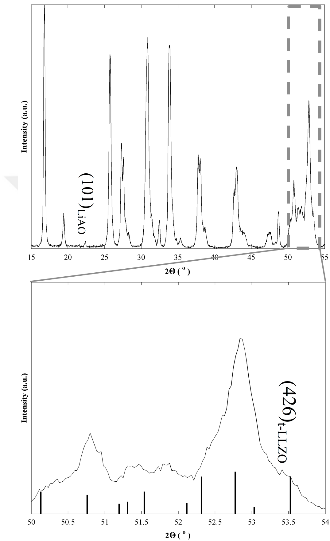
Figure 5.1. XRD pattern of 30 mole % Al containing LLZO pellet sintered at 1100 °C for 24 hours
