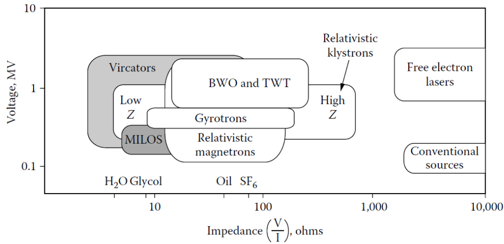
Figure 2.3: Various classes of HPM sources and conventional microwave sources with optimal impedance and voltage [1]
