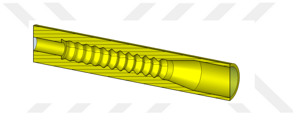
Figure 2.8: Schematic of BWO with output horn antenna [51]
