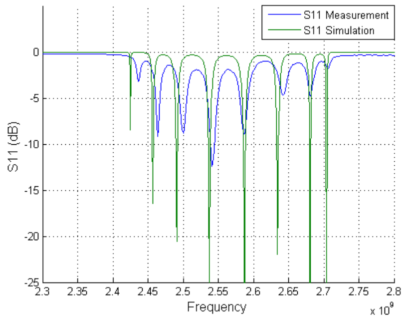
Figure 4.32: S11 of the Fabricated SWS for Mode 3
