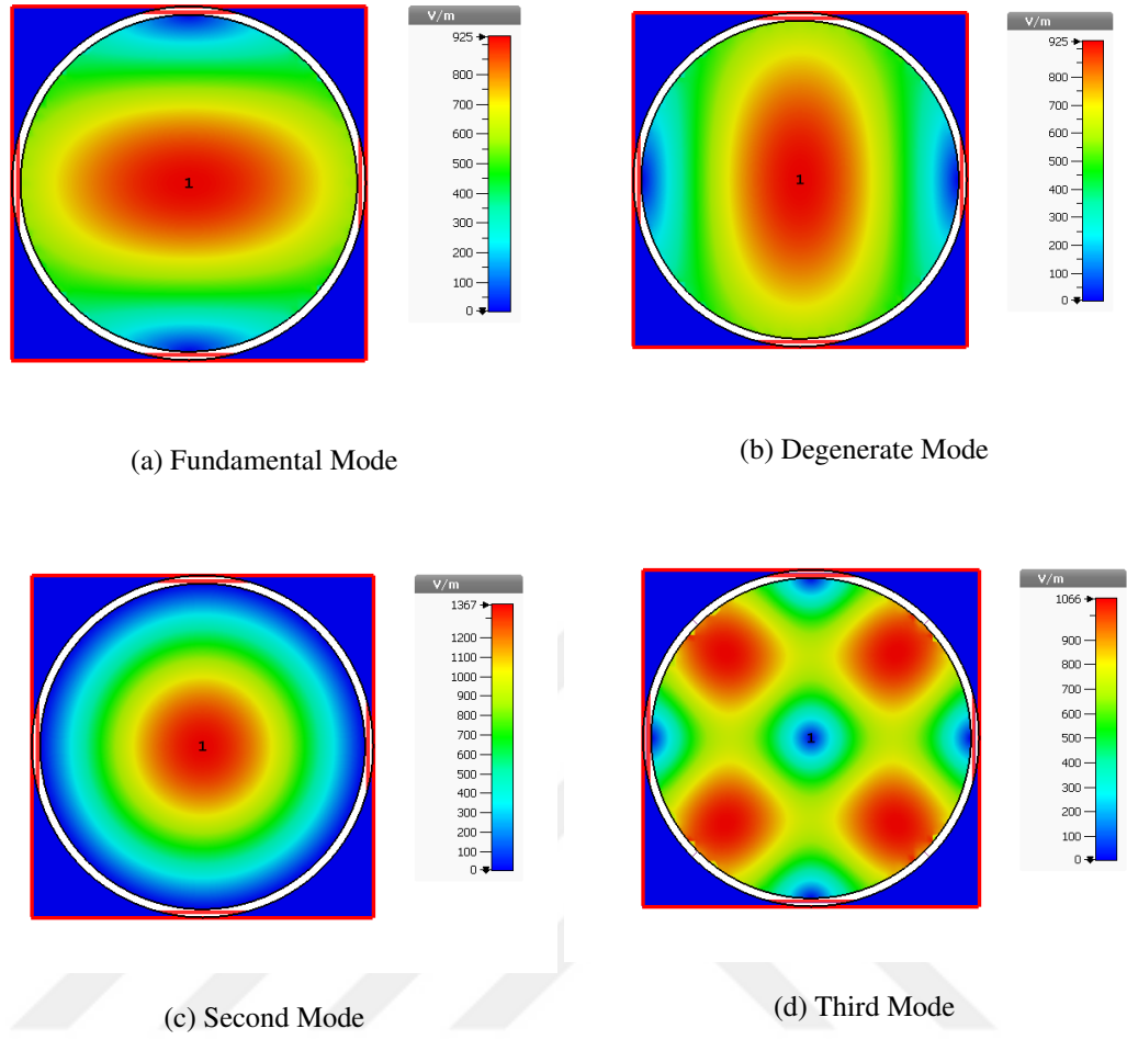
Figure 4.6: Electric Field of Hollow Circular Waveguide for Lowest-order 4 Modes
