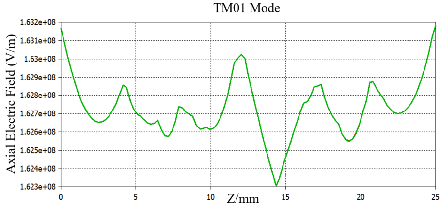
Figure 4.14: TM 01 Axial Electric Field
