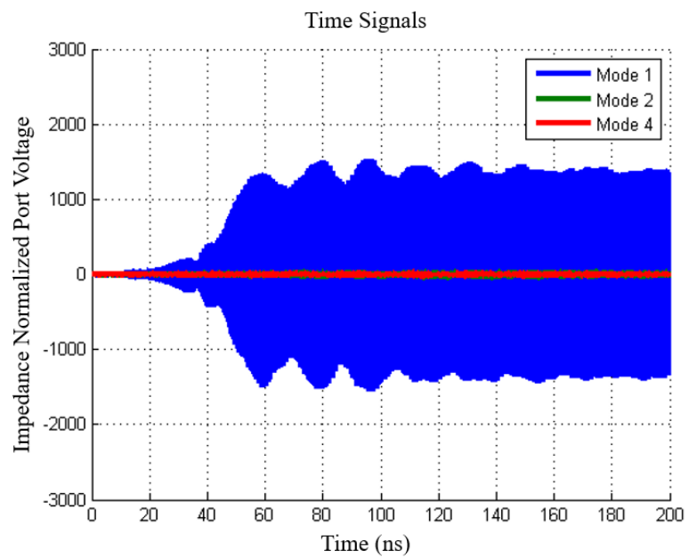
Figure 4.37: Impedance Normalized Output Voltage Signal for Mode 1,2 and 4
