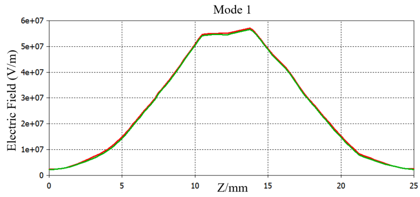
Figure 4.8: Mode 1 Absolute and Axial Component of the Electric Field
