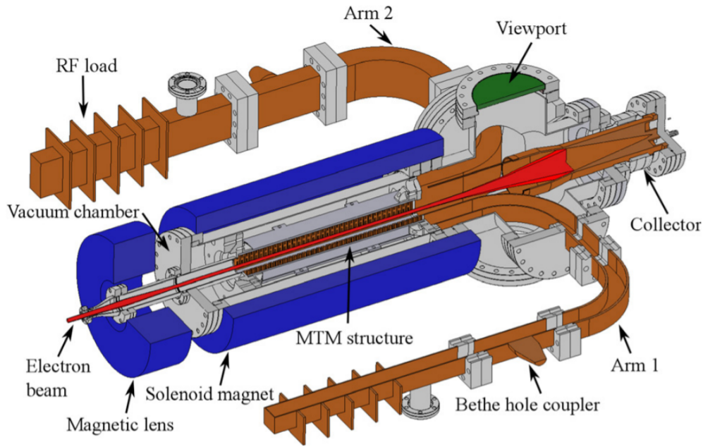
Figure 2.13: Schematic of Metamaterial based BWO [66]
