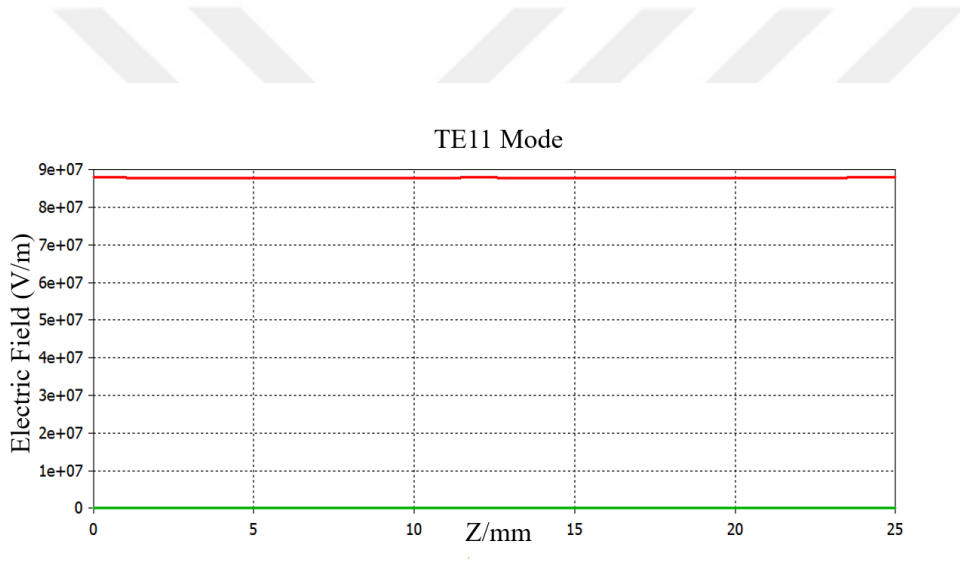
Figure 4.12: TE 11 Absolute and Axial Component of the Electric Field
