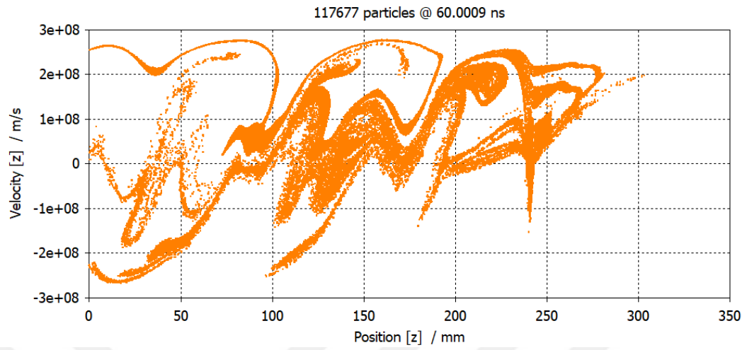
Figure 4.47: Axial Electron Velocity vs. Position at 60 ns
