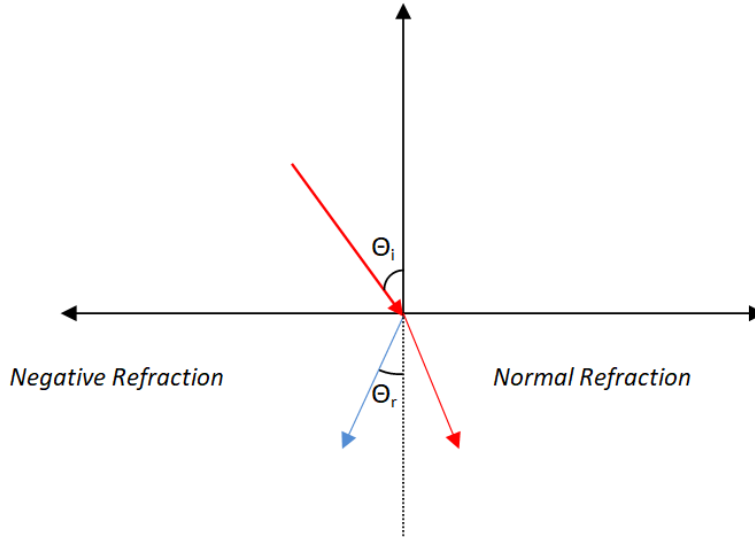
Figure 3.3: Snell's Law in the negative refraction index
