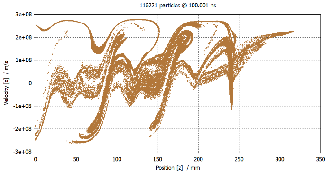
Figure 4.42: Axial Electron Velocity vs. Position at 100 ns
