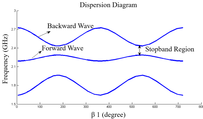
Figure 3.2: Dispersion Diagram of the Lowest Order Modes
