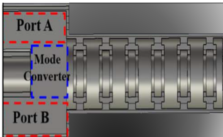
Figure 2.9: Schematic of BWO with mode converter [52]
