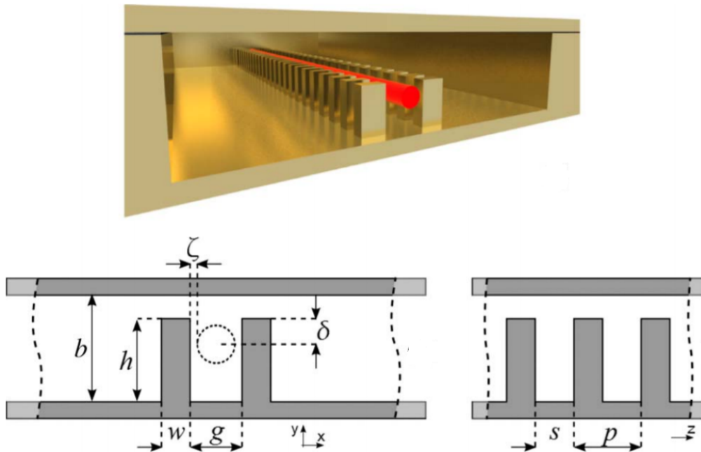
Figure 2.12: Rectangular Solid Corrugation SWS [57]
