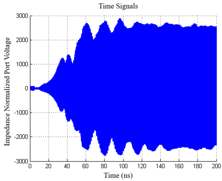
Figure 4.36: Impedance Normalized Output Voltage Signal for Mode 3
