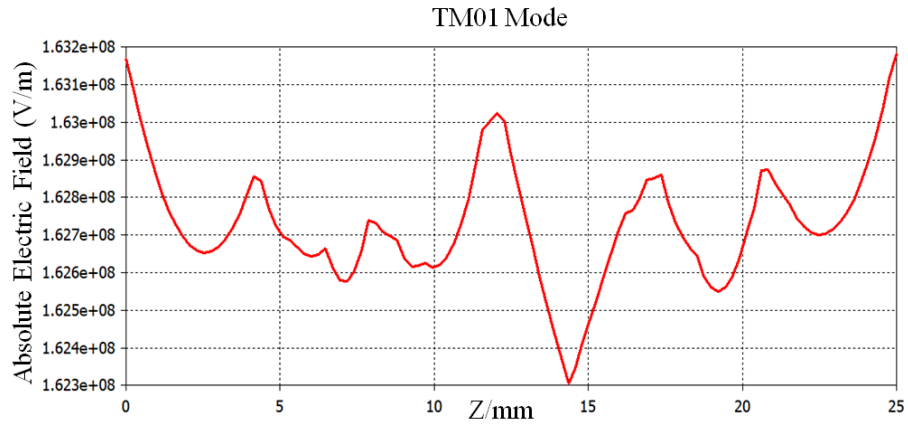
Figure 4.13: TM 01 Absolute Electric Field
