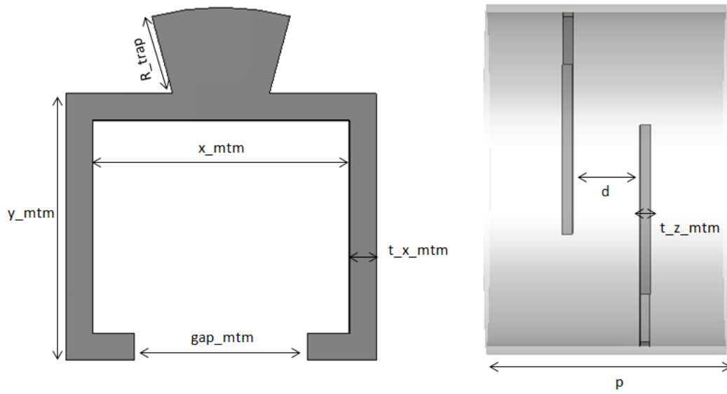
Figure 4.3: Geometry of the SWS
