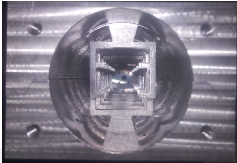
Figure 4.25: Fabricated SWS
