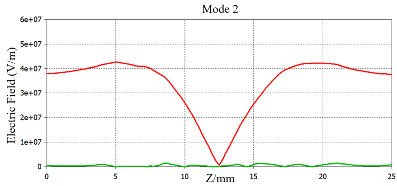
Figure 4.9: Mode 2 Absolute and Axial Component of the Electric Field
