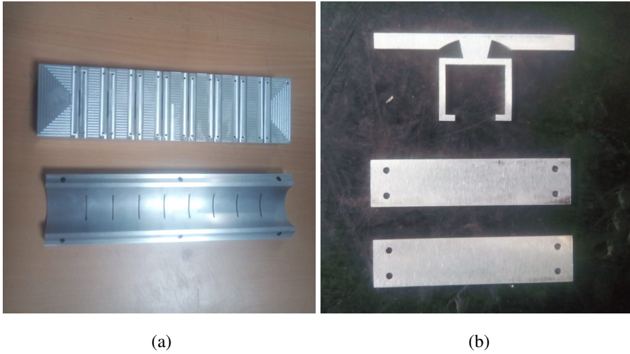
Figure 4.23: Part of the Fabricated SWS
