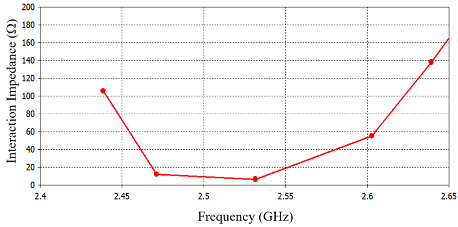
Figure 4.18: Interaction Impedance of the SWS
