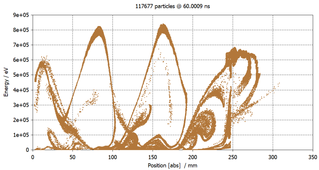
Figure 4.48: Energy of Particles vs. Position at 60 ns
