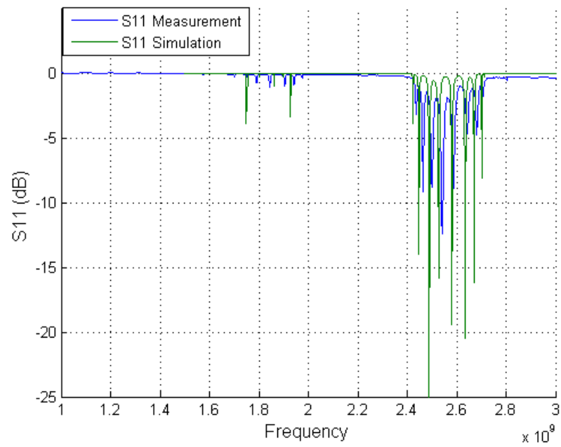
Figure 4.30: S11 of the Fabricated SWS
