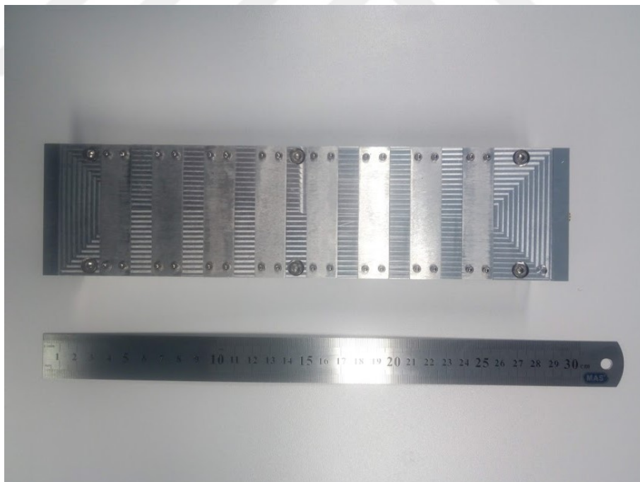
Figure 4.26: Fabricated SWS Dimension
