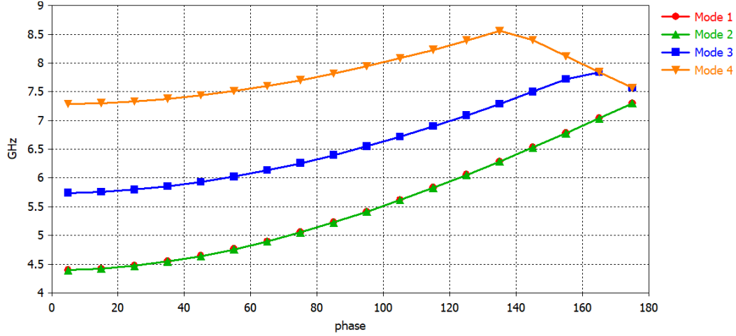
Figure 4.7: Dispersion Diagram of Hollow Circular Waveguide
