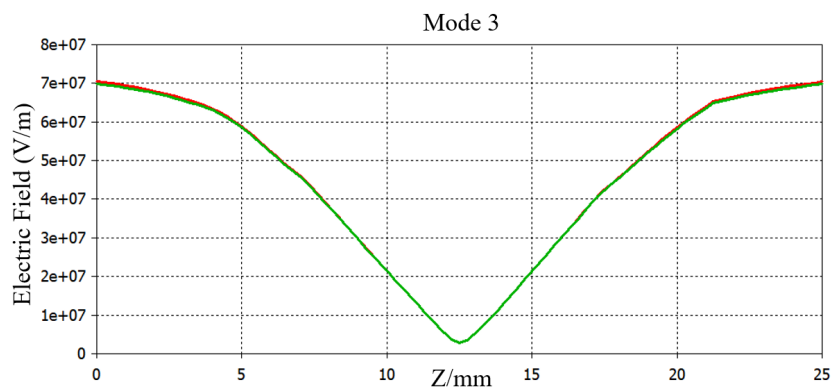
Figure 4.10: Mode 3 Absolute and Axial Component of the Electric Field
