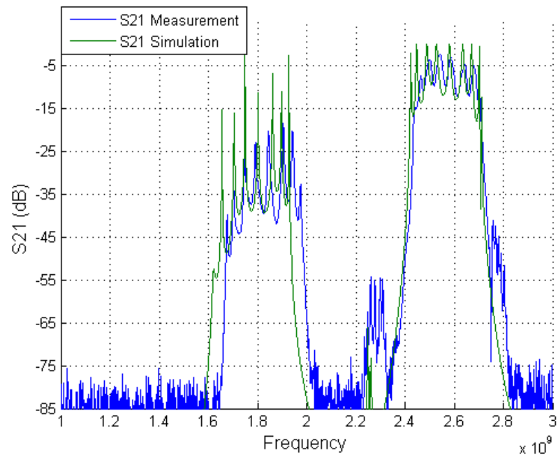
Figure 4.31: S21 of the Fabricated SWS
