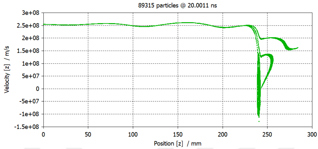
Figure 4.45: Axial Electron Velocity vs. Position at 20 ns
