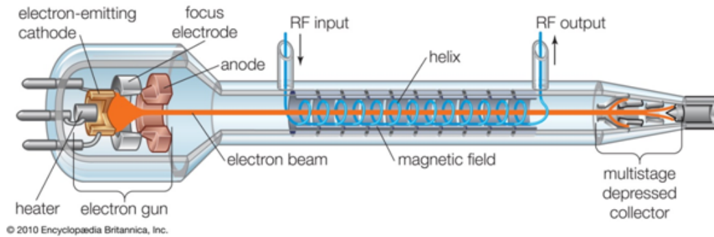
Figure 2.6: Schematic of TWT [41]
