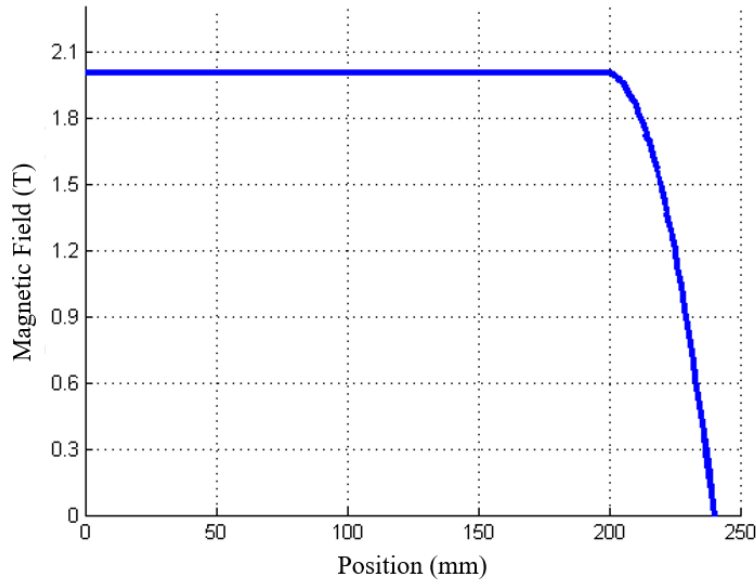
Figure 4.35: Applied Analytical Magnetic Field
