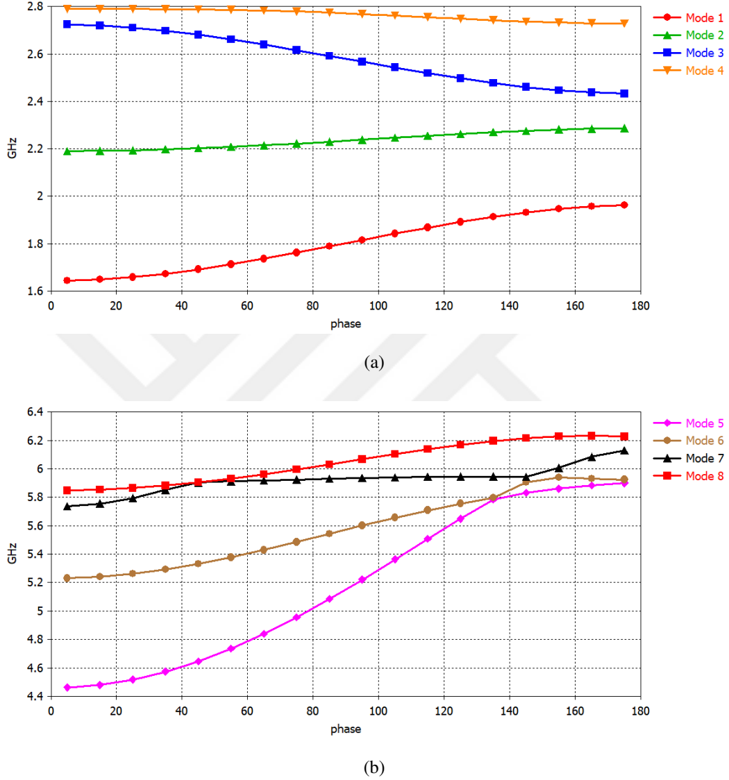
Figure 4.5: (a) Dispersion diagram of lowest order first 4 modes (b) Dispersion diagram of lowest order second 4 modes
