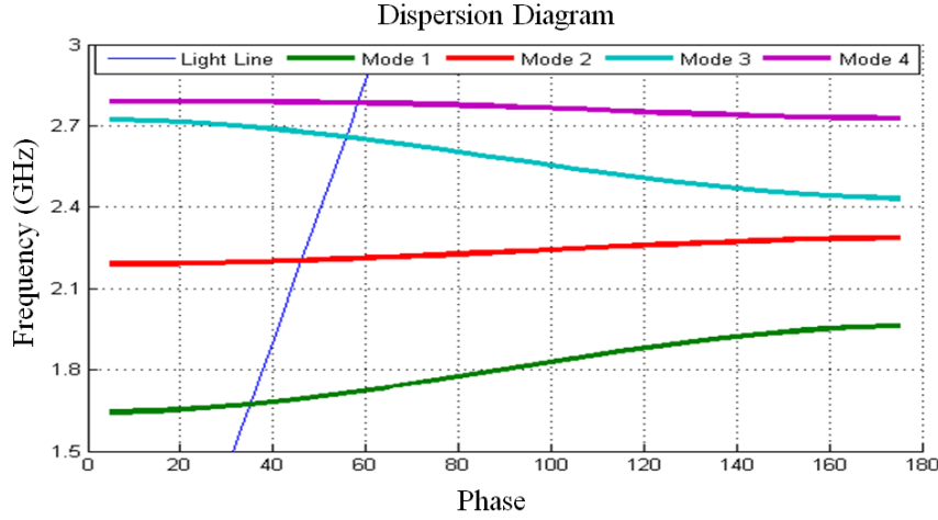
Figure 4.15: Dispersion Diagram of SWS with Light Line
