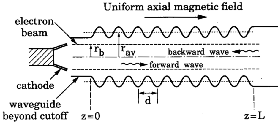
Figure 2.10: Sinusoidally Corrugated SWS [52]
