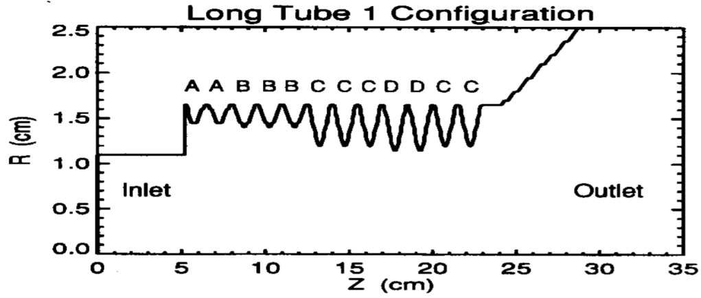
Figure 2.11: Nonuniformly Corrugated SWS [53]
