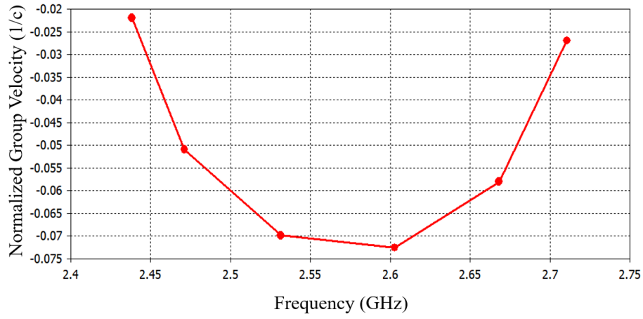
Figure 4.17: Normalized Group Velocity of the Mode 3
