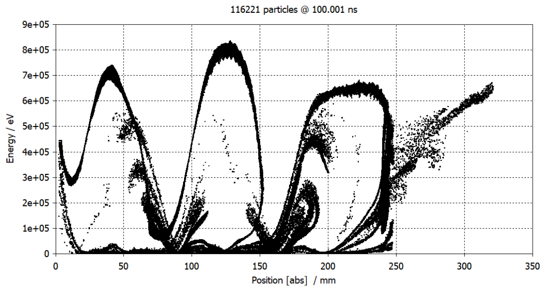
Figure 4.50: Energy of Particles vs. Position at 100 ns
