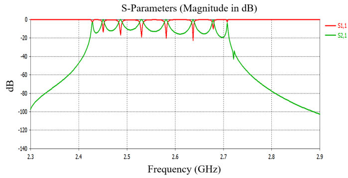
Figure 4.27: S Parameter Simulation of SWS for Mode 3 Frequencies
