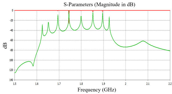
Figure 4.28: S Parameter Simulation of SWS for Mode 1 Frequencies
