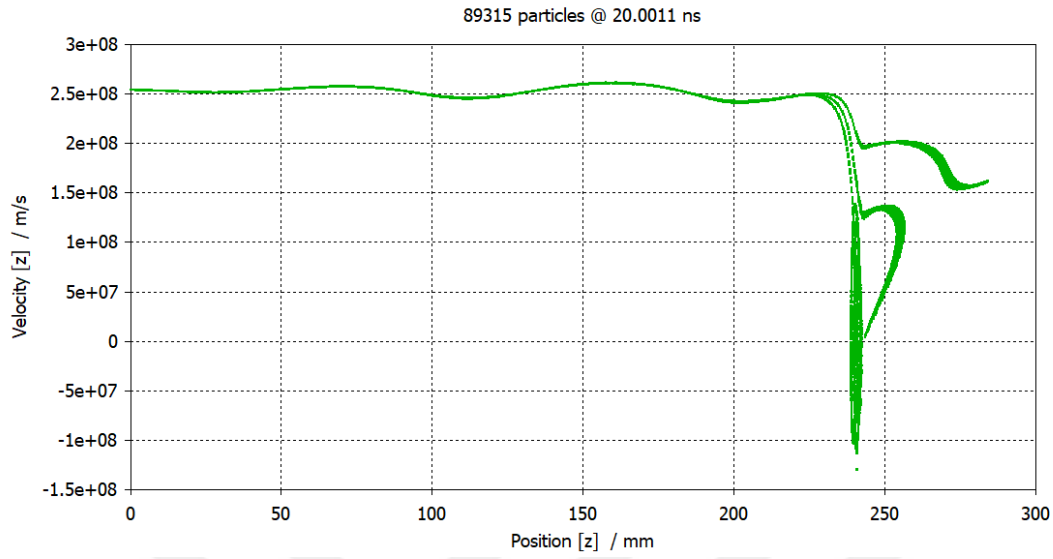
Figure 4.41: Axial Electron Velocity vs. Position at 20 ns
