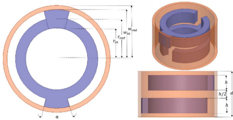
Figure 2.14: Geometry of Metamaterial SWS used in [68]
