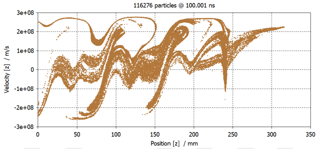
Figure 4.49: Axial Electron Velocity vs. Position at 100 ns
