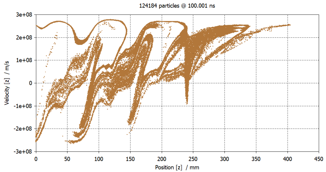
Figure 4.44: Axial Electron Velocity vs. Position at 100 ns for 1 T Magnetic Field
