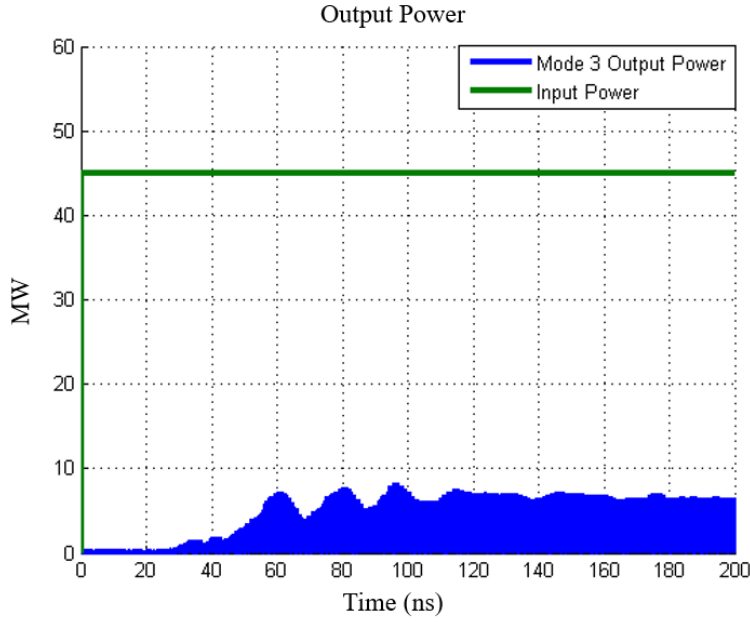
Figure 4.40: Output Power Signal
