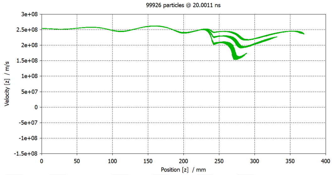
Figure 4.43: Axial Electron Velocity vs. Position at 20 ns for 1 T Magnetic Field
