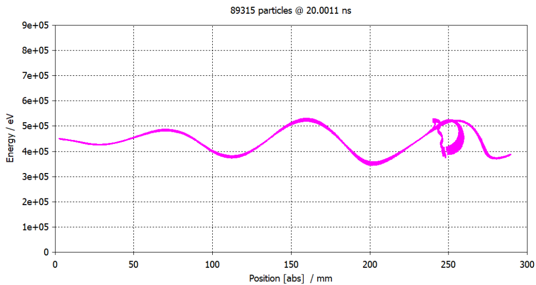
Figure 4.46: Energy of Particles vs. Position at 20 ns
