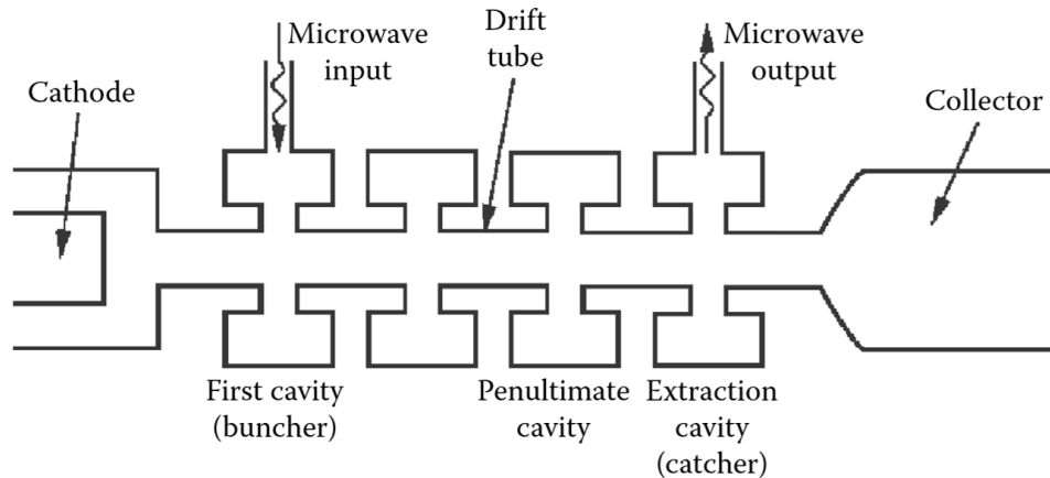
Figure 2.4: Schematic form of Klystron [1]
