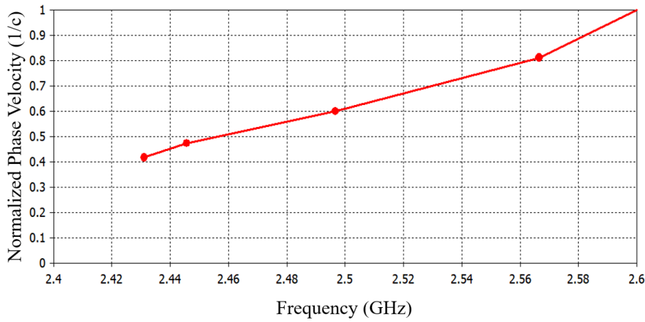
Figure 4.16: Normalized Phase Velocity of the Mode 3
