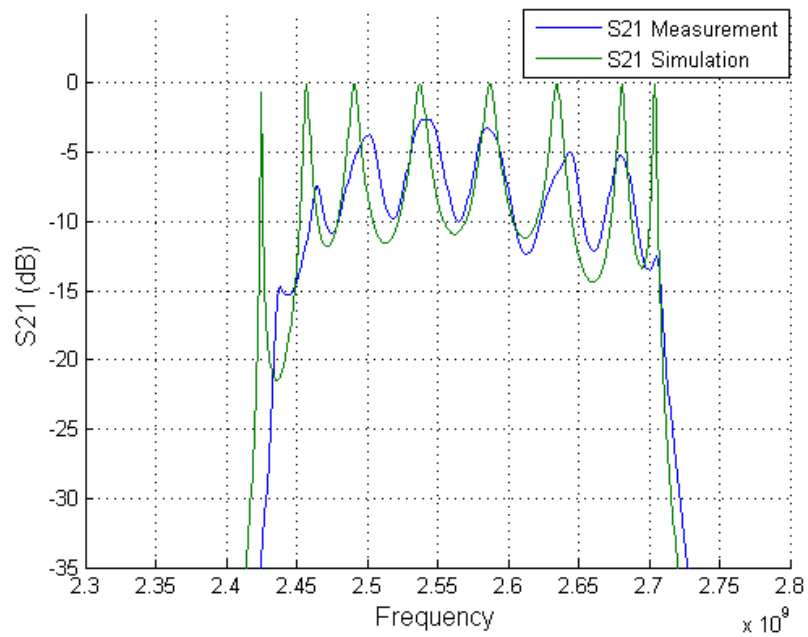
Figure 4.33: S21 of the Fabricated SWS for Mode 3
