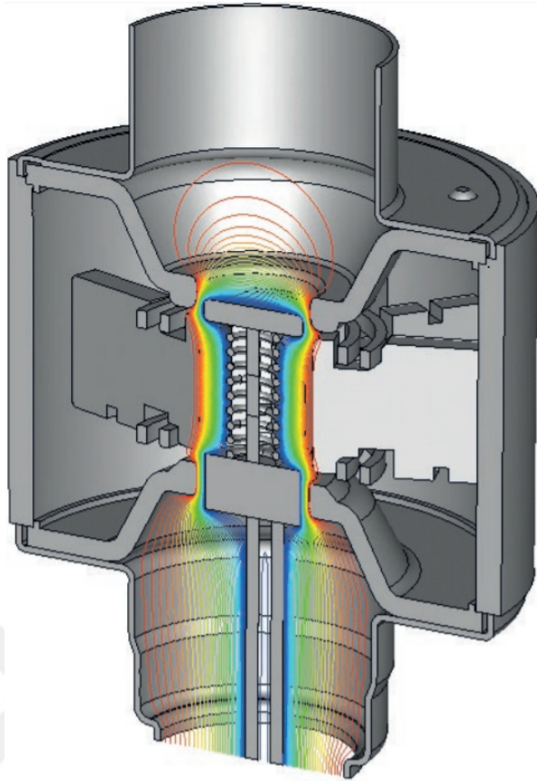
Figure 2.5: 3D Modeling of Magnetron [32]
