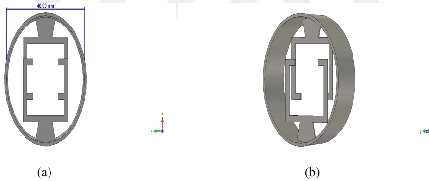
Figure 4.4: (a) Dimension of the SWS (b) One unit of the SWS
