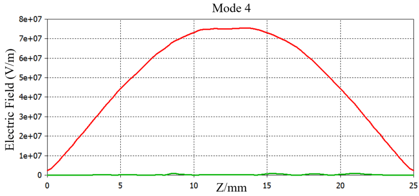
Figure 4.11: Mode 4 Absolute and Axial Component of the Electric Field
