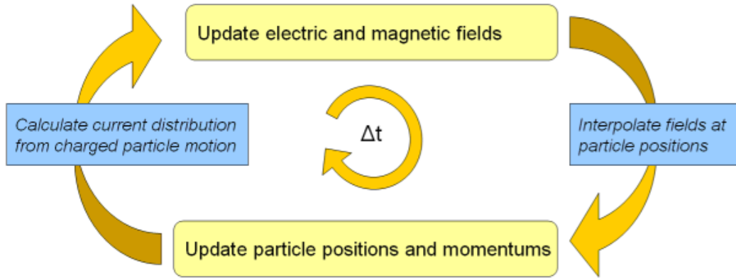
Figure 4.2: PIC Solver Interpolation Schemes
