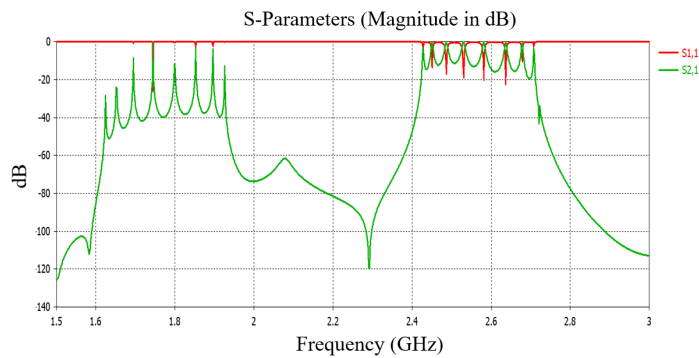
Figure 4.29: S Parameter Simulation of SWS for Mode 1 and Mode 3 Frequencies
