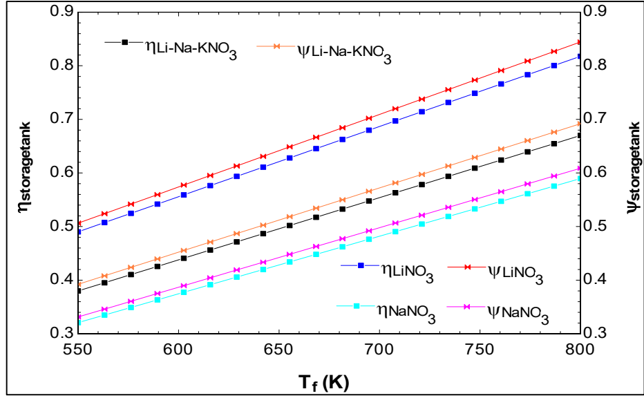
Figure 5.20 Effect of the final temperature of phase change material on the energy and exergy efficiency of the hot storage tank
