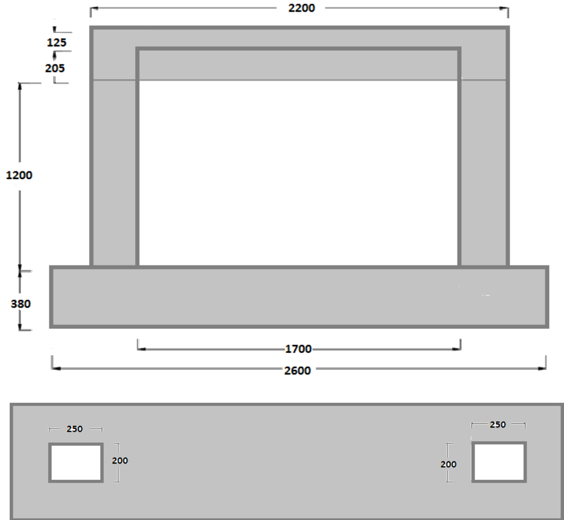
Figure 4.2: Geometry of the specimens.
