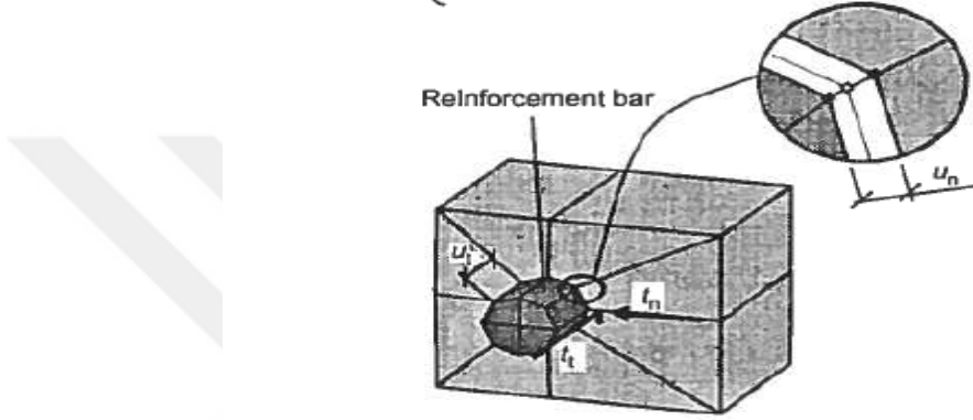
Figure 2.5: Variables of bond model interpretation t_n , t_t , u_n and u_t .
