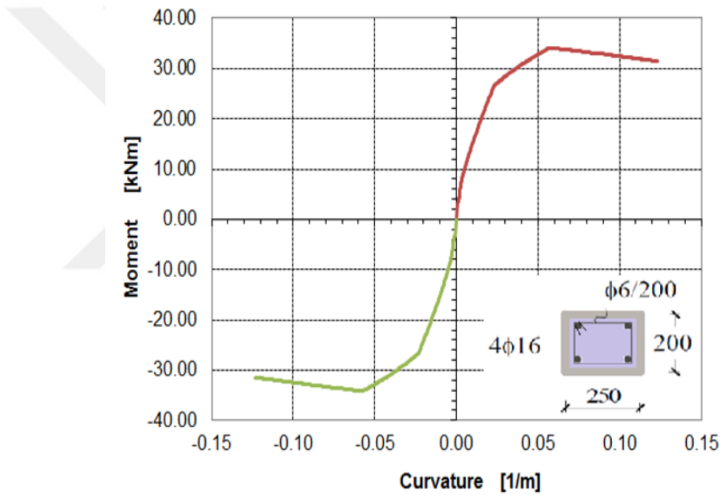
Figure 5.5: moment and curvature relationships of bottom column part of 15 years old frame.
