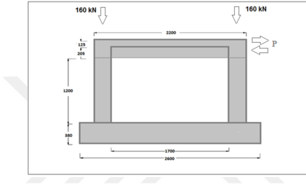
Figure 5.1: Model for analytical study in DC-2B(s2) program .
