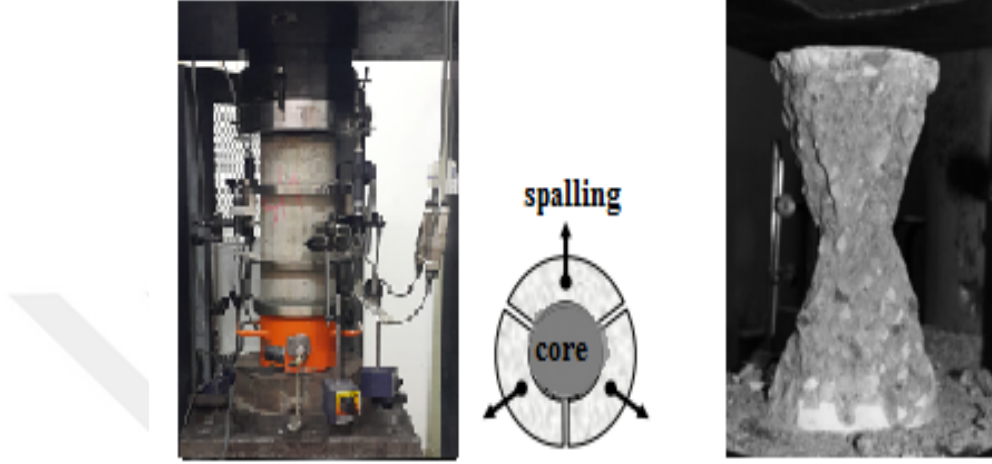
Figure 3.6: Concrete specimens during the compression and after test
