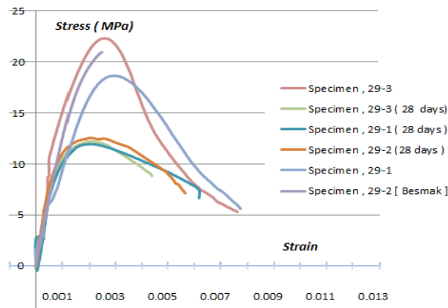
Figure 4.17: Relationship between compressive strength -strain with age for concrete cylinder specimens.
