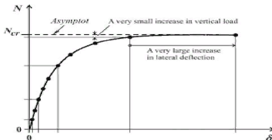
Figure 5.24: P-Delta curve assesment for buckling load.
