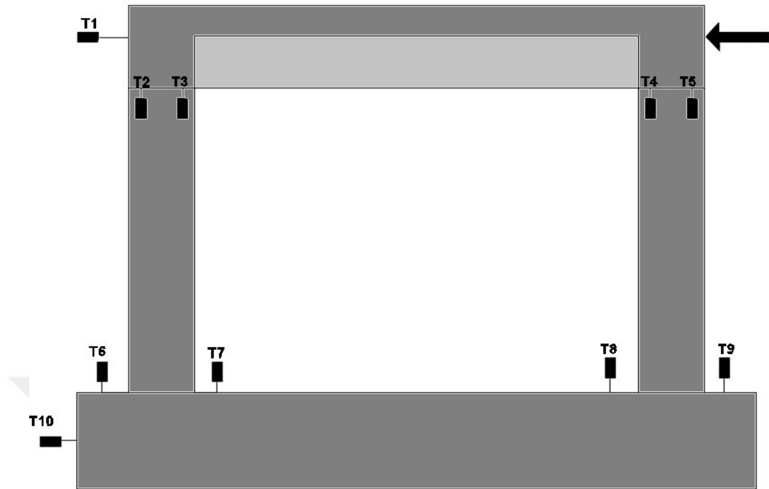
Figure 4.10: LVDTs used in test setup-view of specimen front side.
