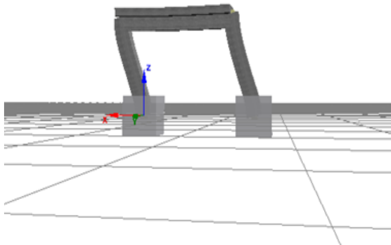
Figure 5.22: Damage shape of analiytical work of RCF-2 at pull cyle.
