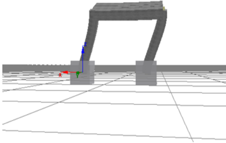
Figure 5.21: Damage shape of analytical work of RCF-2 at push cyle.
