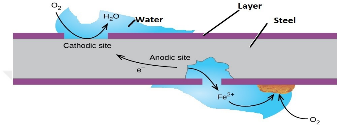
Figure 2.2: Natural corrosion process of reinforcement steel bar.
