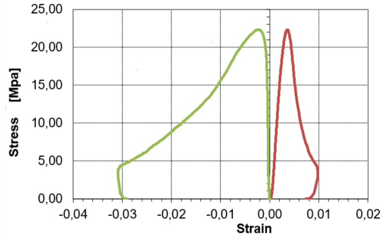
Figure 4.51: Vertical and horizontal strain versus stress diagram of specimen S2/29-1.
