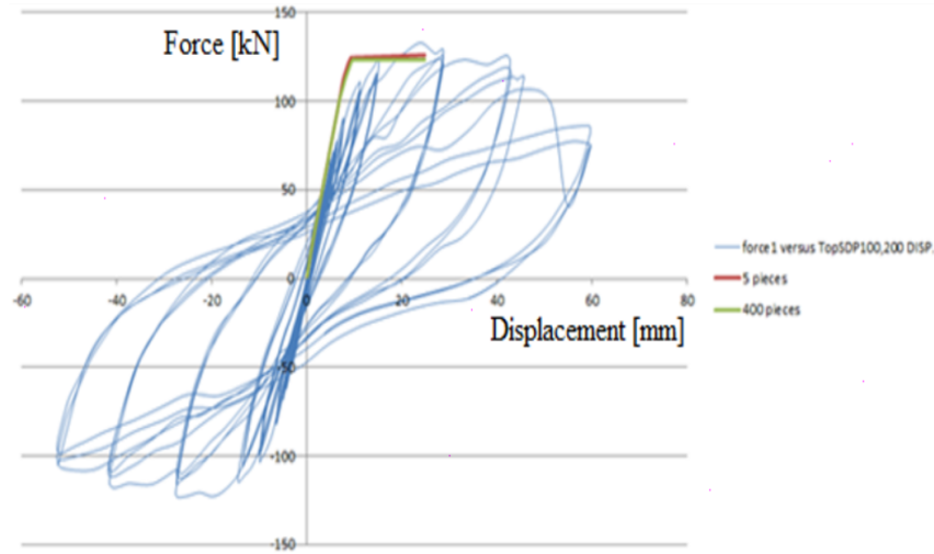
Figure 5.10: Force – Displacement curves of the computer program versus experiment with 5 and 400 pieces for RC members.
