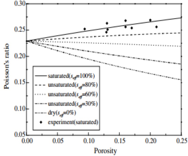
Figure 3.3: Relationship between Poisson's ratio and porosity of unsaturated concrete.
