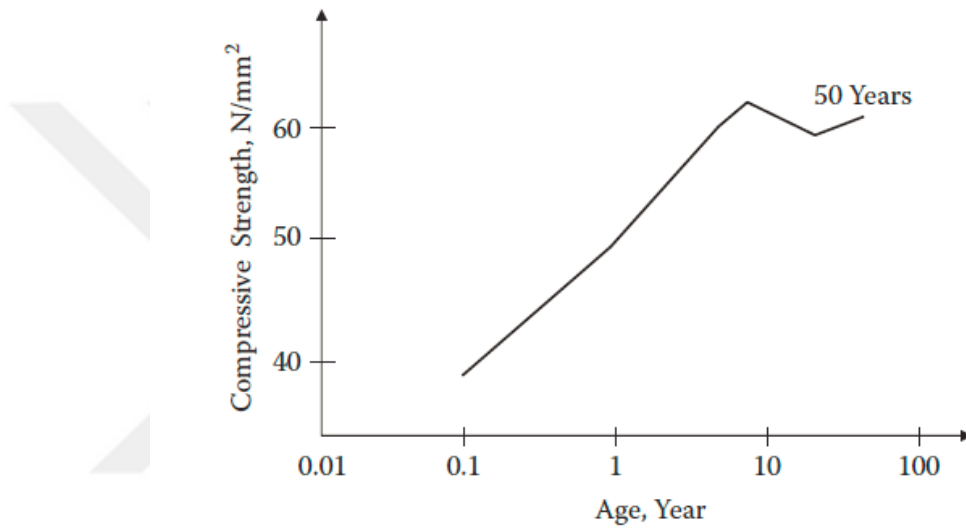
Figure 4.15: Concrete strength variation with age.
