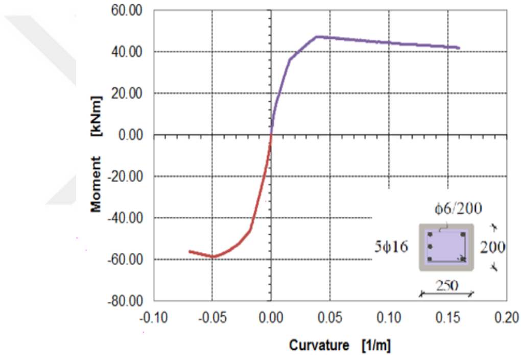
Figure 5.6: Moment and curvature relationships of upper column part of 15 years old frame.
