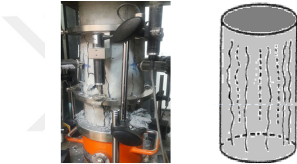
Figure 4.50: Failure mode of specimens S/30-2 under axial loading.
