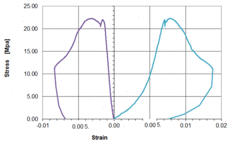
Figure 4.53: Vertical and horizontal strain versus stress diagram of specimen S2/29-1.
