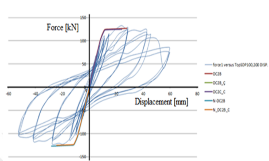
Figure 5.9: Force – Displacement curves of the computer program versus experimental.
