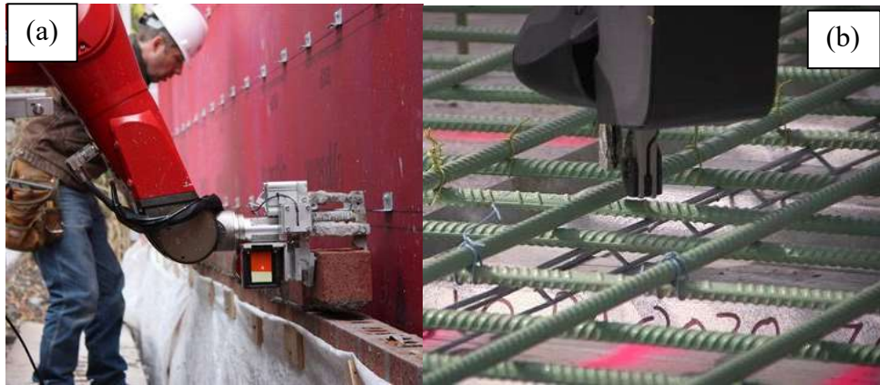
Figure 27 (a) SAM100 world's first commercially available robot [137], (b) Tybot robot for rebar tying [138].
