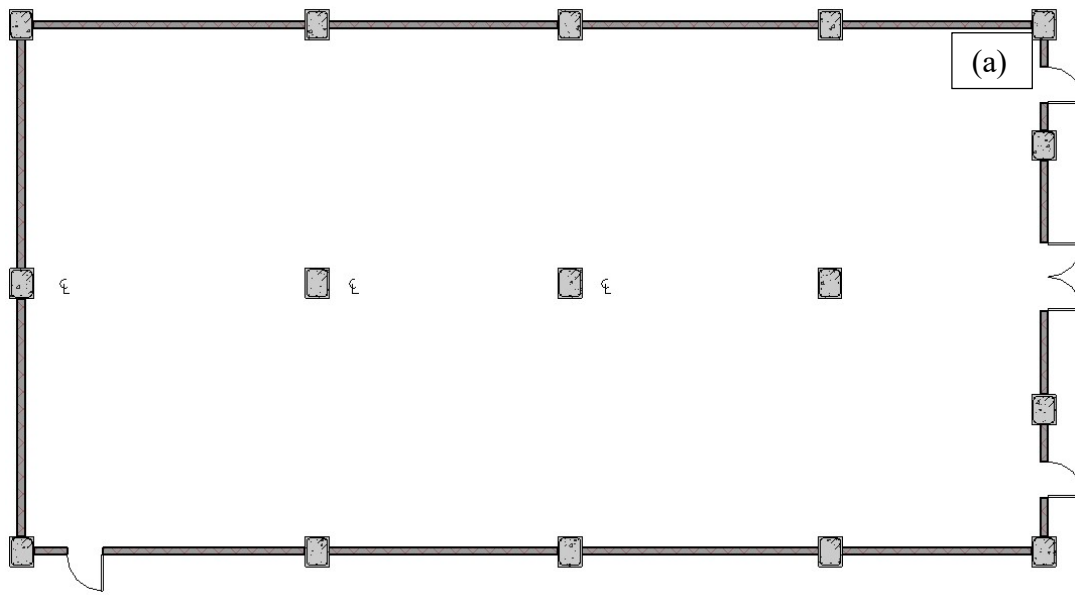
Figure 95 Floor plan for the virtual structure.
