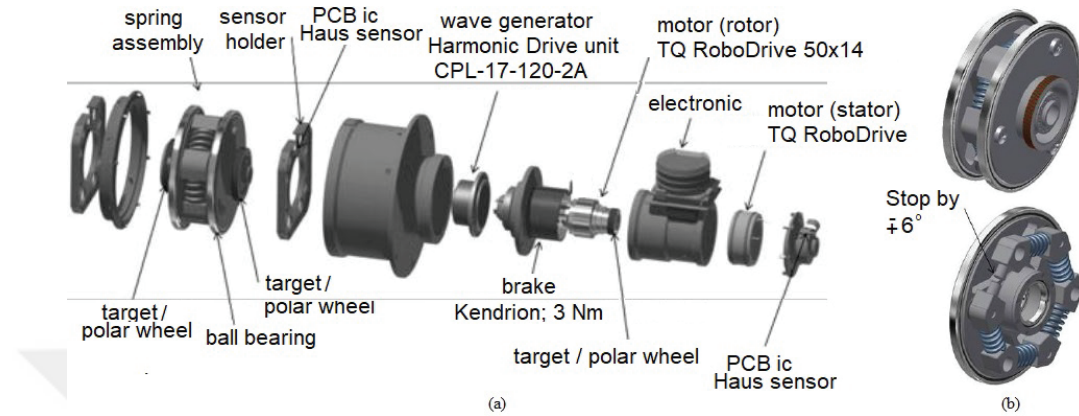
Figure 2.9. (a) Series elastic actuator type II: 50Nm, (b) Elastic element with coil springs (Source: Fernández et al., 2016)
