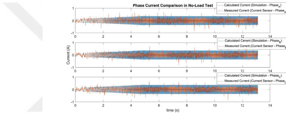
Figure B.1. Current comparison at no-load test - Simscape model
