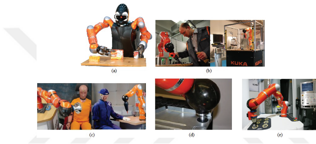
Figure 2.4. (a) DESIRE technology, (b) SMERobot's welding operation, (c) Safety demonstration of PHIRENDS, (d) Manufacturing scenario by placing rubber closures, (e) loading/unloading machine (Source: Bischoff et al., 2010)
