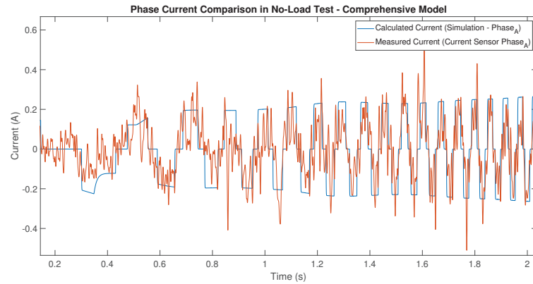
Figure 4.11. Comprehensive model in phase currents at no-load test on winding A
