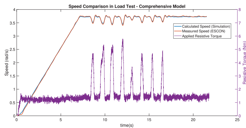
Figure 4.16. Comprehensive model speed results at load test
