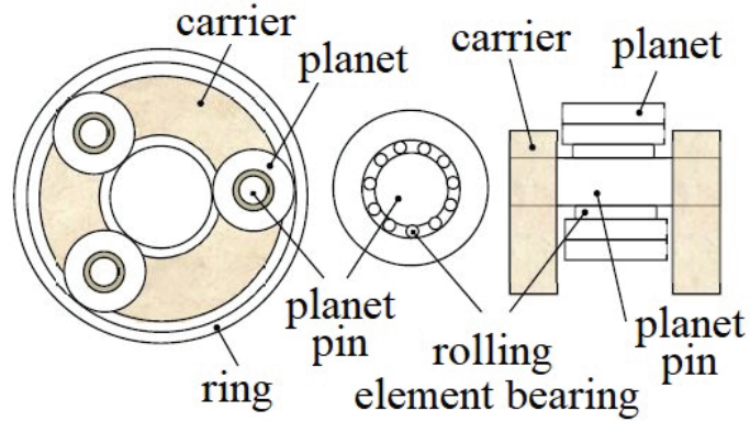
Figure 2.25. Components of the planetary gear set
