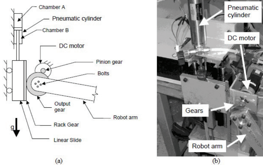
Figure 2.15. The hybrid actuator design (Source: Bone and Chen, 2012)
