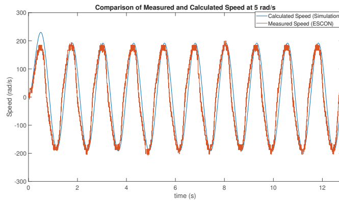
Figure C.14. Comparison of Measured and Theoretical Speed at 5 rad/s
