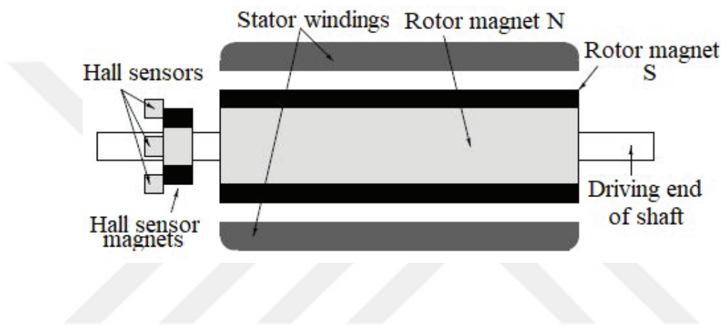
Figure 2.21. Cross-section of a BLDC motor
