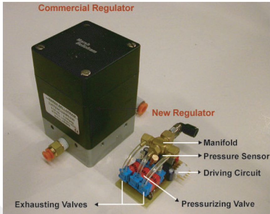
Figure 2.14. The pressure regulator (Source: Shin et al., 2008)
