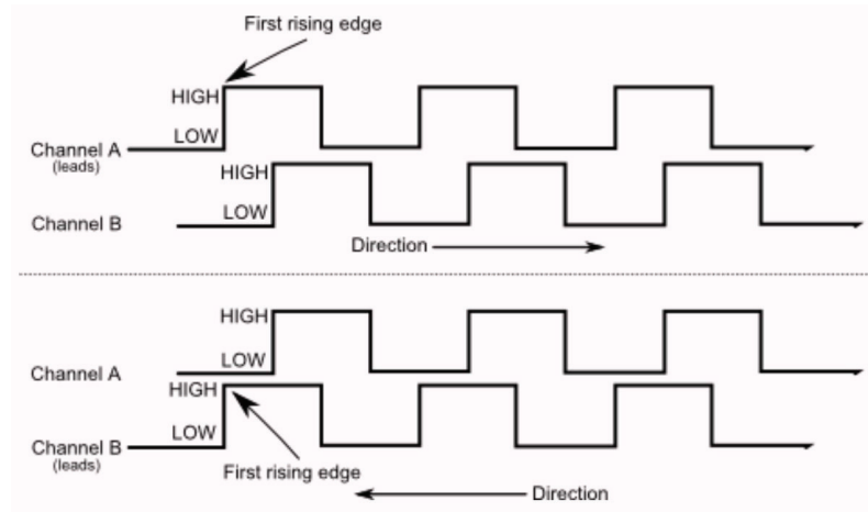
Figure 2.30. Quadrature Encoder
