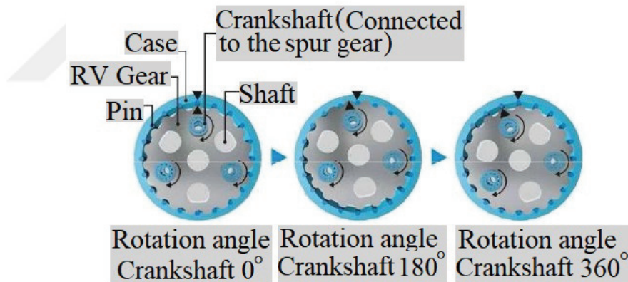
Figure 2.28. A cycloidal gear (Source: Nabstecco, 2018)
