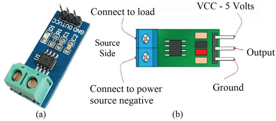
Figure 3.7. (a) The current sensor module, (b) Wiring diagram of the module (Source: Allegromicro, 2018)
