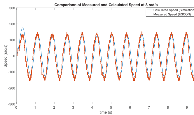
Figure C.15. Comparison of Measured and Theoretical Speed at 8 rad/s
