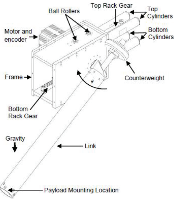
Figure 2.16. The rotary hybrid actuator (Source: Ashby and Bone, 2016)
