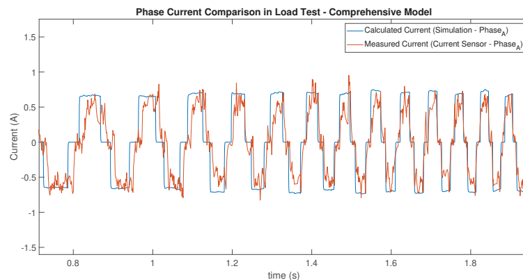
Figure 4.14. Comprehensive model in phase currents at load test on winding A
