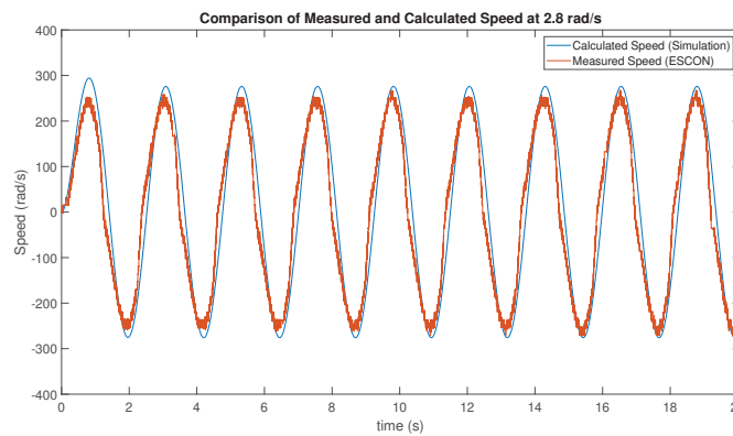
Figure C.9. Comparison of Measured and Theoretical Speed at 2.8 rad/s
