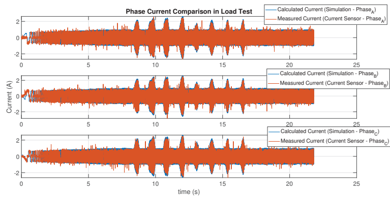
Figure B.4. Current comparison at load test - Comprehensive model
