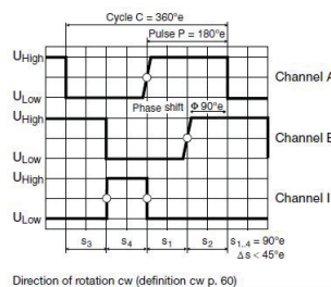
Encoder HEDL 5540 500 CPT, 3 Channels, with Line Driver RS 422
