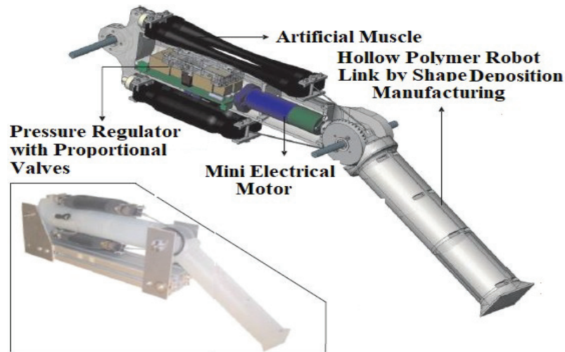
Figure 2.12. Developed DM2 actuator design (Source: Shin et al., 2010)
