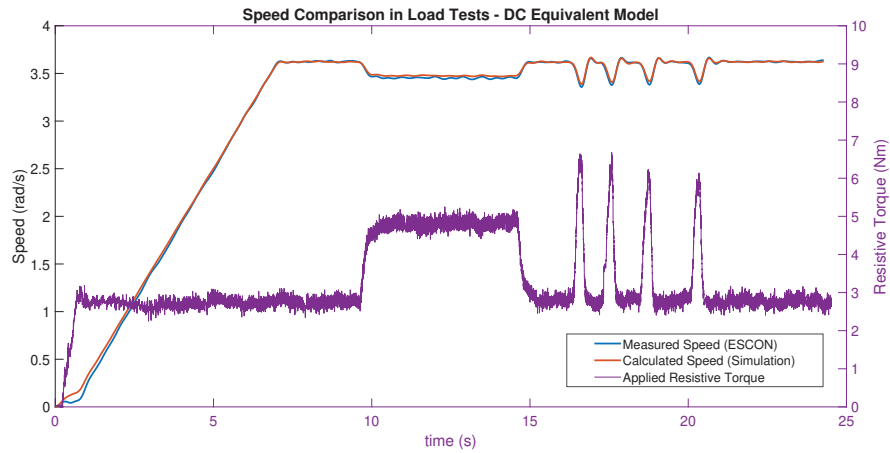
Figure 4.4. DC equivalent model speed results at load test
