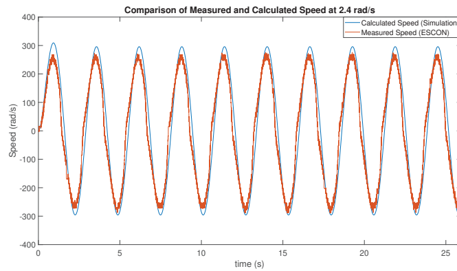
Figure C.8. Comparison of Measured and Theoretical Speed at 2.4 rad/s
