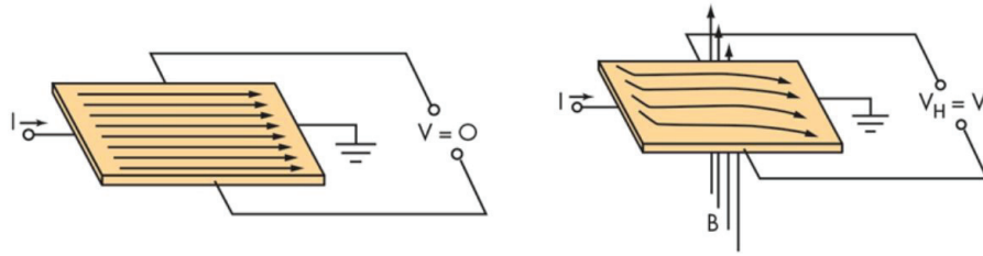
Figure 2.33. Hall voltage according to the magnetic field
