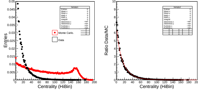
Figure 4.3. (Left) Centrality distribution of MC (red) and data (black) in PbPb collisions in the centrality interval 0-100%. (Right) Ratio between the centrality distribution of data and MC fitted with an exponential function. tributions with using the following function:
