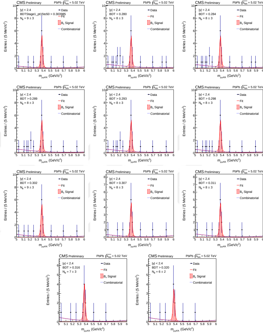
Figure 4.52. Scanning of BDT cut value and the summary plots of resulting mass spectrum fitting for PbPb data. The 1st spectrum on the top left is obtained with using nominal analysis value BDT = 0.30 . The following spectra have the BDT cut value varied from 0.28 increasingly to 0.32.
