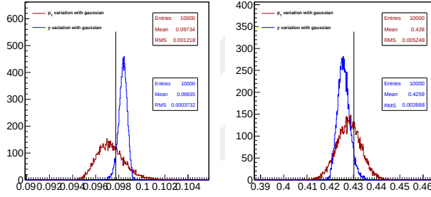
Figure 4.30. Varied acceptance distribution from toy pp MC determined by p_T and rapidity distribution fitting. The red color refers to p_T distribution while blue one is rapidity. The left plot corresponds the B_s^0 p_T 7 to 15 GeV/c and the right one is for 15 to 50 GeV/c. The black line in the middle shows the nominal acceptance value in the analysis.
