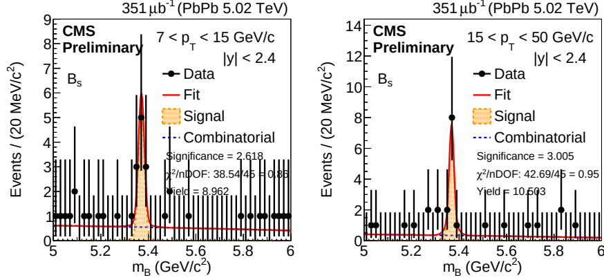
Figure 4.10. Invariant mass distribution and fit of B_s^0 candidates obtained in PbPb collisions in the p_T interval between 7 to 15 \text{GeV}/c and 15 to 50 \text{GeV}/c .
