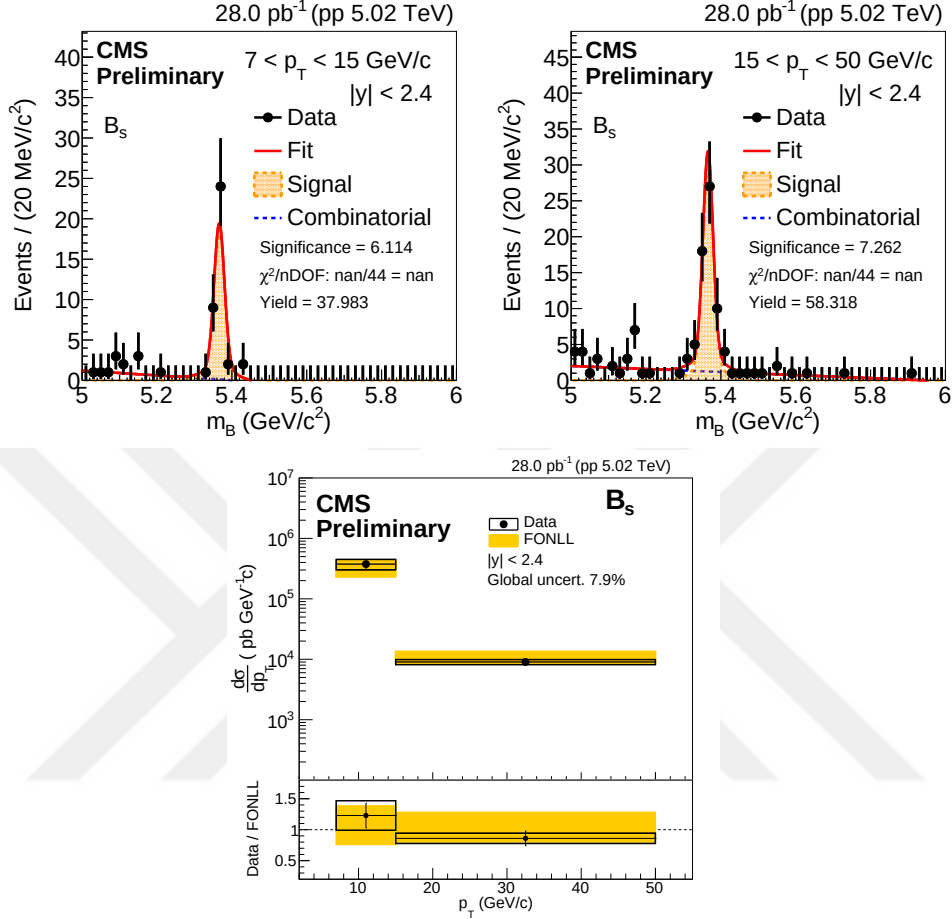
Figure 4.26. The top panels show the B_s^0 invariant mass spectra for p_T interval 7 to 15 \text{GeV}/c (left) and for 15 to 50 \text{GeV}/c (right). The bottom panel refers to the corresponding cross section using the PbPb trained BDT discriminant for p_T interval 7 to 50 \text{GeV}/c in pp data.
