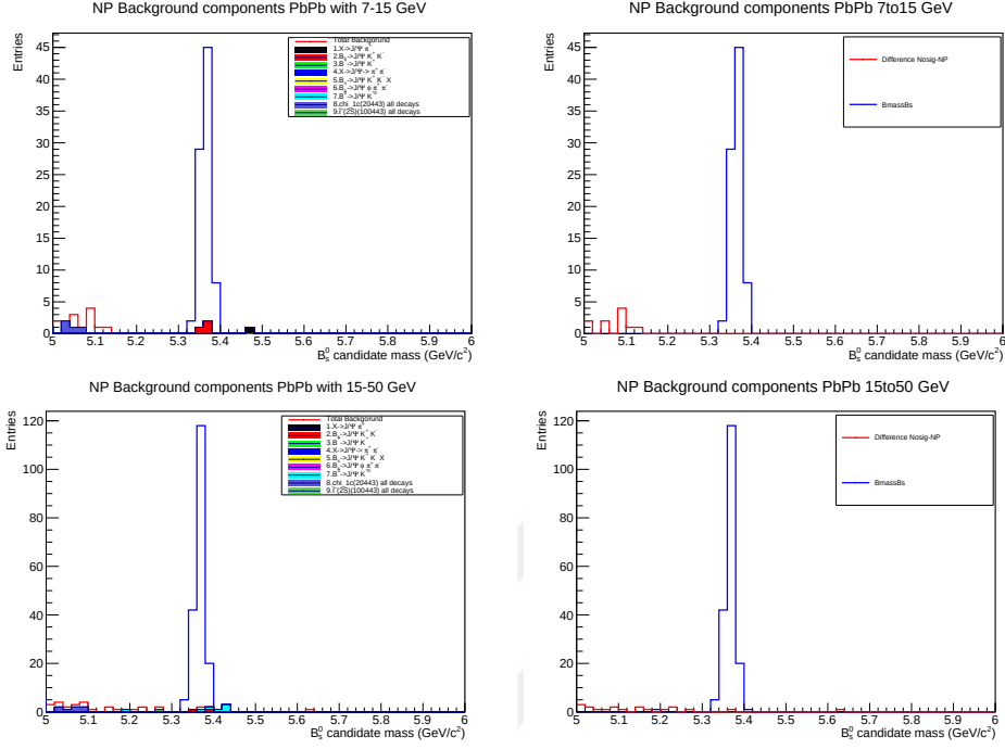
Figure 4.39. Contribution of the Individual Non Prompt Background components produced in different p_T range 7 to 15 GeV/c and 15 to 50 GeV/c for PbPb and comparison of differences of sum of determined channels from total background with B_s^0 signal after optimal cuts.
