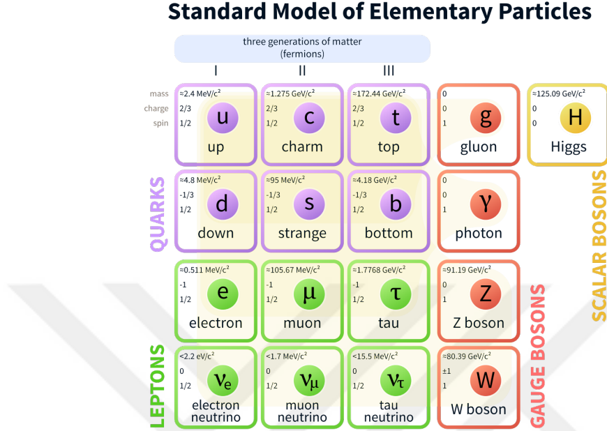
Figure 2.1. The particle content of the SM (Wiki, 2018)
