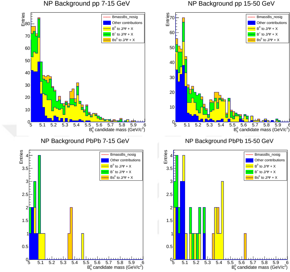
Figure 4.42. B^+ , B_s^0 , B^0 channels make nearly equal contribution in the signal region for 7 to 15 GeV/c and 15 to 50 GeV/c with pp (upper plots) after applying optimal cuts. In terms of PbPb samples, for 7 to 15 GeV/c p_T range B_s^0 to J/\psi + X (orange region) is the most contributed channel in the signal region but in 15 to 50 GeV/c p_T range, both B_s^0 and B^0 make big contribution.
