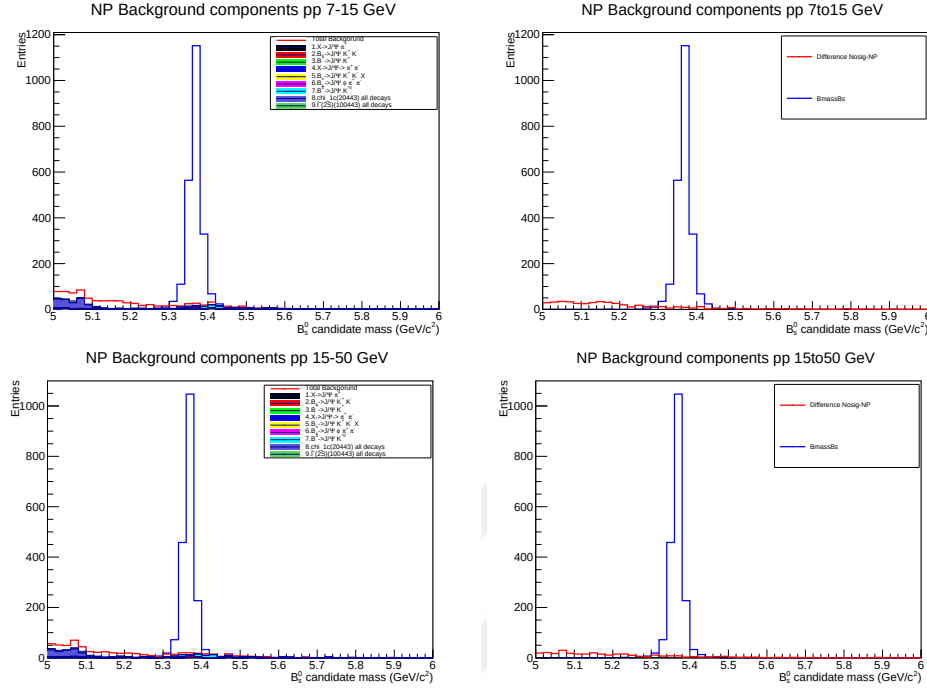
Figure 4.37. Contribution of the Individual Non Prompt Background components produced in different p_T range from 7 to 15 and 15 to 50 GeV/c for pp after optimal cuts. The blue line refers to the B_s^0 signal peak while others are the same as the above plots (top and bottom left plots). The difference of sum of the channel from total background referred with red line with respect to signal (top and bottom right plots).
