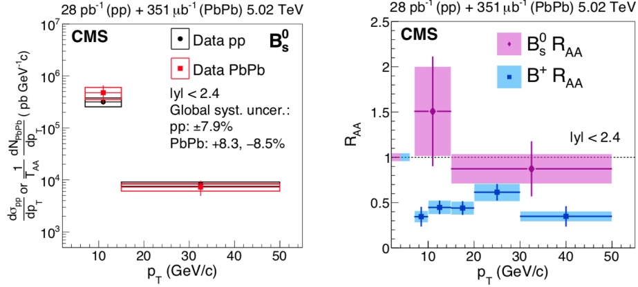
Figure 4.23. The B_s^0 R_{AA} results. The left plot shows the p_T differential production cross section of B_s^0 in pp collisions and the p_T differential corrected yield of B_s^0 scaled by T_{AA} in PbPb collisions at \sqrt{s}=5.02 TeV in two p_T intervals from 7 to 50 GeV/c. The vertical bars indicate statistical (systematic) uncertainties. The systematic uncertainty boxes contain both the correlated and uncorrelated contributions added in quadrature. The global systematic uncertainty includes the uncertainties in T_{AA} , N_{MB} , and B_s^0 . The right plot describes the nuclear modification factor R_{AA} of B_s^0 measured in PbPb collisions at \sqrt{s}=5.02 TeV from 7 to 50 GeV/c. The vertical boxes correspond to statistical (systematic) uncertainties. The global systematic uncertainty, shown as a grey box at R_{AA} = 1 , contains the uncertainties in the integrated luminosity measurement and T_{AA} value.
