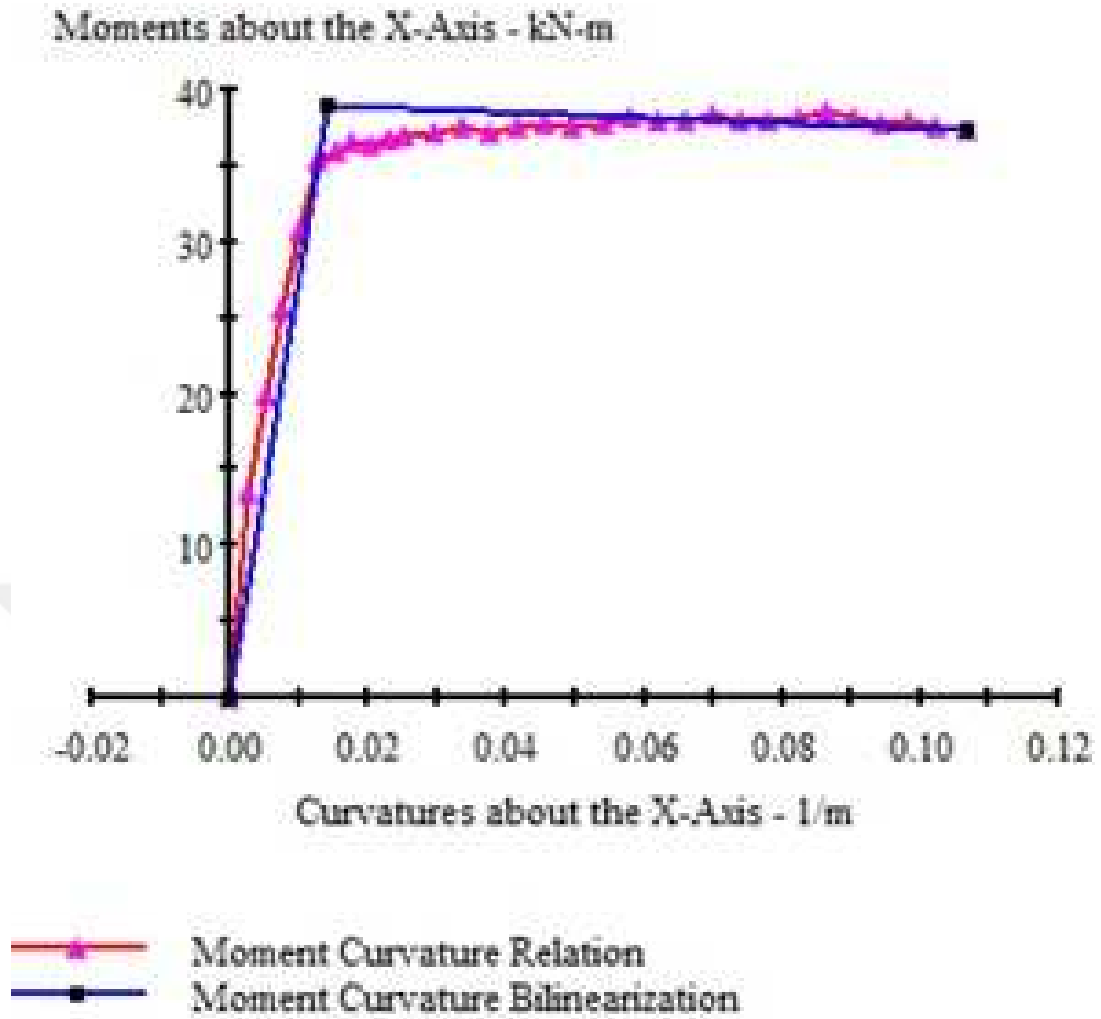
Figure 6.6: Positive moment-curvature relation of asymmetrically reinforced section (top section)
