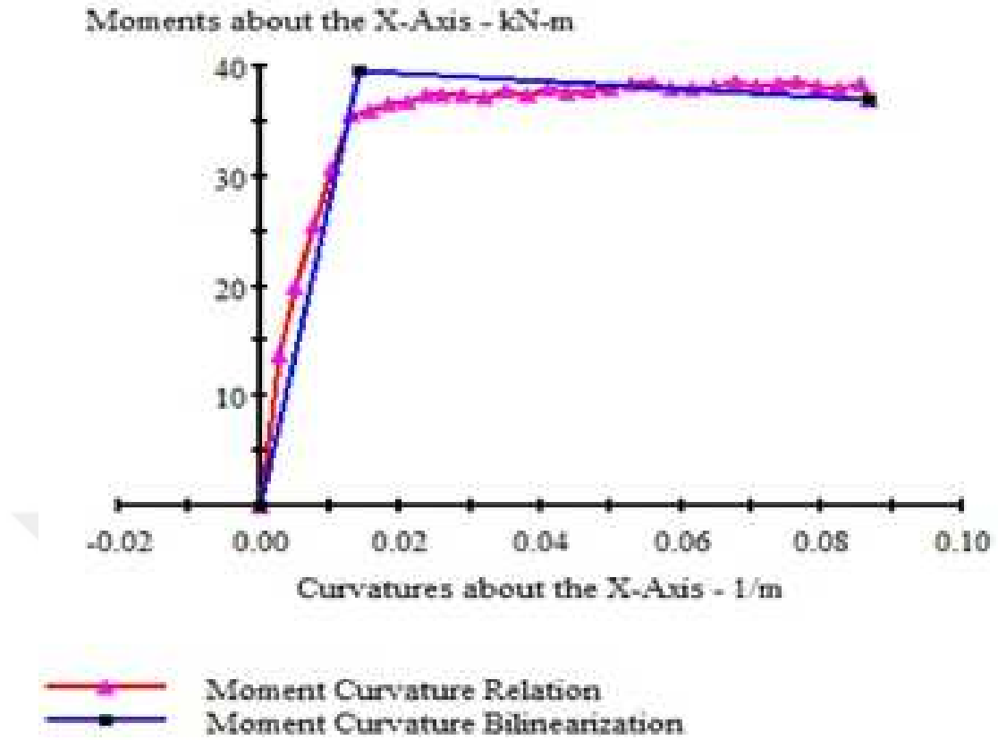
Figure 6.7: Positive and negative moment-curvature relation of symmetrically reinforced section (bottom section)
