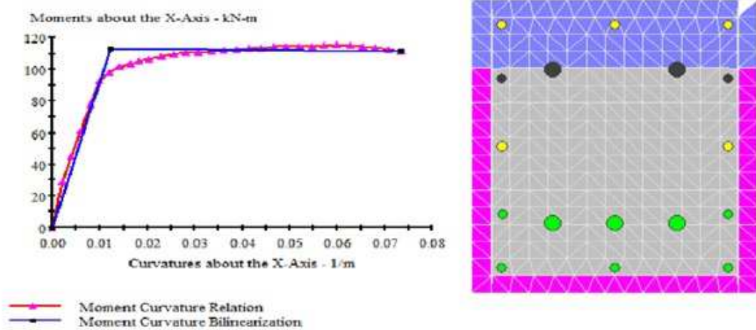
Figure 6.19: Negative moment-curvature relationship of asymmetrically reinforced section and the section after analysis
