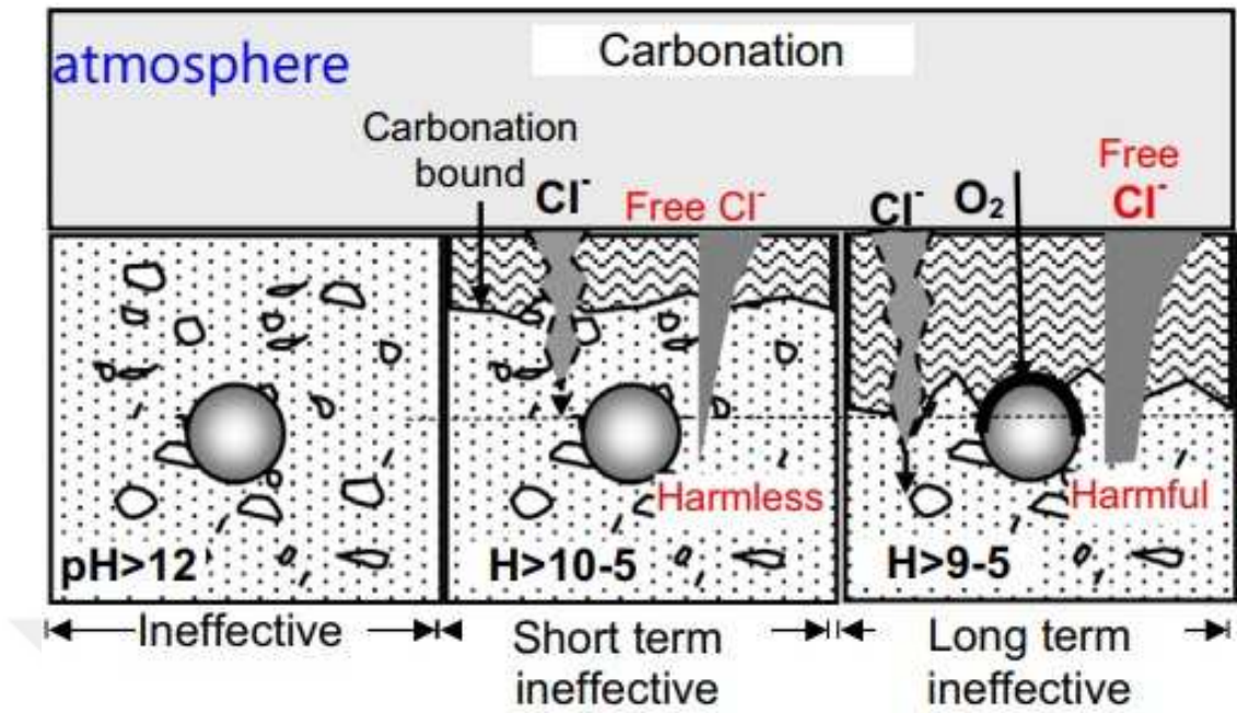
Figure 2.2: Carbonation (Dogan (2015) [2])
