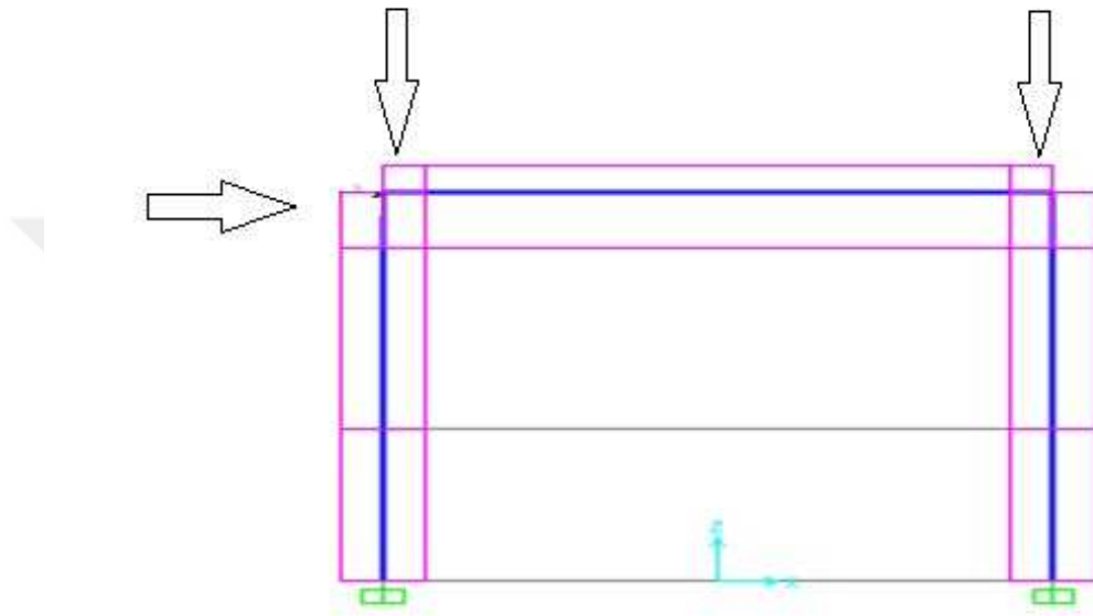
Figure 5.15: Frame model in Sap2000
