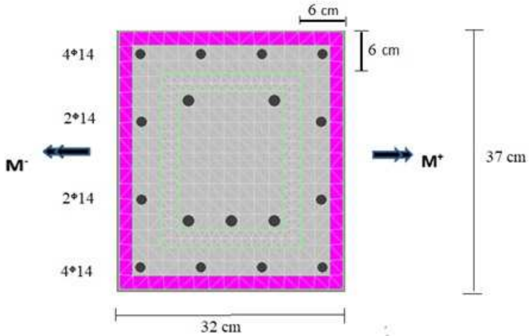
Figure 6.21: View of the cross section in Xtract
