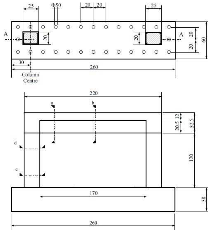
Figure 3.2: Geometry of the 15 years old frame
