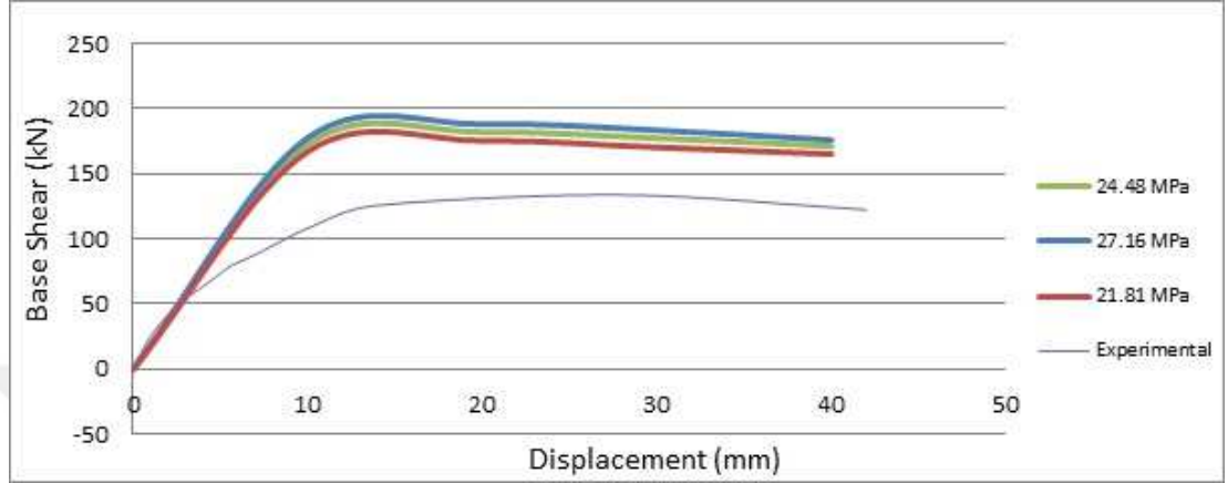
Figure 5.20: Comparison of experimental and analytical base shear top displacement curves for different compressive strength of concrete obtained by SeismoStruct
