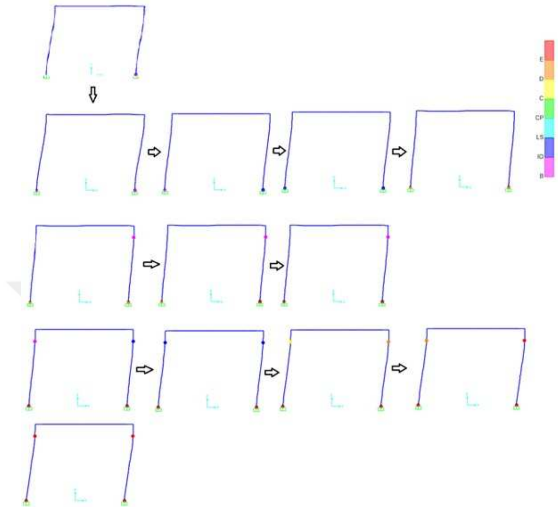
Figure 5.18: Plastic hinge formation for the frame
