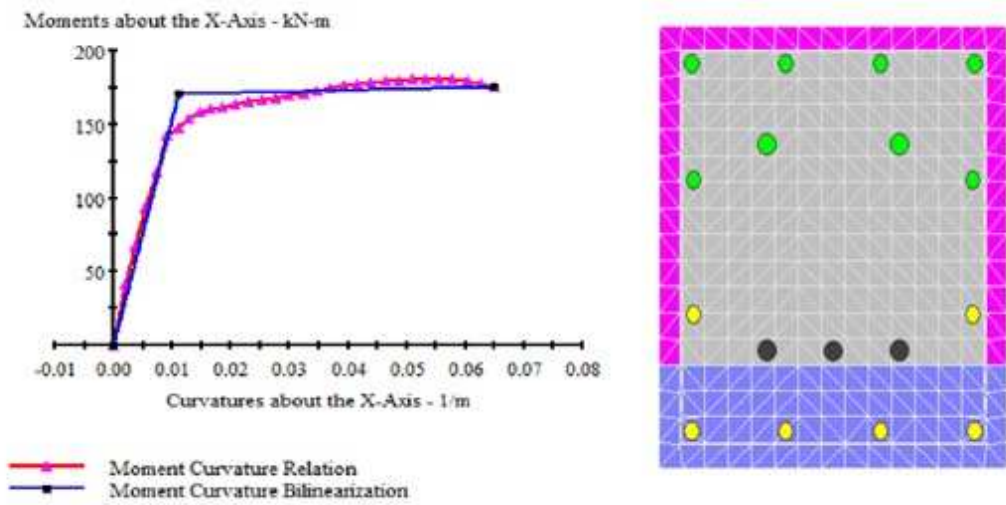
Figure 6.26: Positive moment-curvature relationship of asymmetrically reinforced section and the view of the section after analysis
