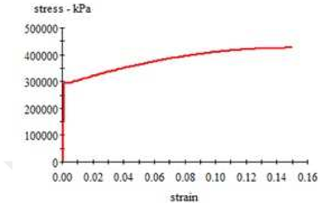
Figure 6.4: Stress-Strain relationship for steel
