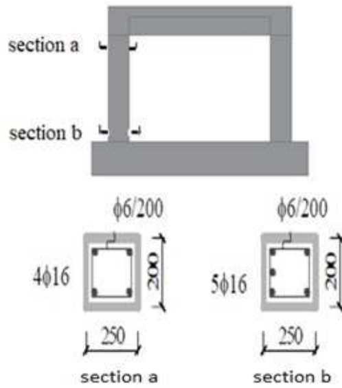
Figure 6.8: Column Sections
