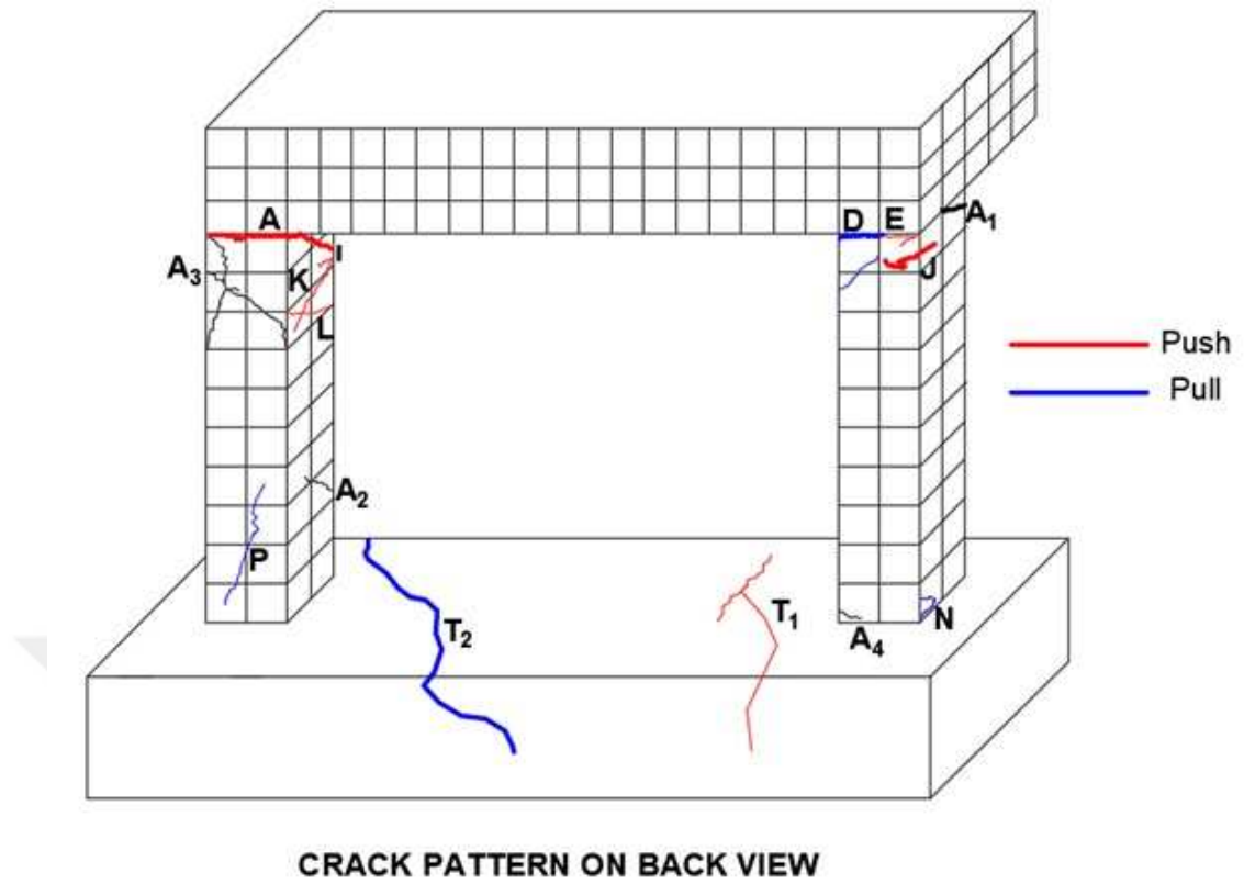
Figure 4.4: Crack pattern on back view of the specimen at the end of the experiment
