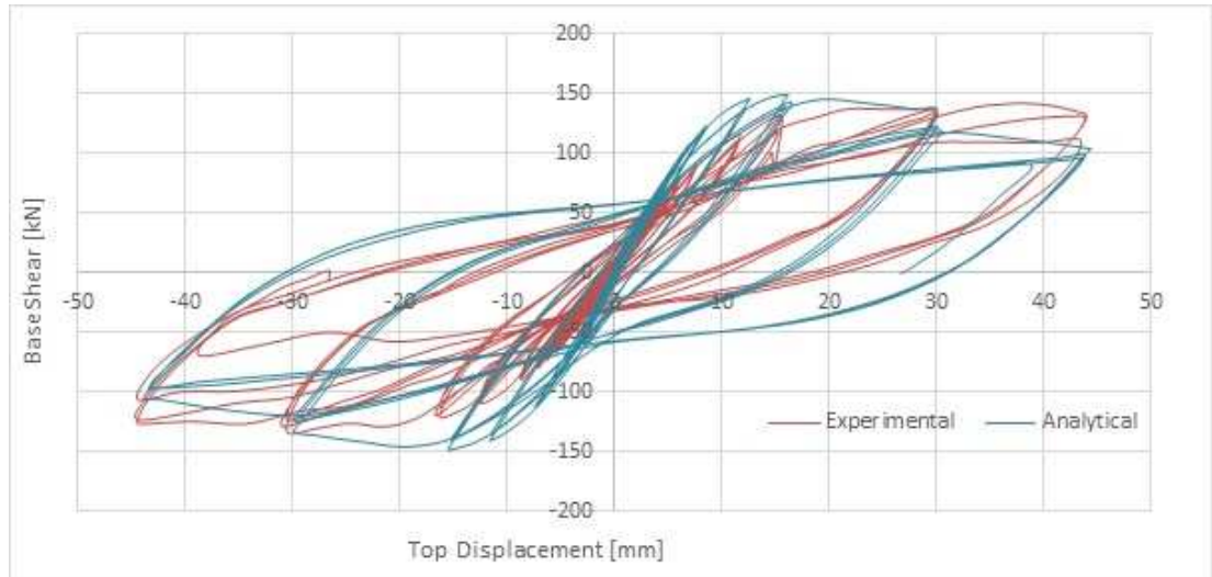
Figure 5.21: Comparison of experimental hysteretic curve and analytical hysteretic curve for compressive strength of 21.81\text{MPa} of concrete obtained by SeismoStruct
