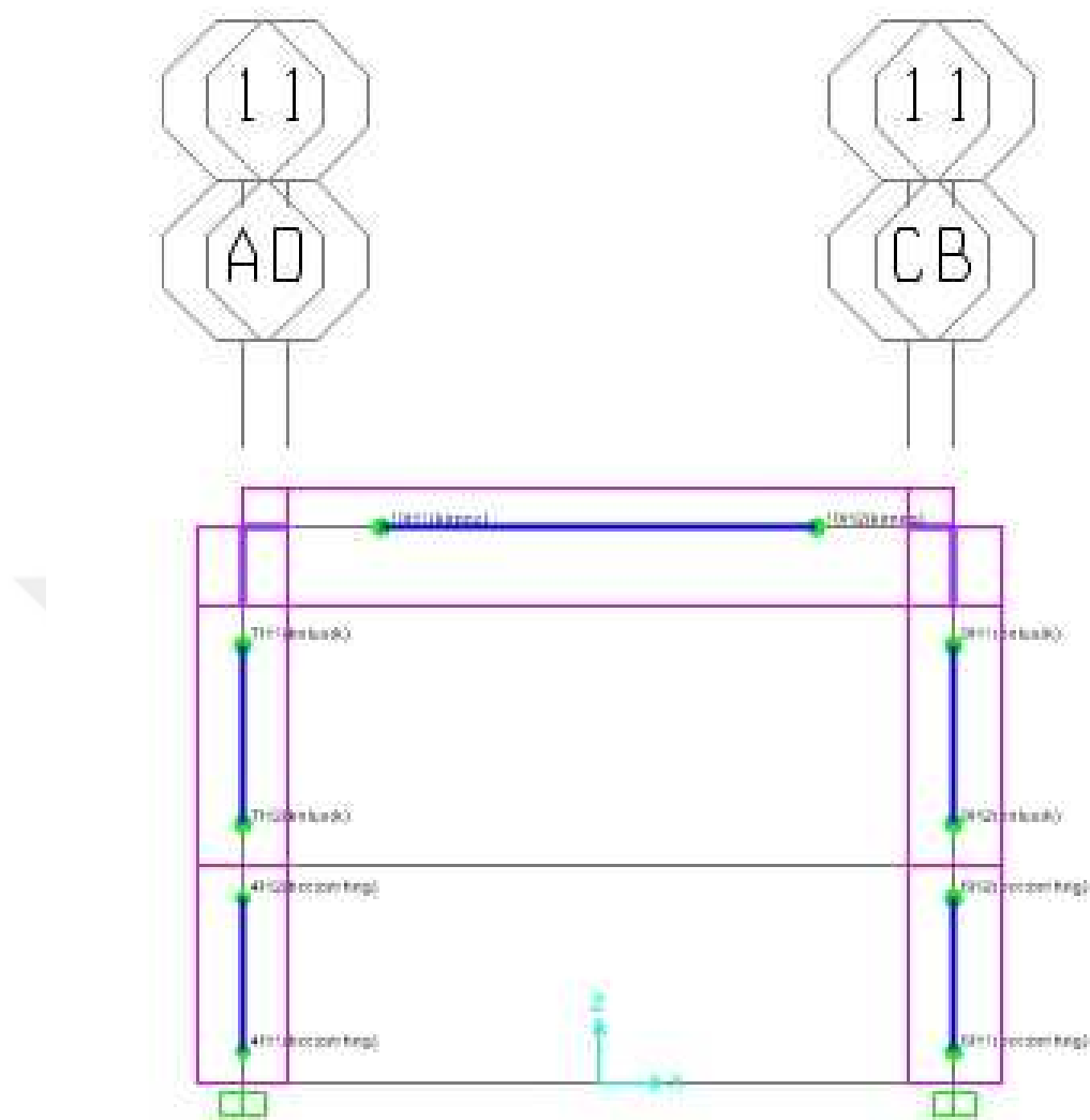
Figure 5.16: Definition of hinges in SAP2000
