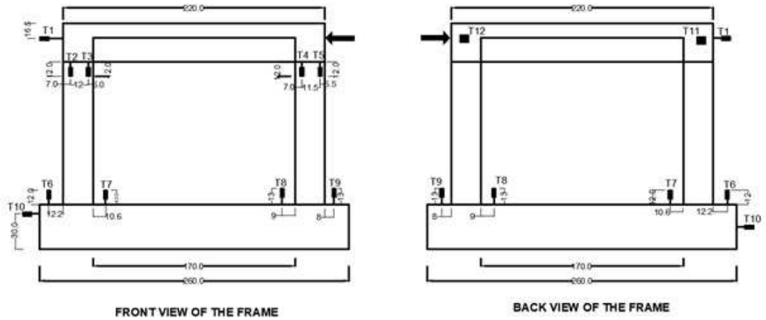
Figure 3.5: Locations of LVDTs
