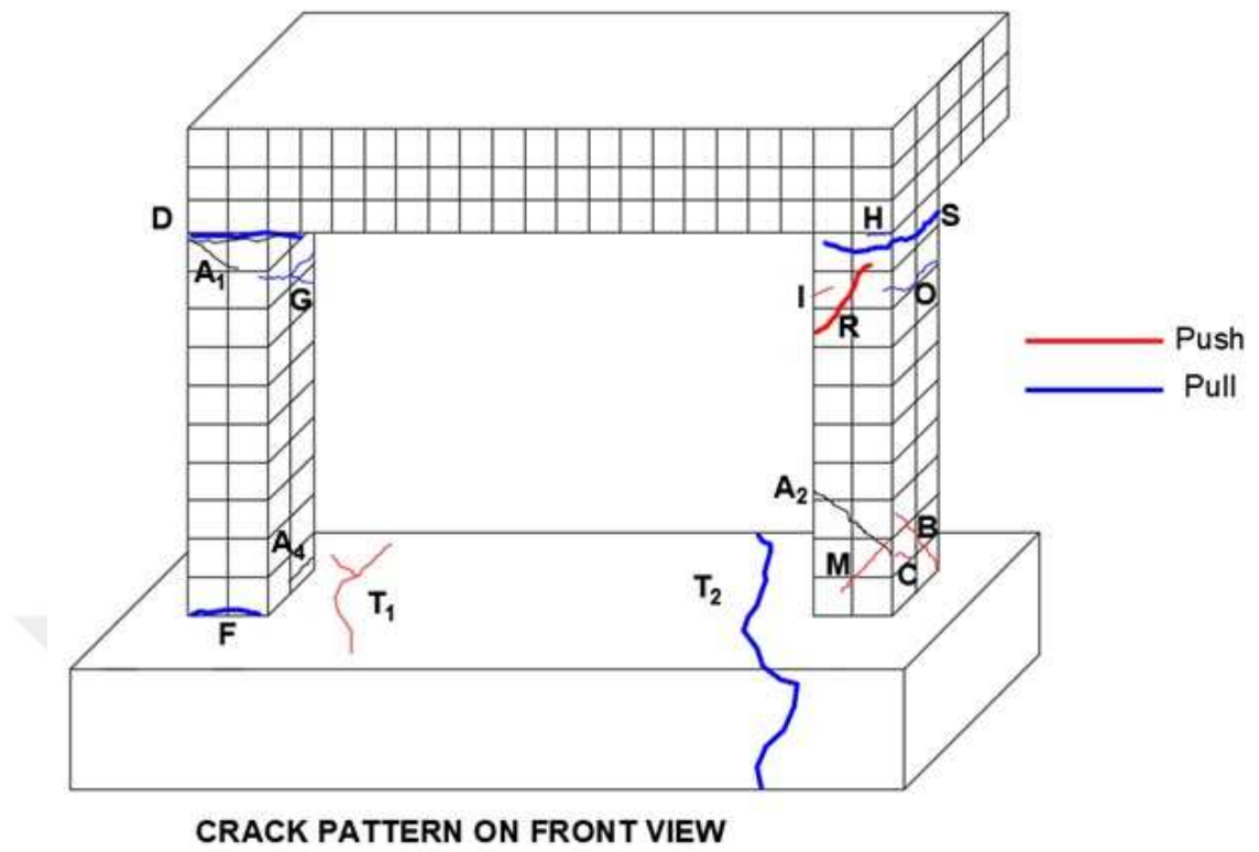
Figure 4.3: Crack pattern on front view of the specimen at the end of the experiment
