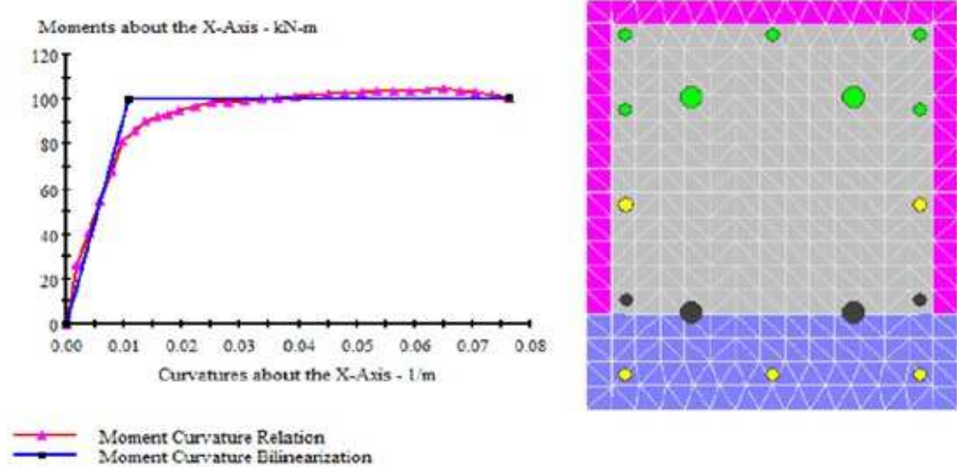
Figure 6.20: Negative and positive moment-curvature relationship of symmetrically reinforced section and the view of the section after analysis
