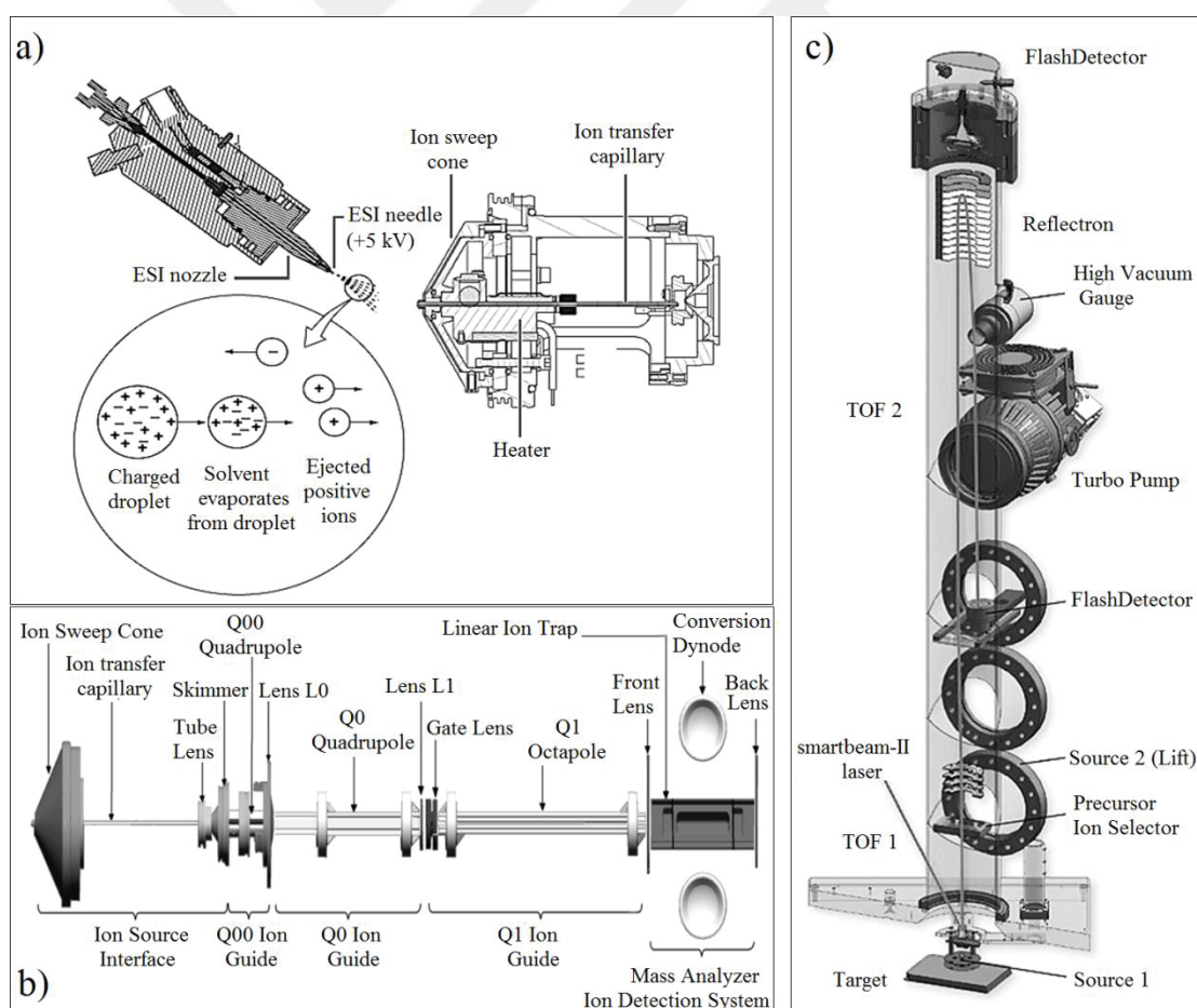
Figure 1.2. Schematic diagram of mass spectrometers used in this study. a) Electrospray b) Internal components of MS detector with the ion path units of LTQ XL TM ESI-Linear Ion Trap MS launched by ThermoFisher Scientific, c) Ion path units of Autoflex MALDI-TOF/TOF MS launched by Bruker Daltonics
