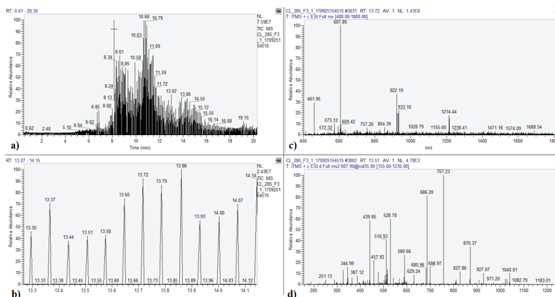
Figure 1.3. Outputs in automatic LC-MS/MS analysis with data-dependent acquisition. a and b) Mass chromatograms, c) MS Spectrum, d) MS/MS Spectrum
