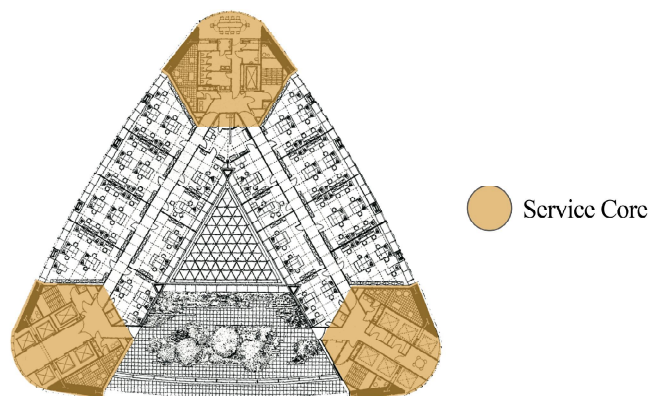
Figure 2.16. Commerzbank Tower, floor plan (Foster+Partners, 1997)
