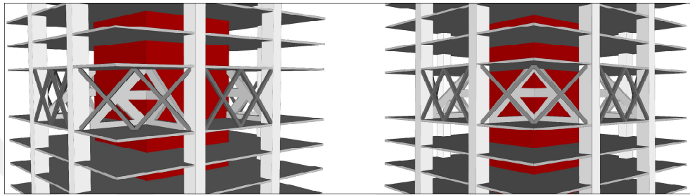
Figure 3.14. Outrigger levels with belt trusses
