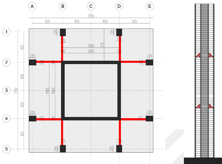
Figure 3.7. Typical floor plan (left) and elevation (right) of "primary core building" with outriggered frame system
