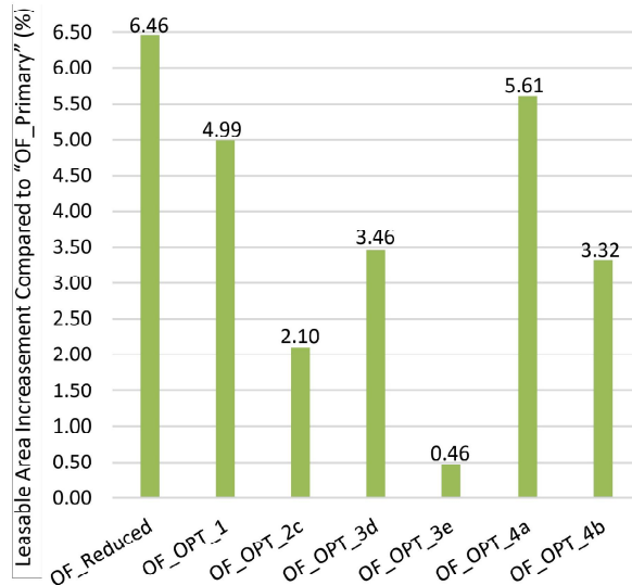
Figure 4.3. Leasable increase of outriggered frame buildings compared to “OF_Primary”
