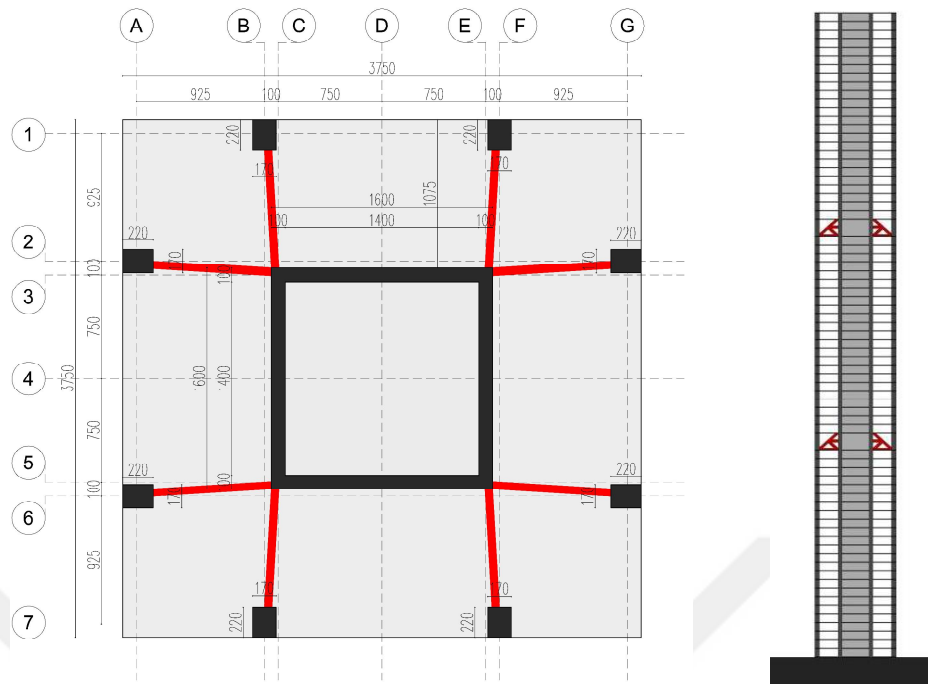
Figure 3.8. Typical floor plan (left) and elevation (right) of "reduced core building" with outrigger frame system
