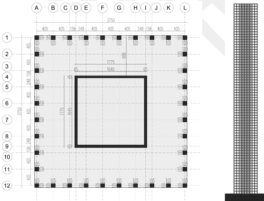
Figure 3.9. Typical floor plan (left) and elevation (right) of "primary core building" with framed-tube system
