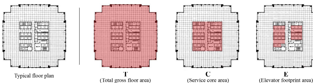
Figure 3.4. Demonstration of “T, C and E” on typical floor plan of One Liberty Place
