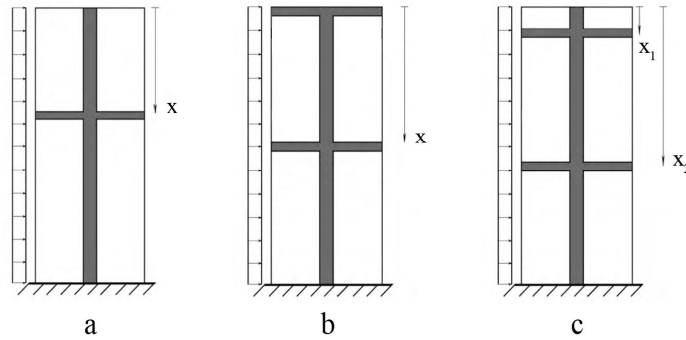
Figure 2.7. Location of outriggers (Günel and Ilgın, 2014)
