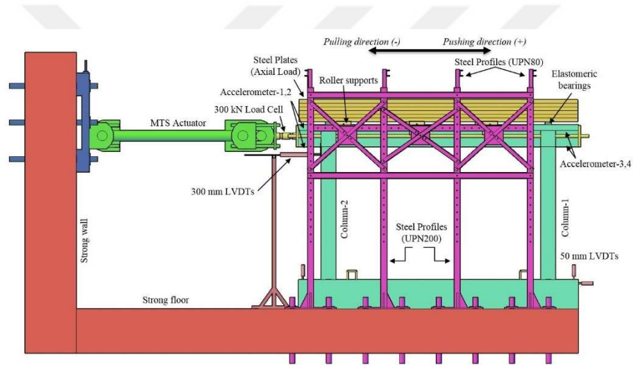
Figure 3.40. Left view of frame test setup
