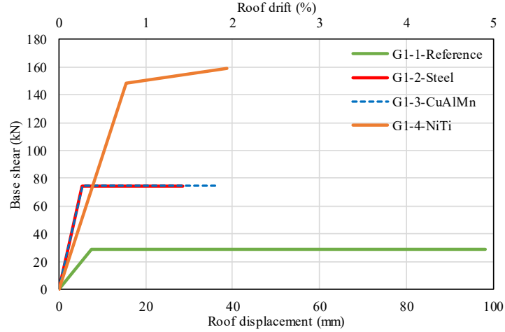
Figure 5.12. Comparison of idealized curves
