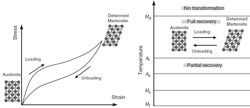
Figure 2.2. Superelastic effect (Ozbulut, Hurlebaus and Desroches, 2011, p. 1533)
