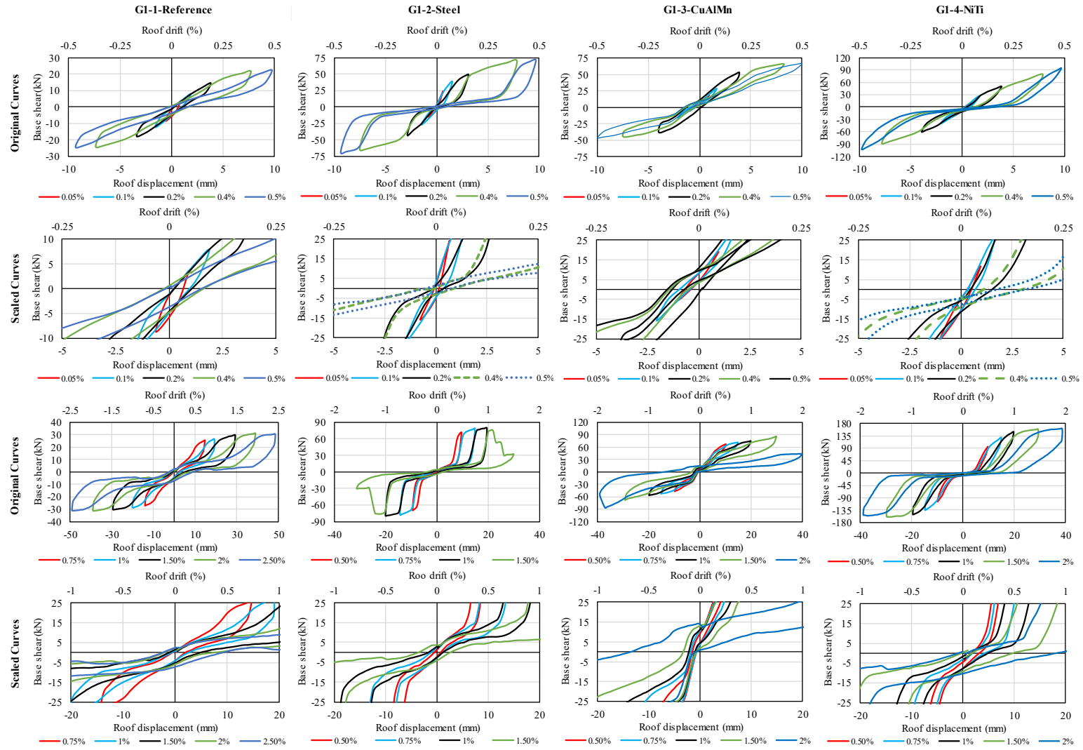
Figure 5.17. Comparison of hysyteretic curves in re-centering property
