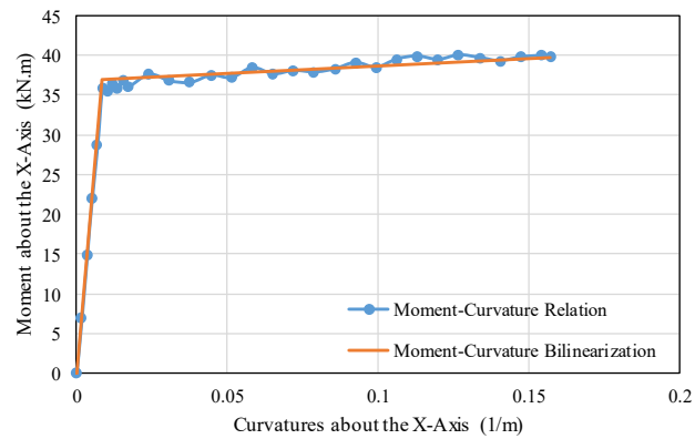
Figure 3.5. Moment-curvature analysis of the beam section
