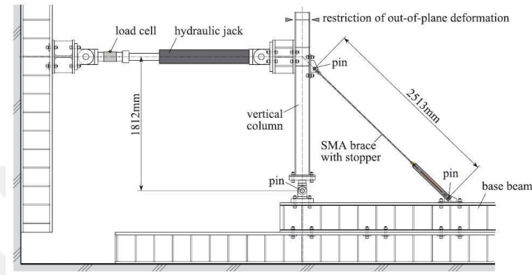
Figure 2.11. An experimental system (Araki et al., 2015)
