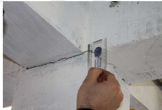
(b) A crack measuring at -1% drift ratio
