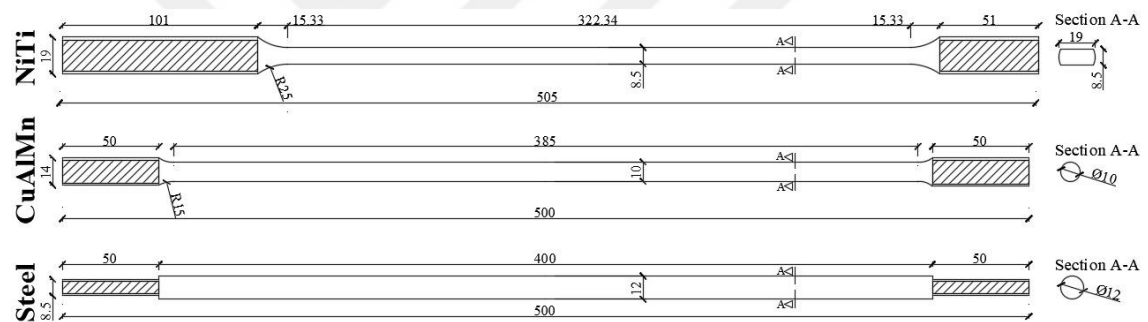
Figure 3.10. Sectional properties of strengthening bars (Units are in mm)
