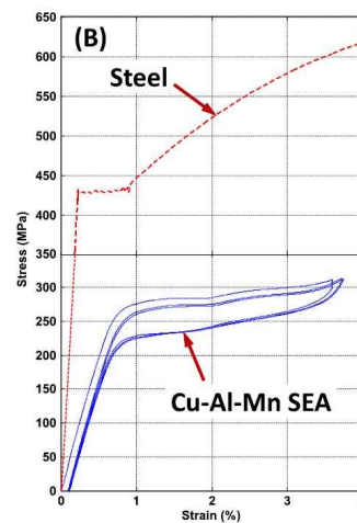
(b) Stress-strain relations and comparison with steel reinforcement
