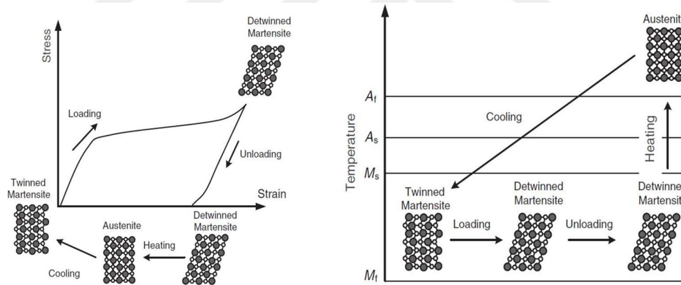
Figure 2.1. Shape memory effect (Ozbulut, Hurlbaums and Desroches, 2011, p. 1533)
