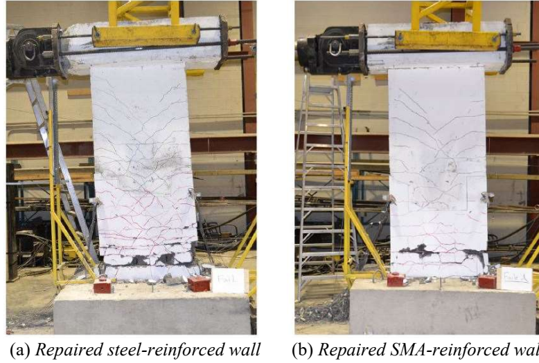
Figure 2.10. Condition of walls at the end of testing (Cortés-Puentes et al. 2018)
