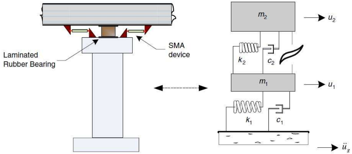
Figure 2.8. Model of an isolated bridge with an SMA/rubber isolation system (Ozbulut and Hurlebaus, 2010)
