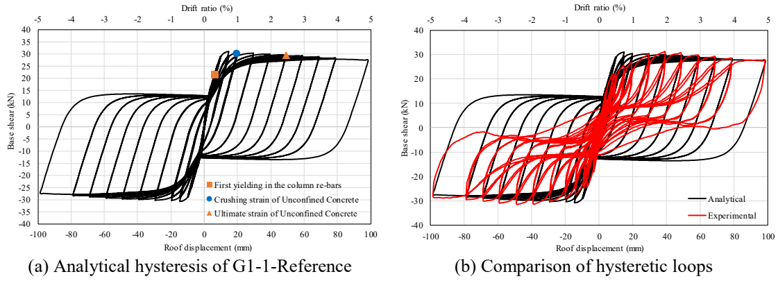
Figure 6.6. Hysteretic behavior of G1-1-Reference
