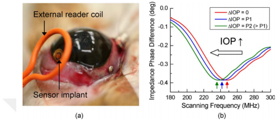
Figure 1.3. (a) Experimental setup for in vivo pressure sensing test (rabbit), (b) measured phase-dip curves [41].
