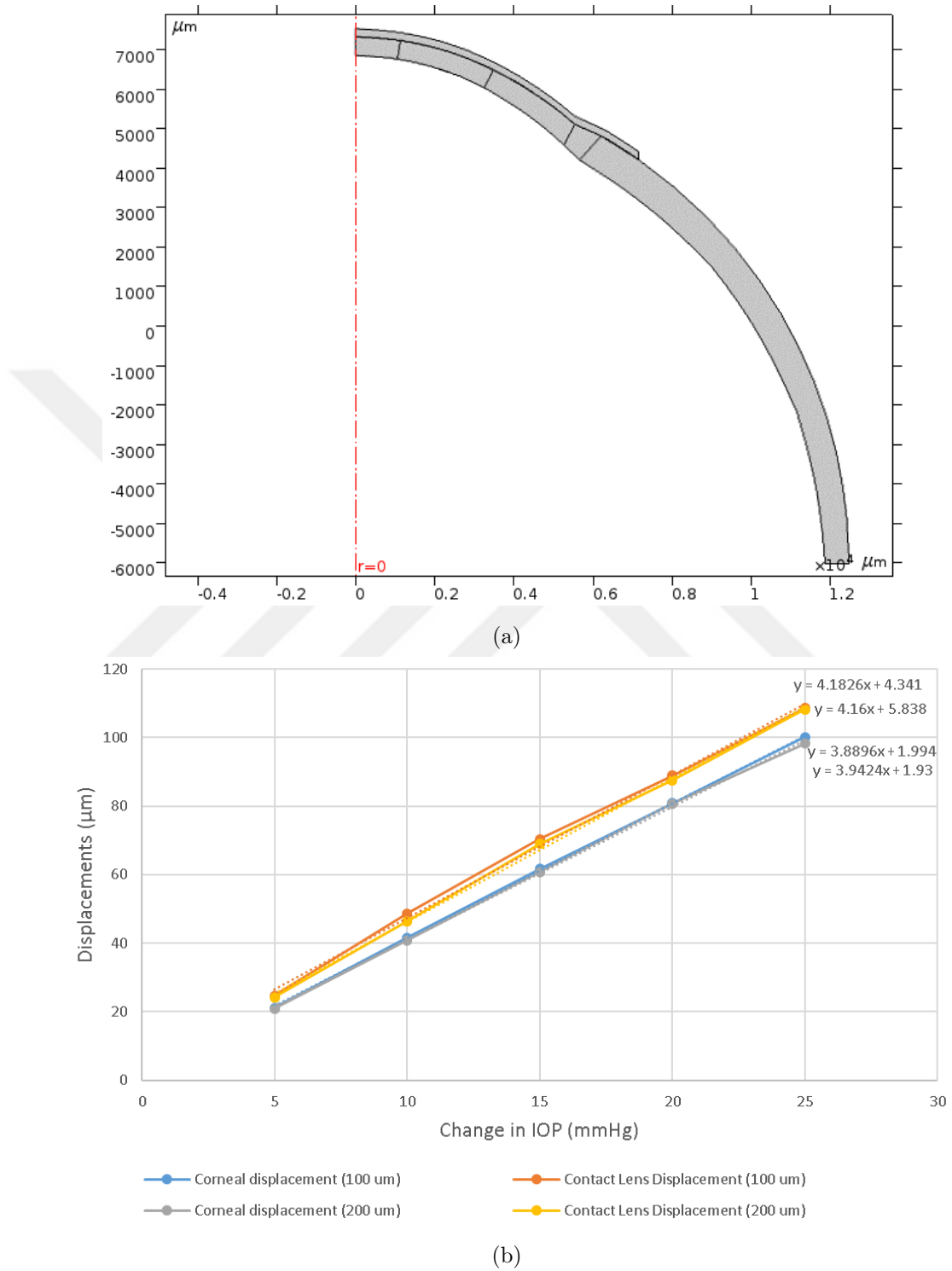
Figure 2.8. (a) Computational model including an eyeball and a CL, (b) maximum displacement values for CLs with thicknesses of 100 \mu\text{m} and 200 \mu\text{m} with respect to changes in IOP levels.
