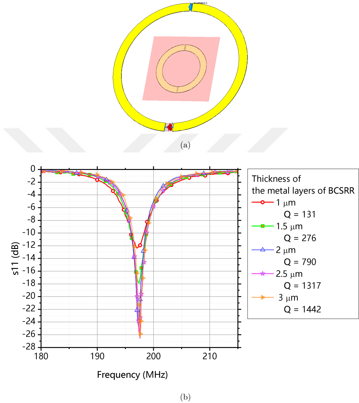
Figure 4.5. (a) Illustration of the simulated folded dipole antenna and BC-SRR embedded in the PI substrate. (b) Simulated s_{11} spectra with respect to varying values of thicknesses of the metal layers of BC-SRR.
