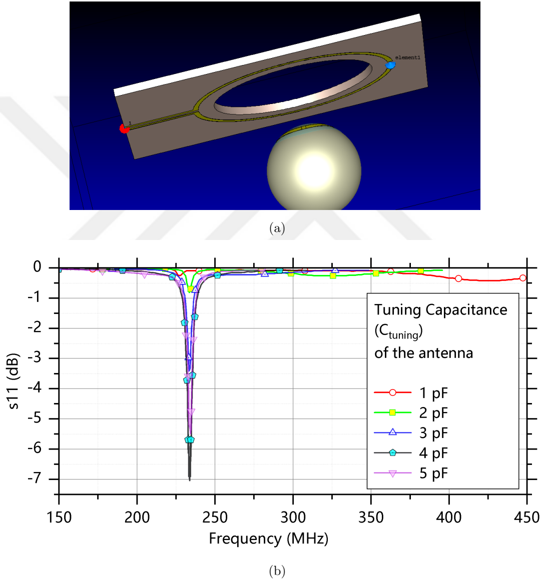
Figure 4.9. (a) Illustration of the simulated folded dipole antenna with the BC-SRR based CLS placed on the eye-globe material. (b) Simulated s_{11} behavior of the system with respect to varying values of C_{\text{tuning}} (pF).
