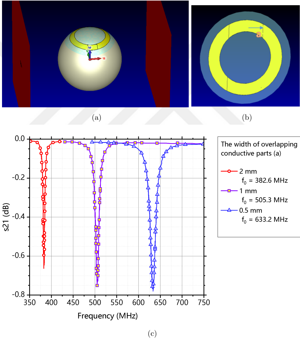
Figure 4.7. (a) Illustration of the simulated sensor bent on eye-globe material, (b) Detailed illustration of the planar sensor showing defined a and (c) Simulated s_{21} spectra for varying a (mm).
