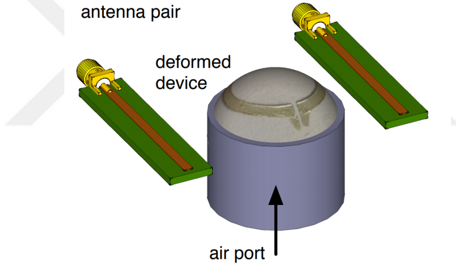
Figure 1.6. An illustration of the experimental setup for the SRR sensor realized on flexible latex rubber [44].
