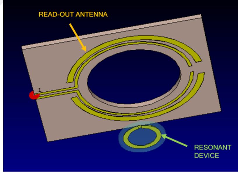
Figure 4.1. Illustration of the simulated folded dipole antenna coupled BC-SRR embedded in PDMS.
