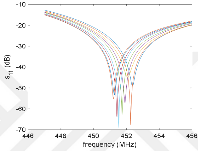
Figure B.1. Measured s_{11} spectra for trial 1 showing the resonant frequencies with respect to varying values of IOP levels.
