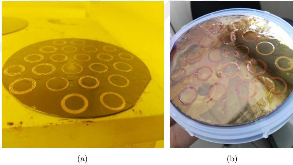
Figure 5.2. (a) Soft baking of the last spin coated PI layer. (b) Photograph of the hard-baked wafer.
