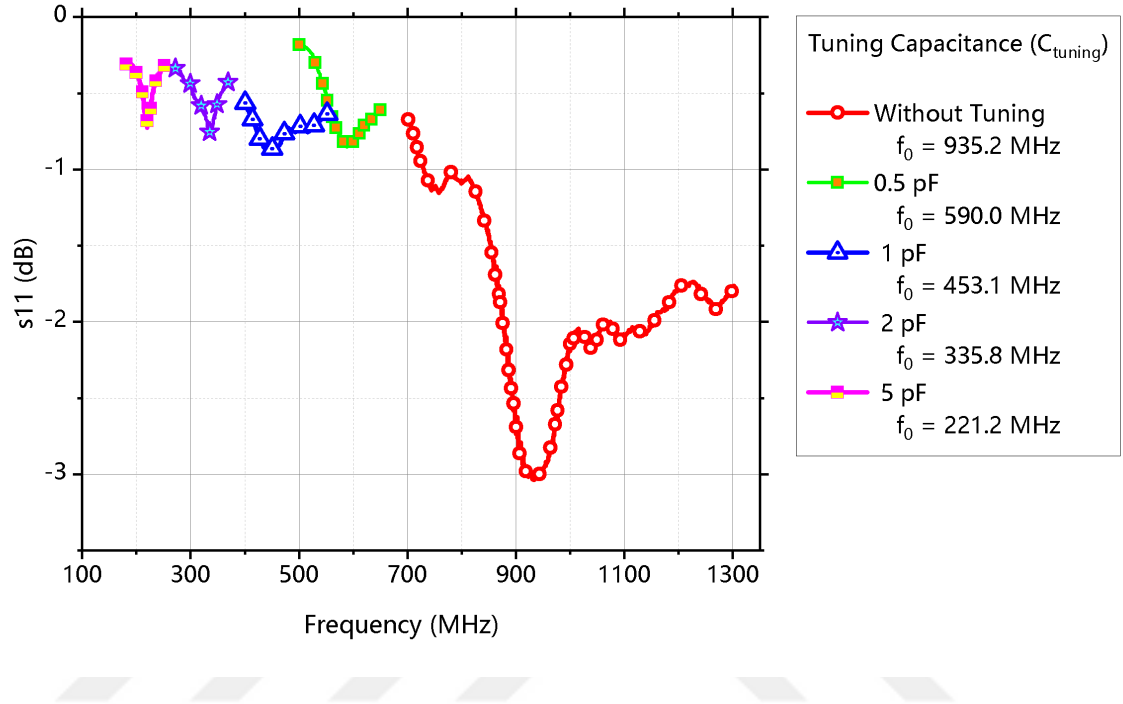
Figure 3.3. Measured s_{11} spectra of the folded dipole antenna with respect to varying values of the C_{\text{tuning}} .
