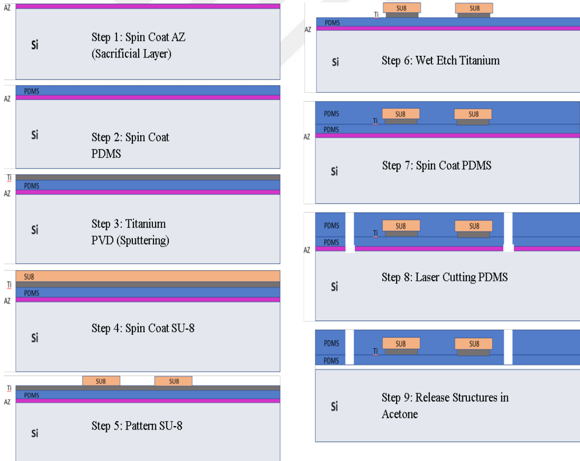
Figure 2.13. SRR embedded in PDMS fabrication process flow.
