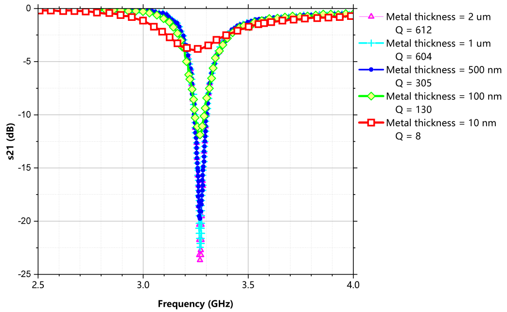
Figure 2.4. (a) Simulation model and (b) s_{21} spectra of simulated model for various thicknesses of gold.
