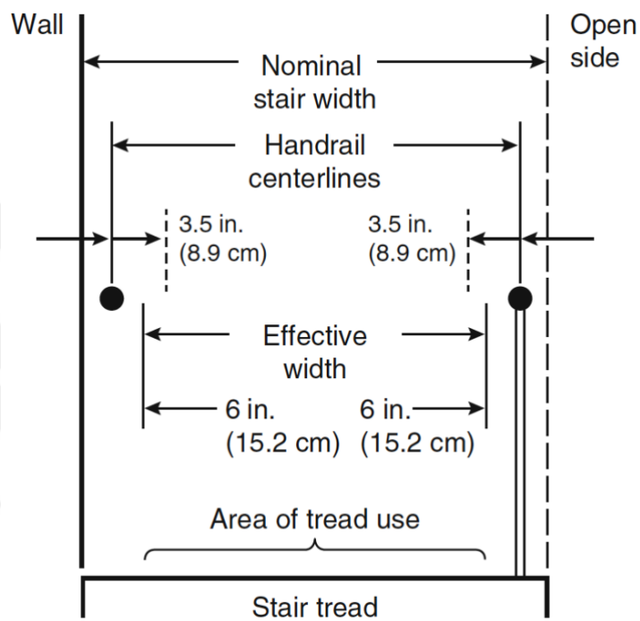
Figure 2.14. The effective width of stairs in relation to walls and handrails (Gwynne et al. , 2016).
