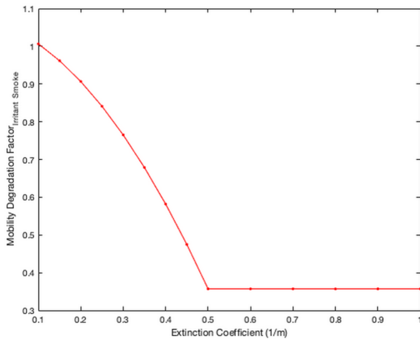
Figure 3.6. The impact of smoke upon MDF_{Irritant\ Smoke}
