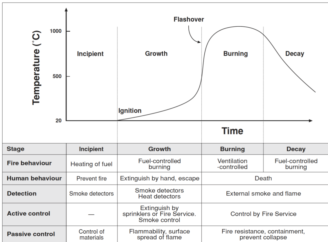
Figure 2.2. Typical fire development curve (Buchanan, 2001).
