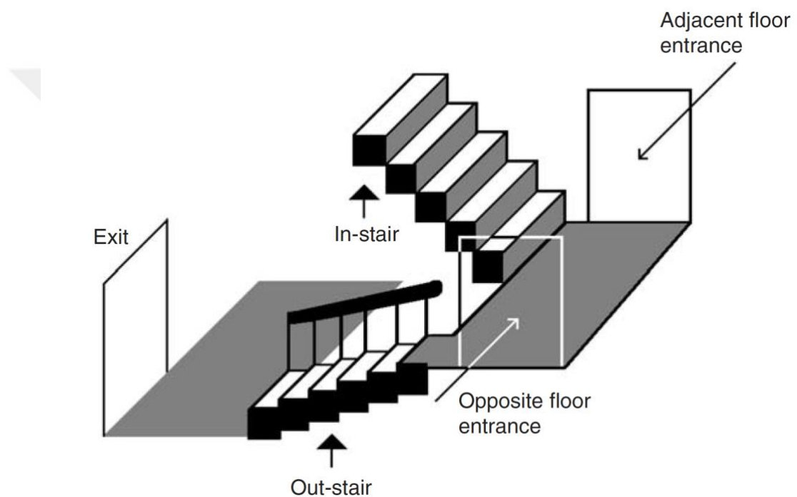
Figure 2.8. Adjacent and opposite floor-stair interface connections (Galea et al. , 2008).
