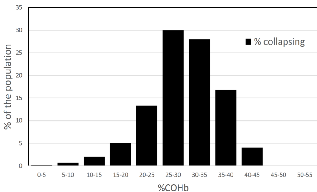
Figure 2.9. Population distribution of CO sensitivity to cause incapacitation (Purser and McAllister, 2016).
