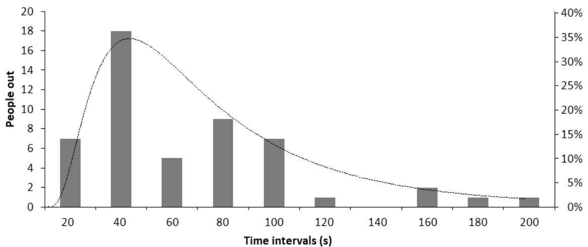
Figure 2.7. Response Time distribution of a Turkish sample (Galea et al. , 2011).
