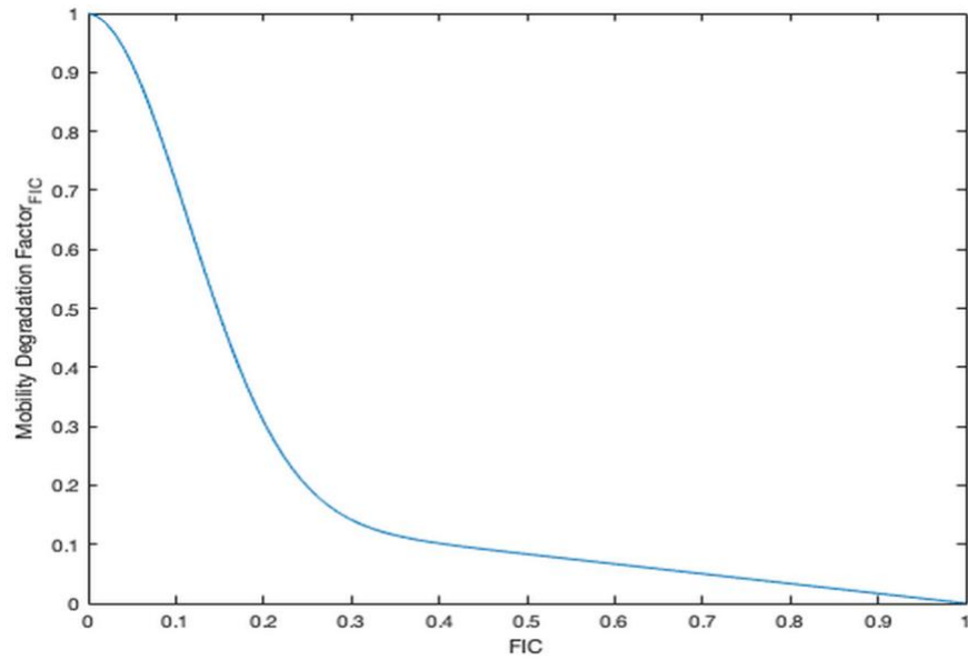
Figure 3.5. Mobility Degradation Factor for irritant gases.
