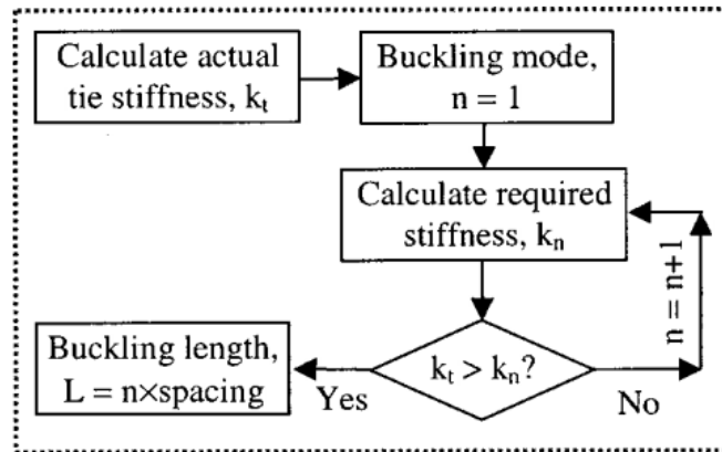
Figure 3.2. Flow-Chart of Buckling Length Determination (Dhakar and Maekawa, 2002b).
