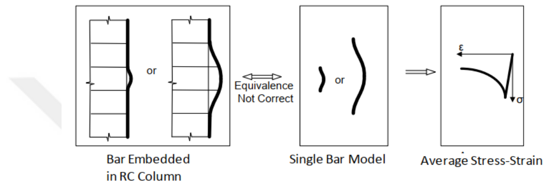
(a) Analogy is Correct for Local Buckling but Flawed for Global Buckling.
