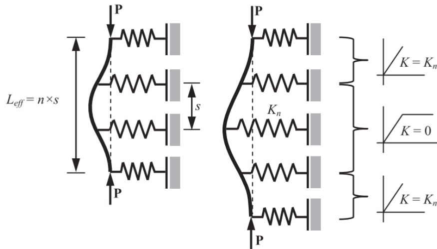
Figure 3.1. Simulation of Reinforcing Bars and Lateral Ties (Dhakar and Maekawa, 2002b).
