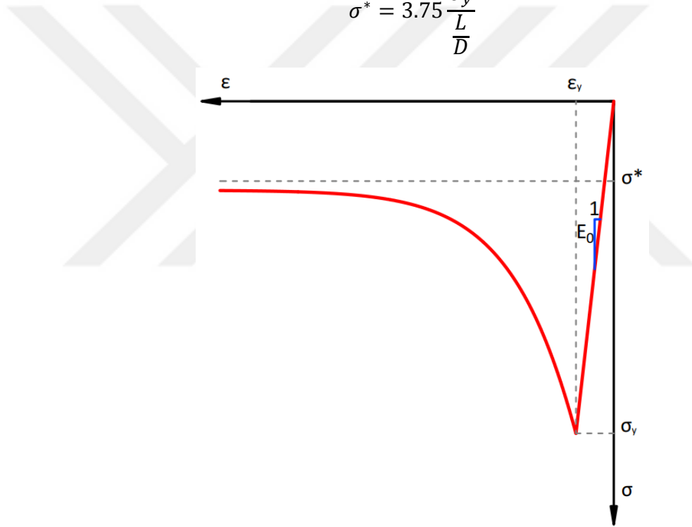
Figure 3.5. Compression Envelope (Kashani et al. , 2015a).
