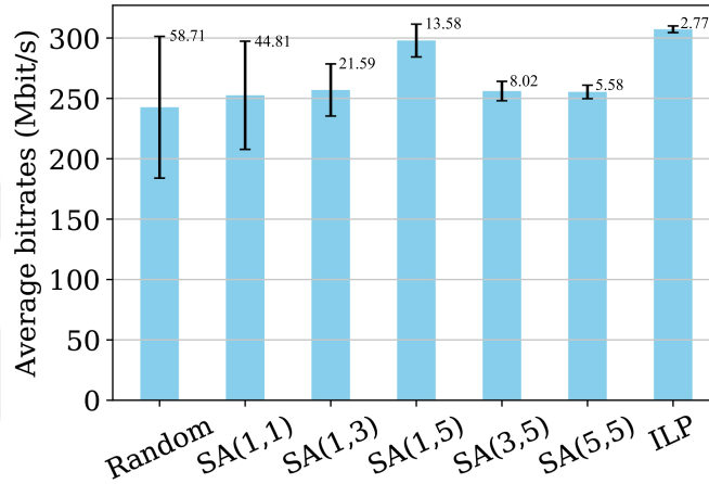
Figure 4.30. Average bitrates for switch failure with densely distributed flows.
