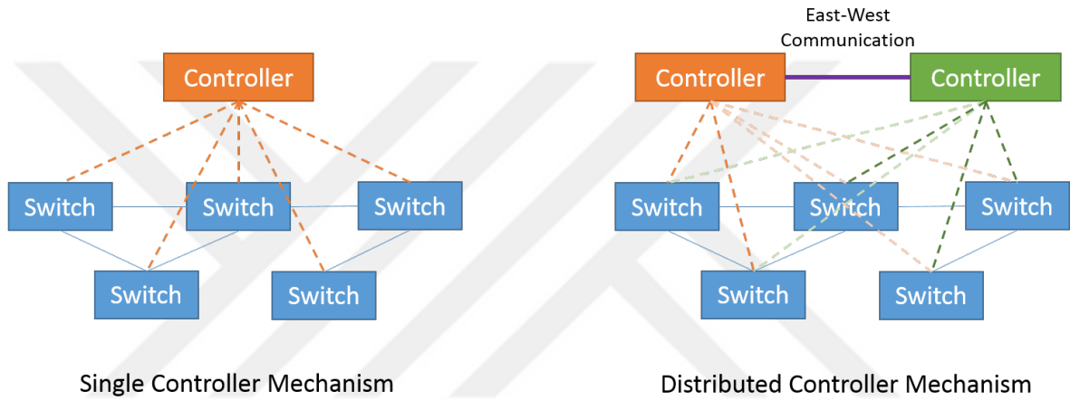
Figure 1.1. Single vs. distributed controller mechanism
