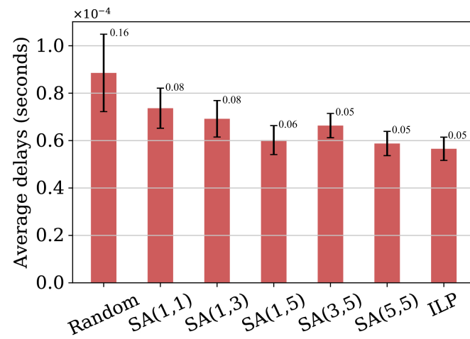
Figure 4.20. Average delays for only the flows during controller failure.
