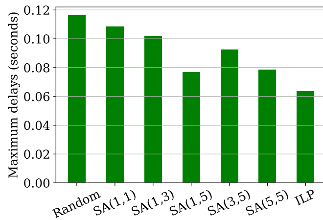
Figure 4.25. Average delays for link failure with sparsely distributed flows.
