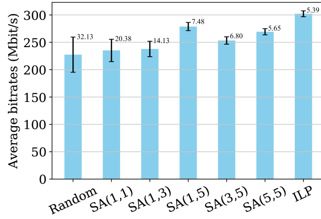
Figure 4.24. Average bitrates for link failure with sparsely distributed flows.
