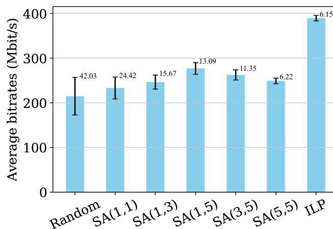
Figure 4.15. Average bitrates for only the flows during switch failure.
