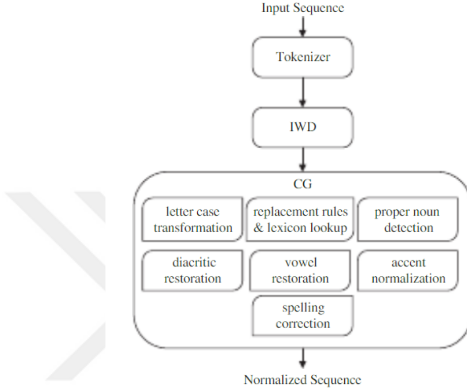
Figure 16: Normalization Architecture
