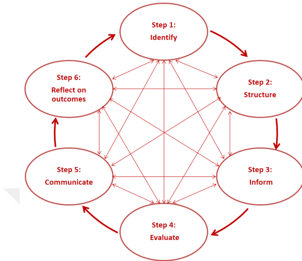
Figure 2-8 INTEGRAAL framework
