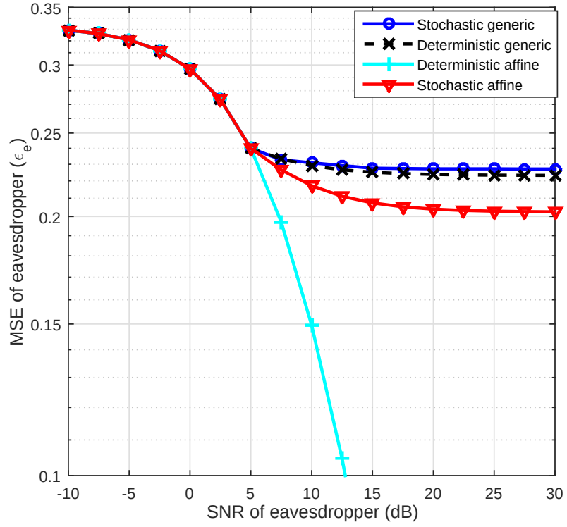
Figure 4.9: MSE of eavesdropper ( \epsilon_e ) versus SNR of eavesdropper when SNR of intended receiver is 5 dB, and estimation accuracy limit \alpha_2 is 0.24.
