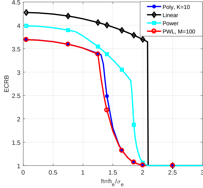
Figure 2.5: ECRB versus h for various solution approaches when \alpha = 0.15 with uniform prior distribution.
