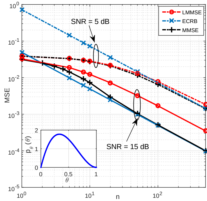
Figure 4.4: ECRB, LMMSE and MMSE versus n , where \theta has beta distribution with parameters (2, 3) in [0, 1] .
