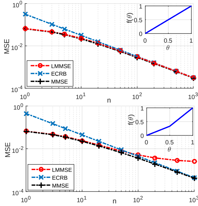
Figure 4.2: ECRB, LMMSE and MMSE versus n for two simple encoding scenarios.
