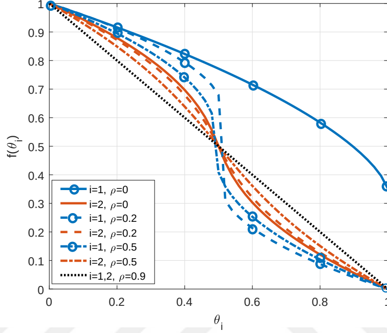
Figure 3.3: The optimal encoding functions for \theta_1 and \theta_2 for \rho = \{0, 0.2, 0.5, 0.9\} when h_{e,1} = 1.2 .
