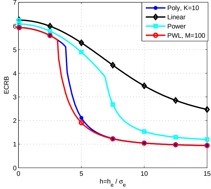
Figure 2.8: ECRB versus h for various solution approaches when \alpha = 0.34 for w(\theta) = 2\theta for \theta \in [0, 1] .
