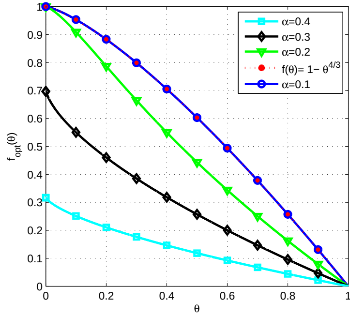
Figure 2.7: f_{\text{opt}}(\theta) versus \theta for piecewise linear approximation ( M = 100 ), where \alpha = 0.1, 0.2, 0.3 , and 0.4 . f(\theta) = 1 - \theta^{4/3} is the optimal function under no secrecy constraints according to Proposition 1.
