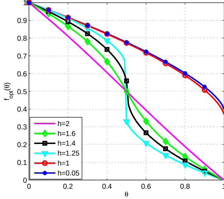
Figure 2.6: f_{opt}(\theta) versus \theta for the piecewise linear approximation when \alpha = 0.15 with uniform prior distribution.
