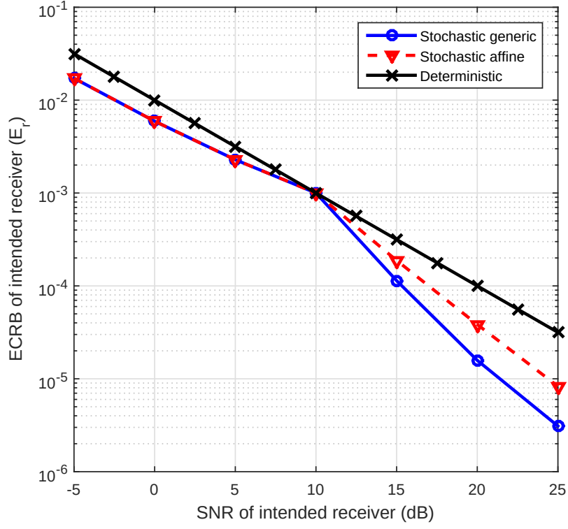
Figure 4.11: ECRB of intended receiver ( E_r ) versus SNR of intended receiver when SNR of eavesdropper is 10 dB, and target secrecy level \eta_1 is 0.001.
