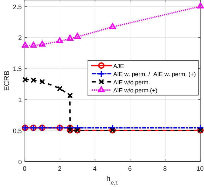
Figure 3.9: Total ECRB versus h_{e,1} for different approaches.
