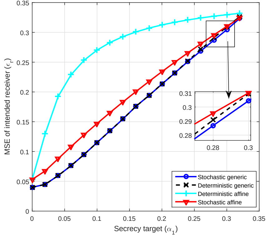
Figure 4.6: MSE of intended receiver ( \epsilon_r ) versus secrecy target ( \alpha_1 ) when SNRs of eavesdropper and intended receiver are 15 and 5 dB, respectively.
