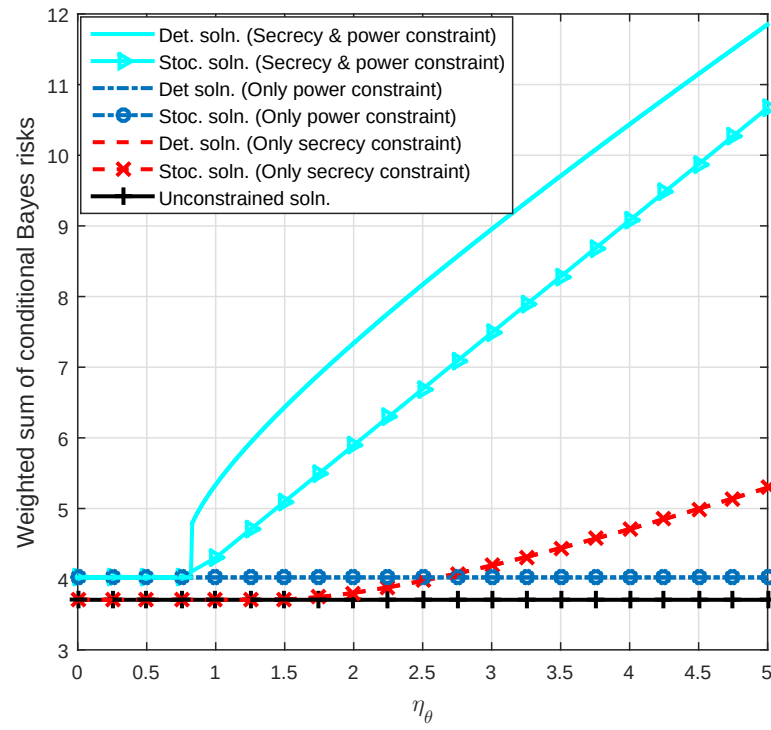
Figure 5.3: Weighted sum of conditional Bayes risks versus \eta_\theta .
