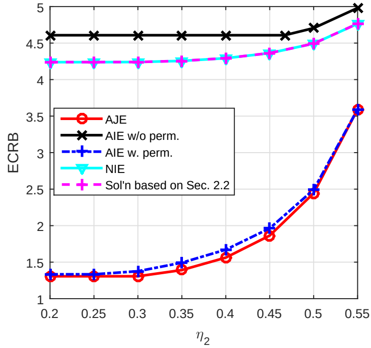
Figure 3.11: Total ECRB versus \eta_2 for different approaches.
