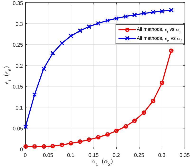
Figure 4.10: \epsilon_r versus \alpha_1 and \epsilon_e versus \alpha_2 when SNRs of eavesdropper and intended receiver are 5 and 15 dB, respectively.
