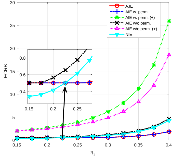
Figure 3.10: Total ECRB versus \eta_1 for different approaches.
