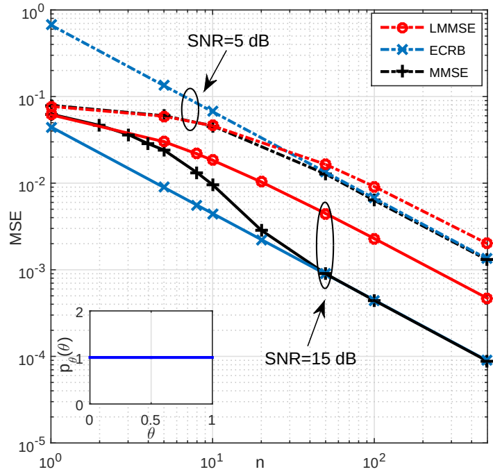
Figure 4.3: ECRB, LMMSE and MMSE versus n , where \theta has uniform distribution in [0,1] .
