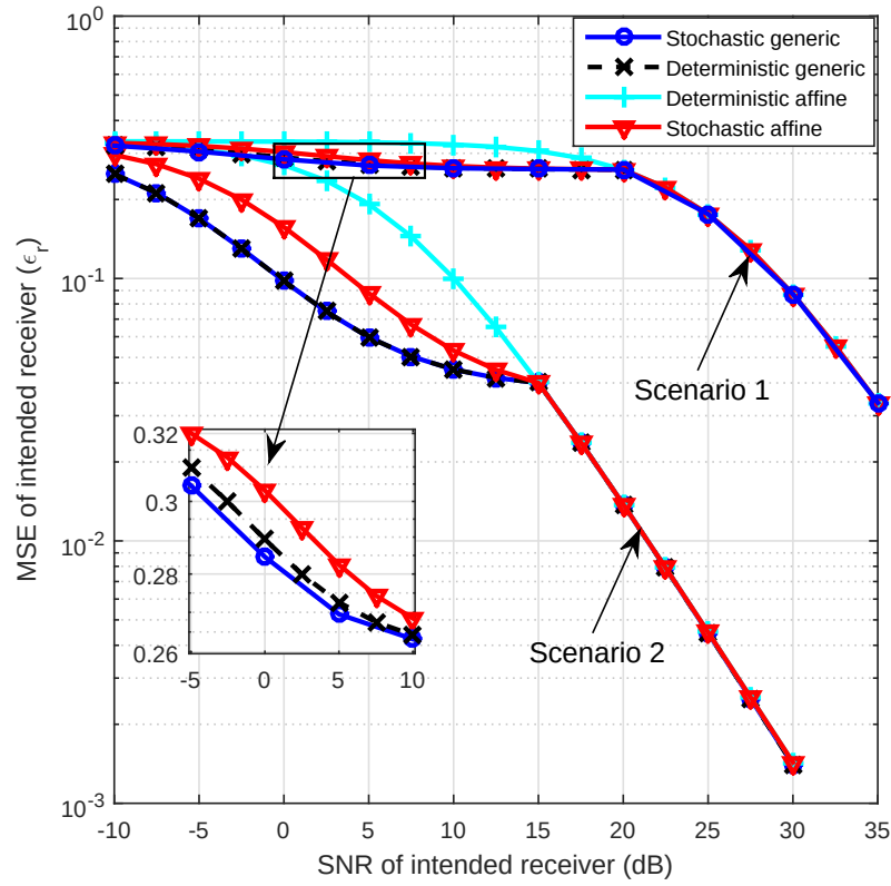
Figure 4.5: MSE of intended receiver ( \epsilon_r ) versus SNR of intended receiver for two different scenarios.
