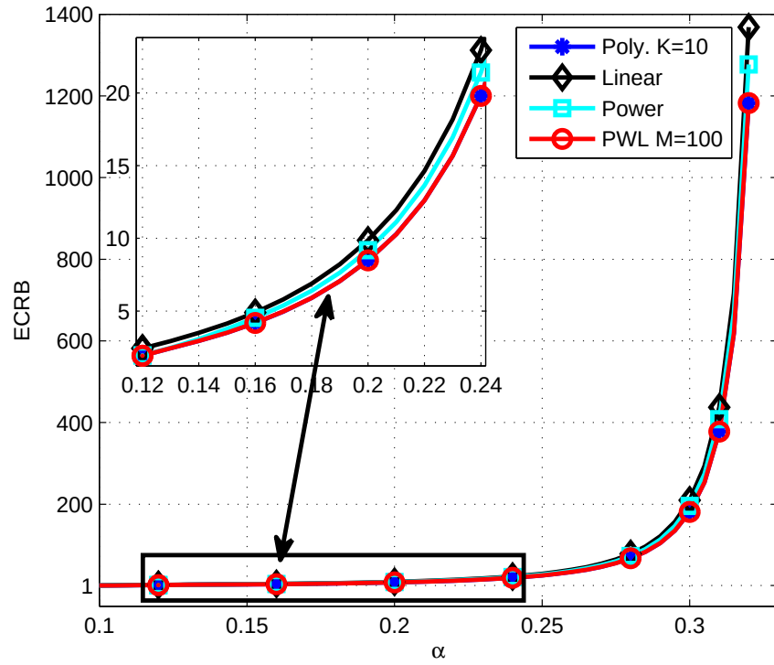
Figure 2.3: ECRB versus \alpha for various solution approaches, where h = 1 and 0.1 \leq \alpha \leq 0.32 .
