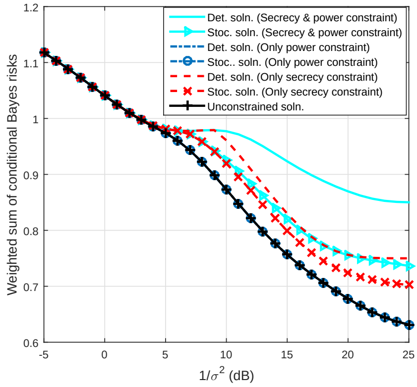
Figure 5.5: Weighted sum of conditional Bayes risks versus 1/\sigma^2 for different scenarios.
