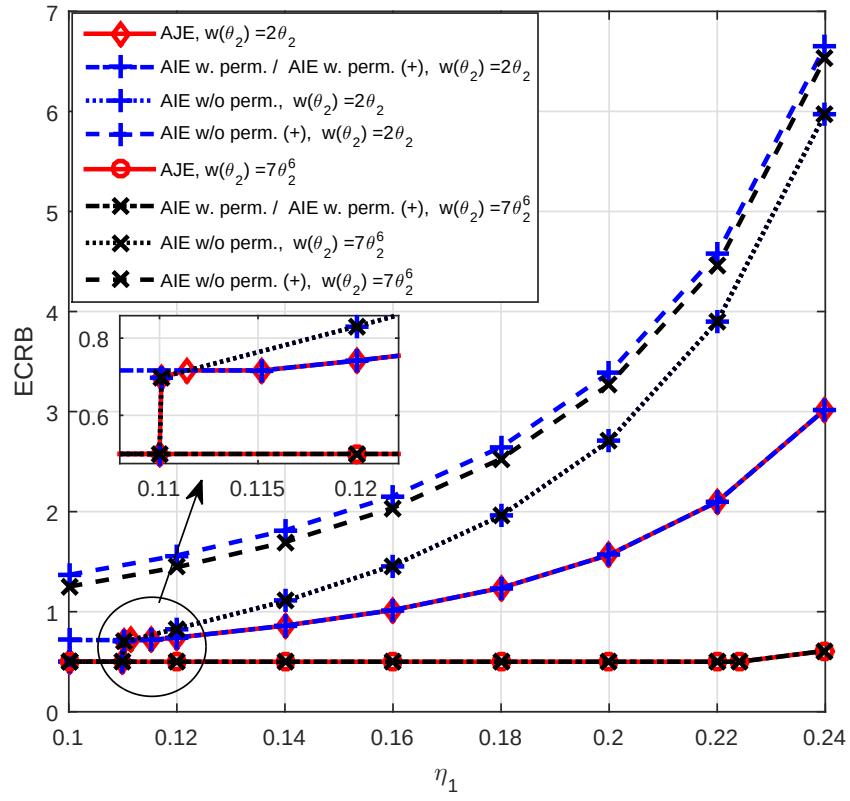
Figure 3.8: Total ECRB versus \eta_1 for different approaches.
