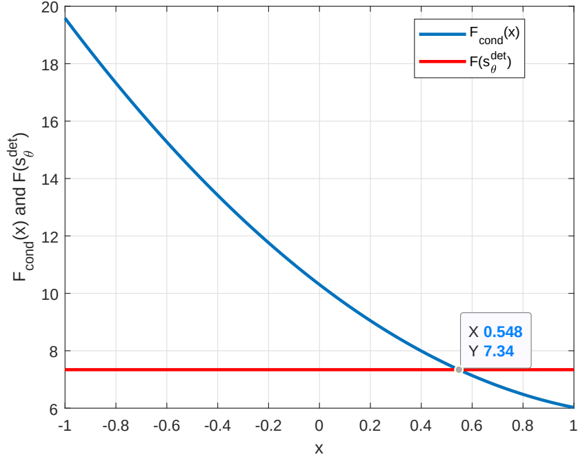
Figure 5.4: For x \in [0.548, 1] , F_{cond}(x) < F_{\theta}(s_{\theta}^{det}) = 7.340 .
