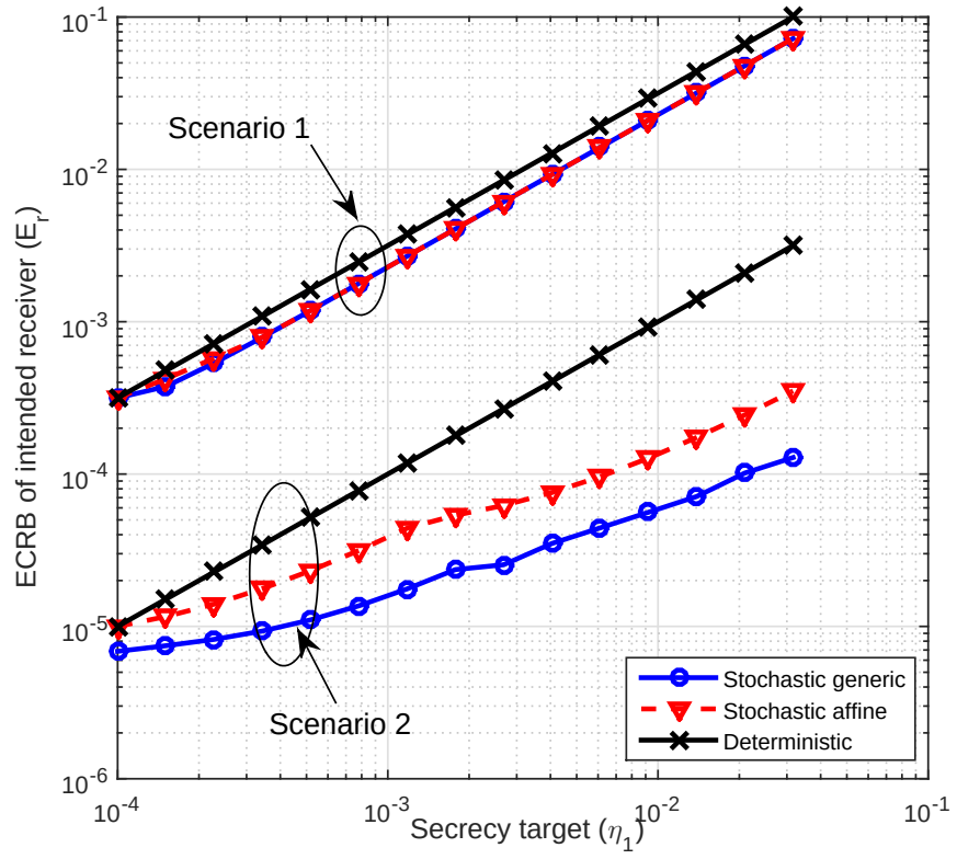
Figure 4.13: ECRB of intended receiver ( E_r ) versus secrecy target ( \eta_1 ) for two different scenarios.
