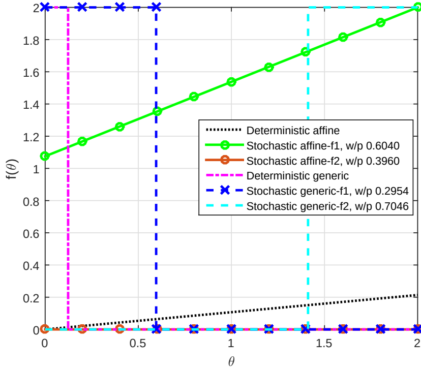
Figure 4.7: Optimal encoding functions for different strategies when SNRs of eavesdropper and intended receiver are 10 and 0 dB, respectively, and secrecy target \alpha_1 is 0.28.
