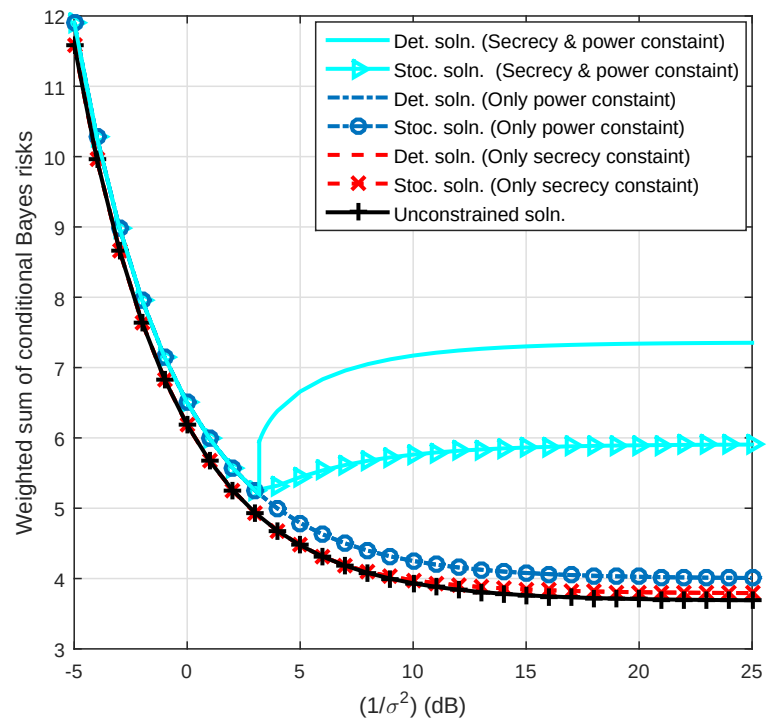
Figure 5.2: Weighted sum of conditional Bayes risks versus 1/\sigma^2 .
