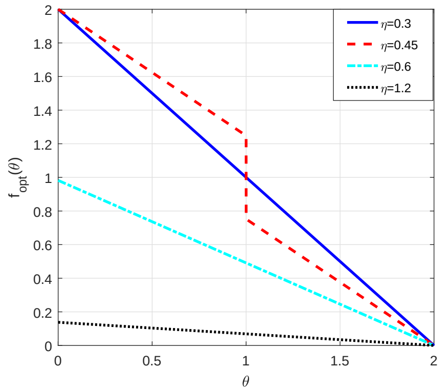
Figure 2.11: f_{\text{opt}}(\theta) versus \theta for h = 0.5 .
