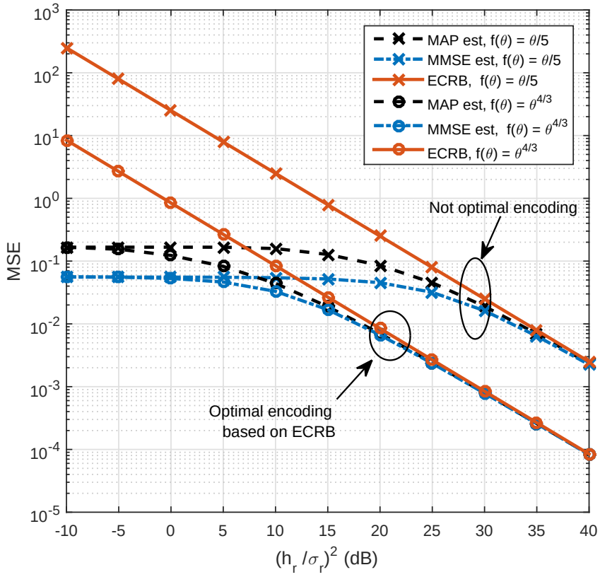
Figure 2.2: MSE versus (h_r/\sigma_r)^2 for MMSE, MAP estimators and ECRB when an optimal and non-optimal encoding functions are used for w(\theta) = 2\theta for \theta \in [0, 1] . Note that h_r = 1 .
