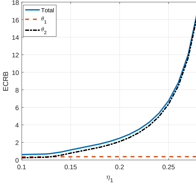
Figure 3.4: Total and individual ECRB values versus \eta_1 .
