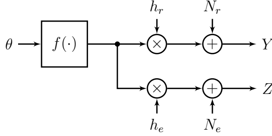
Figure 2.1: System model for the parameter encoding problem.
