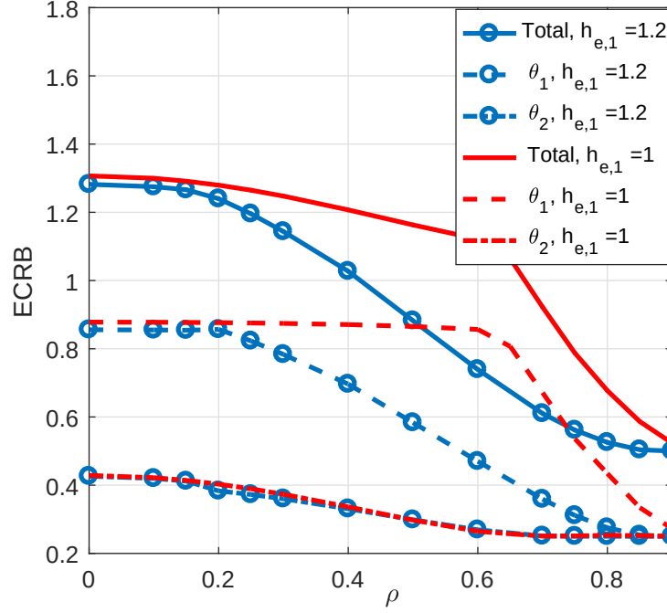
Figure 3.2: Total and individual ECRB values versus \rho for h_{e,1} = 1 and h_{e,1} = 1.2 .
