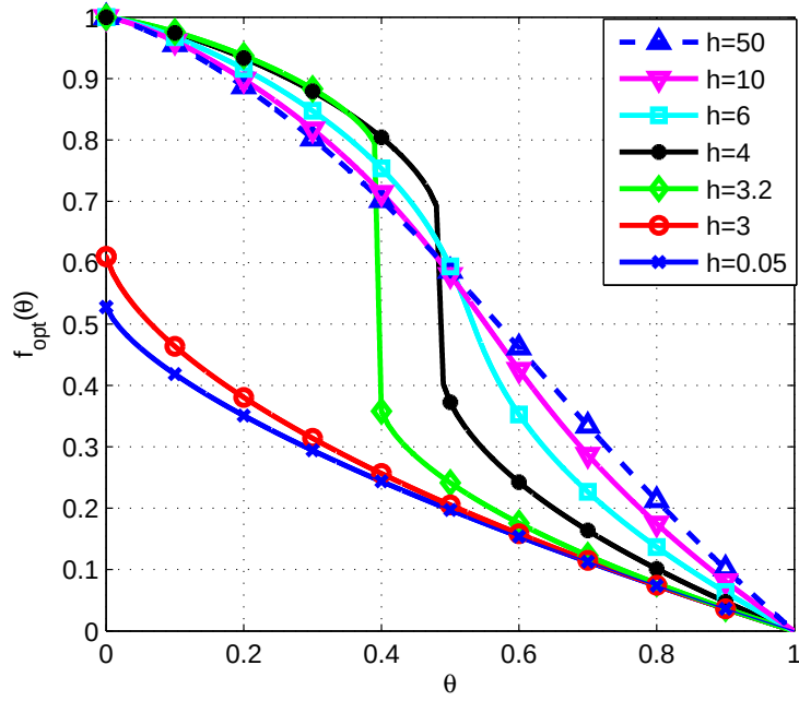
Figure 2.9: f_{opt}(\theta) versus \theta for piecewise linear approximation when \alpha = 0.34 with w(\theta) = 2\theta for \theta \in [0, 1] .
