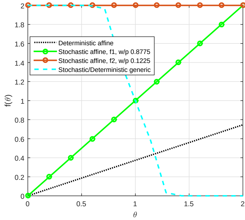
Figure 4.8: Optimal encoding functions for different strategies when SNRs of eavesdropper and intended receiver are 15 and 5 dB, respectively, and secrecy target \alpha_1 is 0.04.
