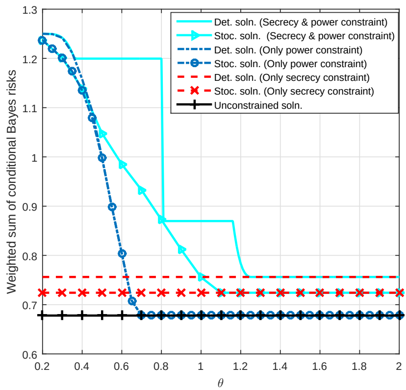
Figure 5.6: Weighted sum of conditional Bayes risks versus \theta for different scenarios.
