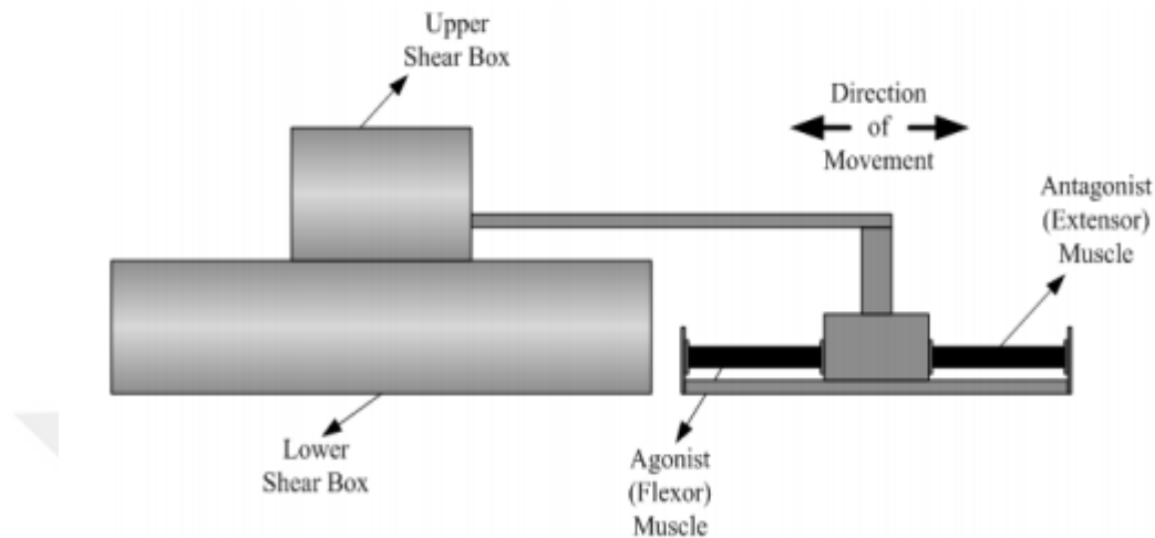
Figure 3.6. The drawing of cyclic actuator [41].
