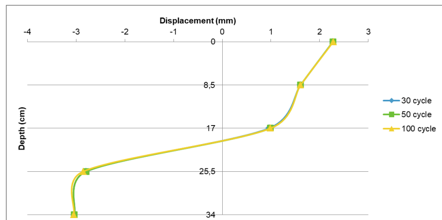
Figure 4.42. Displacement of the Segmental Pile with Post-Tension Force 2250 N in Medium-Dense Soil.
