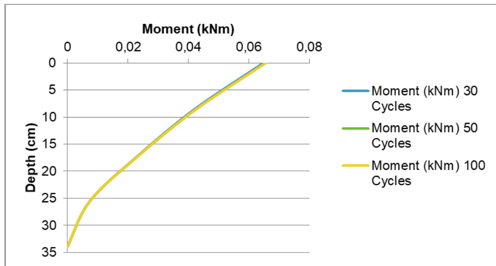
Figure 4.63. Moment of the Segmental Pile with Post-Tension Force 750 N in Loose Soil.
