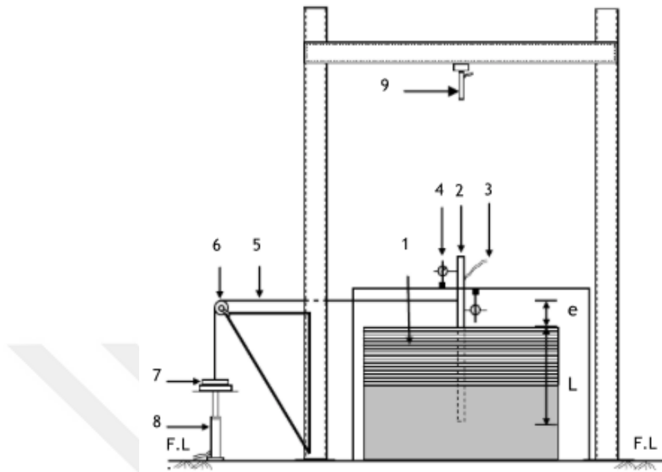
Figure 2.4. Experimental set-up schematic diagram [26].
