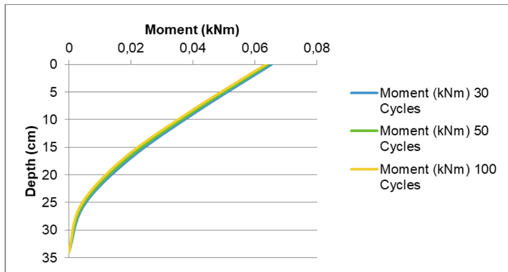
Figure 4.69. Moment of the Segmental Pile with Post-Tension Force 2250 N in Loose Soil.
