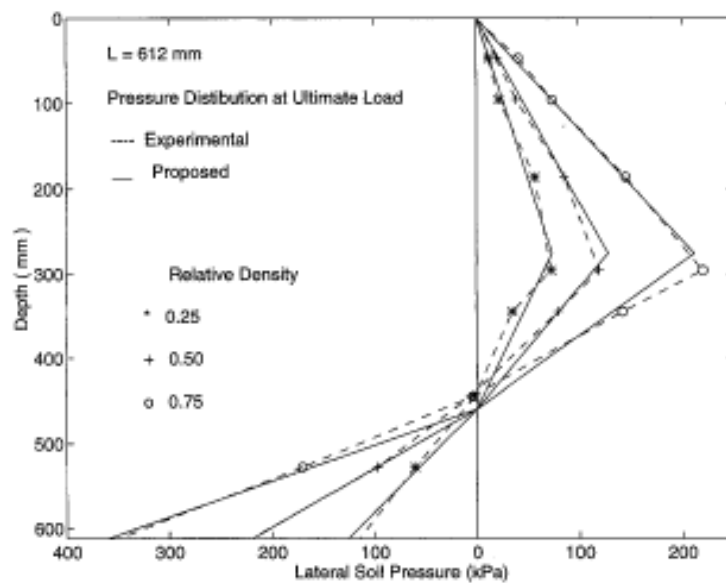
Figure 2.3. Soil pressure versus depth [25].
