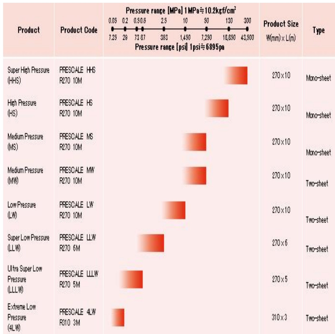
Figure 2.28. Different types of prescale films with different pressure range[35].
