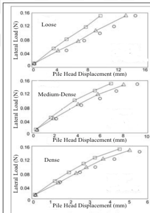
Figure 2.23. Load versus displacement [12].
