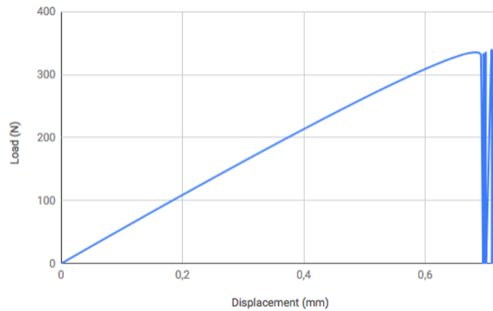
Figure A.11. Mortar Beam in Medium-Dense Soil.
