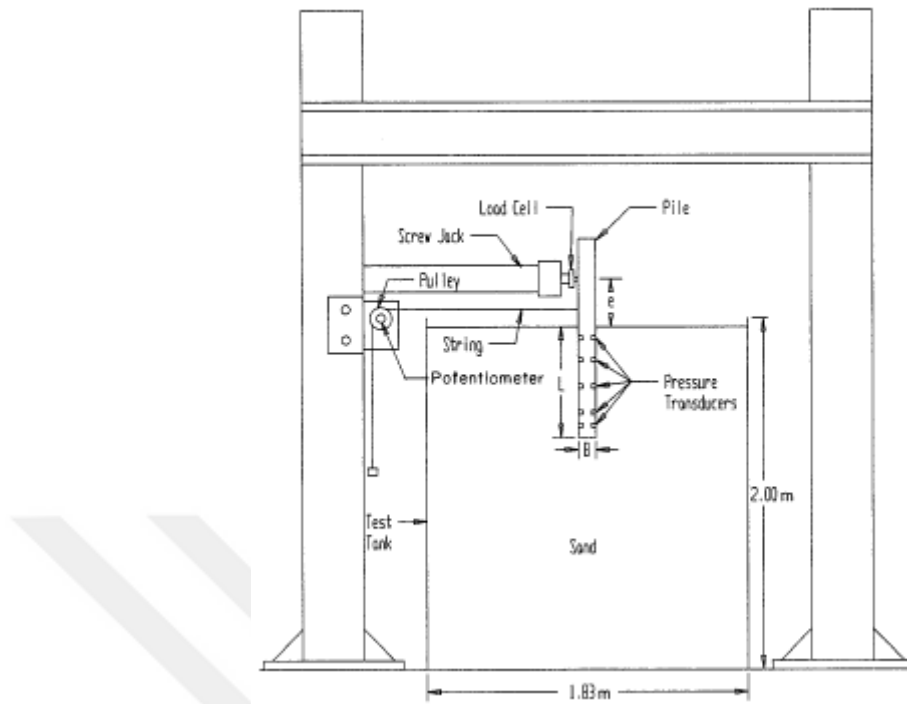
Figure 2.1. Experimental set-up schematic diagram [25].
